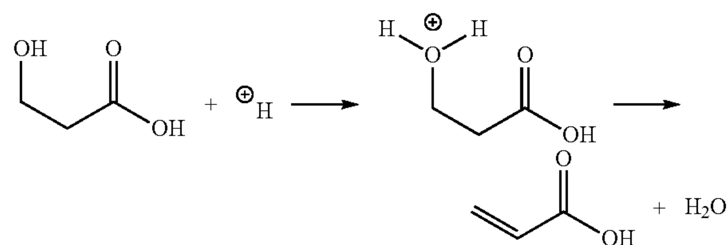
Scheme 2
