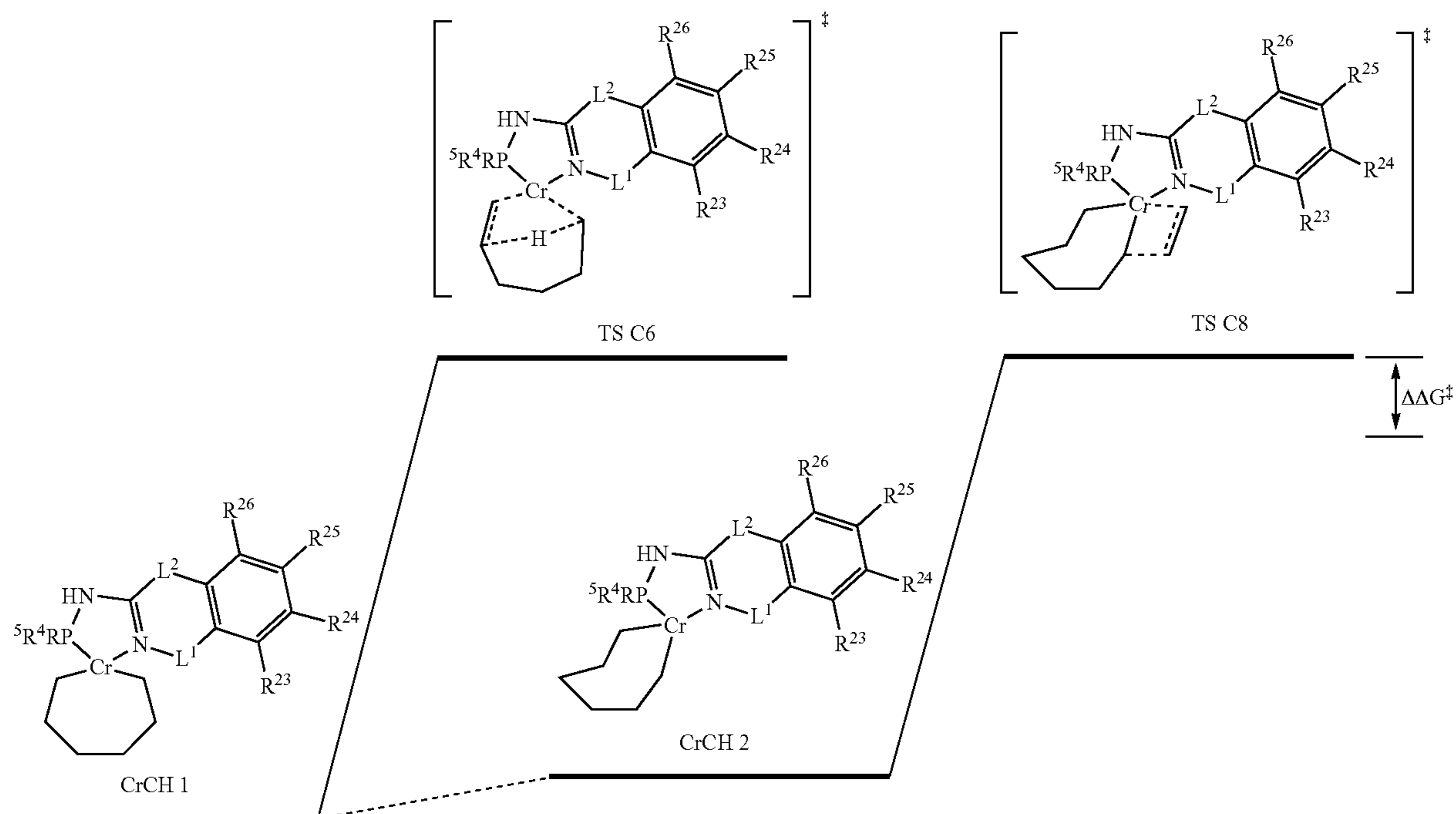
Scheme 3
