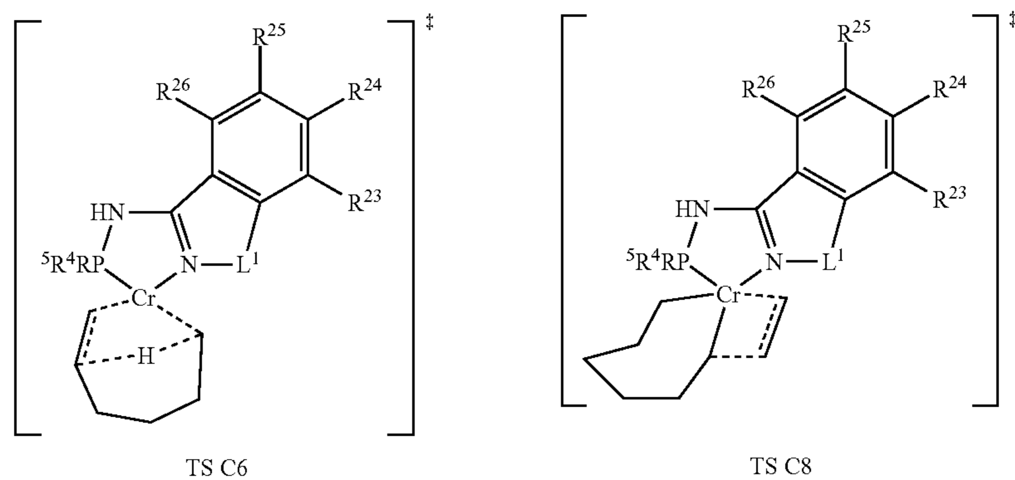
Scheme 2
