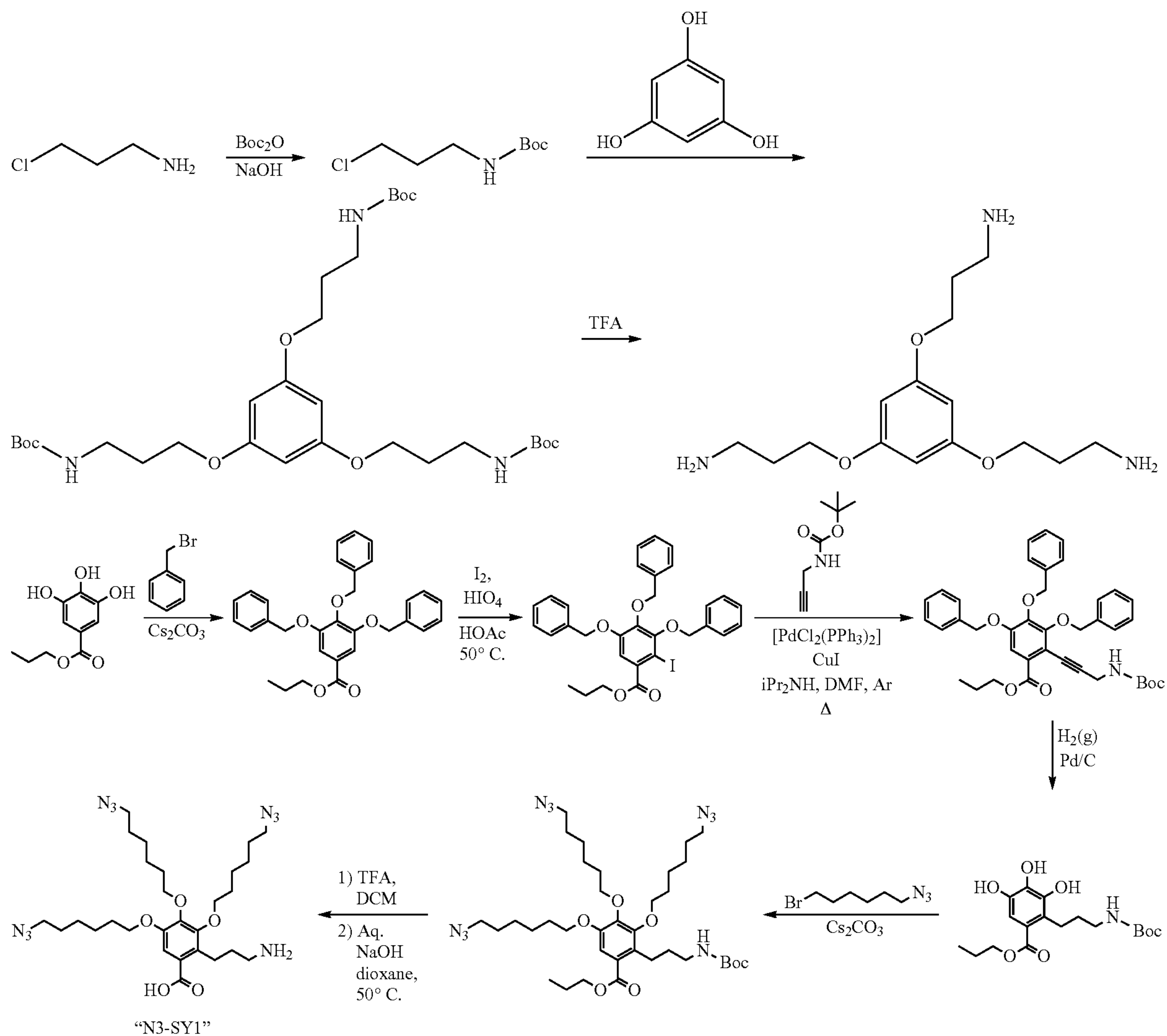
Scheme 14
