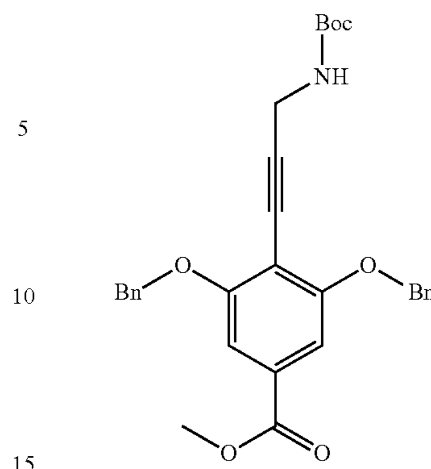
Methyl 3,5-bis(benzyloxy)-4-(3-((tert-butoxy)carbonyl)amino}prop-1-yn-1-yl)benzoate (4-6)
