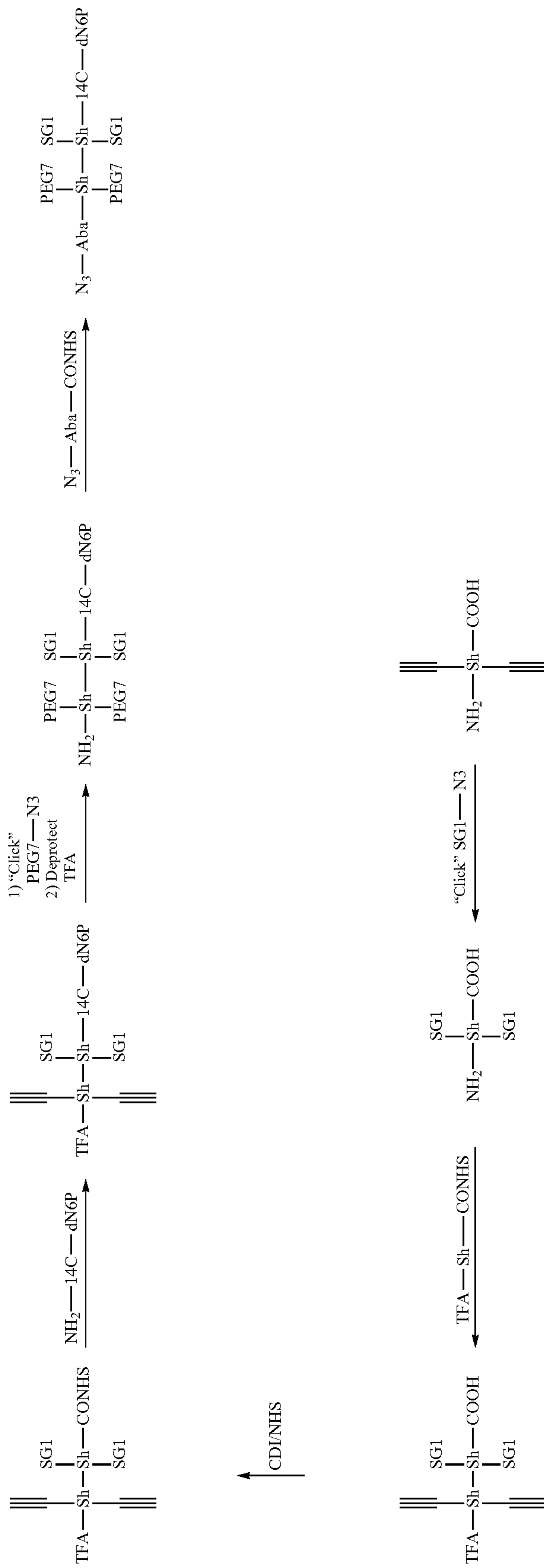
Scheme 7-2
