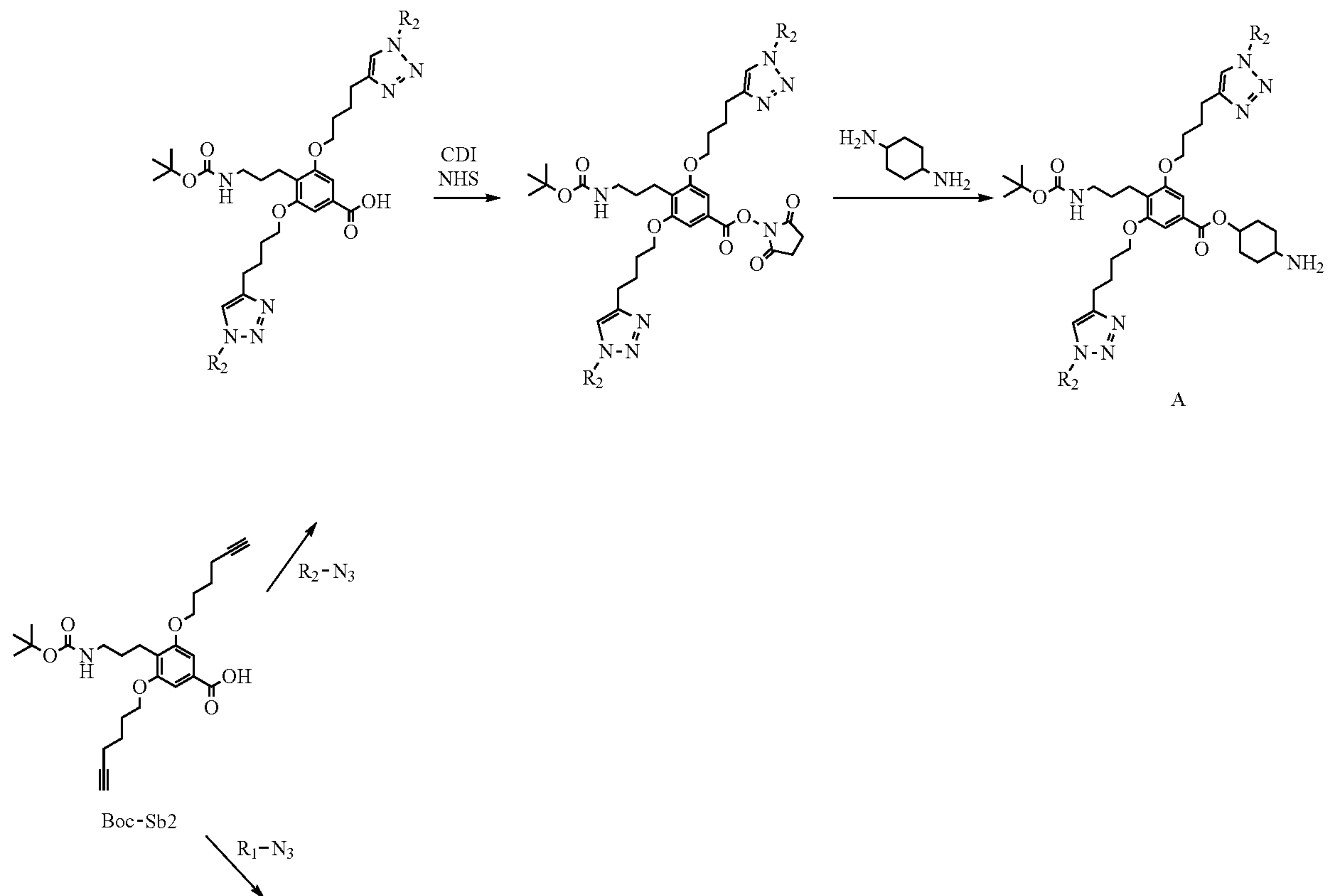
Scheme 7-5
