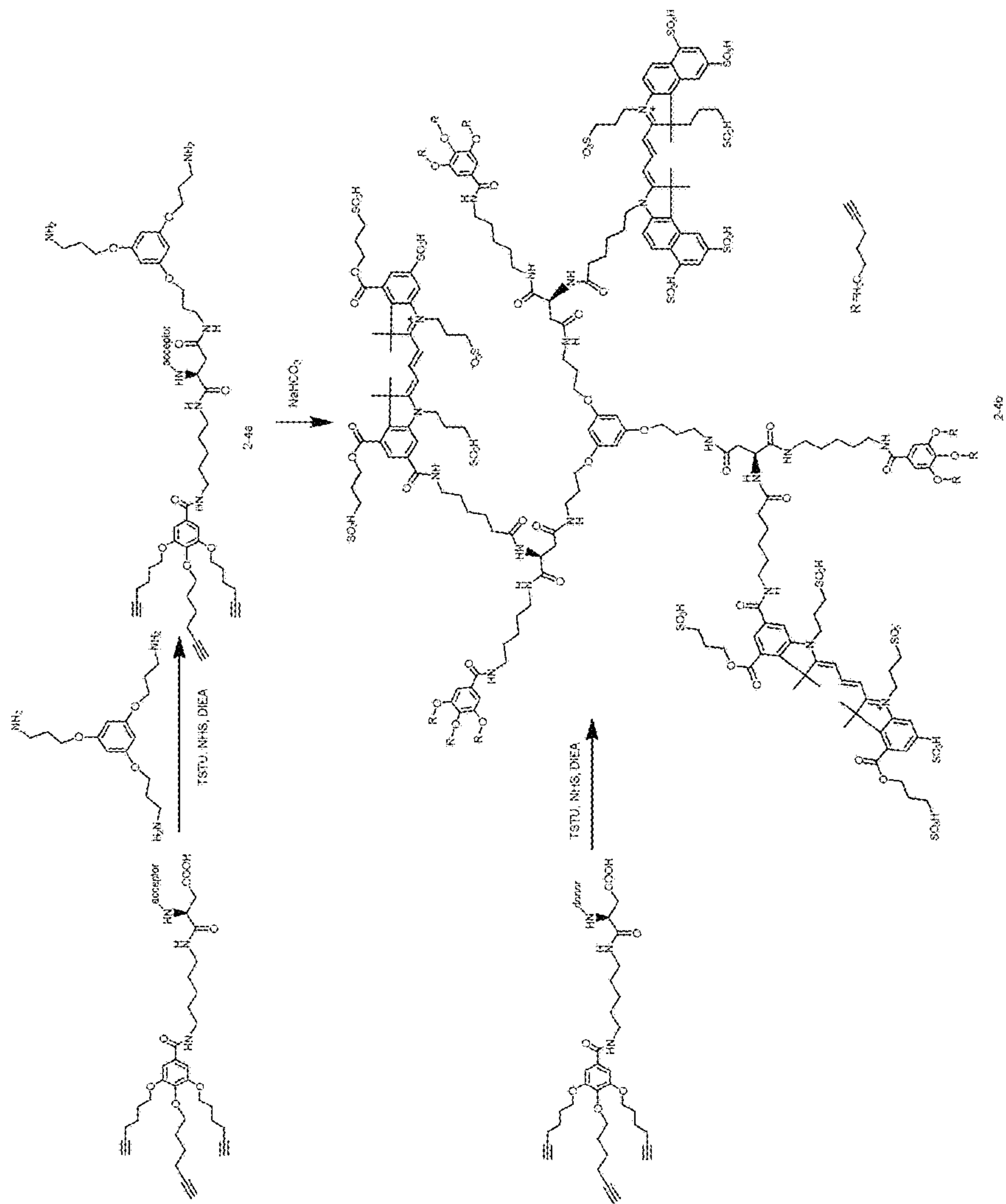
Scheme 24
