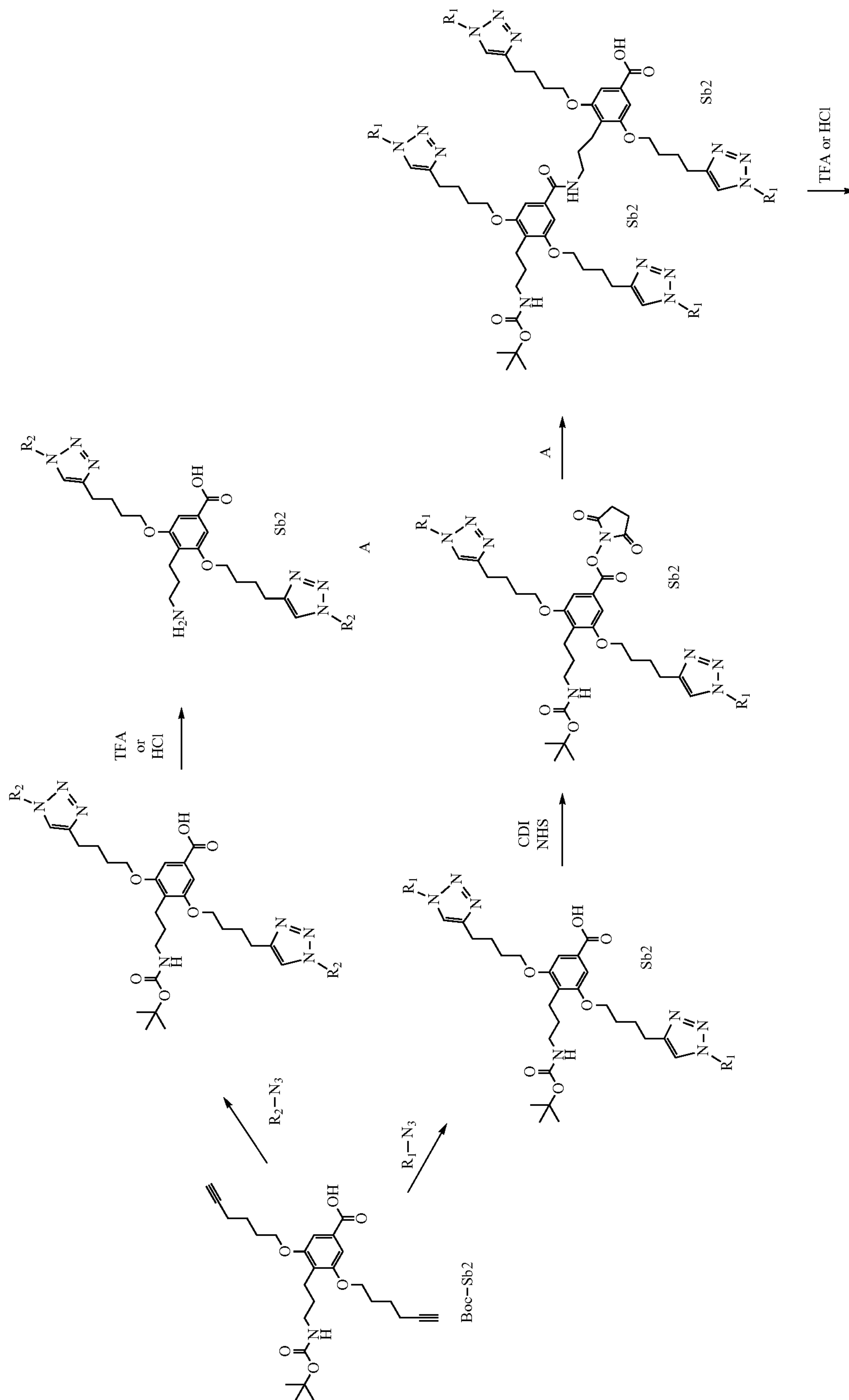
Scheme 15-1
