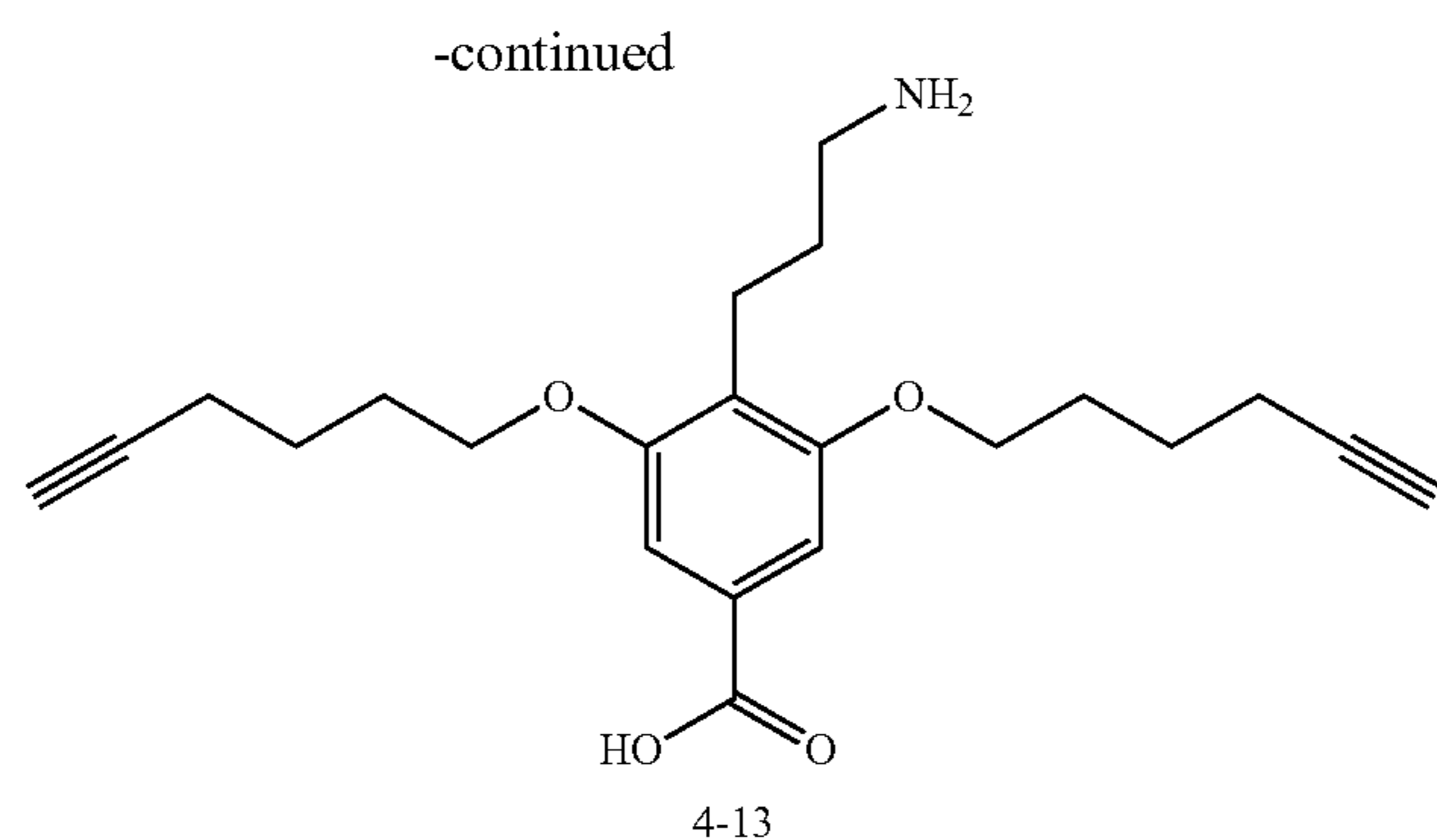
4-(3-Aminopropyl)-3,5-bis(hex-5-ynoxy)benzoic acid, "Sb2" (4-13)
