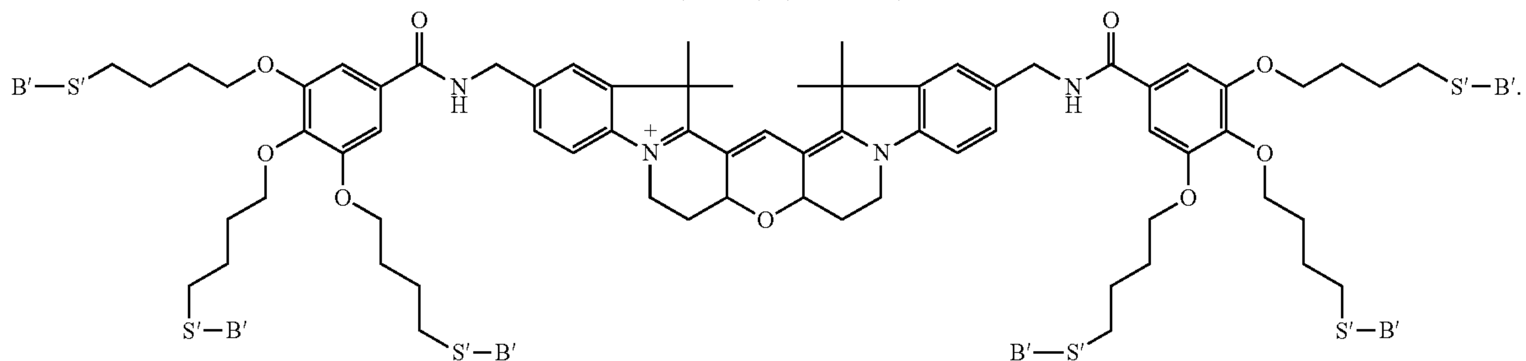
D012-(Gal) 2 (Hexavalent)
