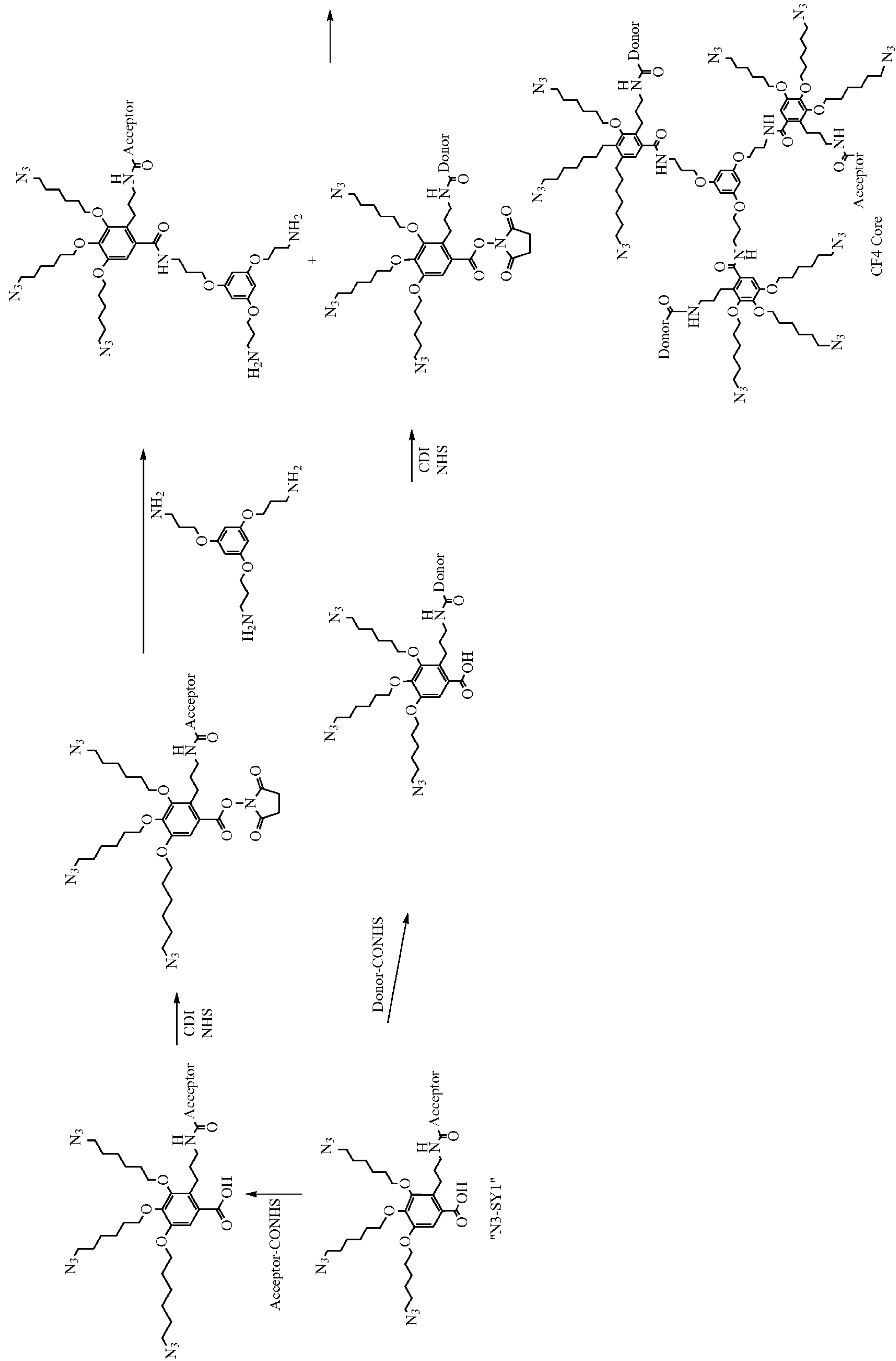
Scheme 12
