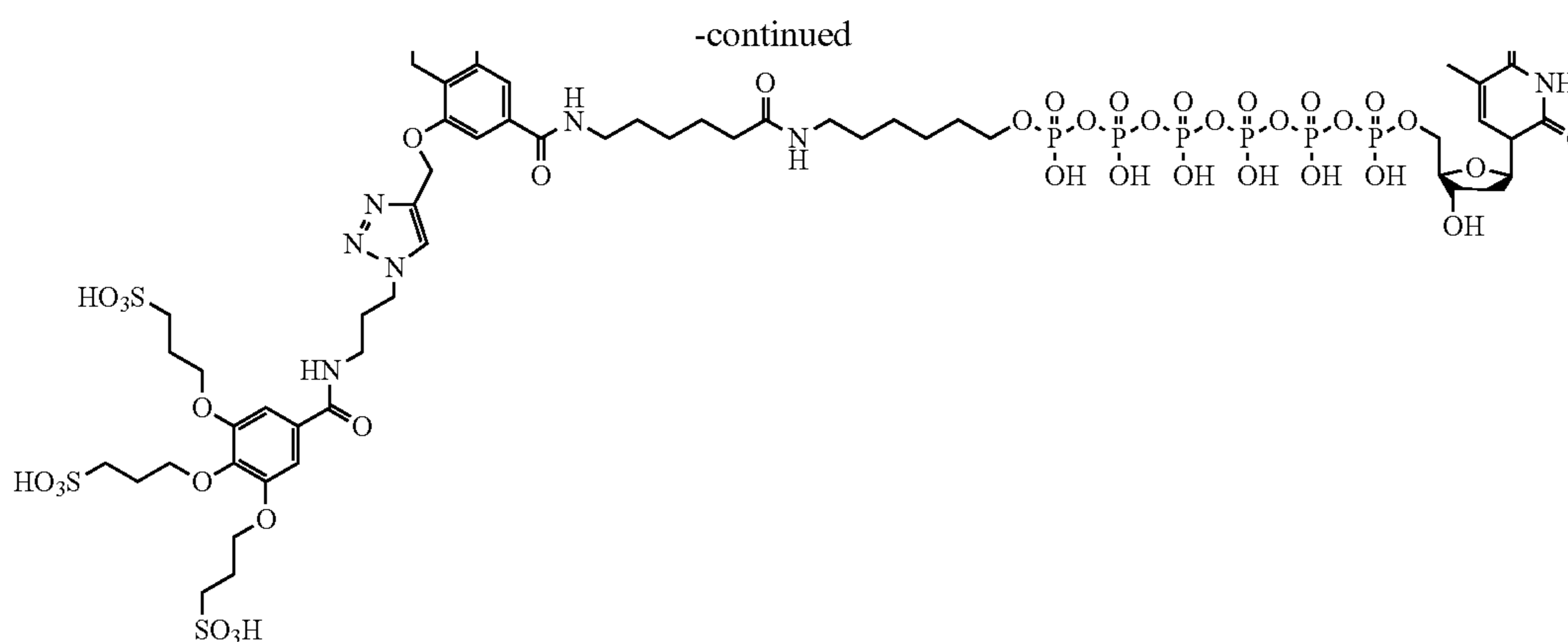
NH 2 -Sh(SG1) 2 -14C-dT6P (5-5)
