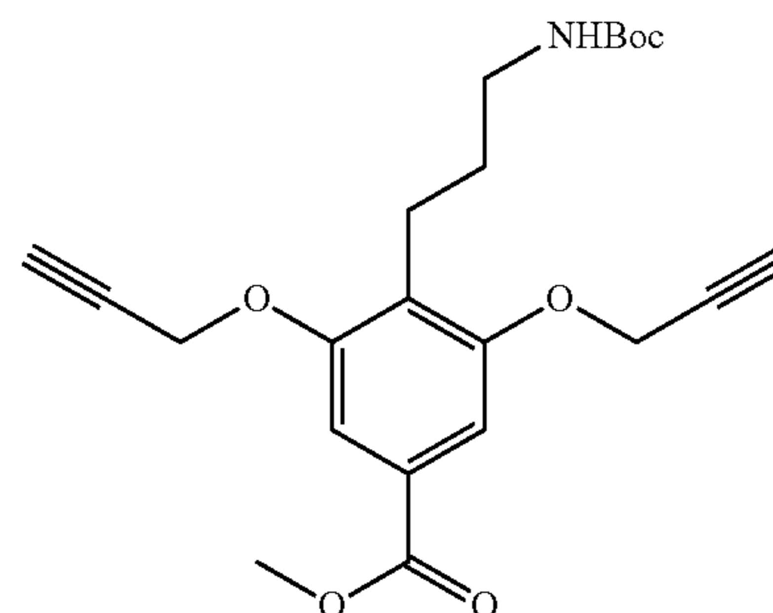
Methyl 4-(3-((tert-butoxy)carbonyl)amino}propyl)-3,5-bis(prop-2-yn-1-yloxy)benzoate (4-9)
