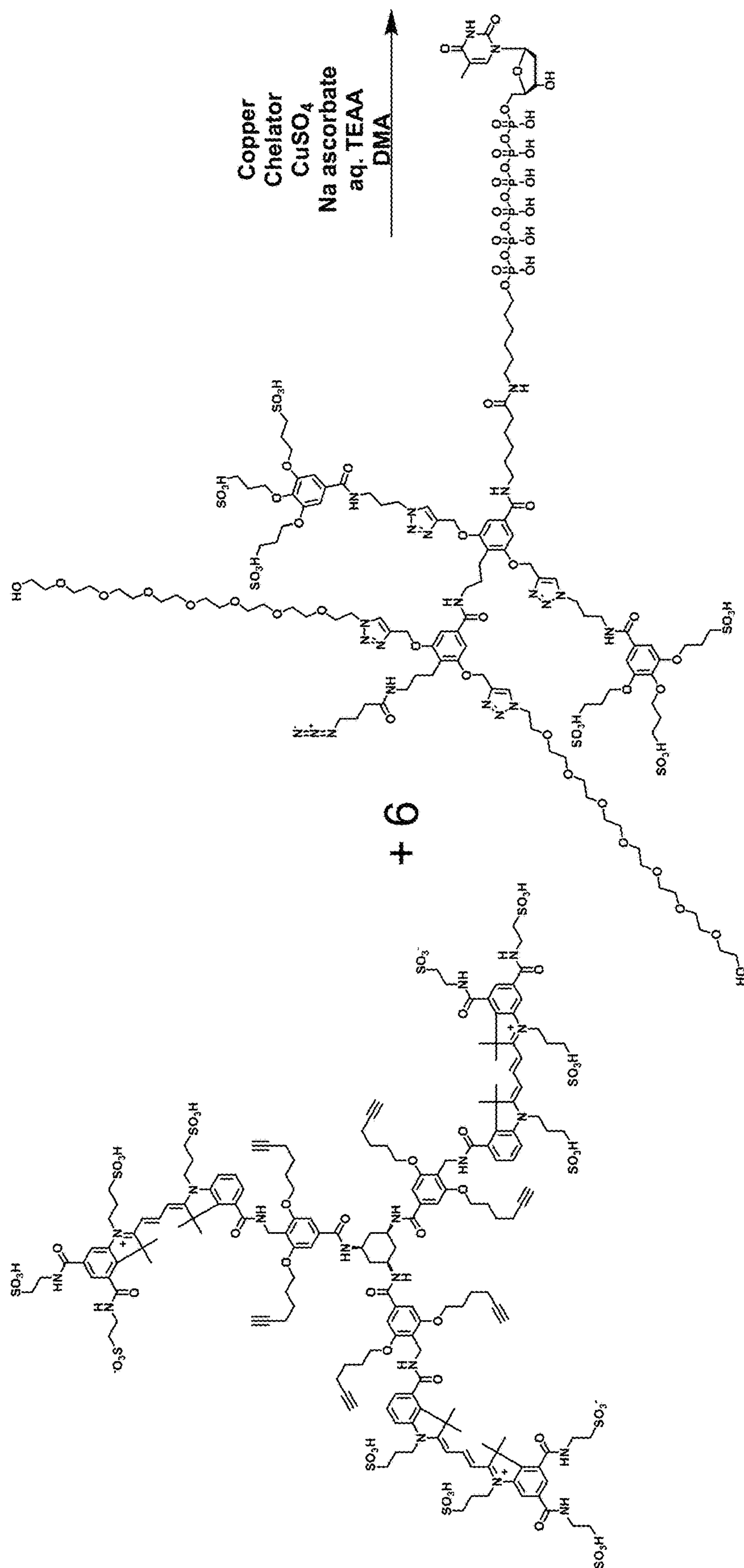
Scheme 9
