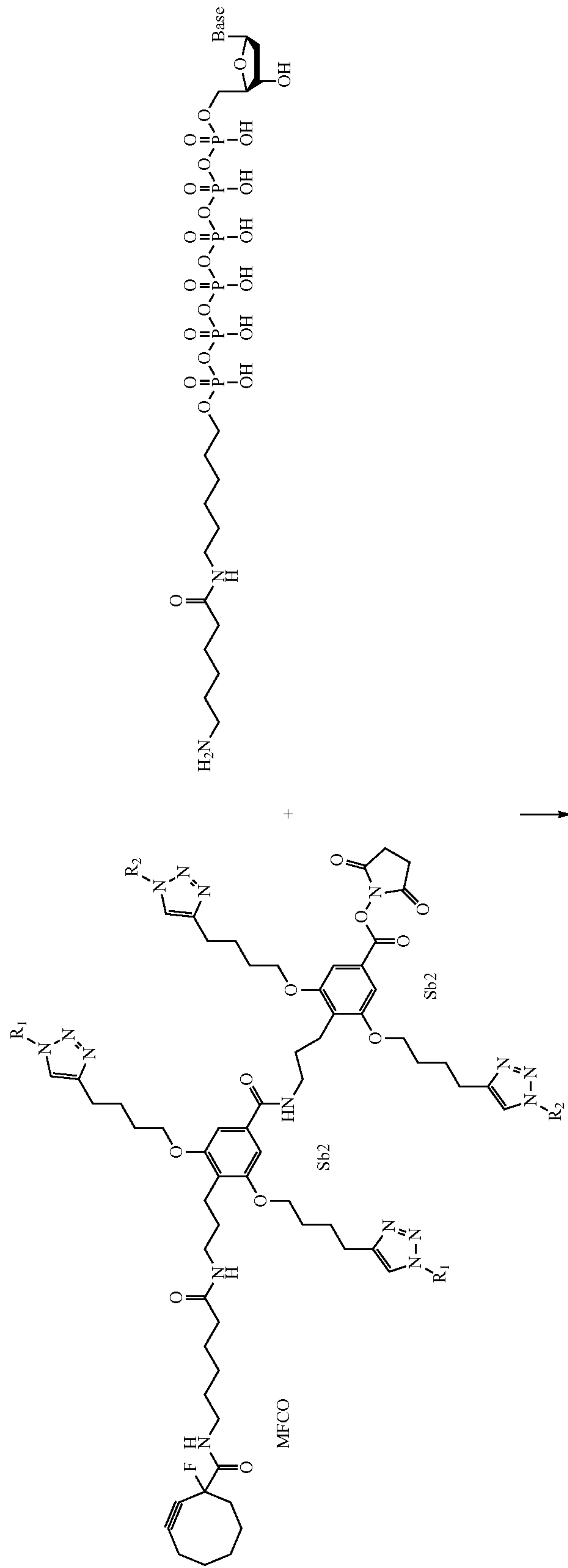
Scheme 15-2
