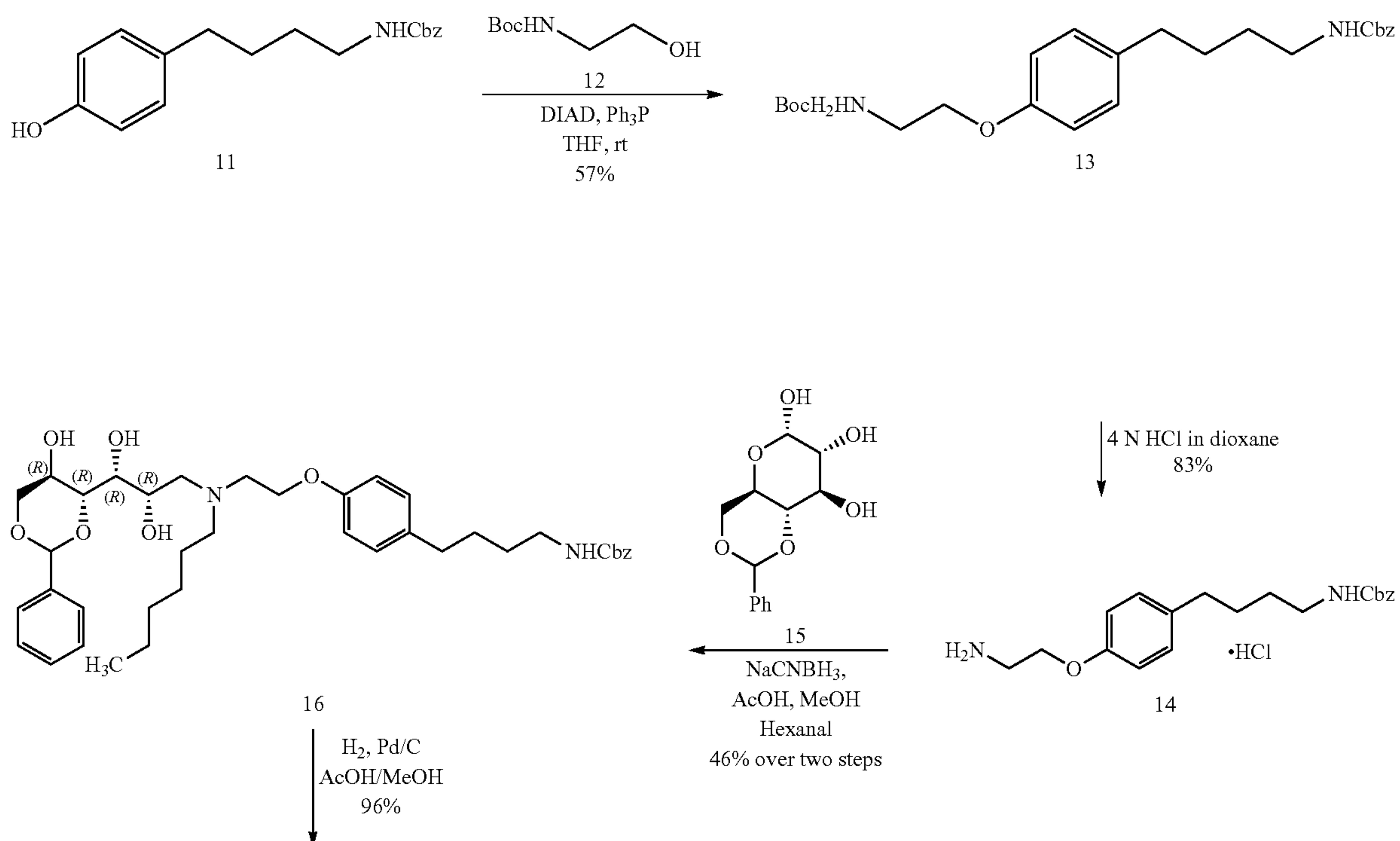
Scheme 2. Preparation of 3,5-Diamino-6-chloro-N-(N-(4-(4-(2-(hexyl((2S,3R,4R,5R)-2,3,4,5,6-pentahydroxyhexyl)amino)ethoxy)phenyl)butyl)carbaminimidoyl)pyrazine-2-carboxamide
