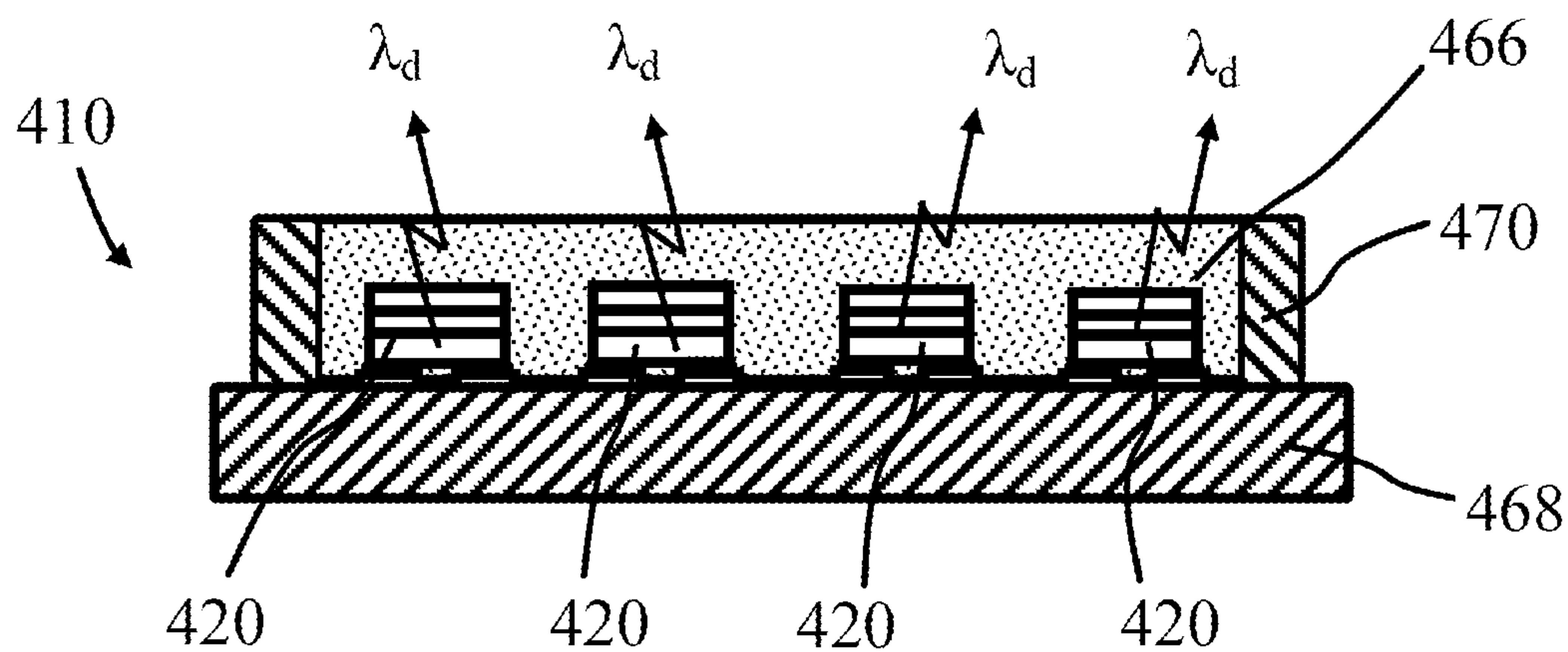
SECTION B-B
