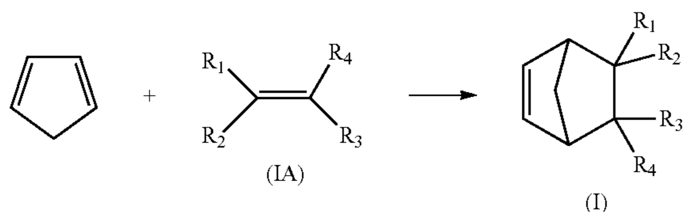
Scheme I
