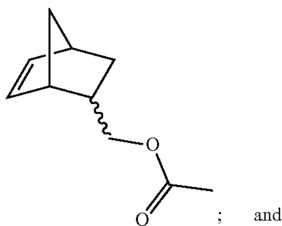
(bicyclo[2.2.1]hept-5- en-2-yl) methyl acetate (NBMeOAc)
