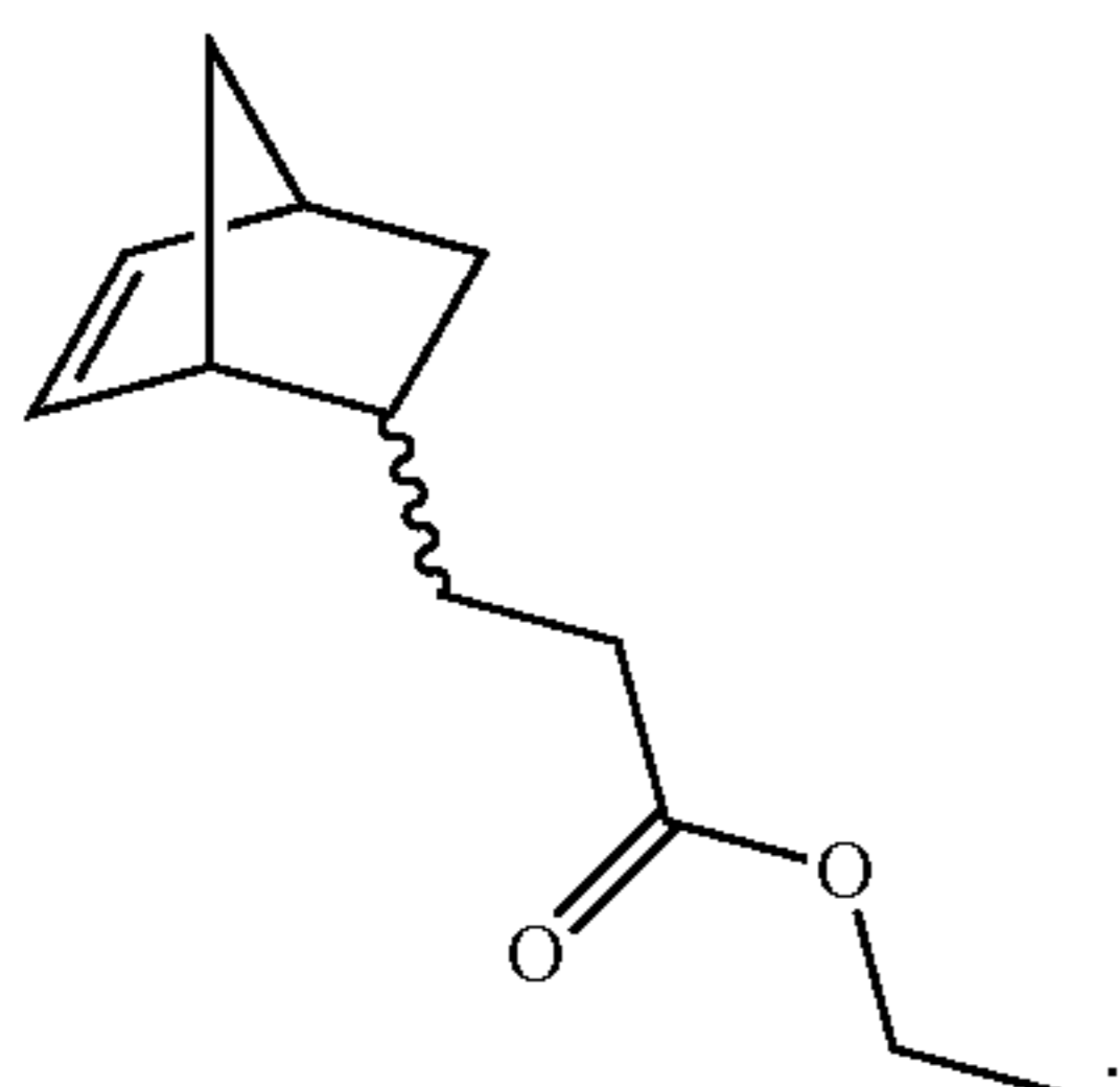
ethyl 3-(bicyclo[2.2.1]hept-5- en-2-yl)propanoate (EPEsNB)
