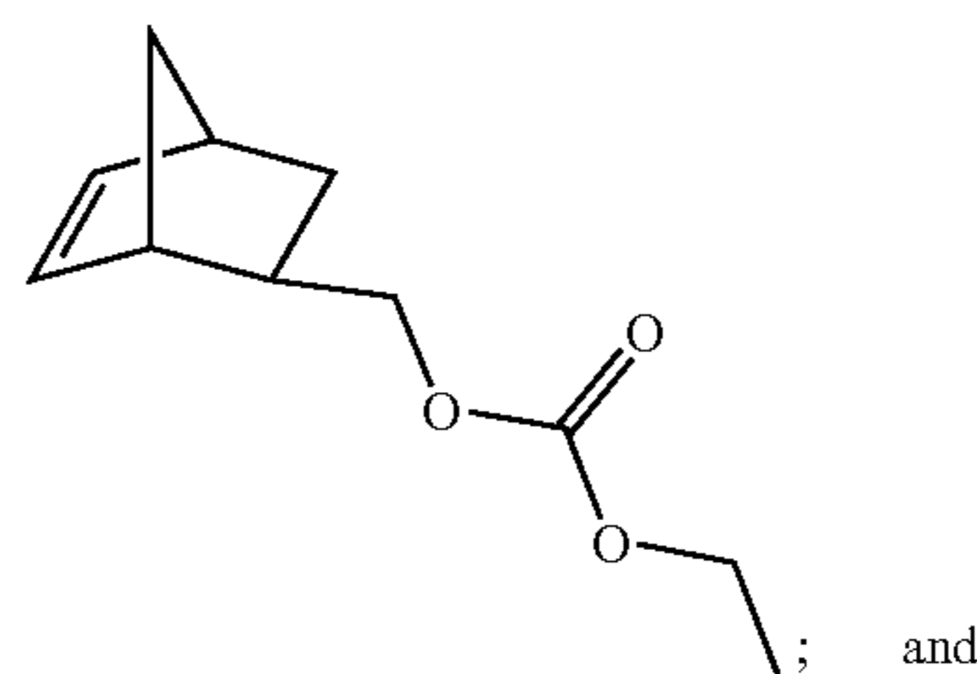
(bicyclo[2.2.1]hept-5-en-2-yl) methyl ethyl carbonate (NBEtCarb)
