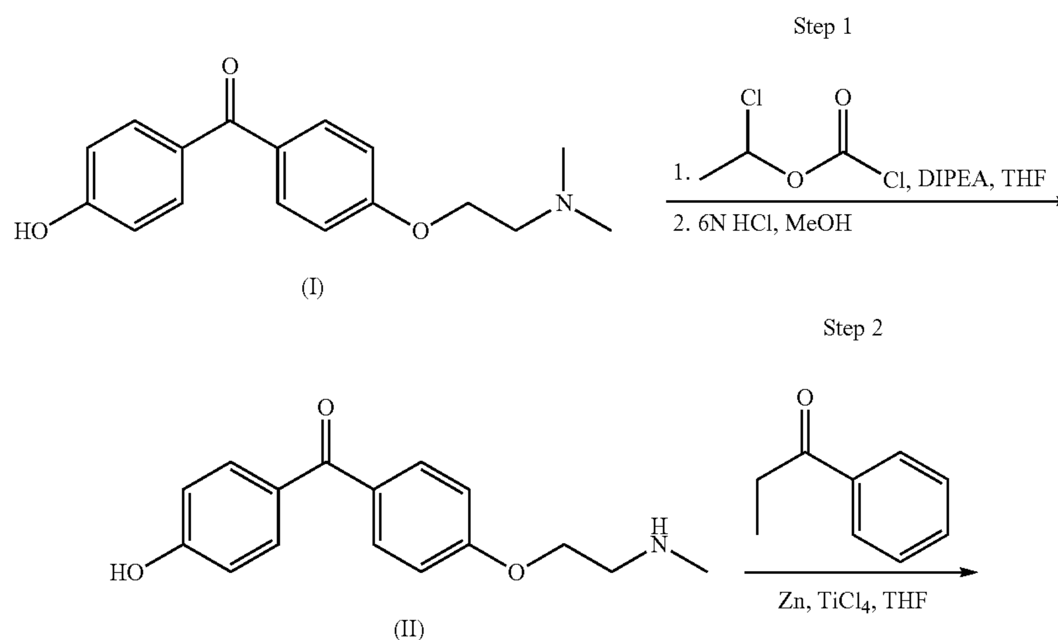
Schema 1. Synthesis of (Z)-endoxifen Free Base
