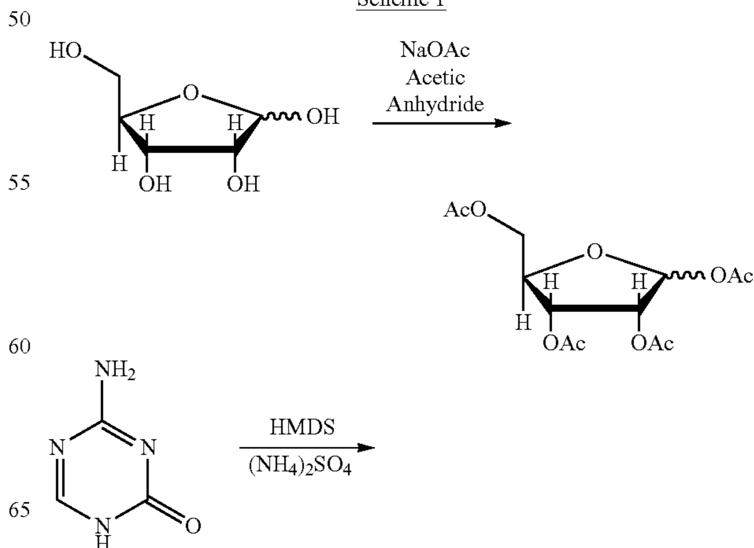
Scheme 1
