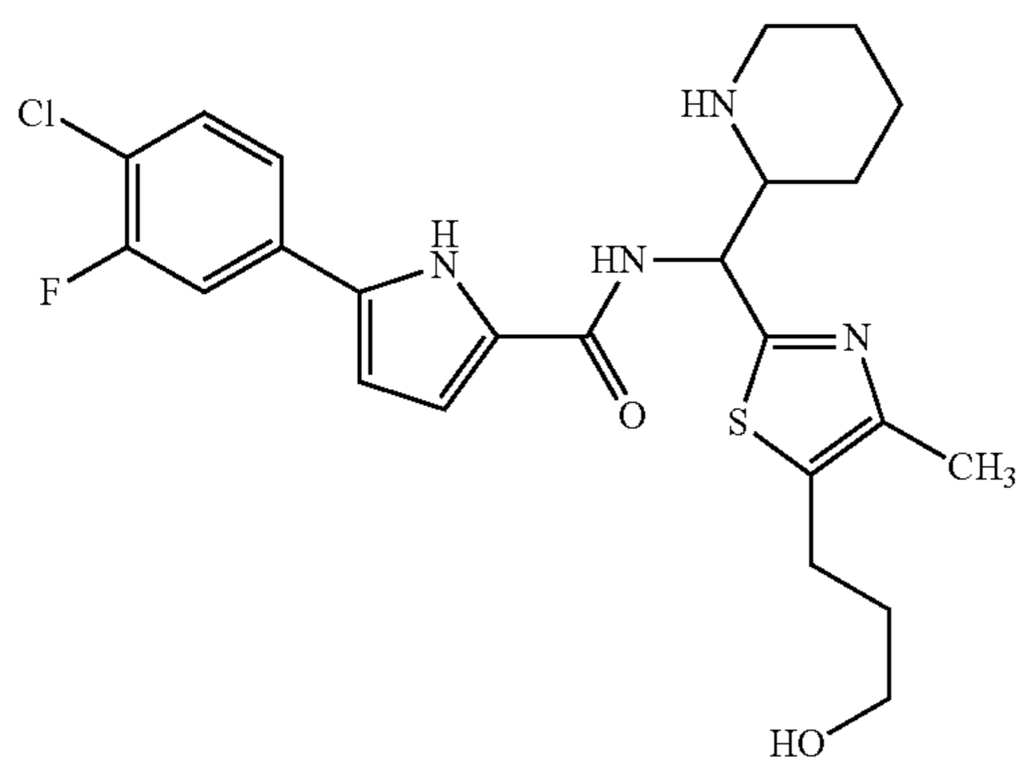
Diastereoisomer 1
