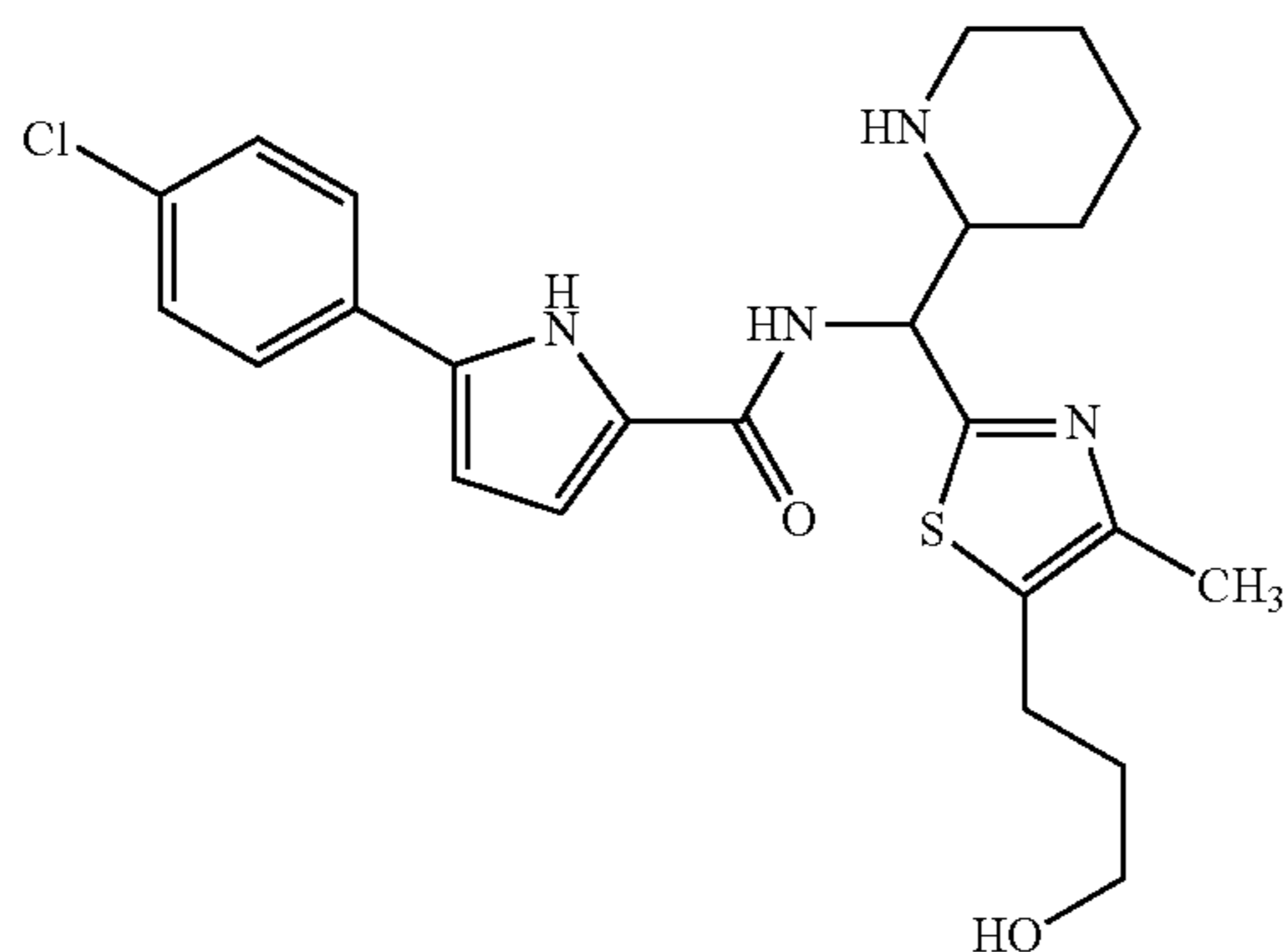
Stereoisomeric mixtures
