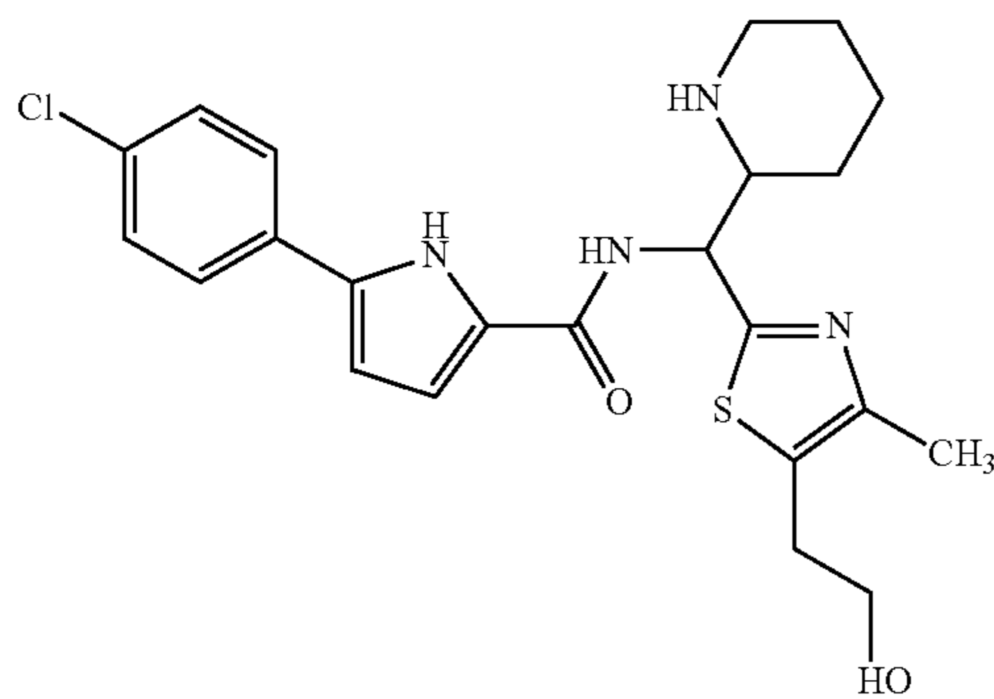
Diastereoisomer 1
