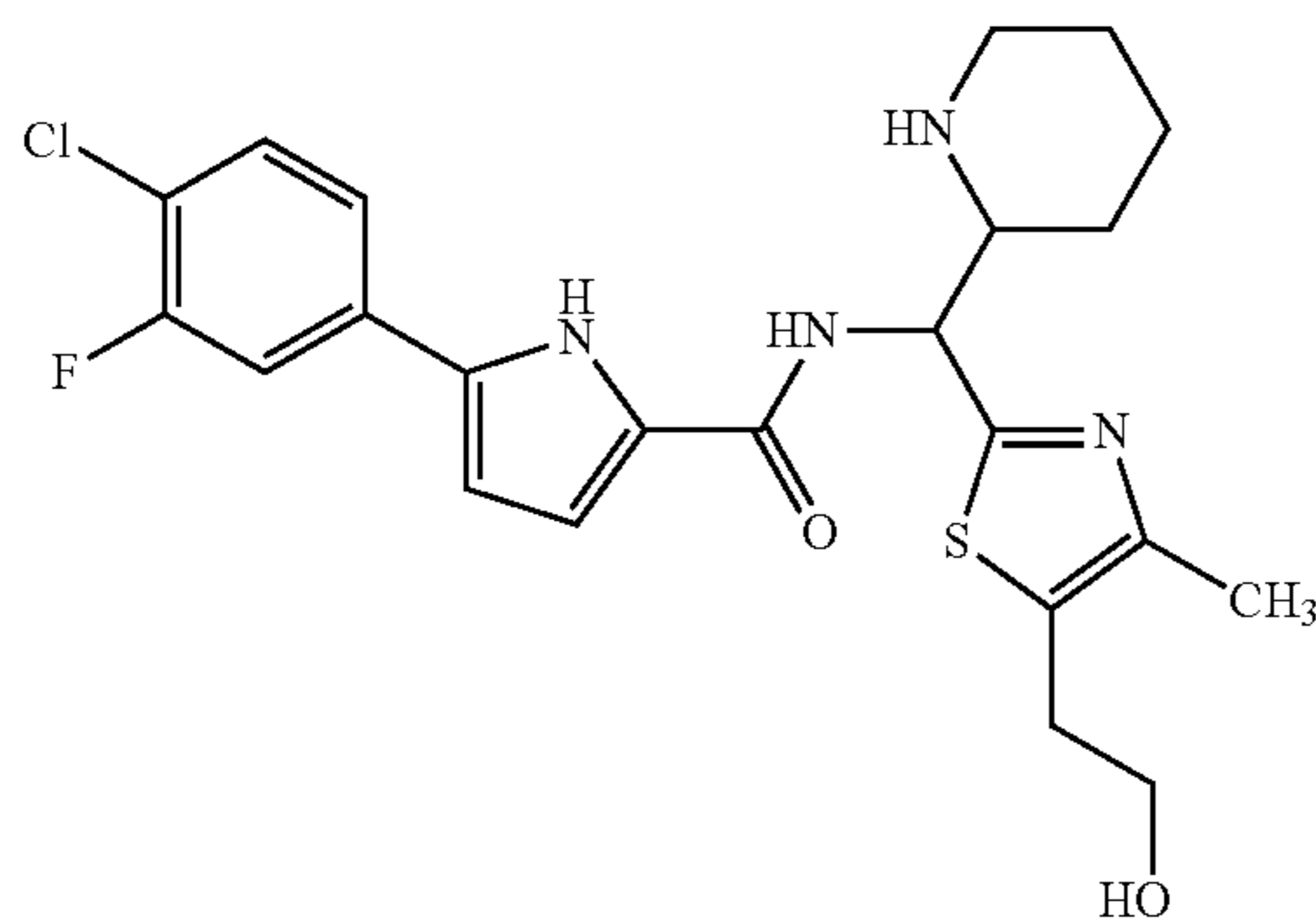
Diastereoisomer 2
