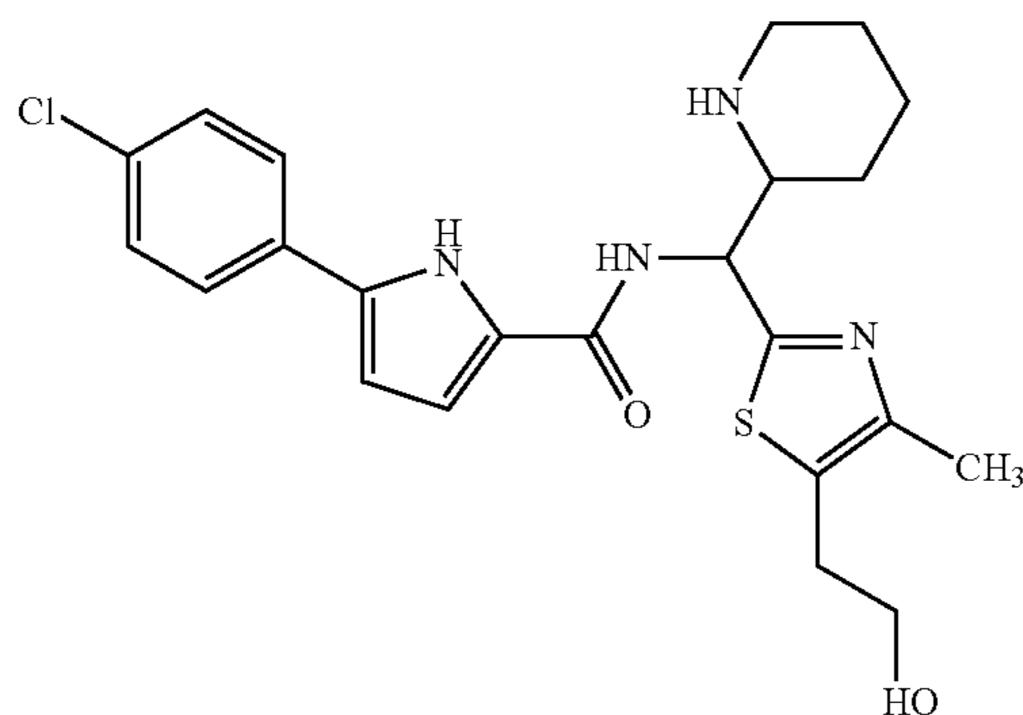
Diastereoisomer 2
