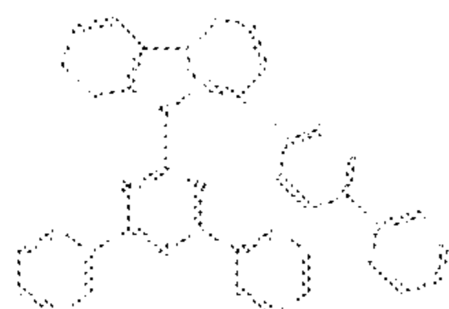
Compound 4
