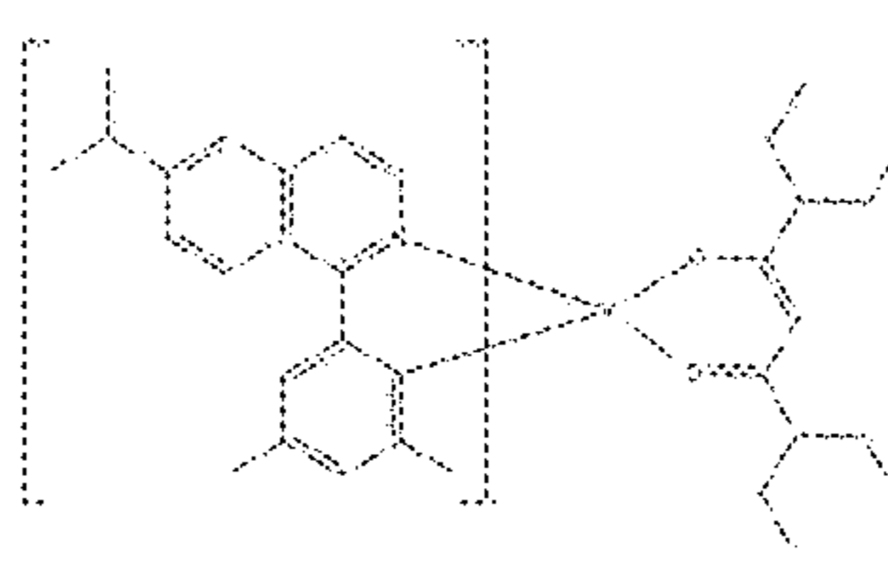
Compound 11
