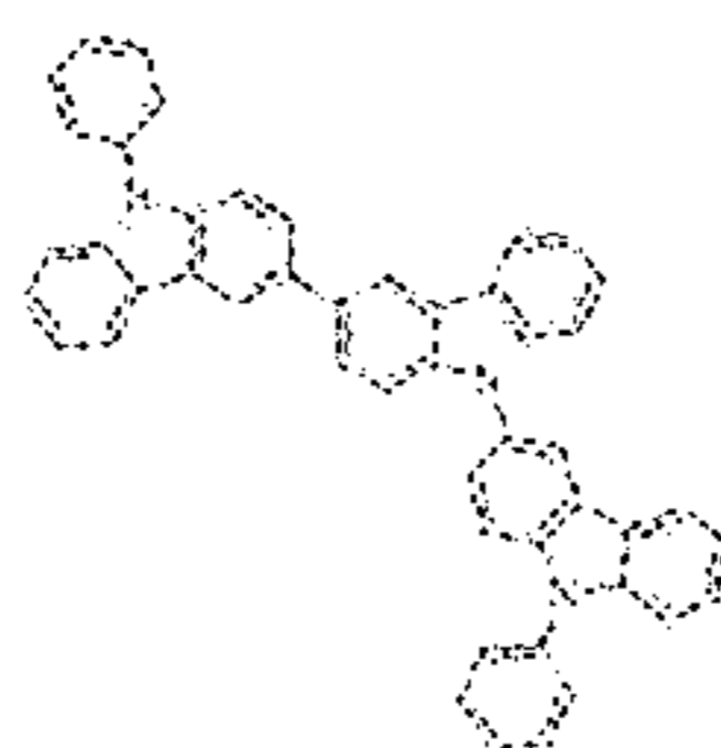
Compound 3
