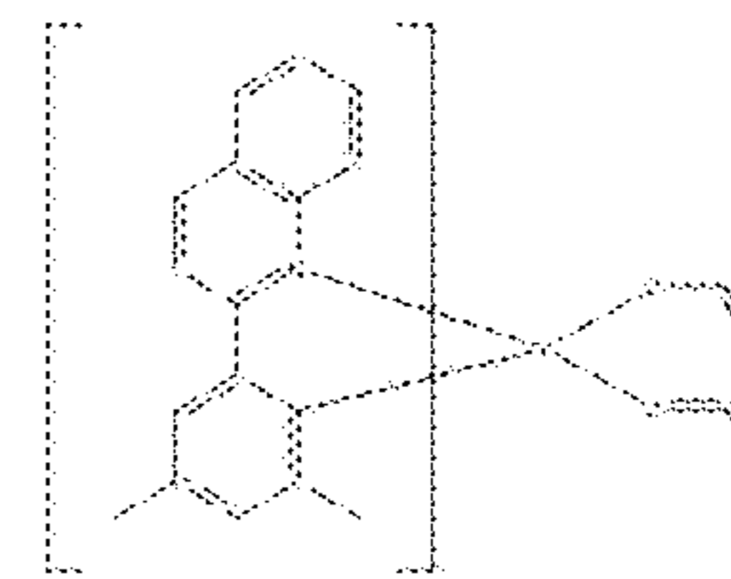
Compound 12
