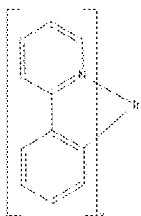
Compound 13
