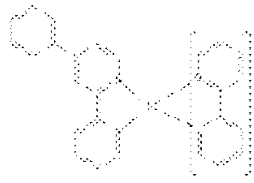
Compound 5
