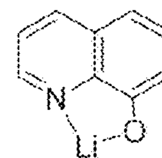
Compound 7
