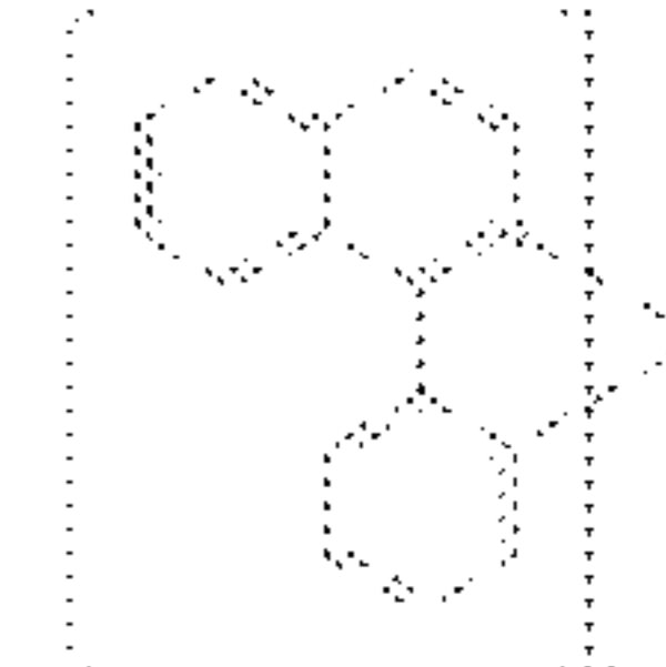
Compound 9
