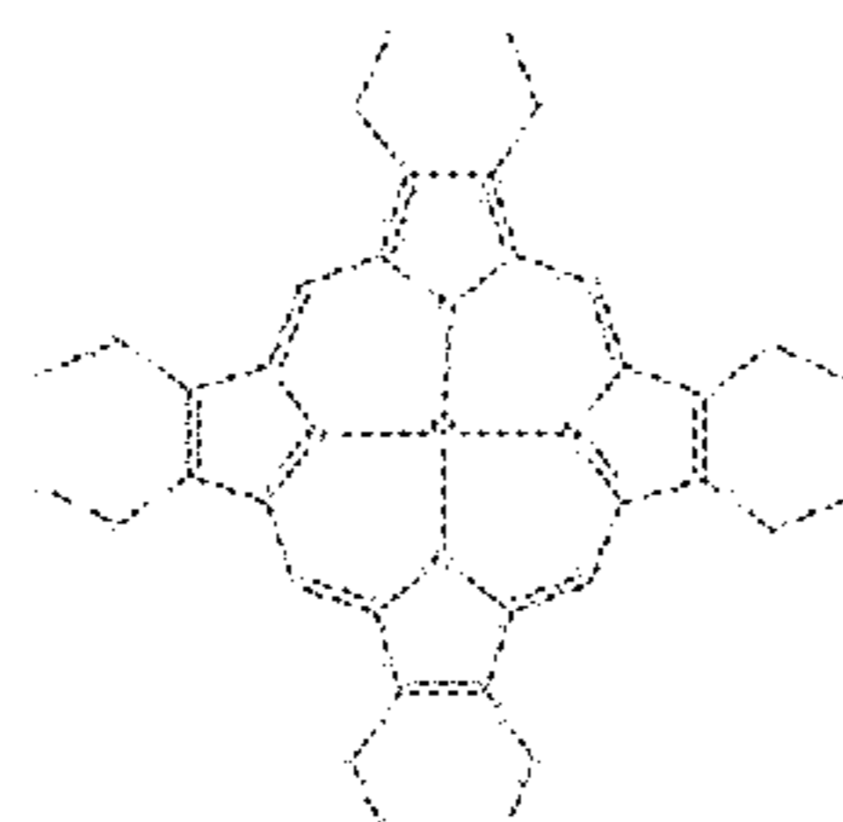
Compound 14
