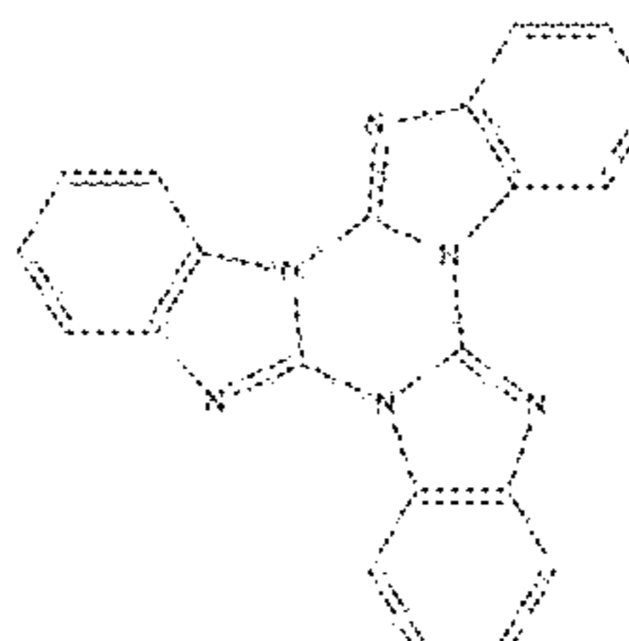
Compound 15
