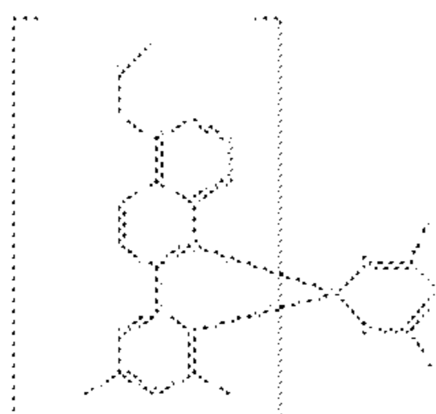
Compound 10
