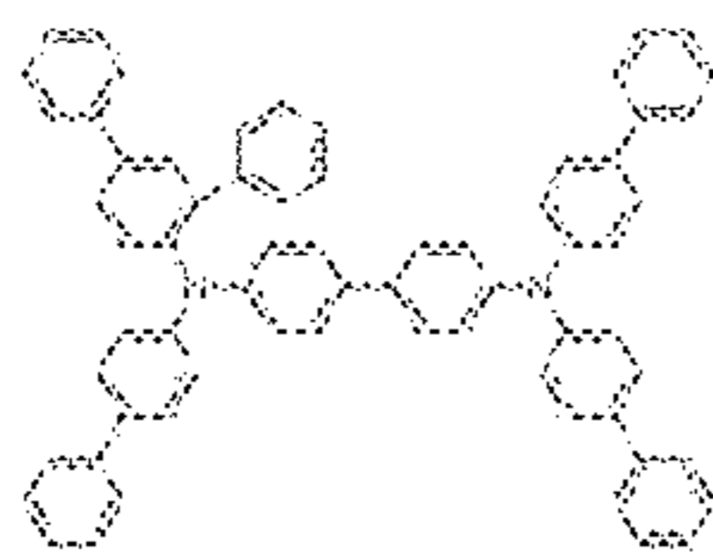
Compound 2
