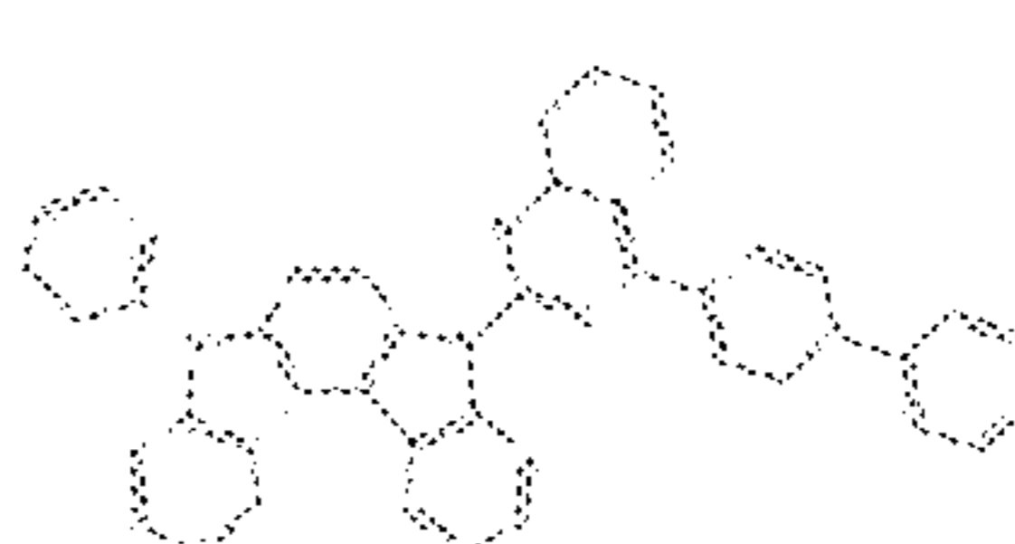
Compound 8
