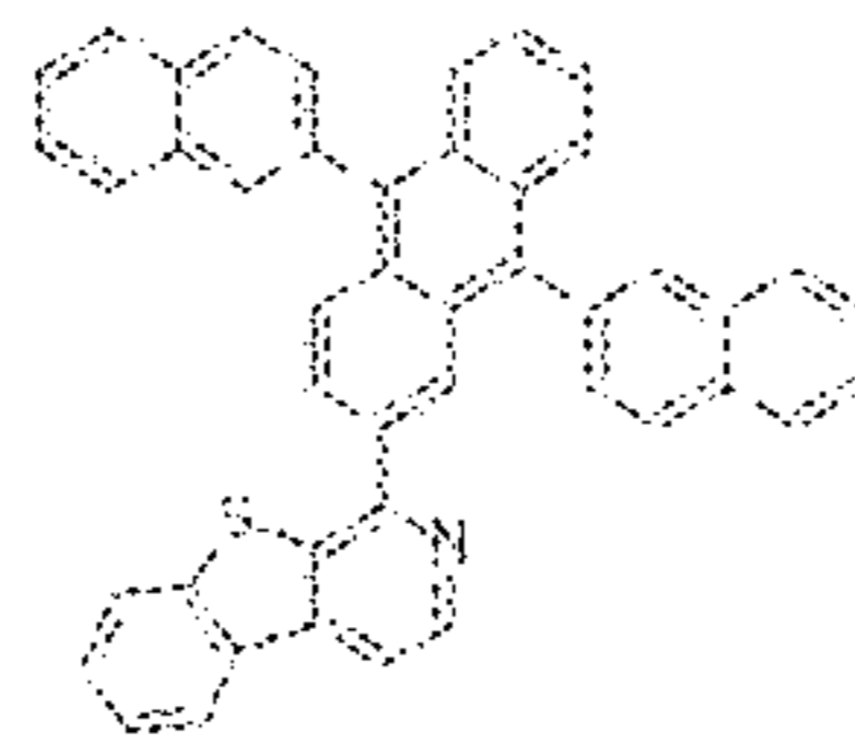
Compound 6
