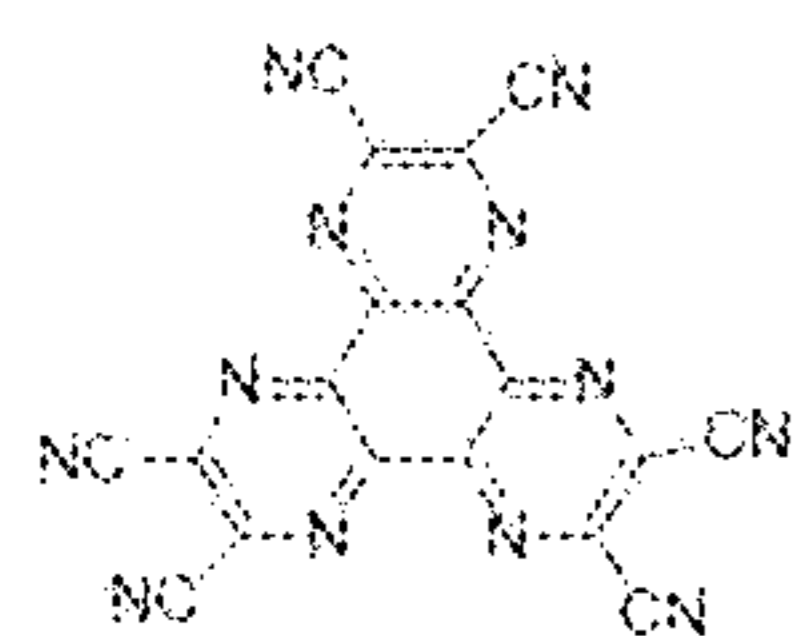
Compound 1
