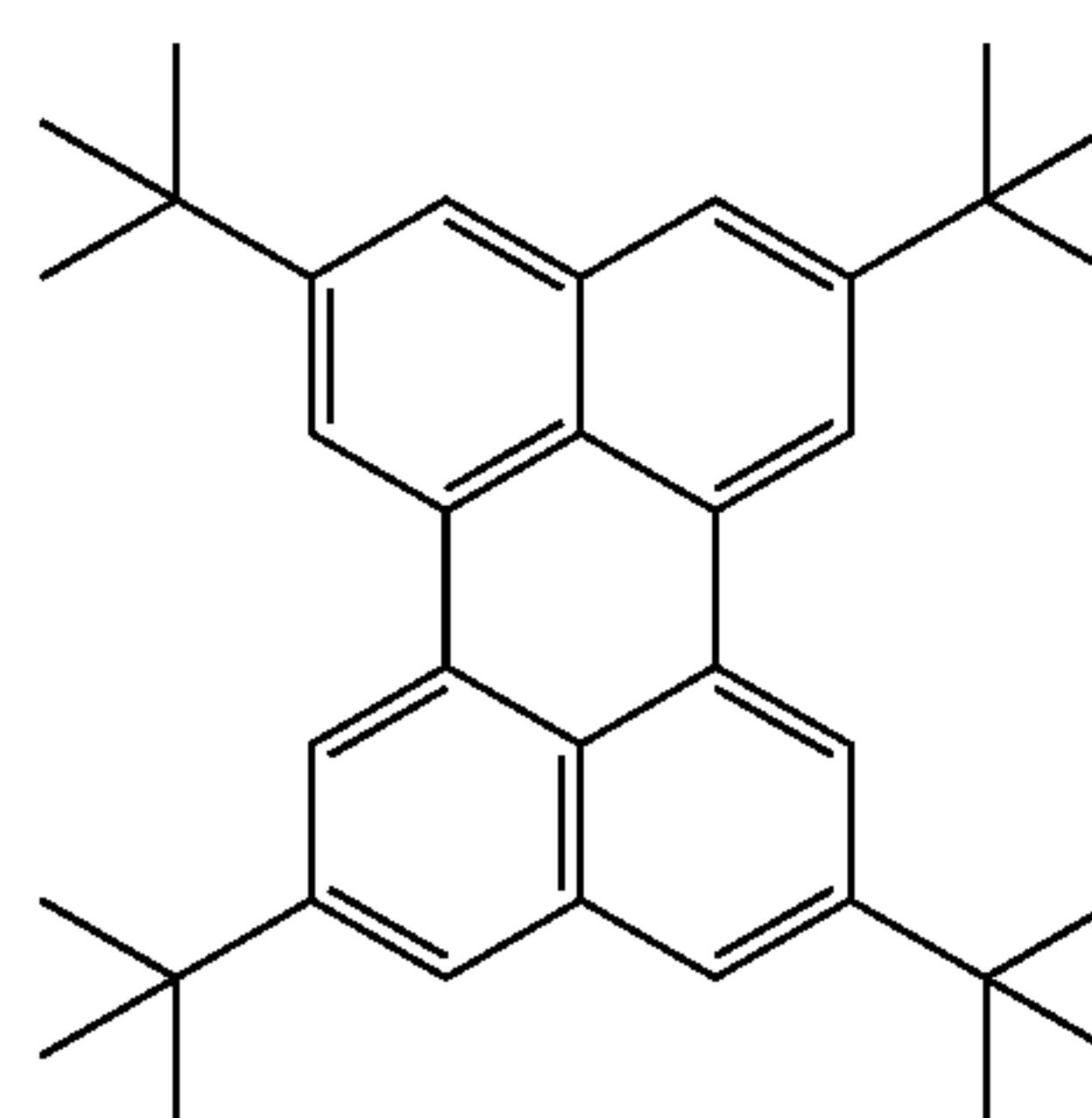
TBPc
