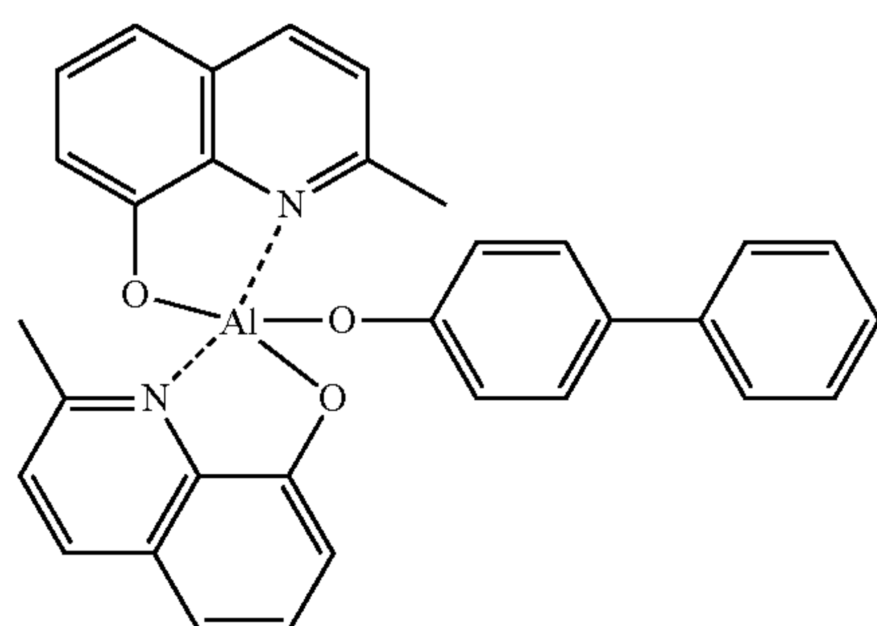
BAq
