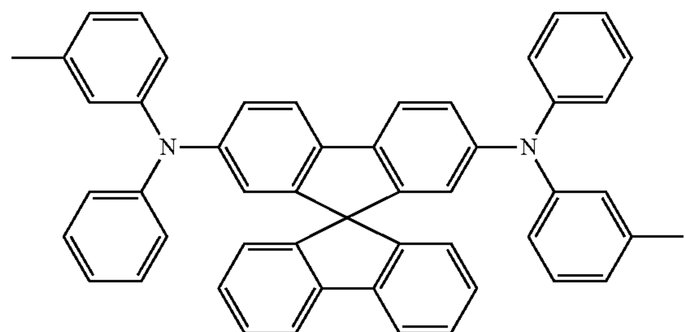
Spiro-TPD
