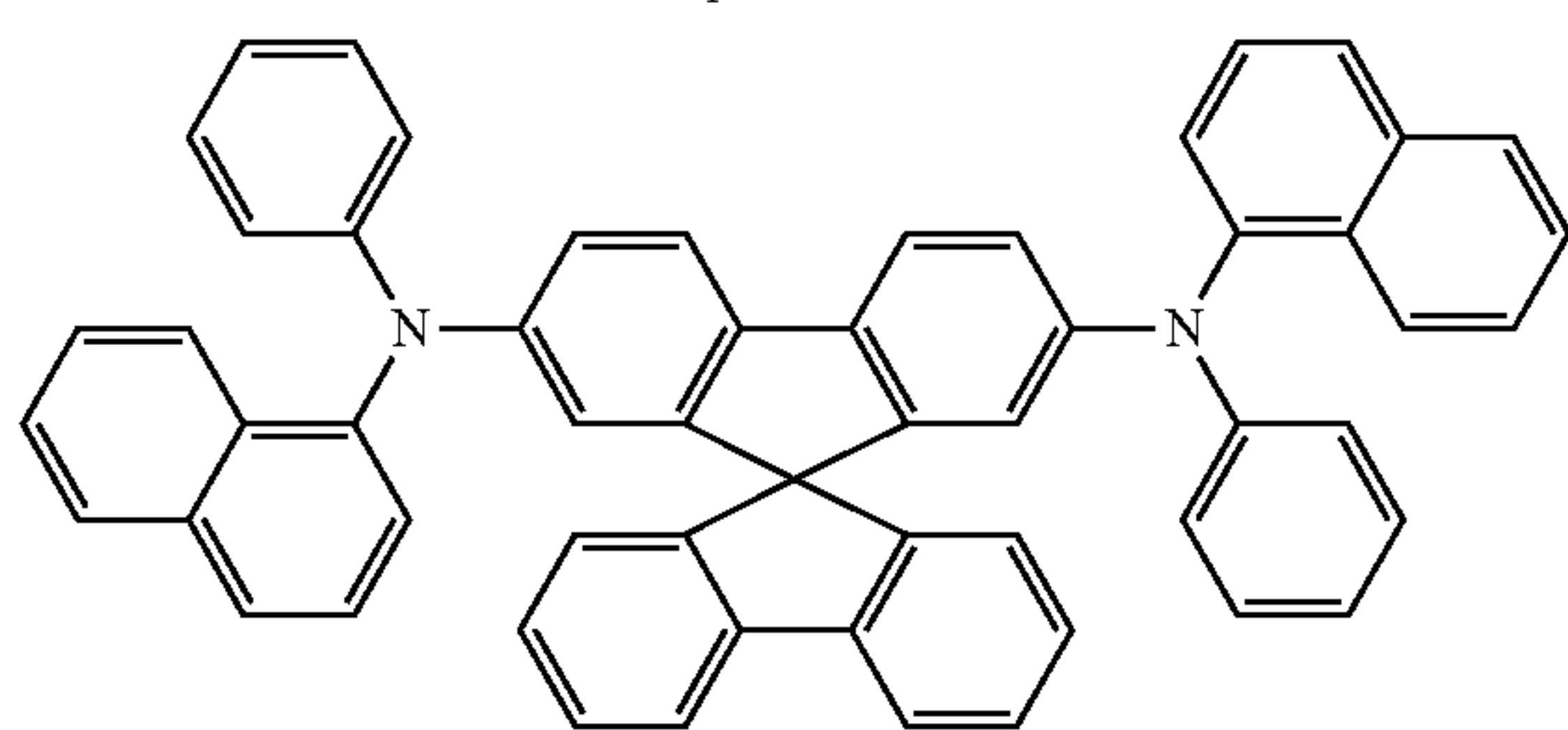
Spiro-NPB
