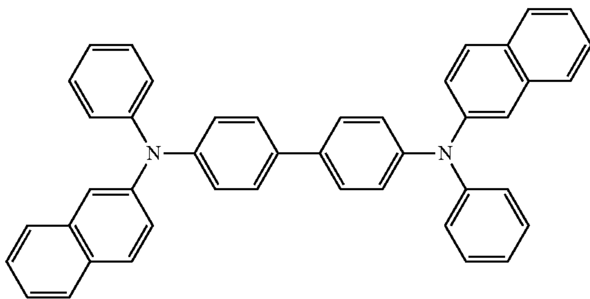
\beta -NPB
