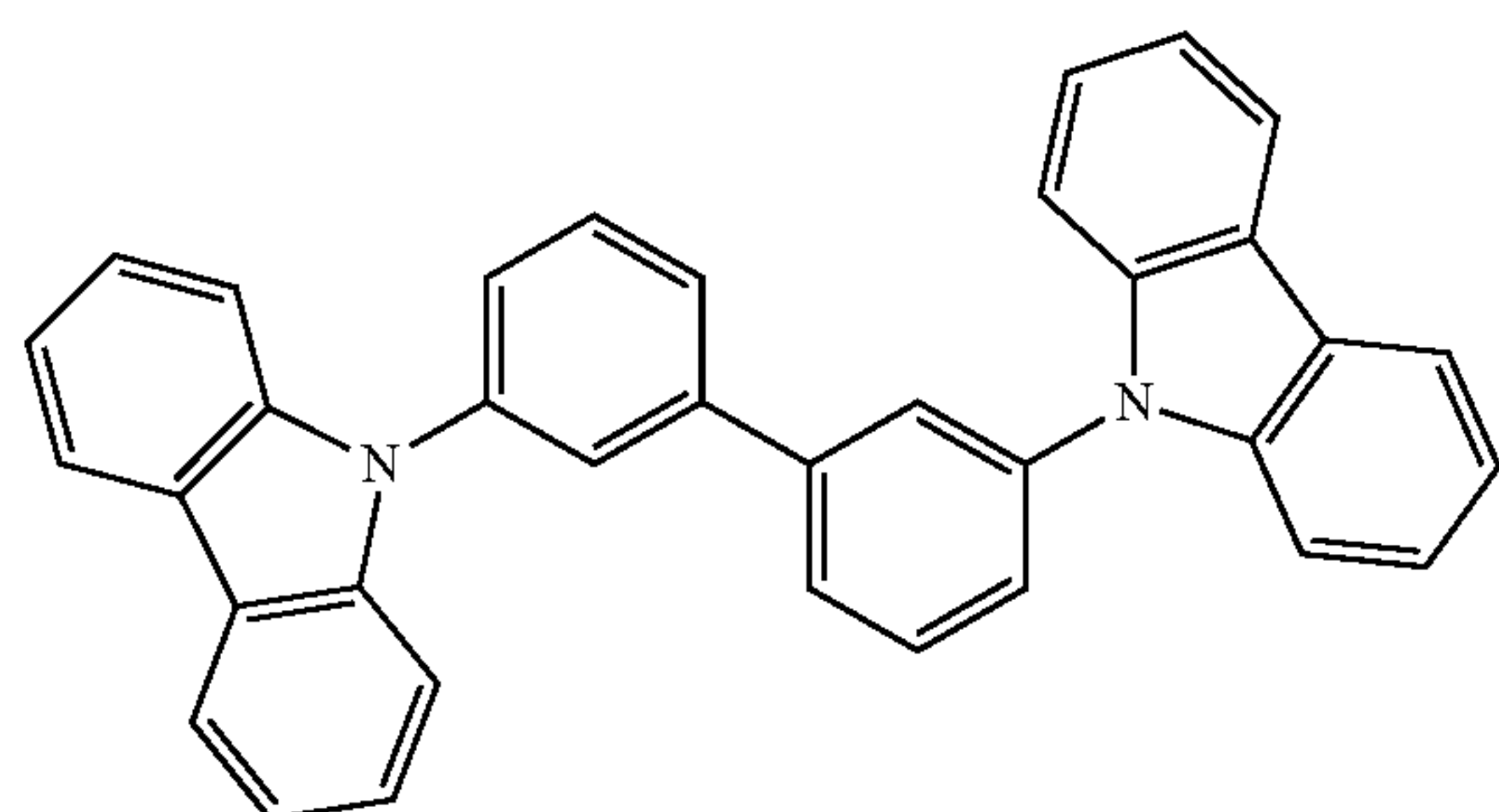
mCBP
