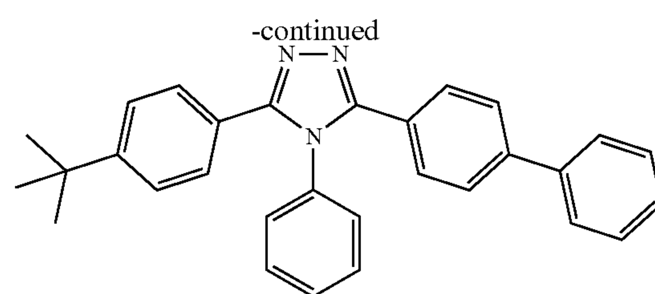
TAZ
