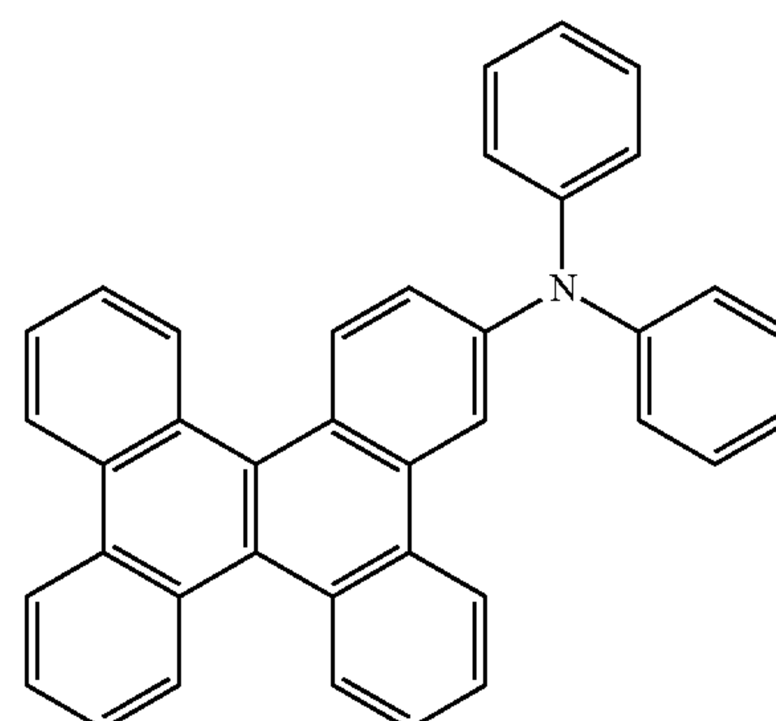
3-DPADBC
