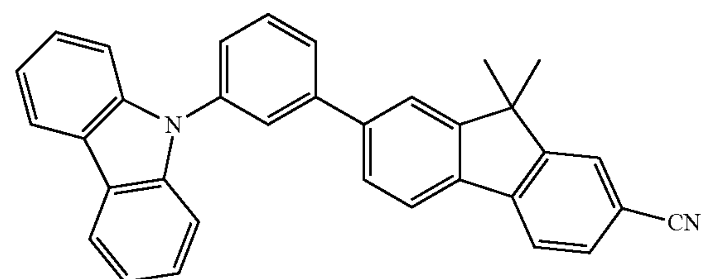
m-CF-PhCz
