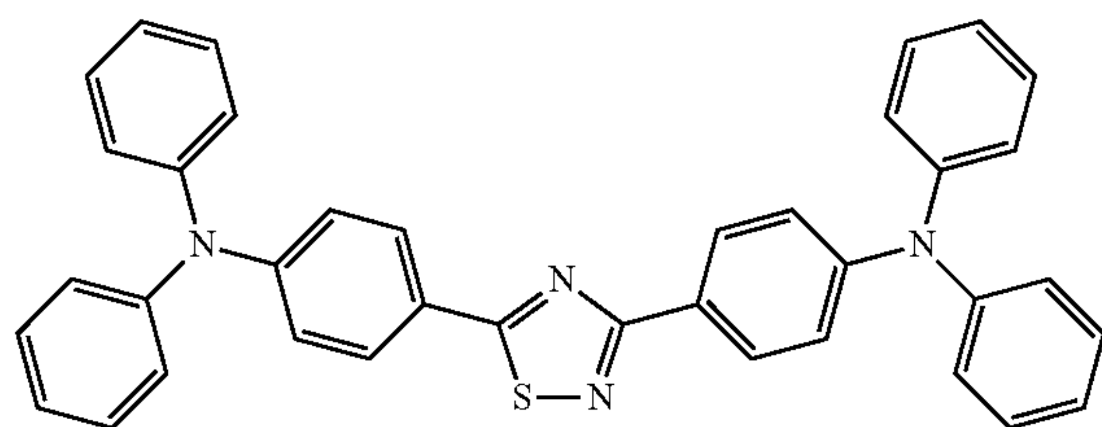
p-TPATHZ
