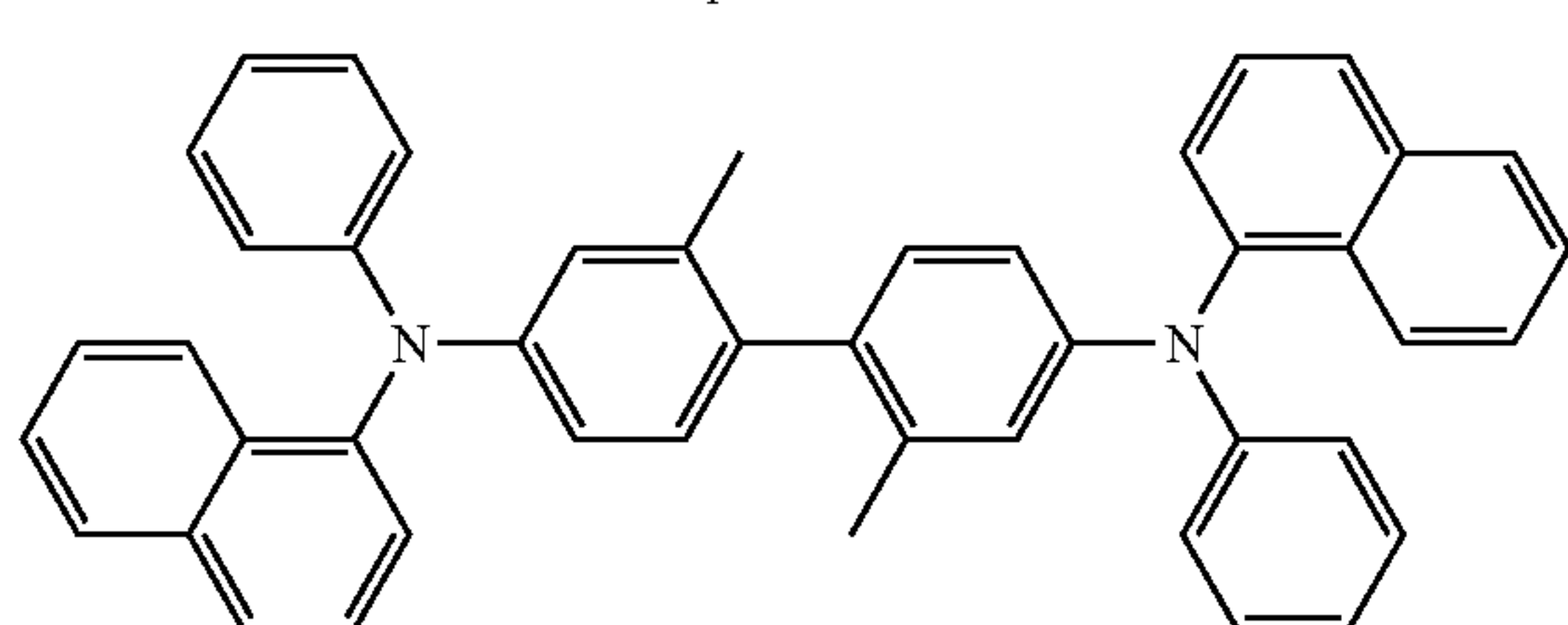
methylated NPB
