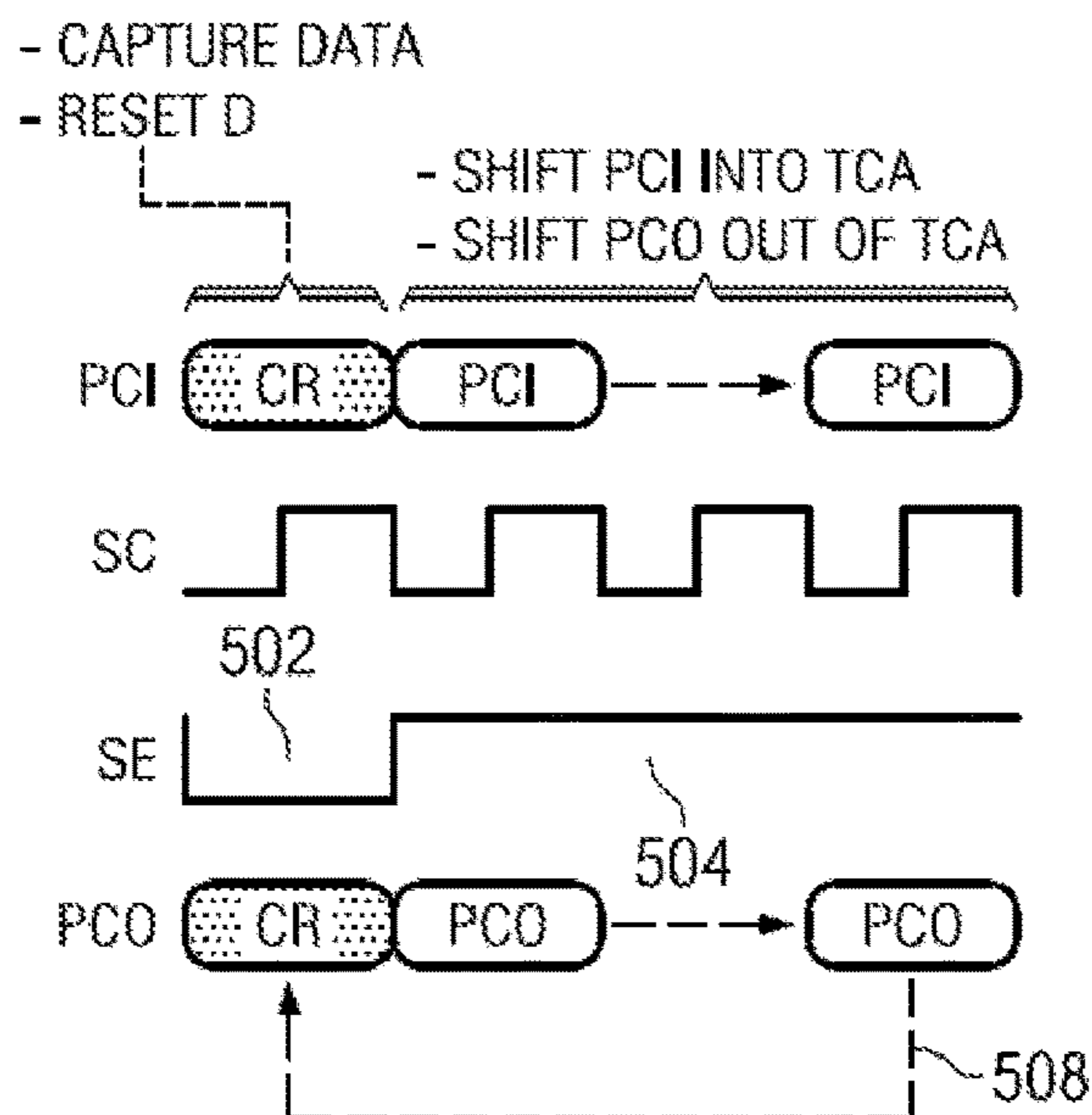
FIG. 5 (PRIOR ART)
