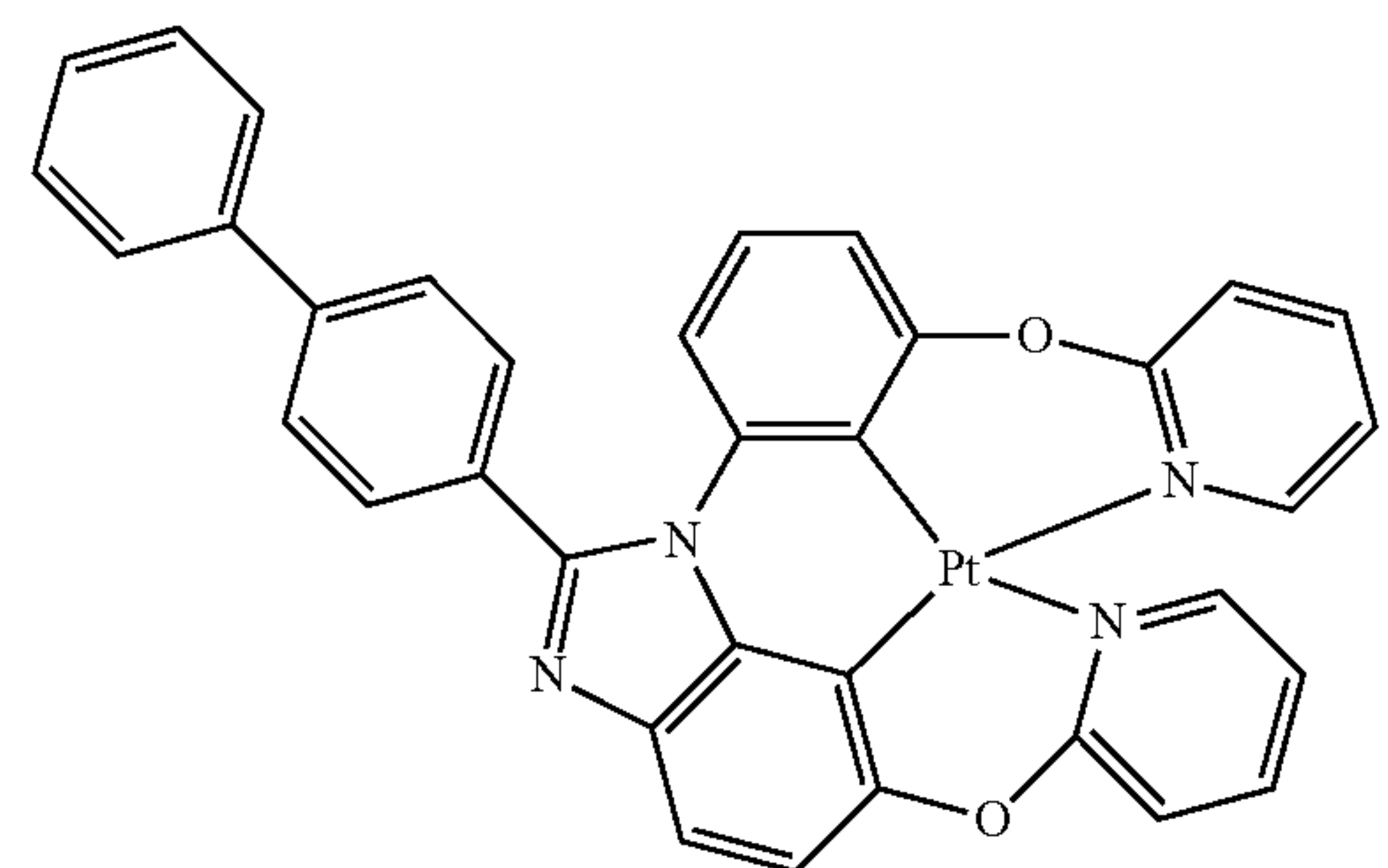
Compound 12
