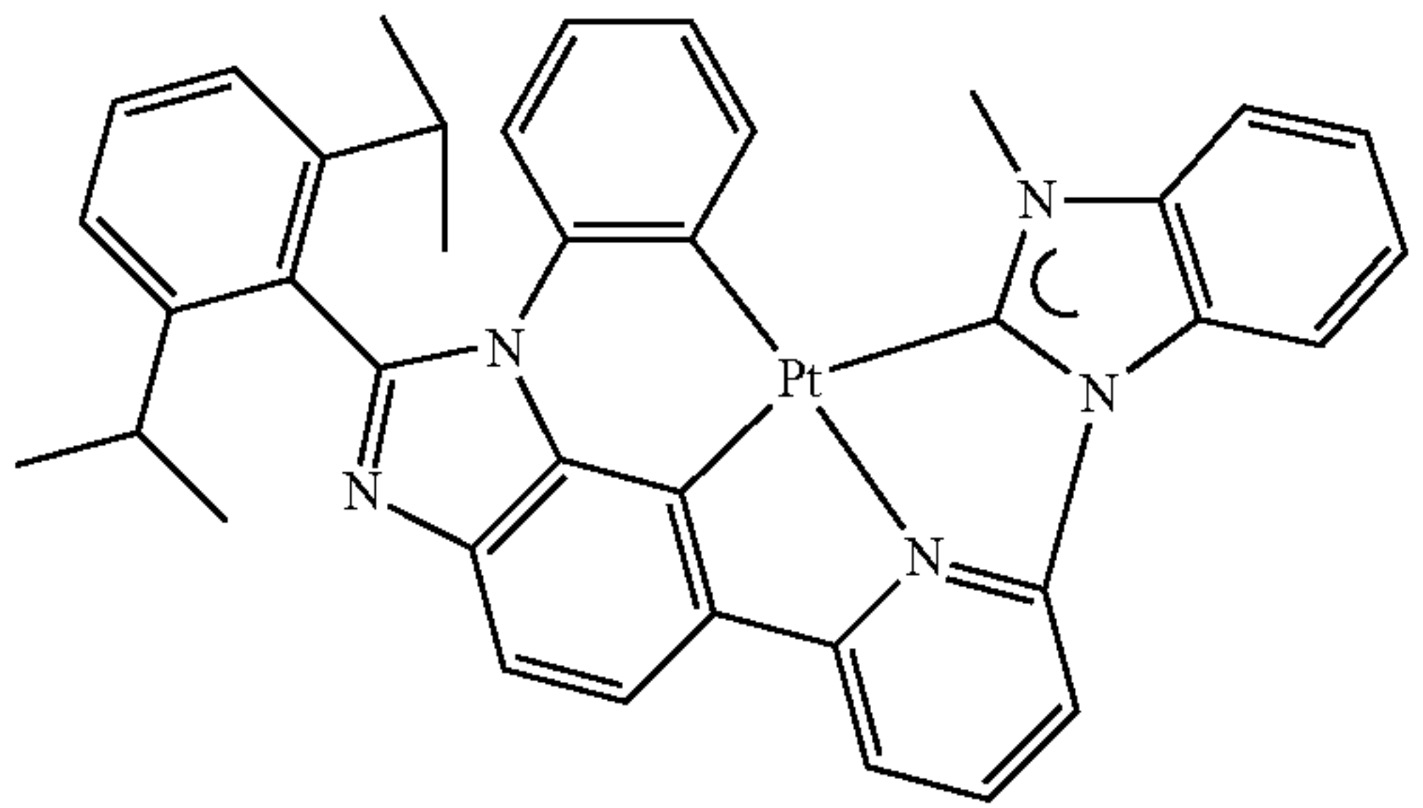
Compound 25
