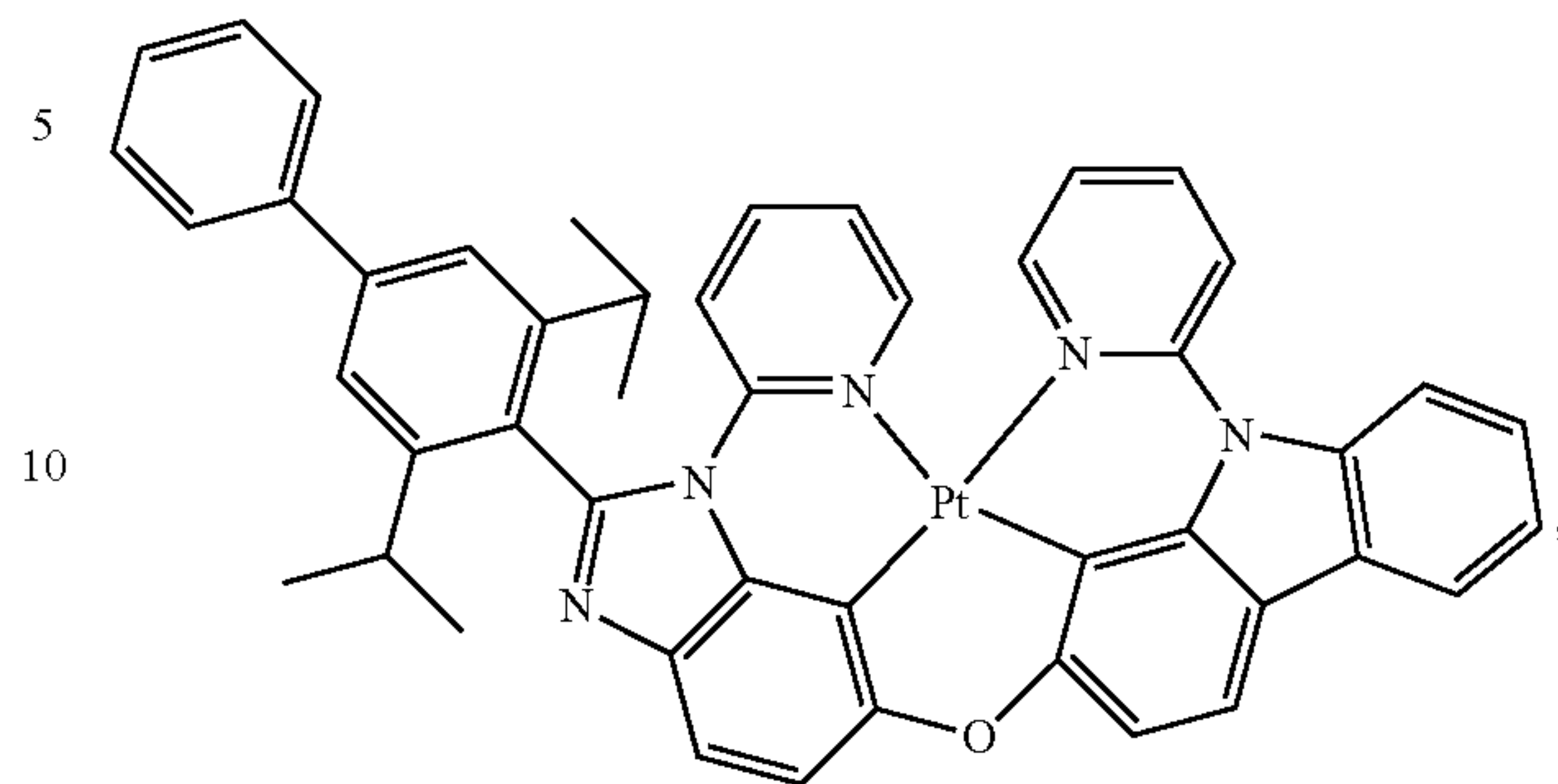
Compound 69
