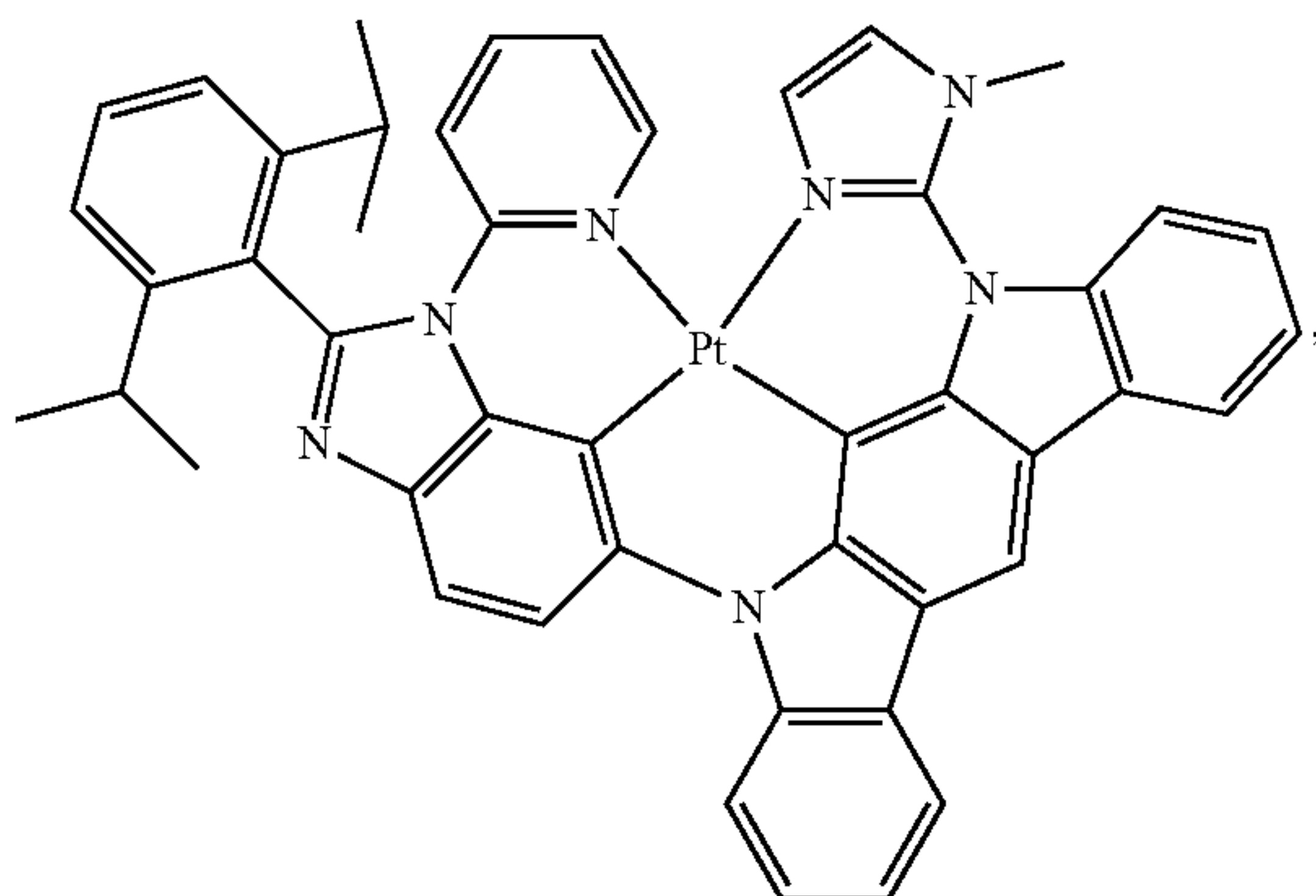
Compound 94
