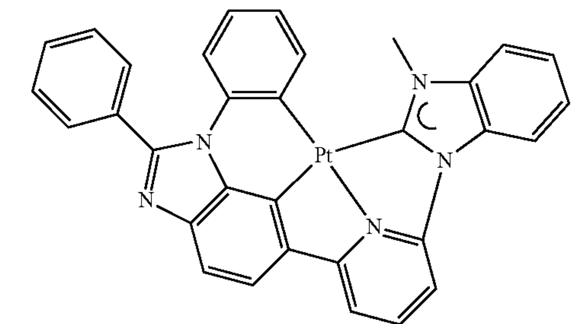
Compound 22
