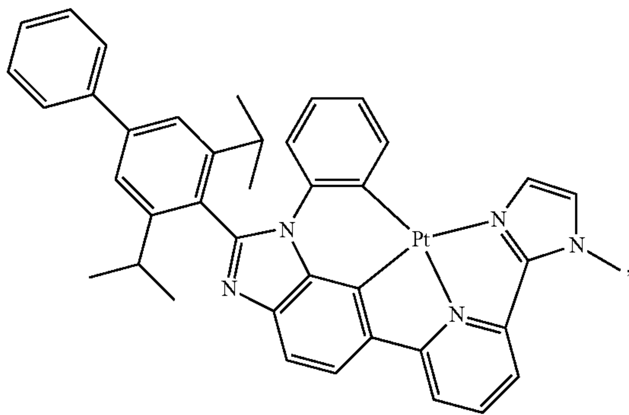
Compound 44
