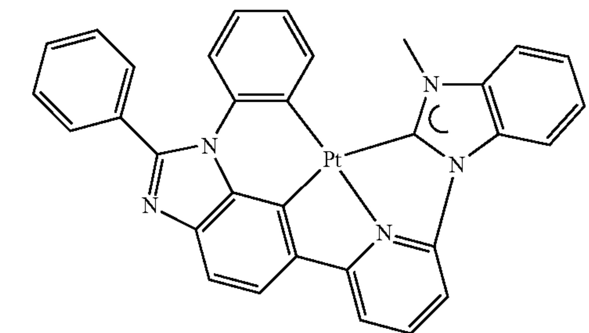
Compound 22
