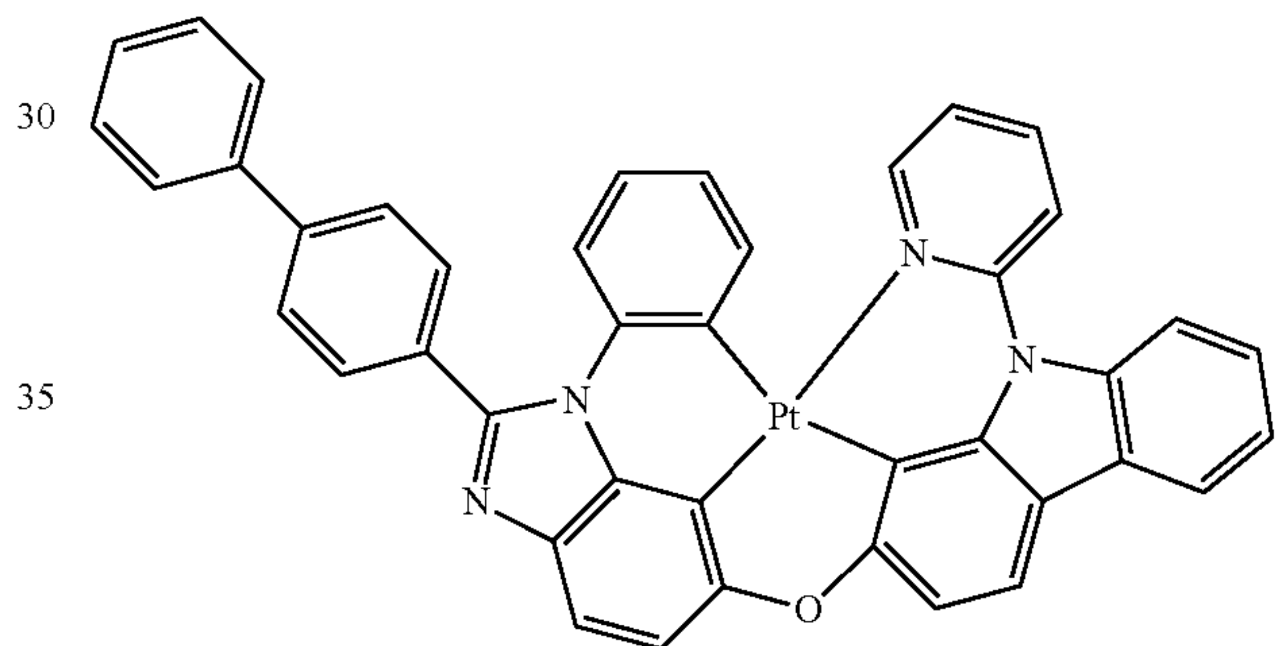
Compound 71
