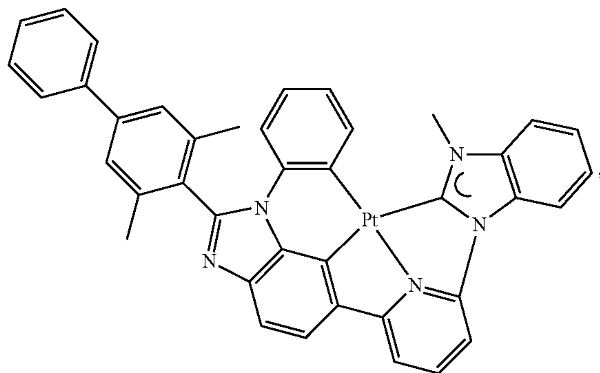
Compound 26
