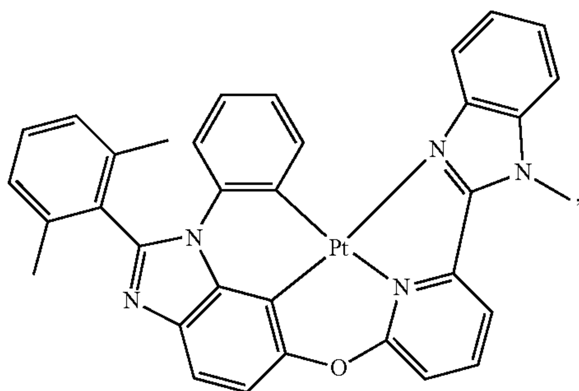
Compound 46
