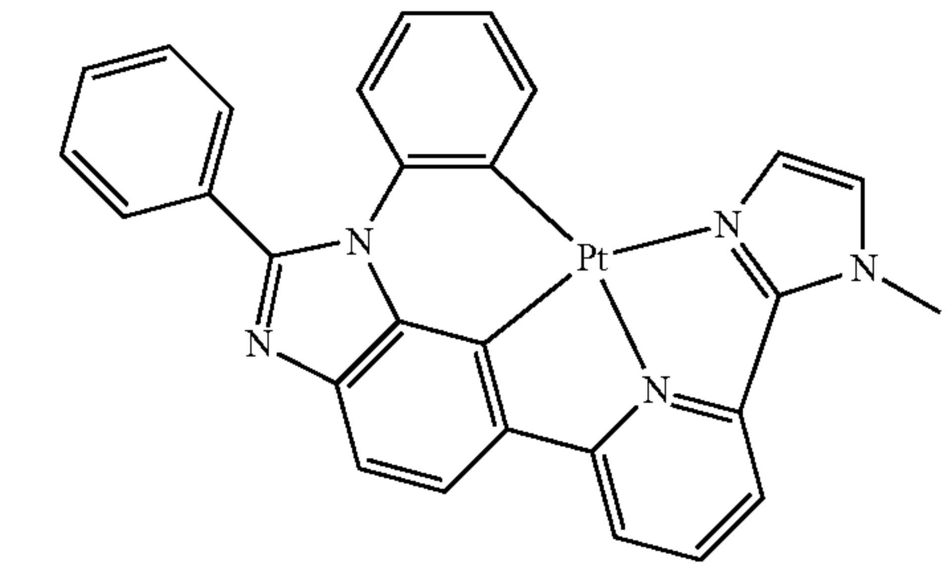
Compound 41
