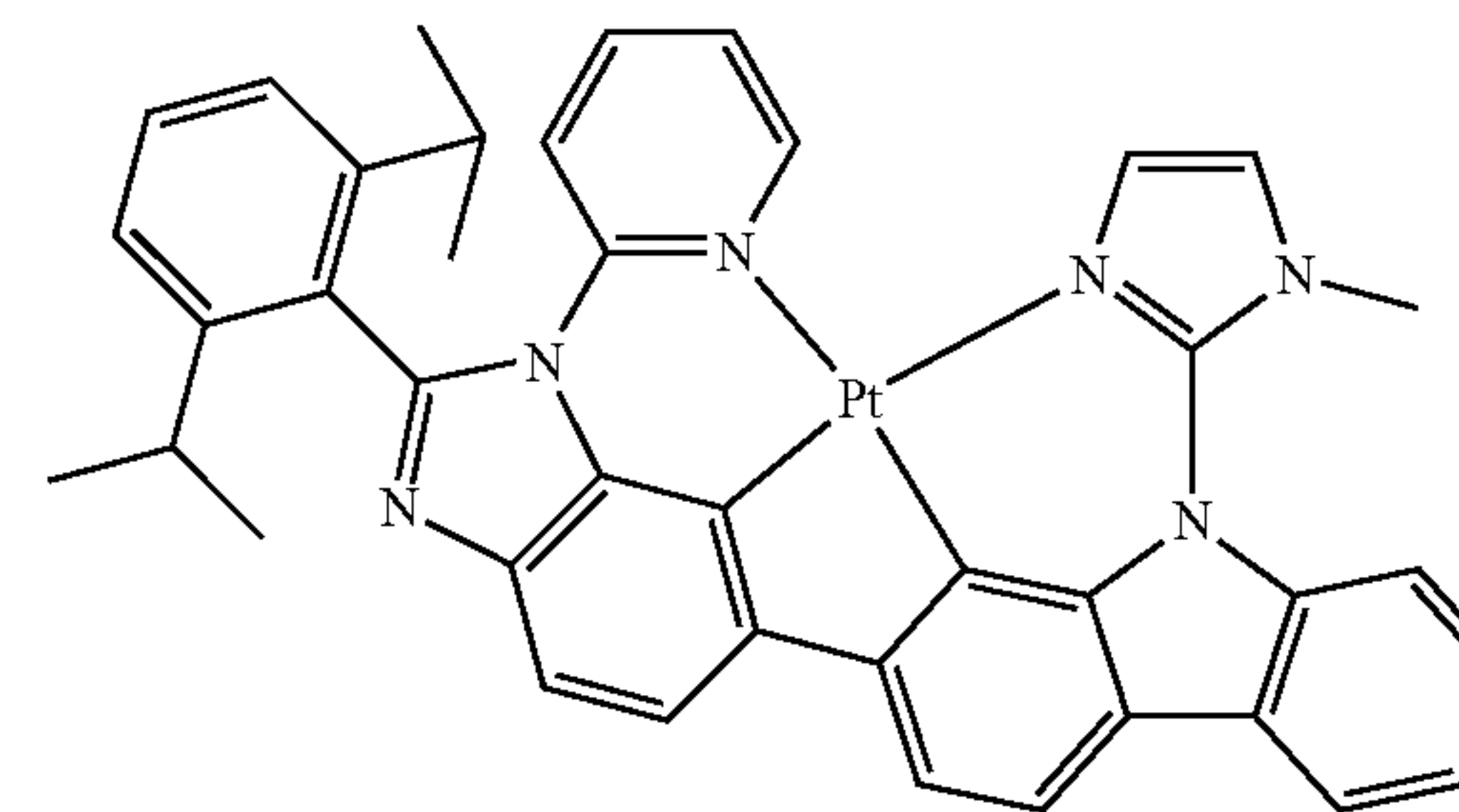
Compound 80
