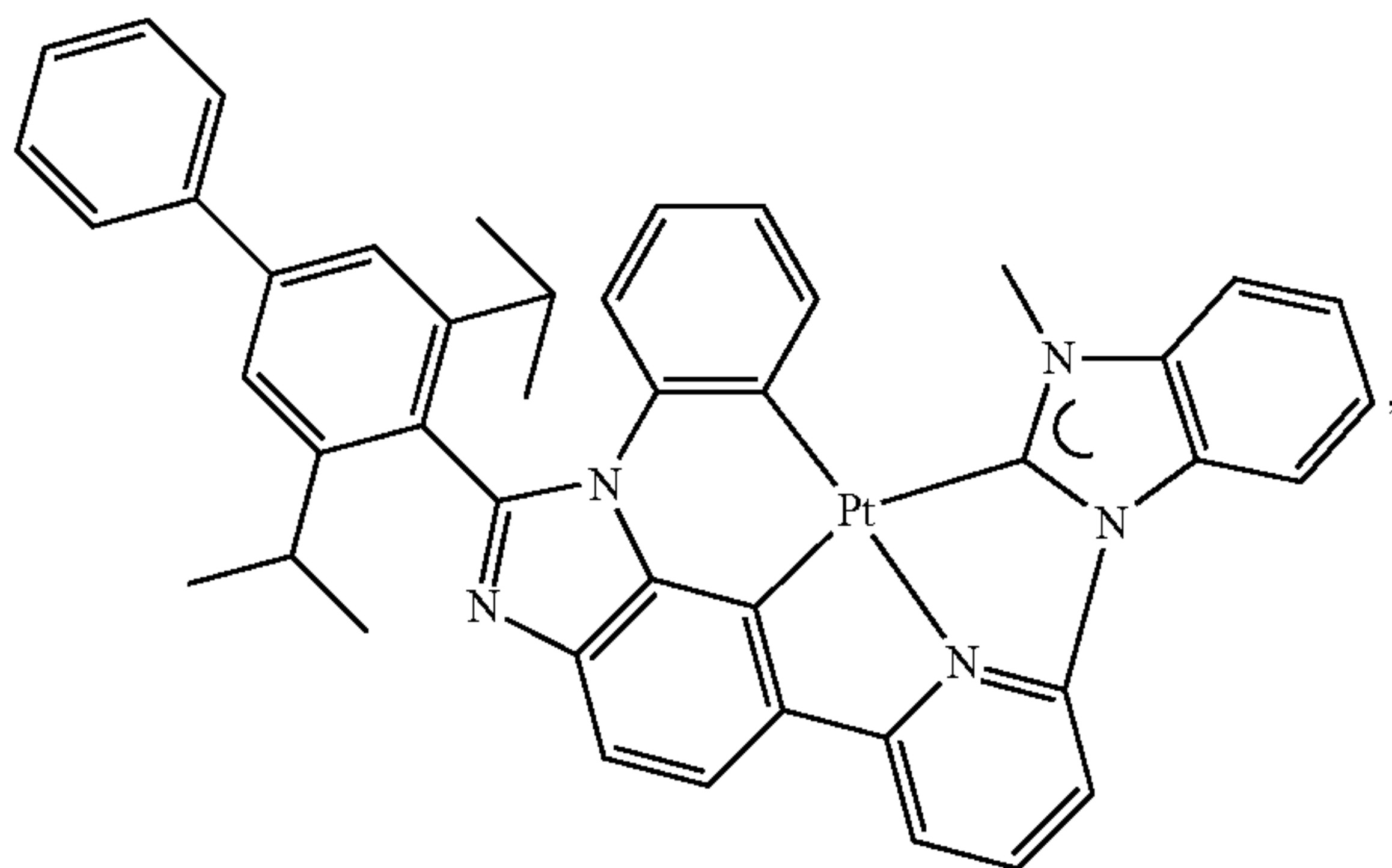
Compound 27
