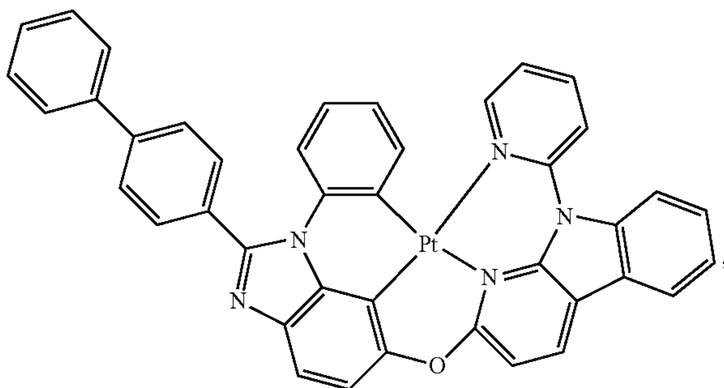
Compound 86
