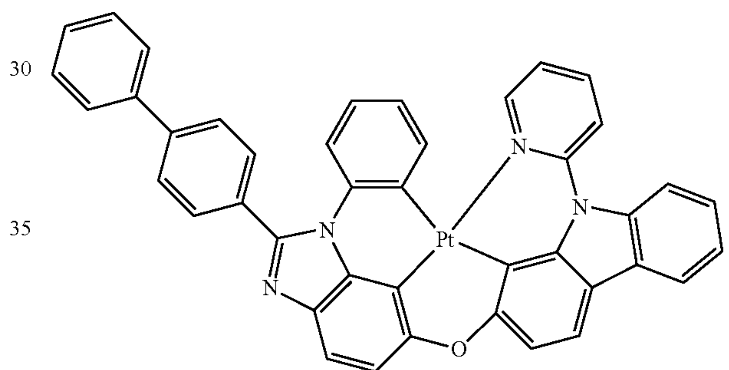
Compound 71
