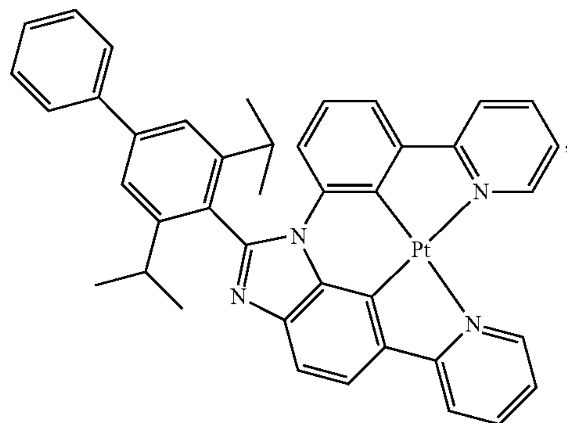
Compound 7
