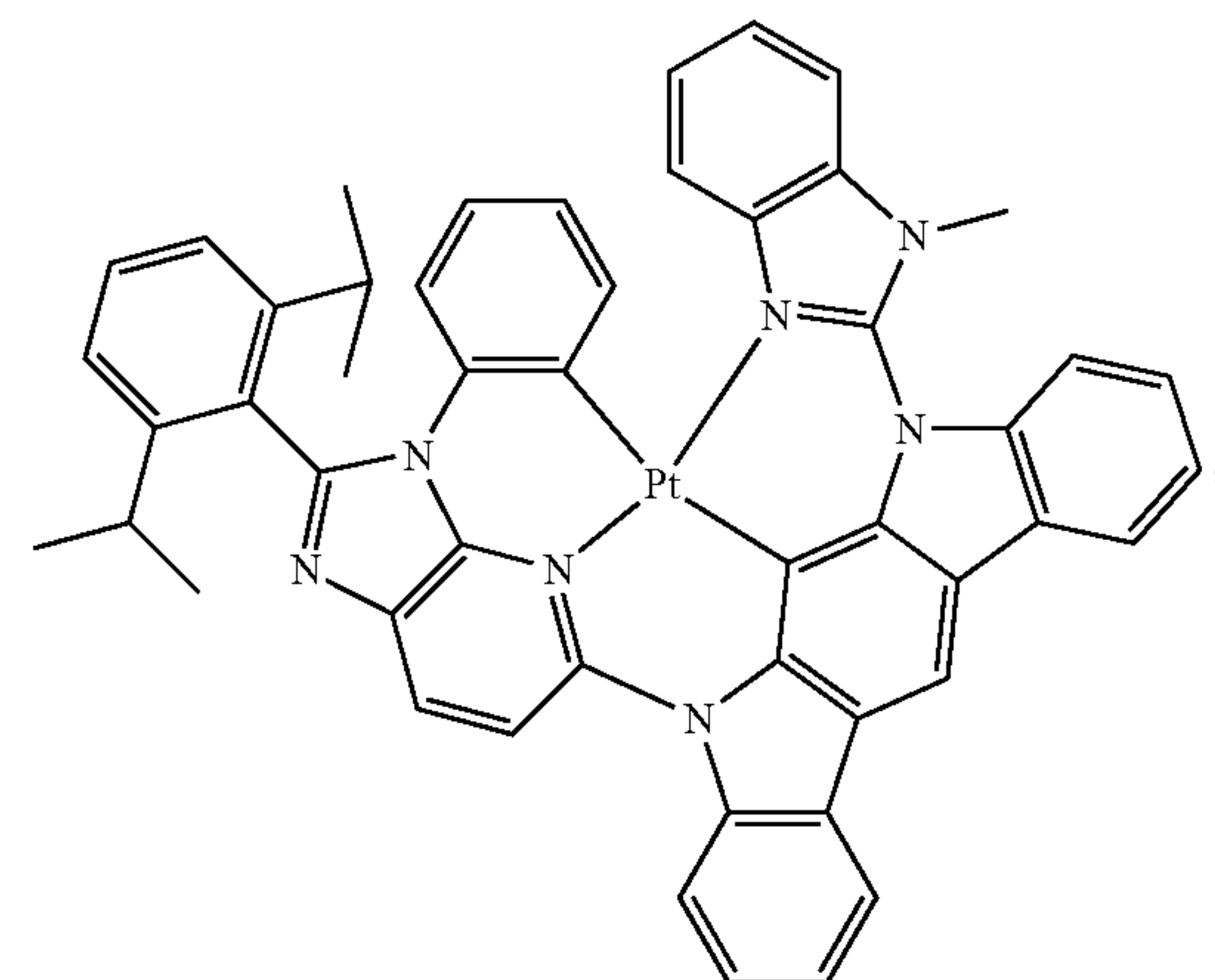
Compound 97
