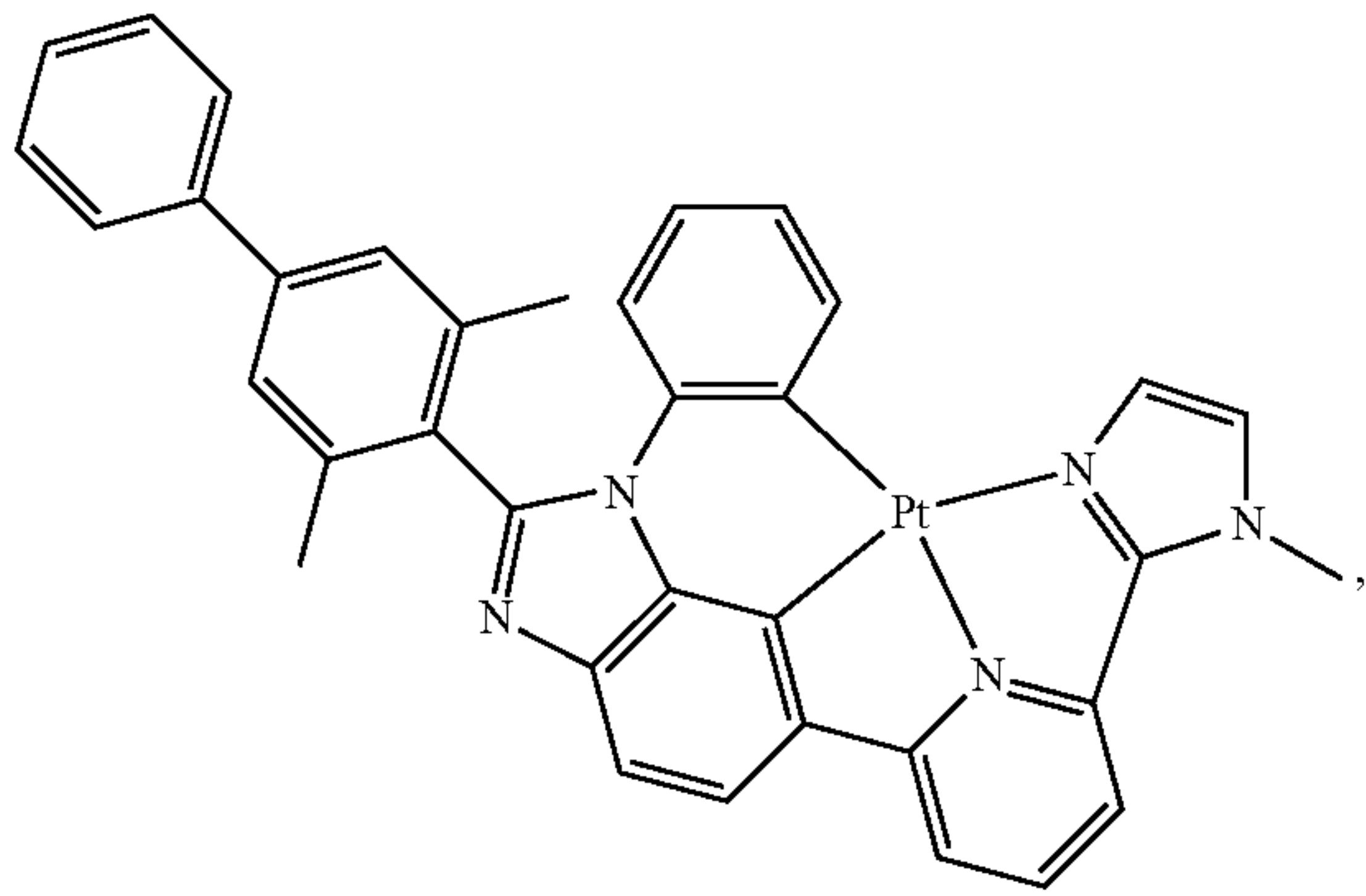
Compound 44
