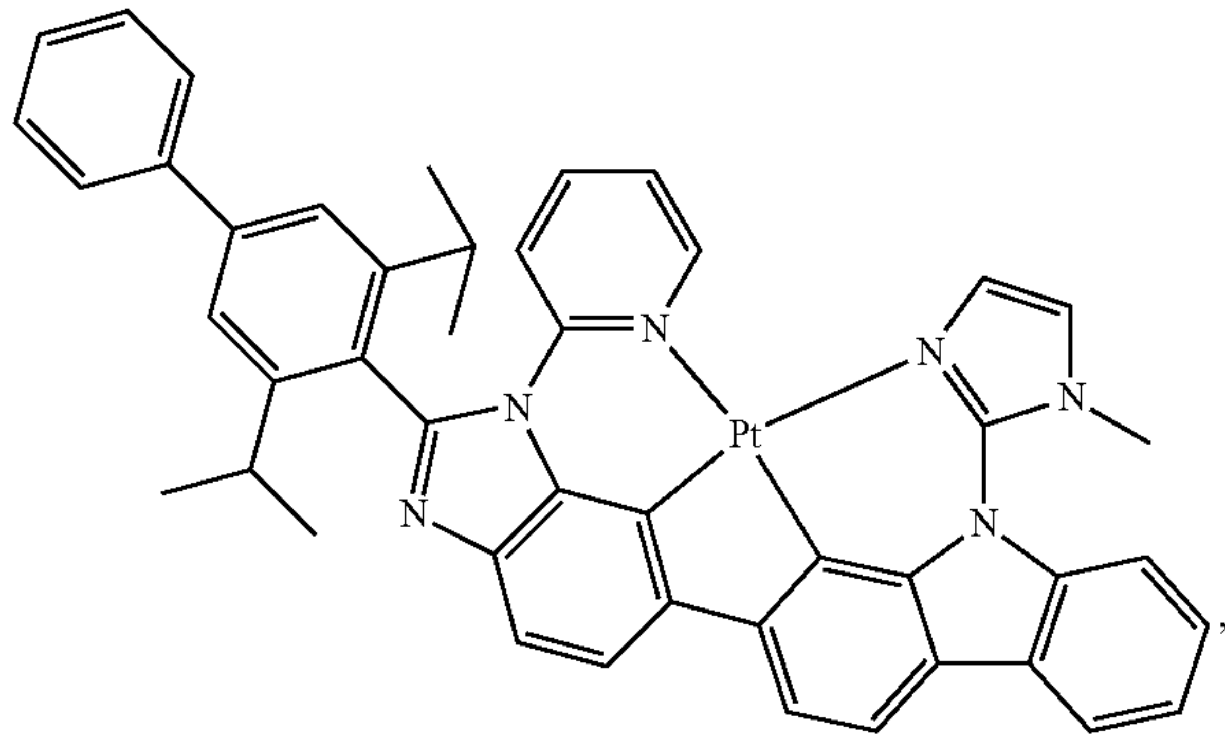
Compound 83
