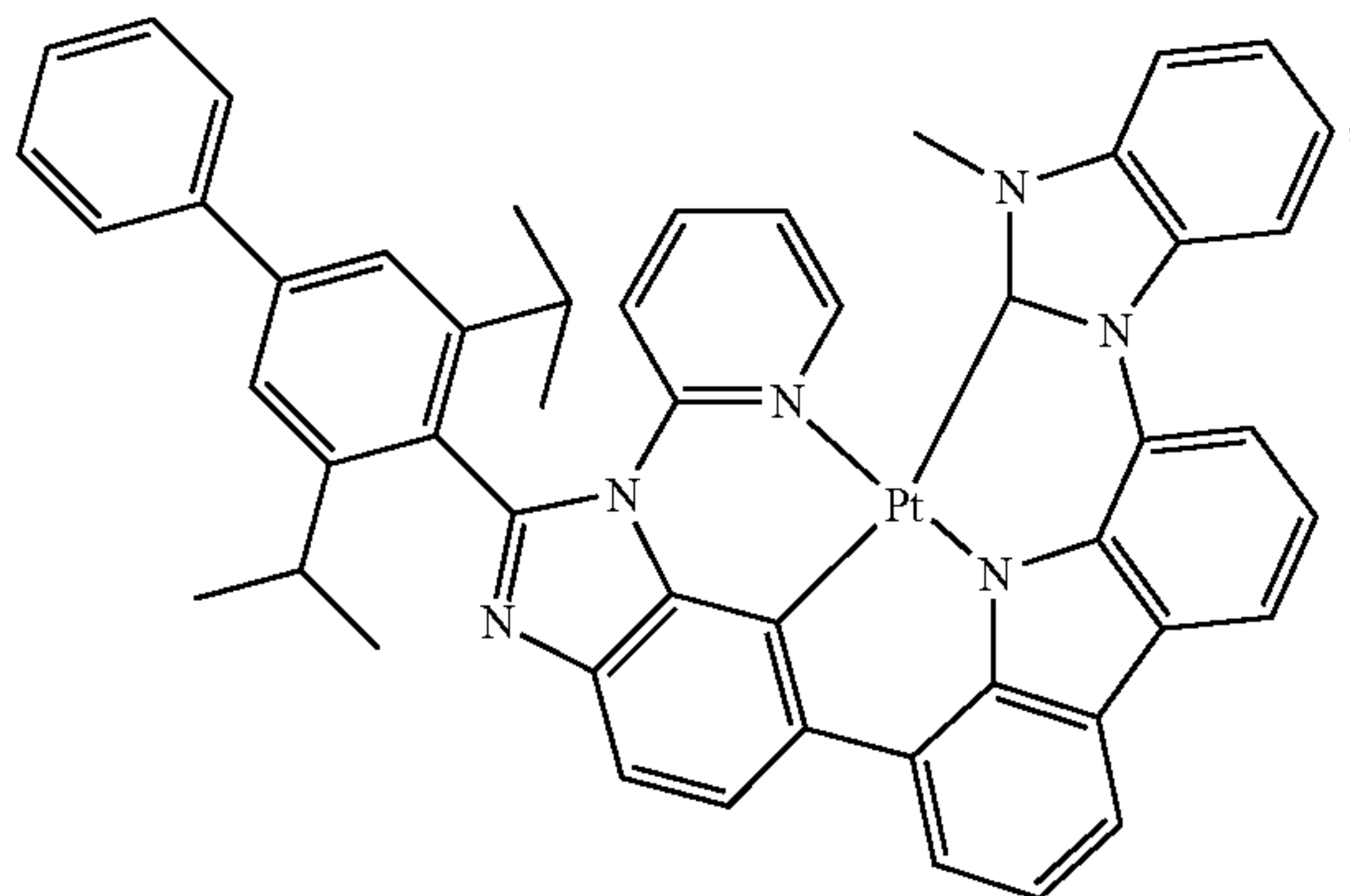
Compound 74
