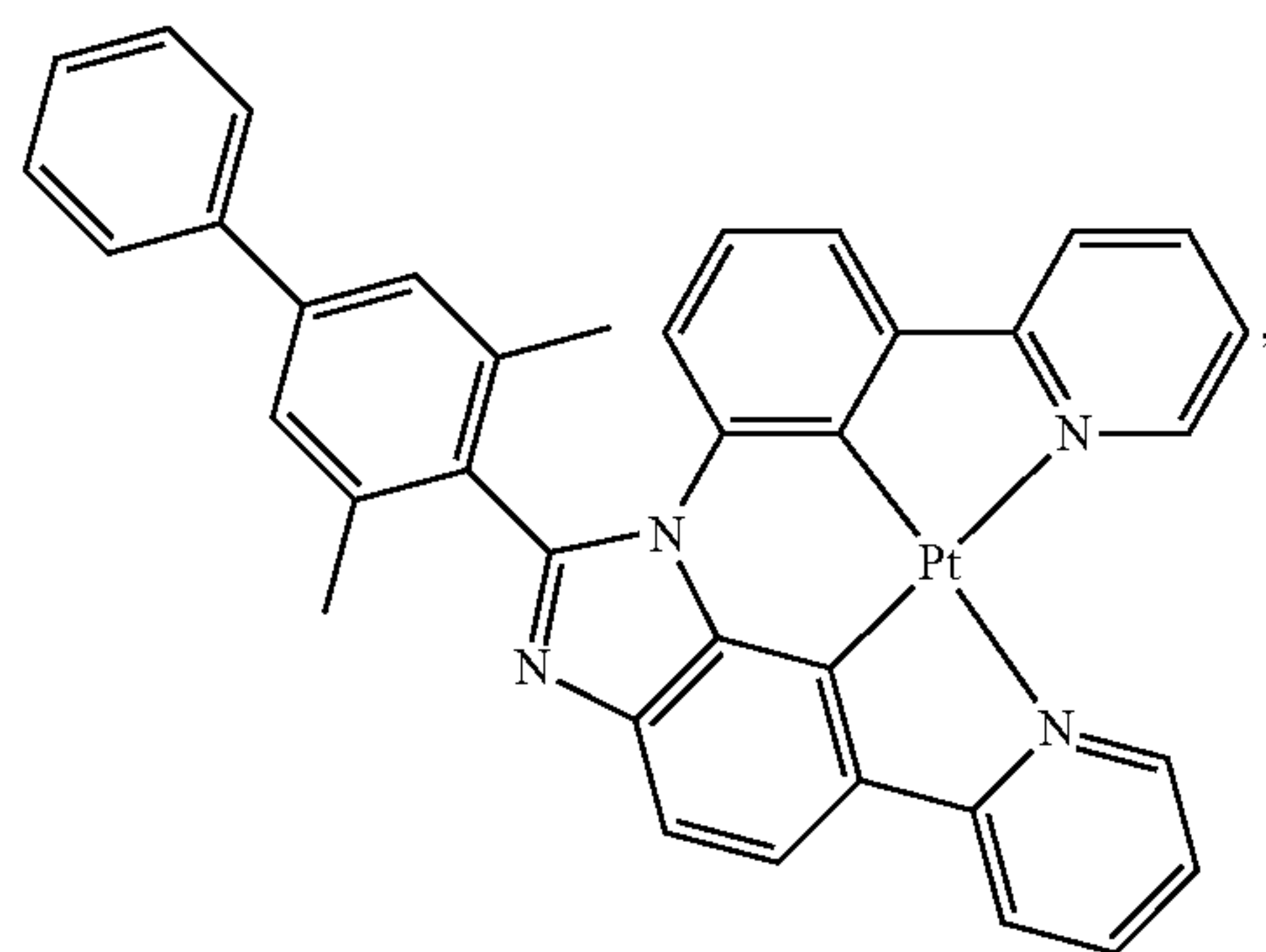
Compound 6
