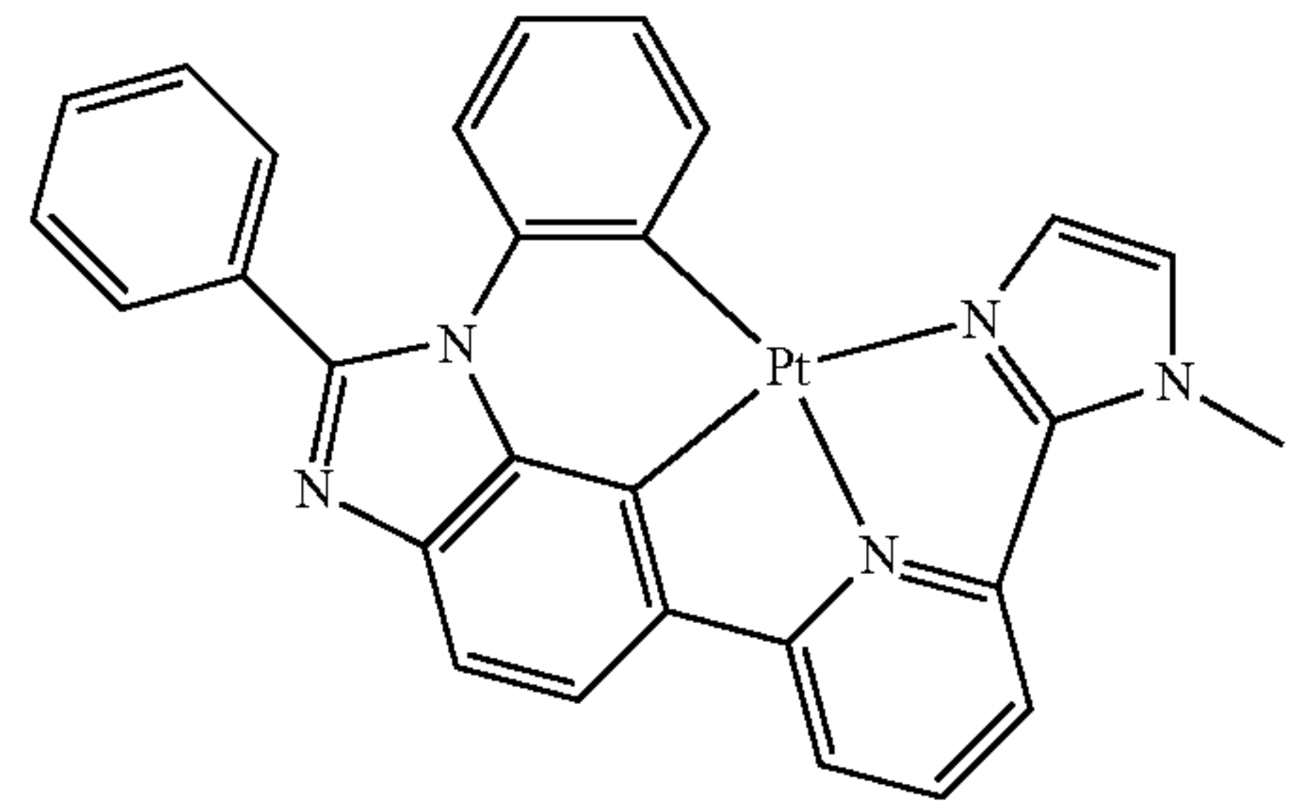
Compound 41
