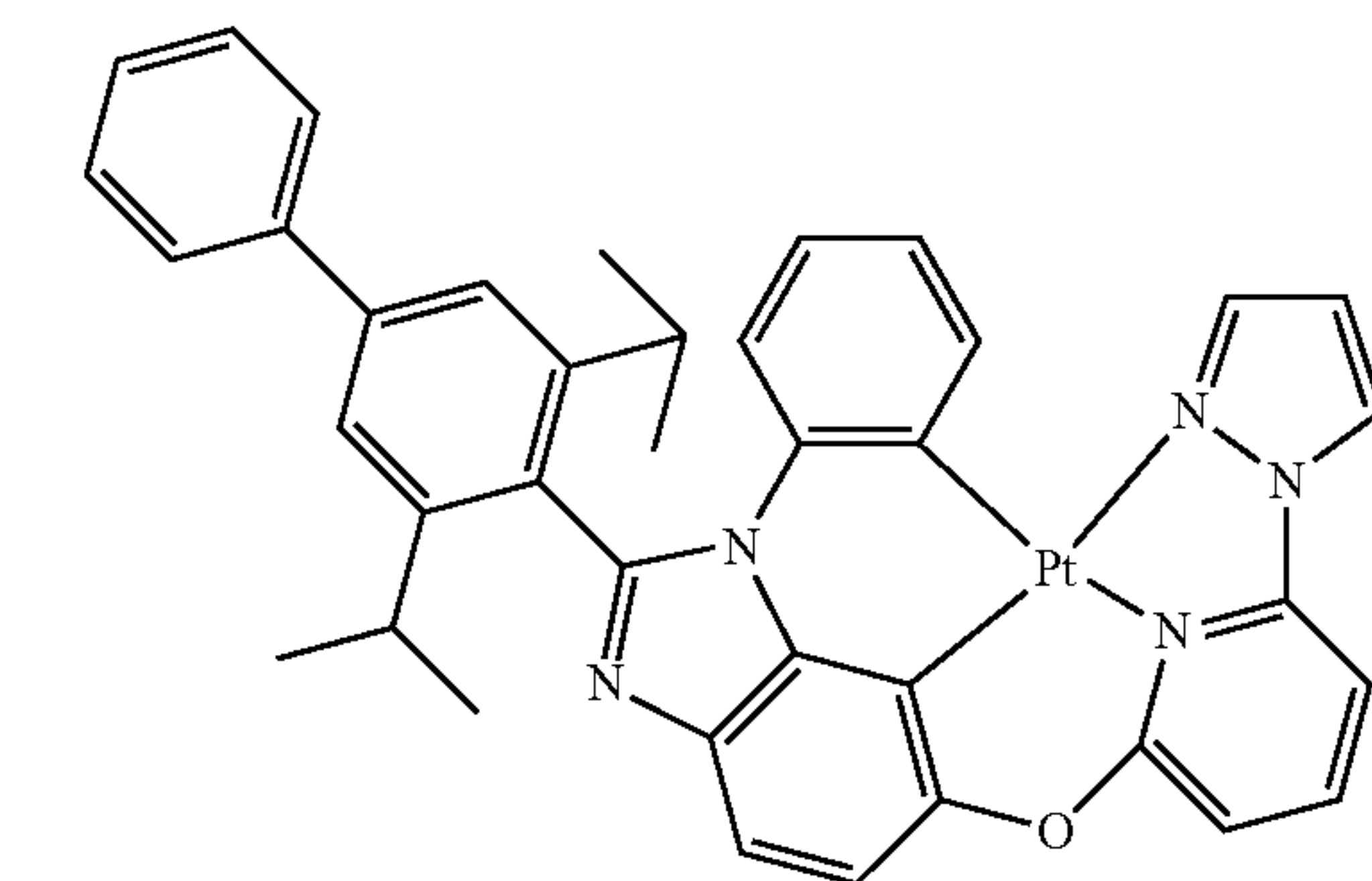
Compound 61
