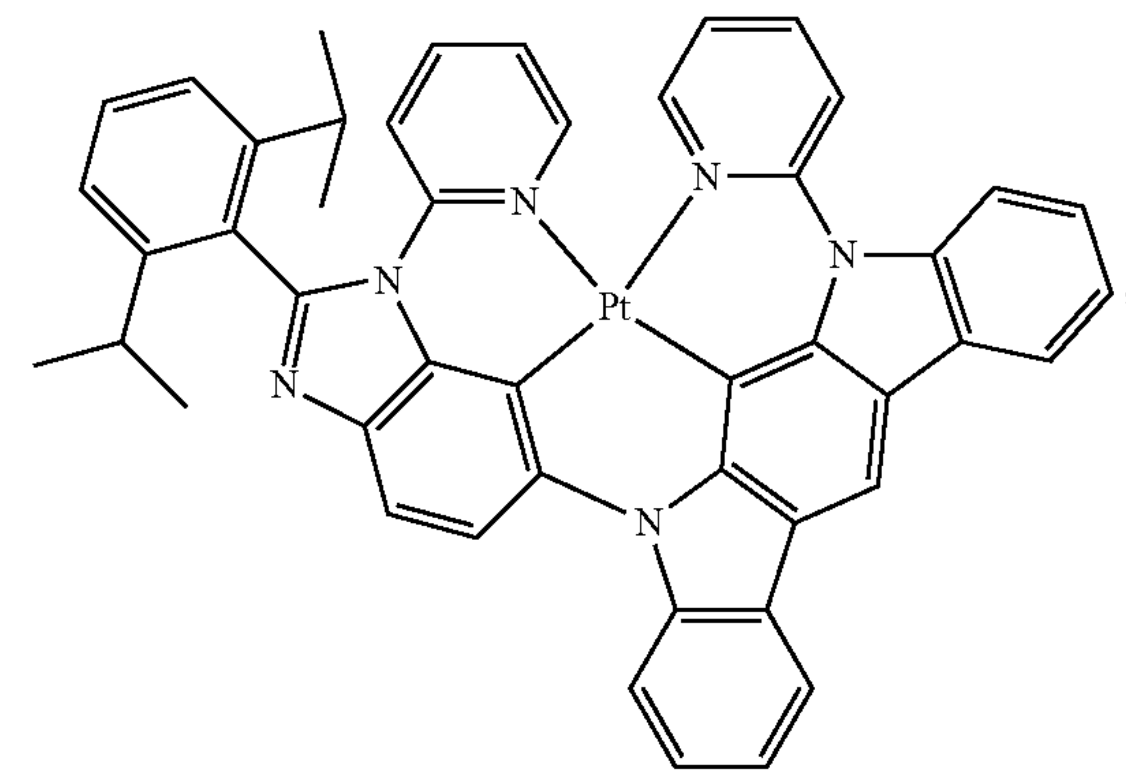
Compound 89
