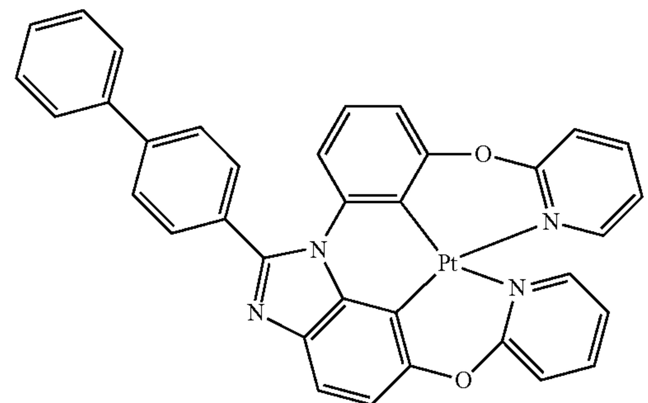
Compound 12
