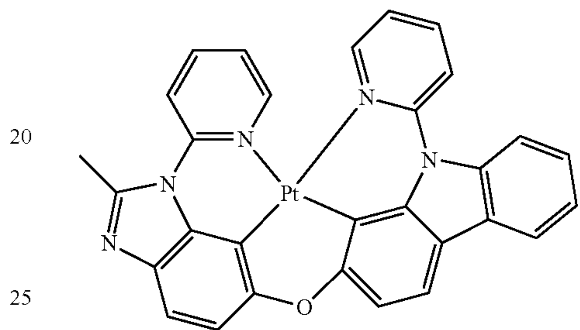
Compound 65
