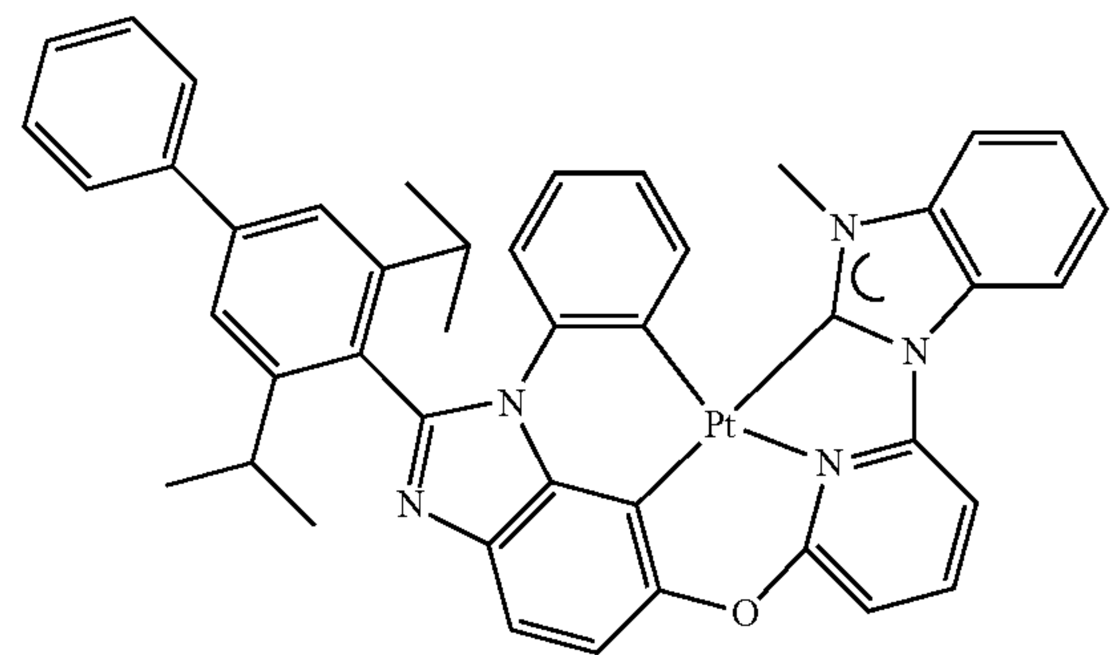
Compound 31
