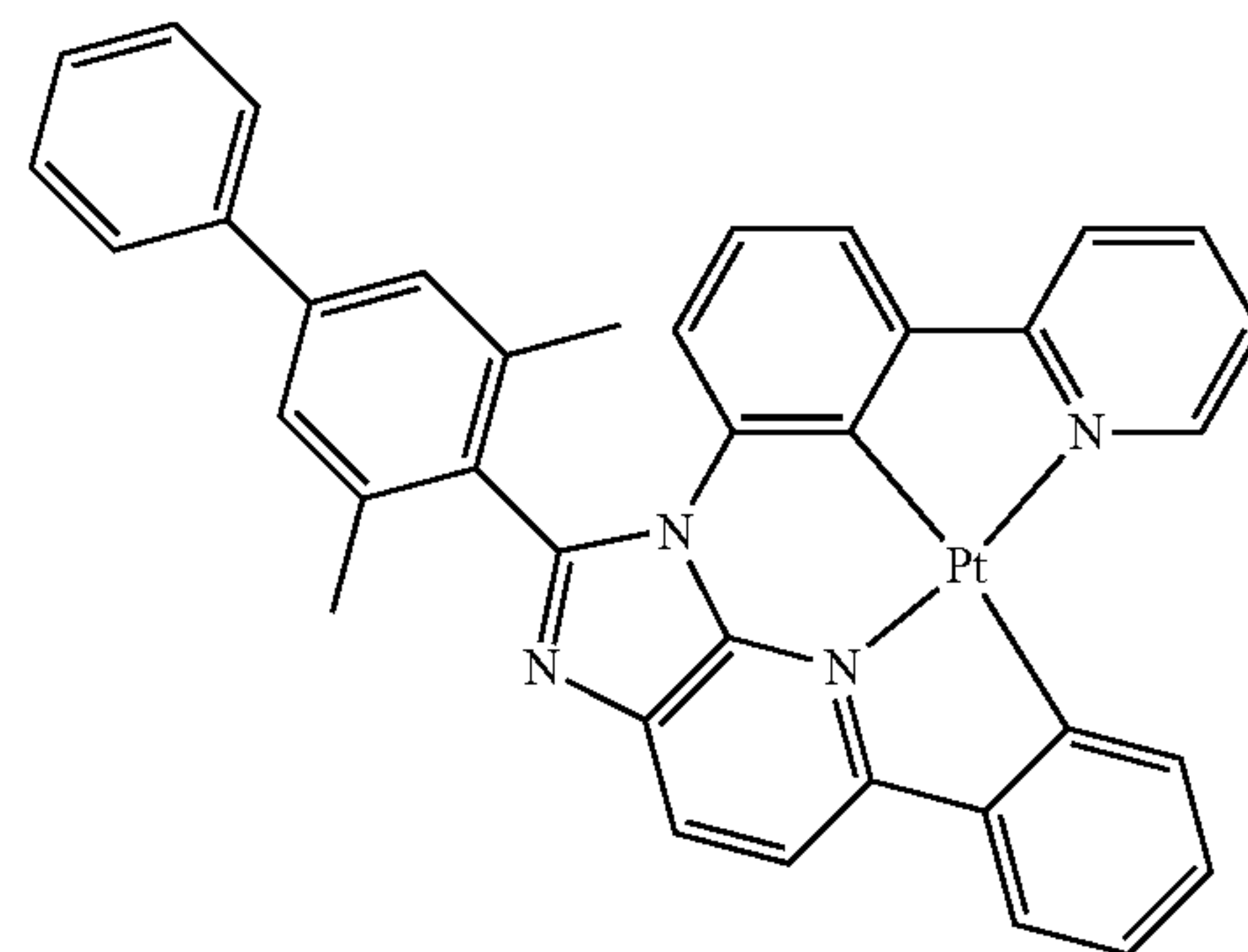
Compound 103
