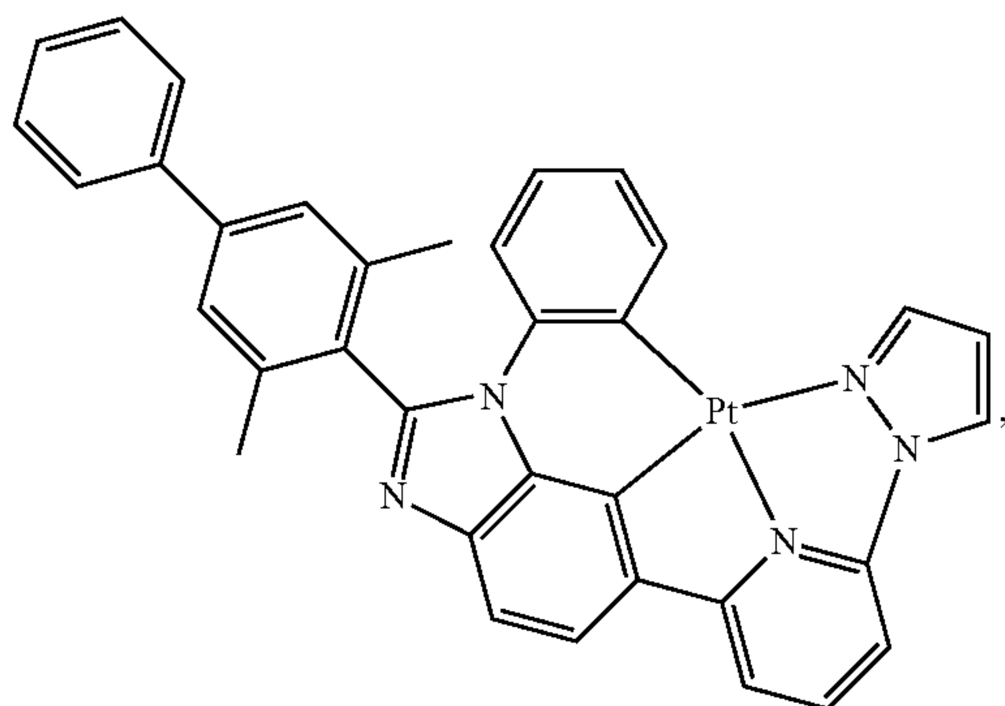
Compound 56
