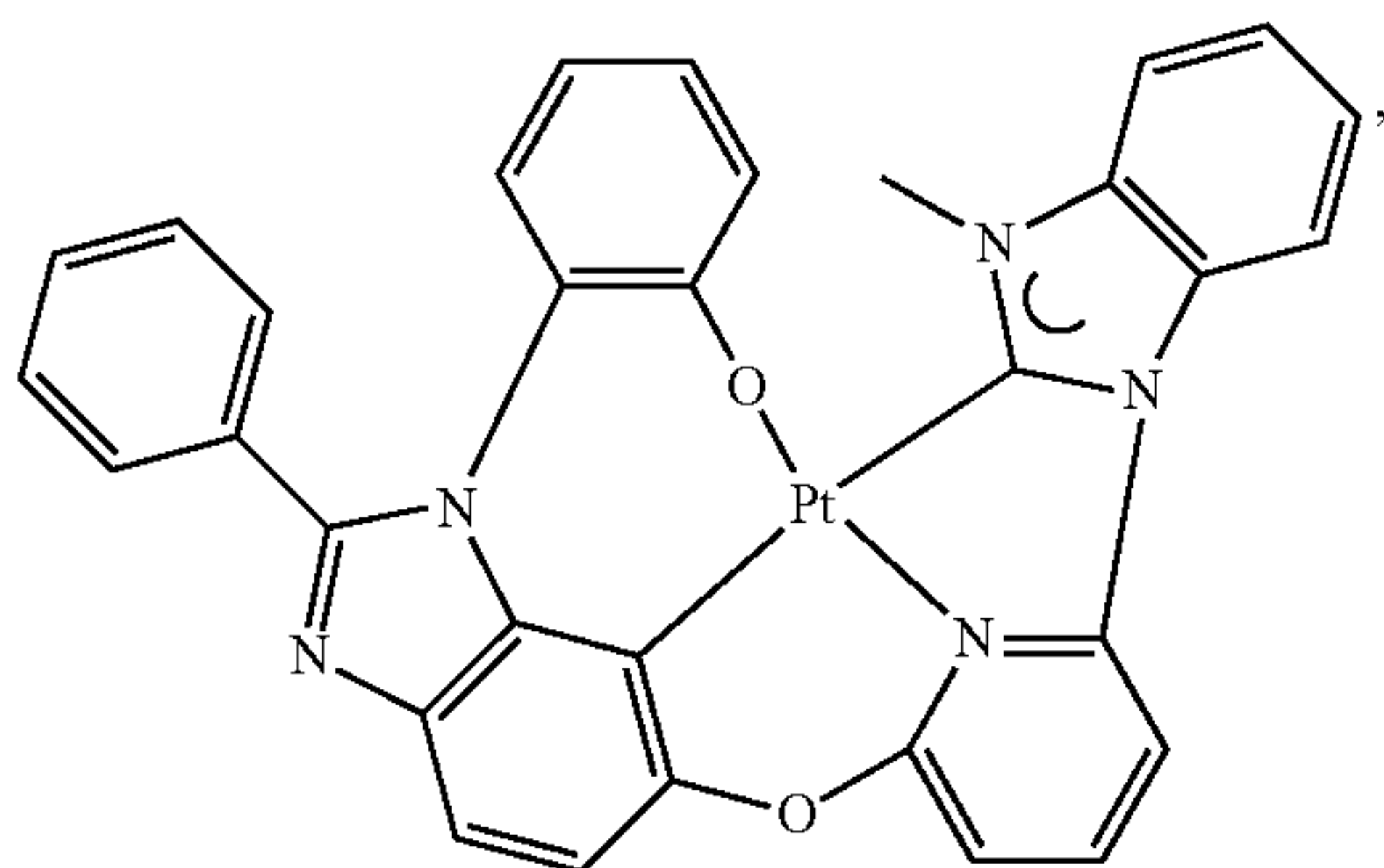
Compound 36
