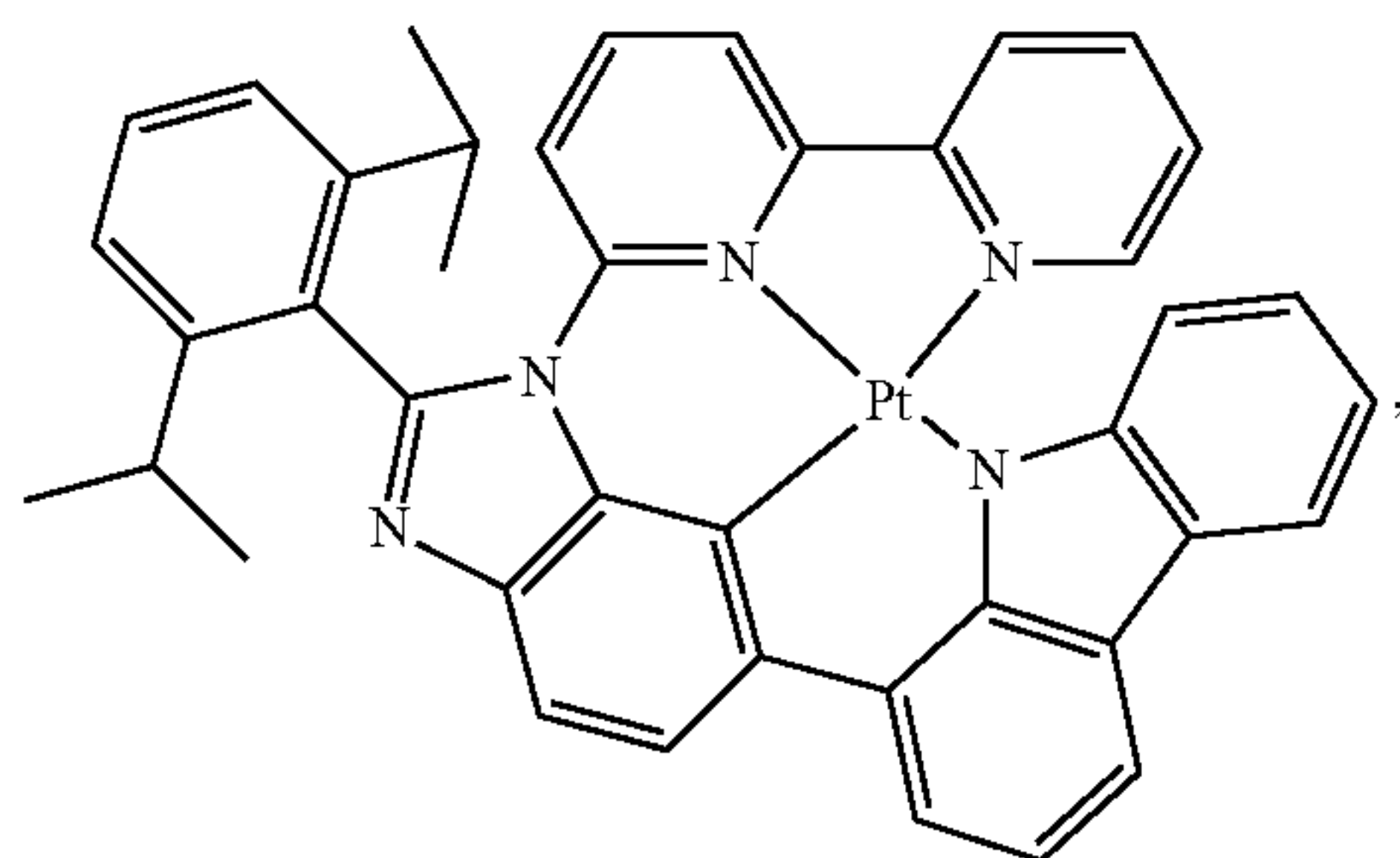
Compound 66
