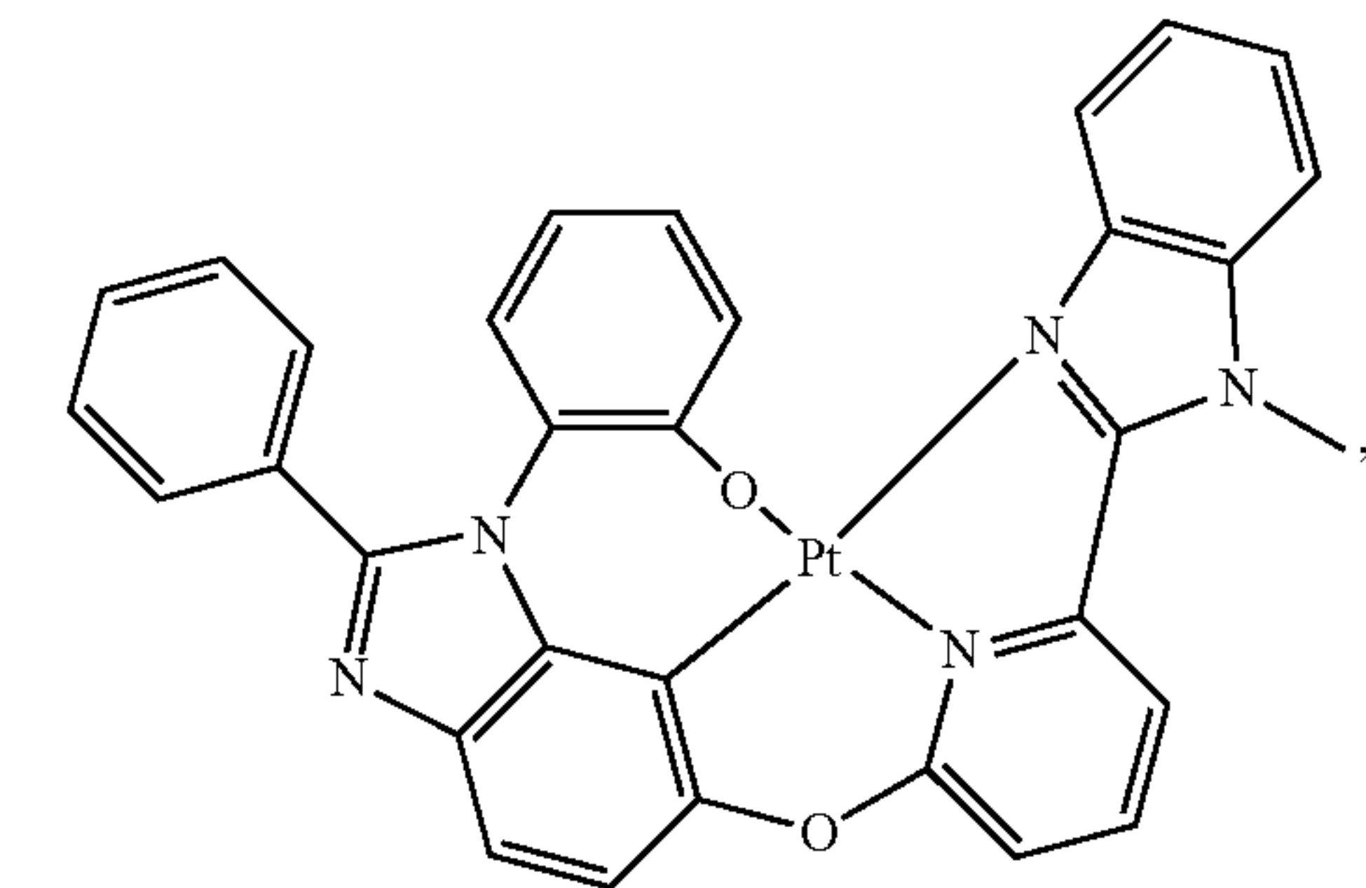
Compound 50
