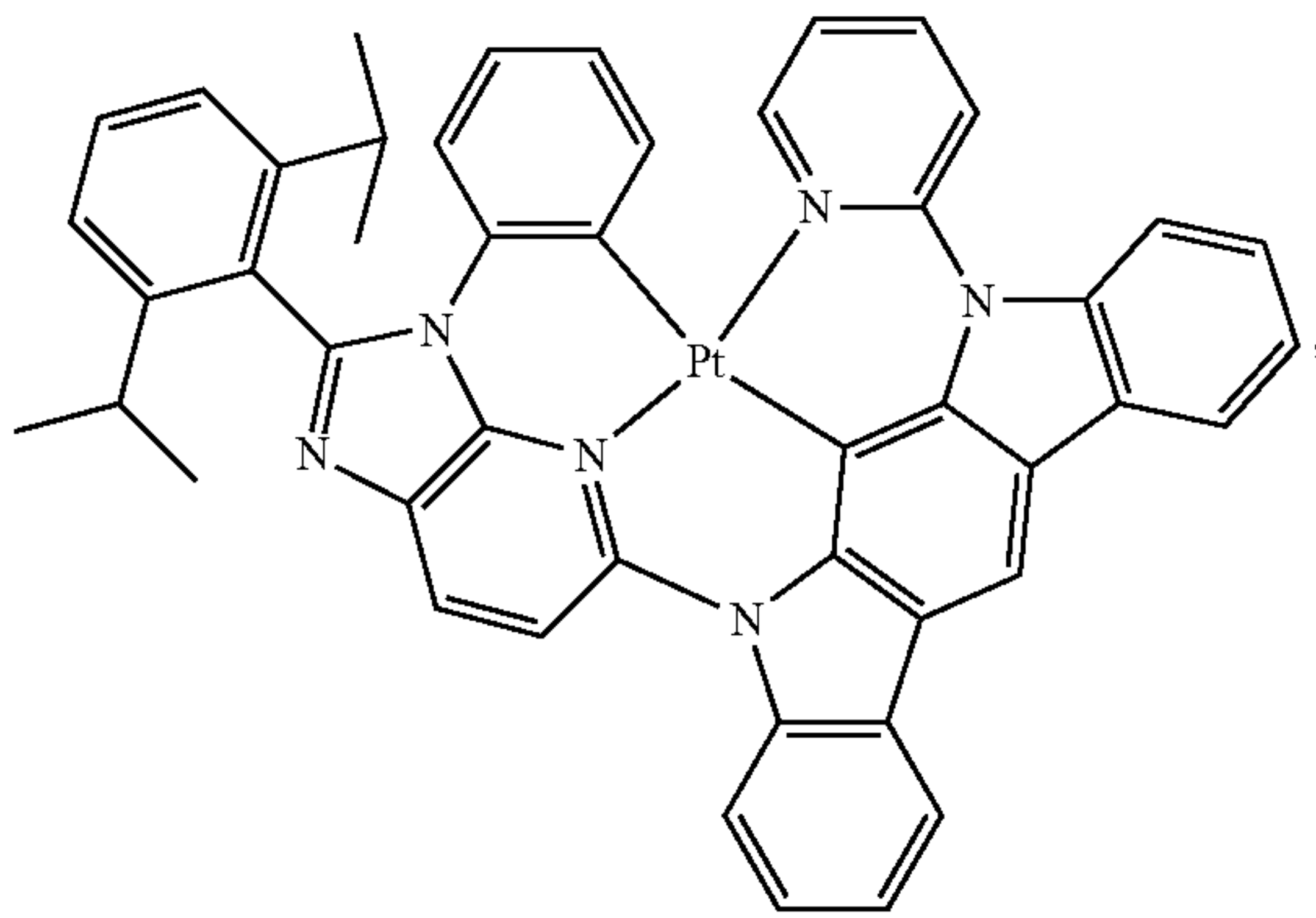
Compound 92
