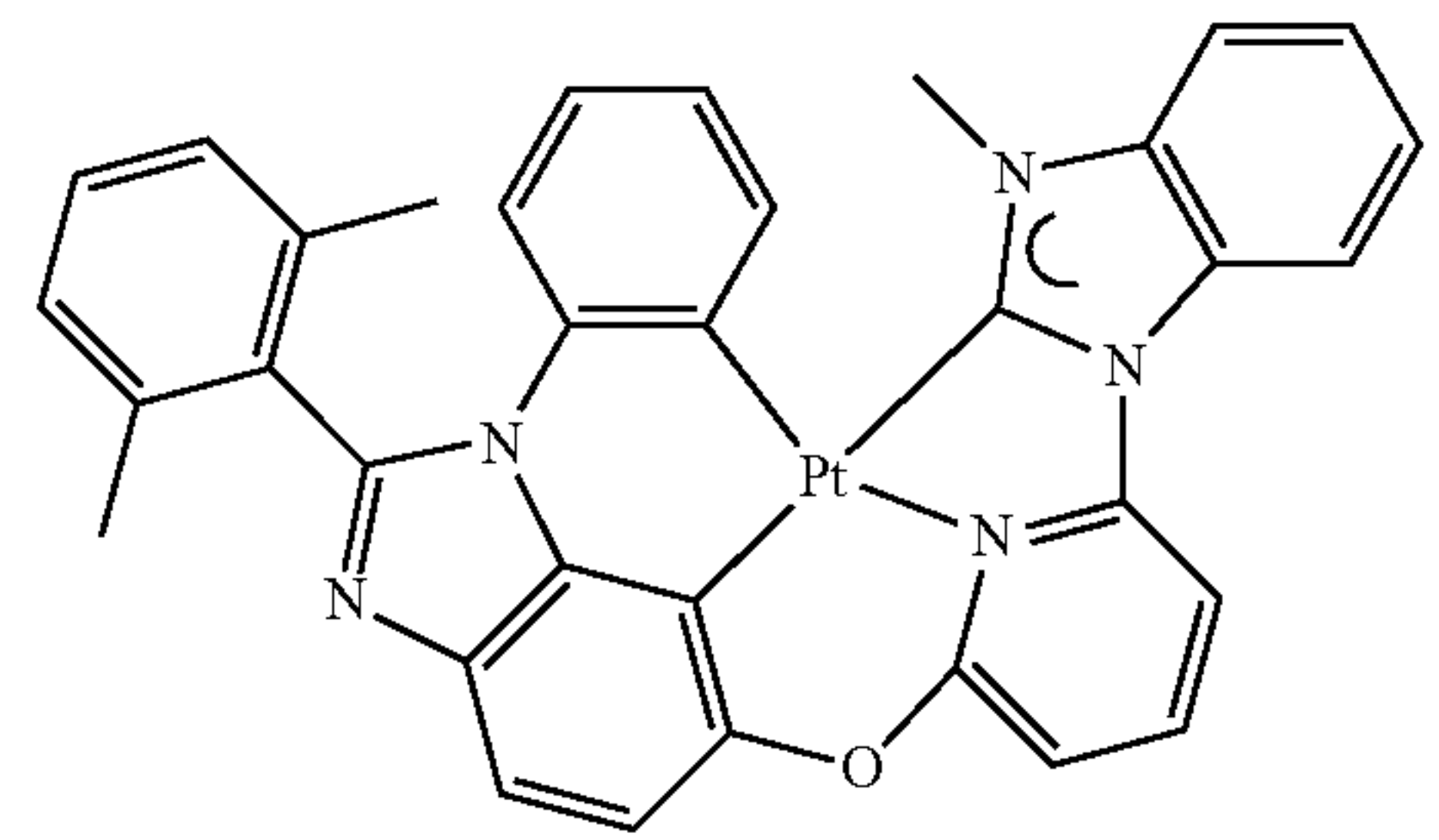
Compound 29
