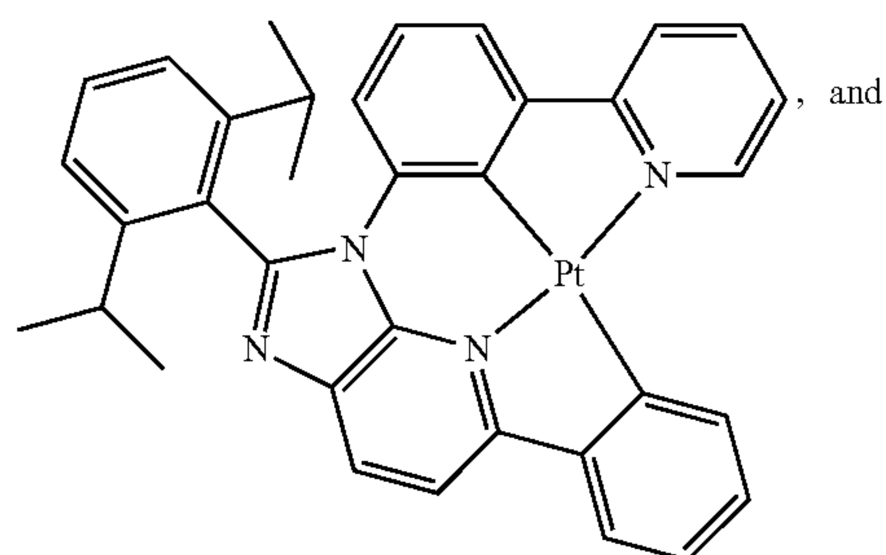
Compound 102
