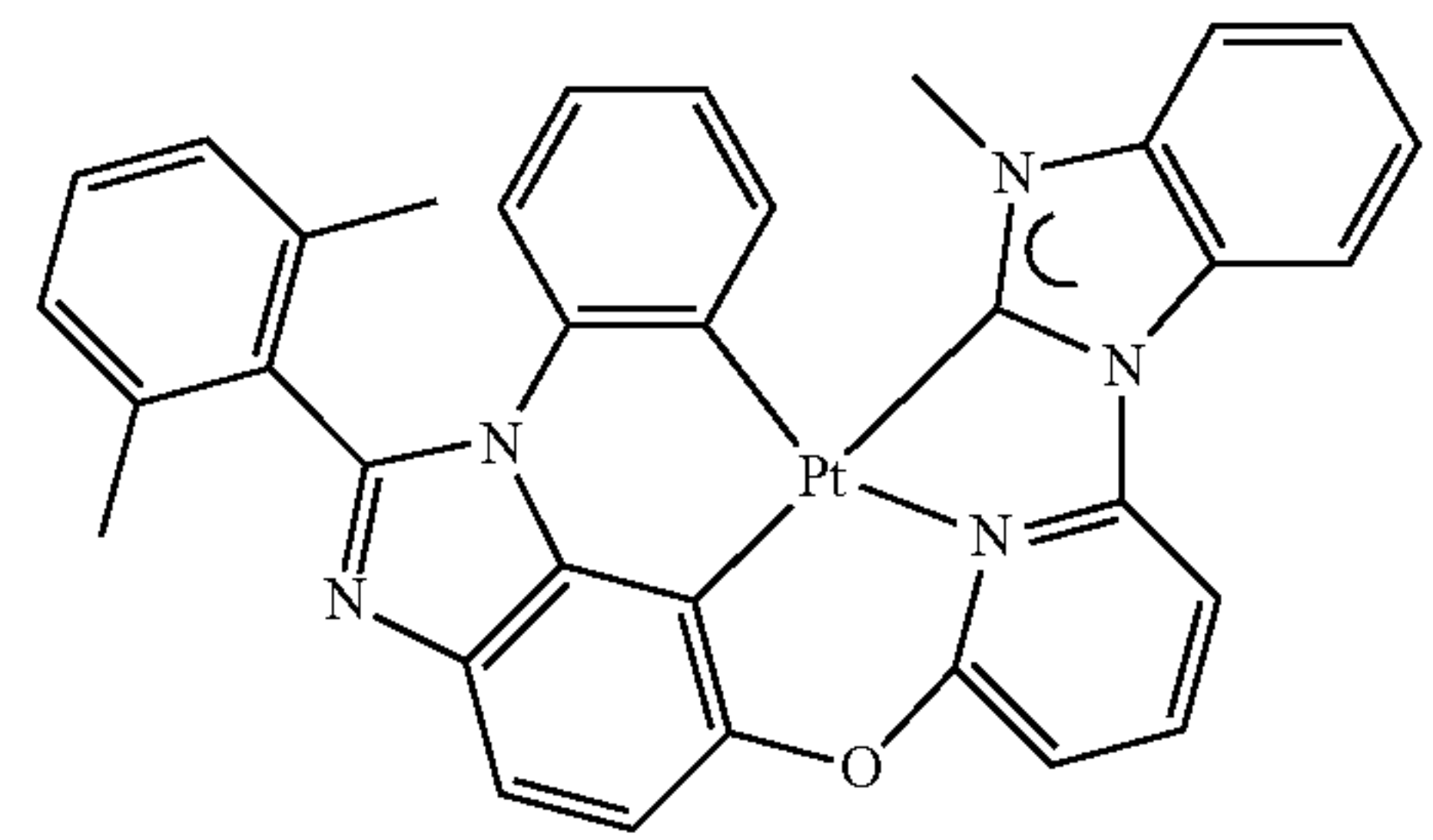
Compound 29
