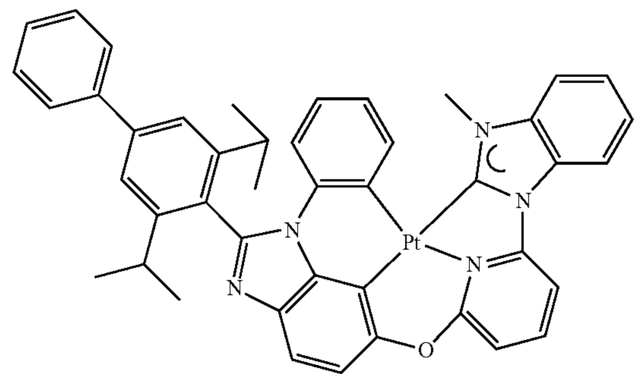
Compound 31
