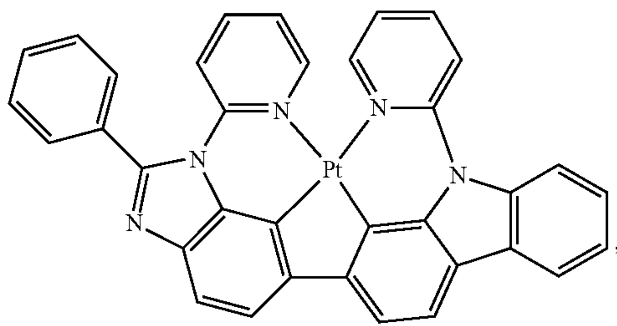
Compound 65
