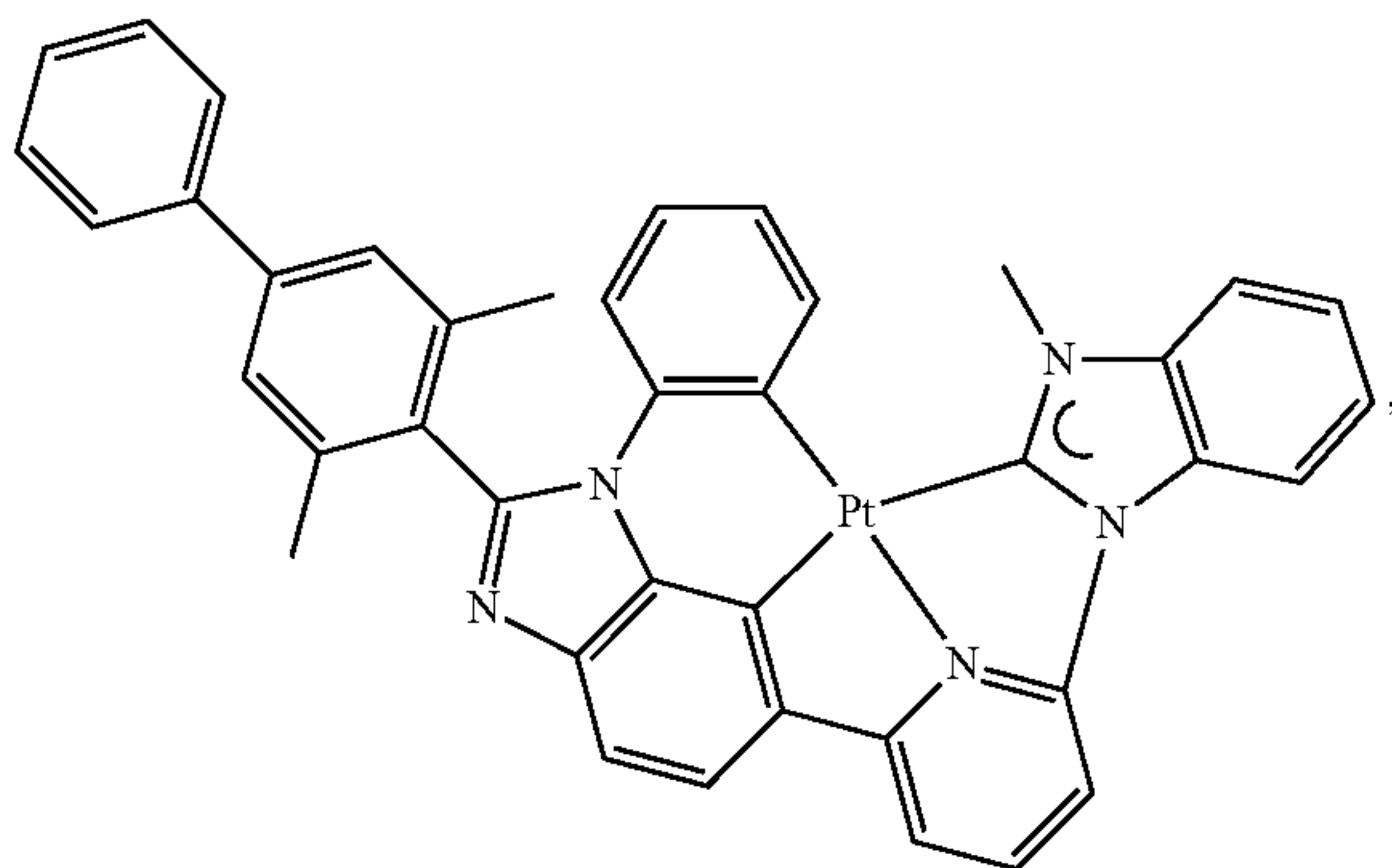
Compound 26
