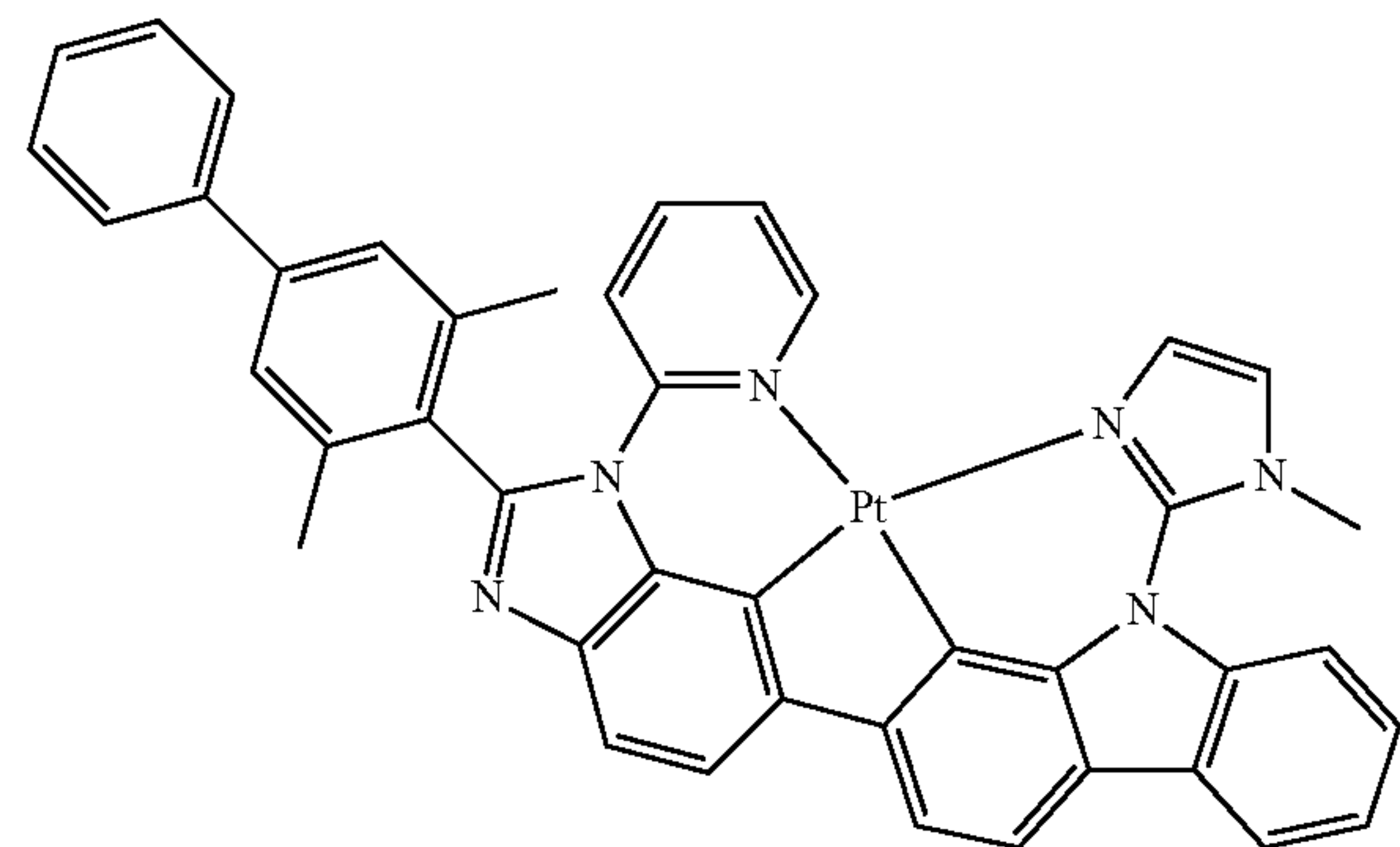
Compound 81
