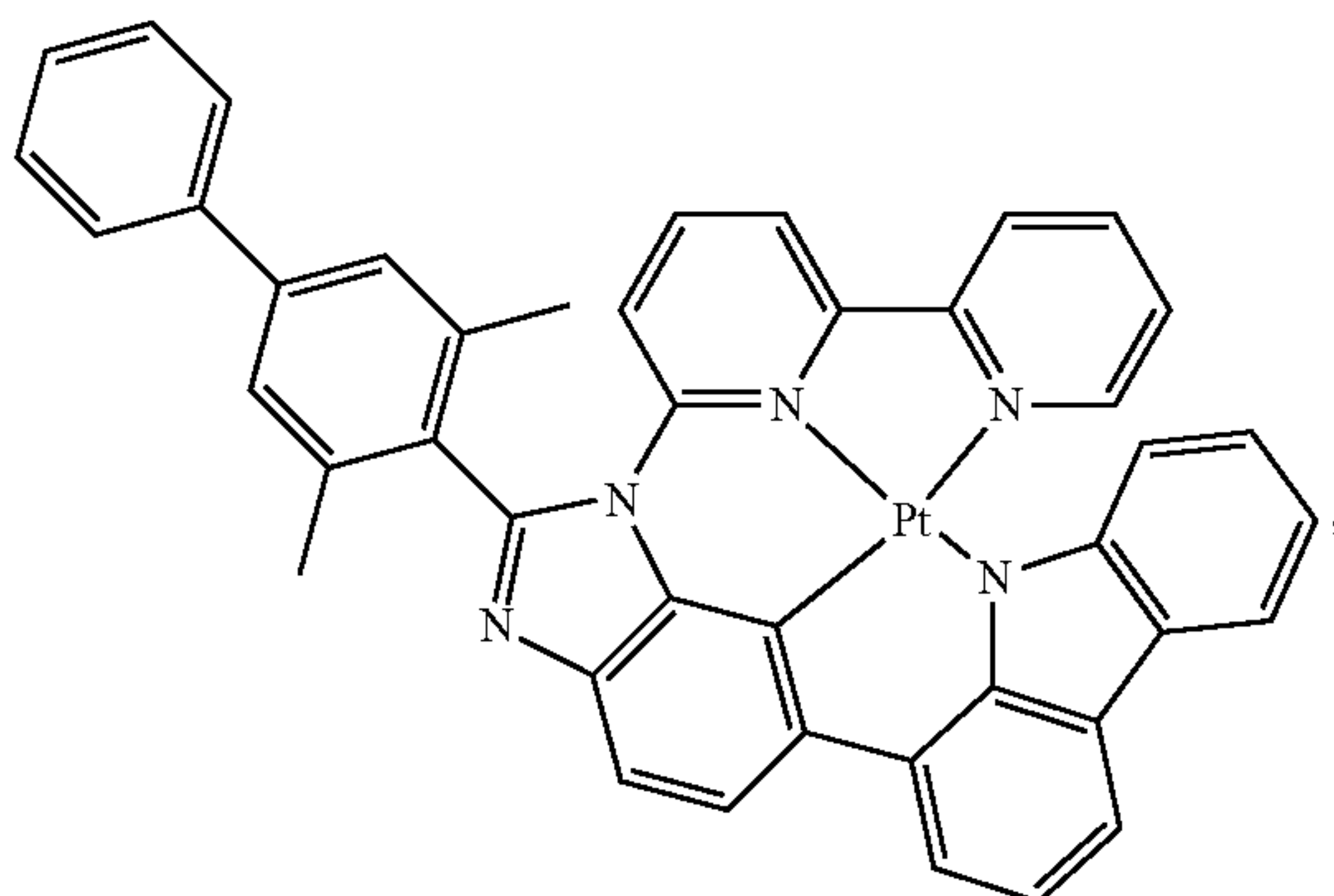
Compound 67
