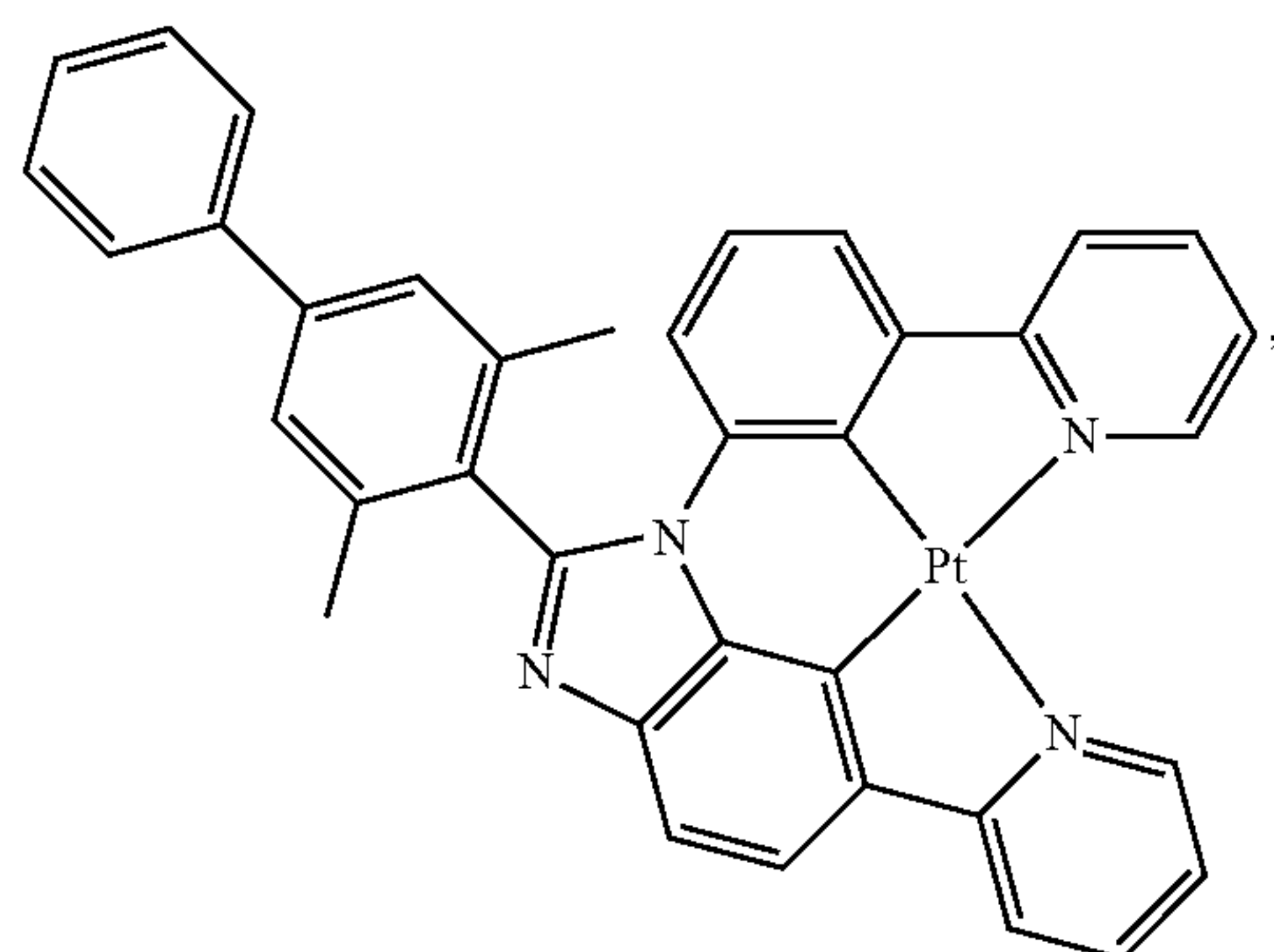
Compound 6
