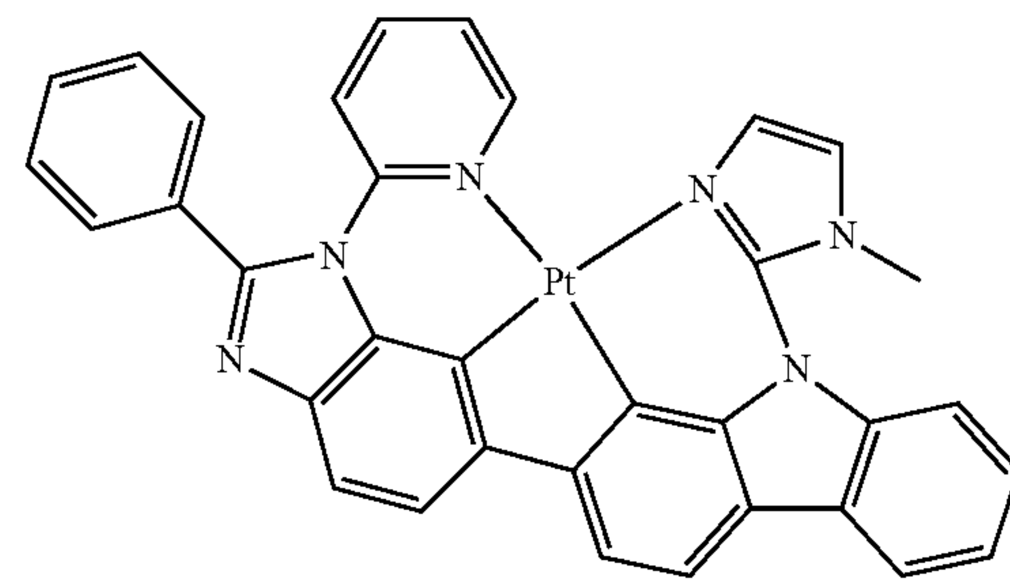
Compound 79
