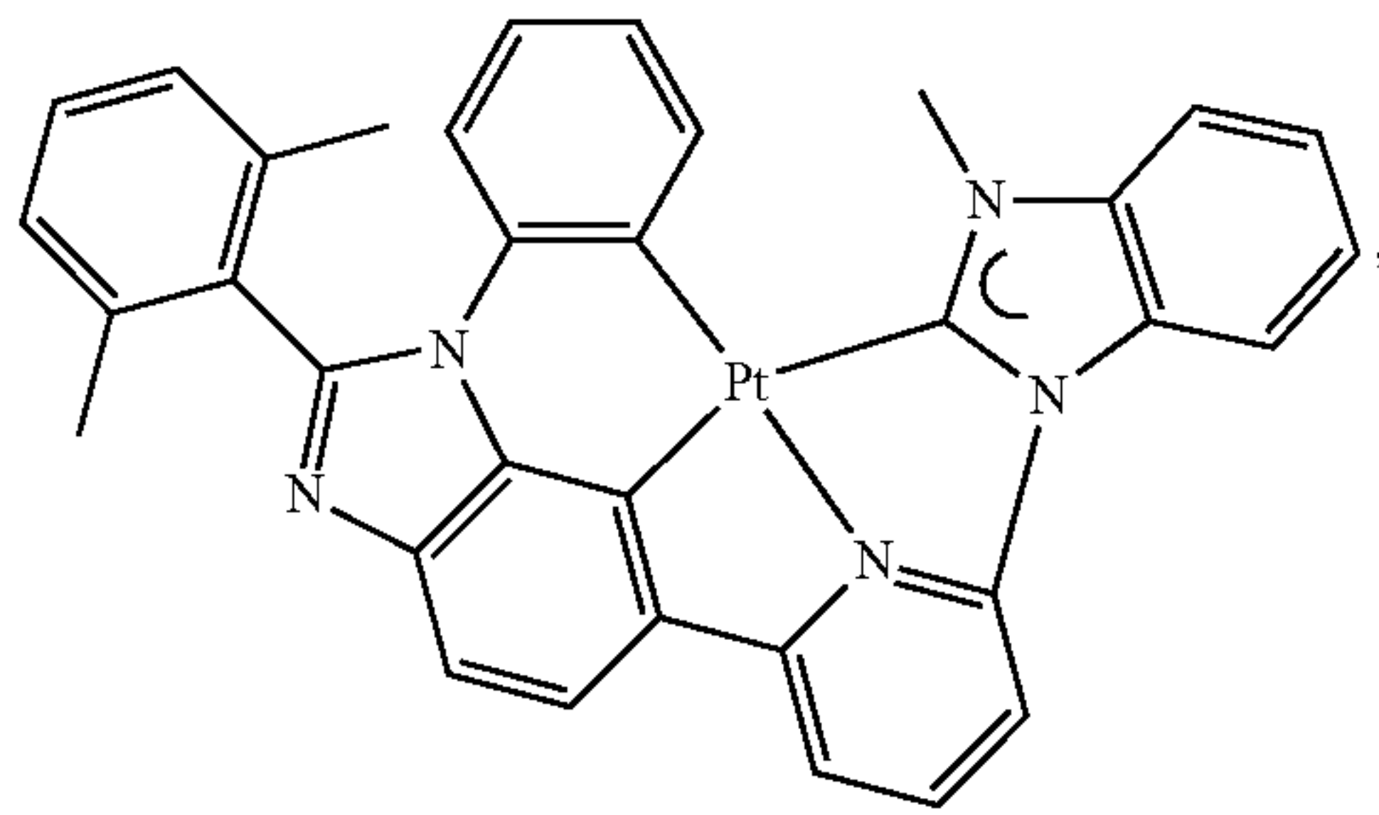
Compound 24
