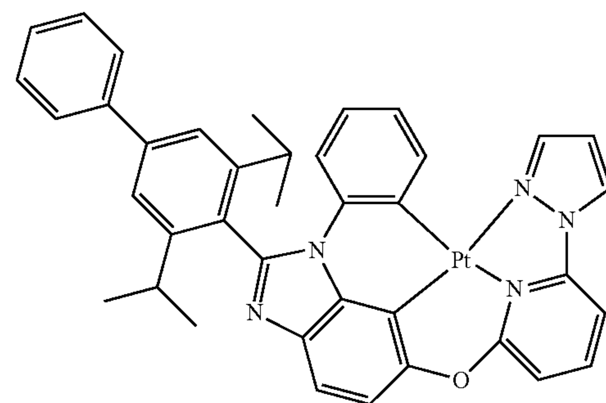
Compound 61
