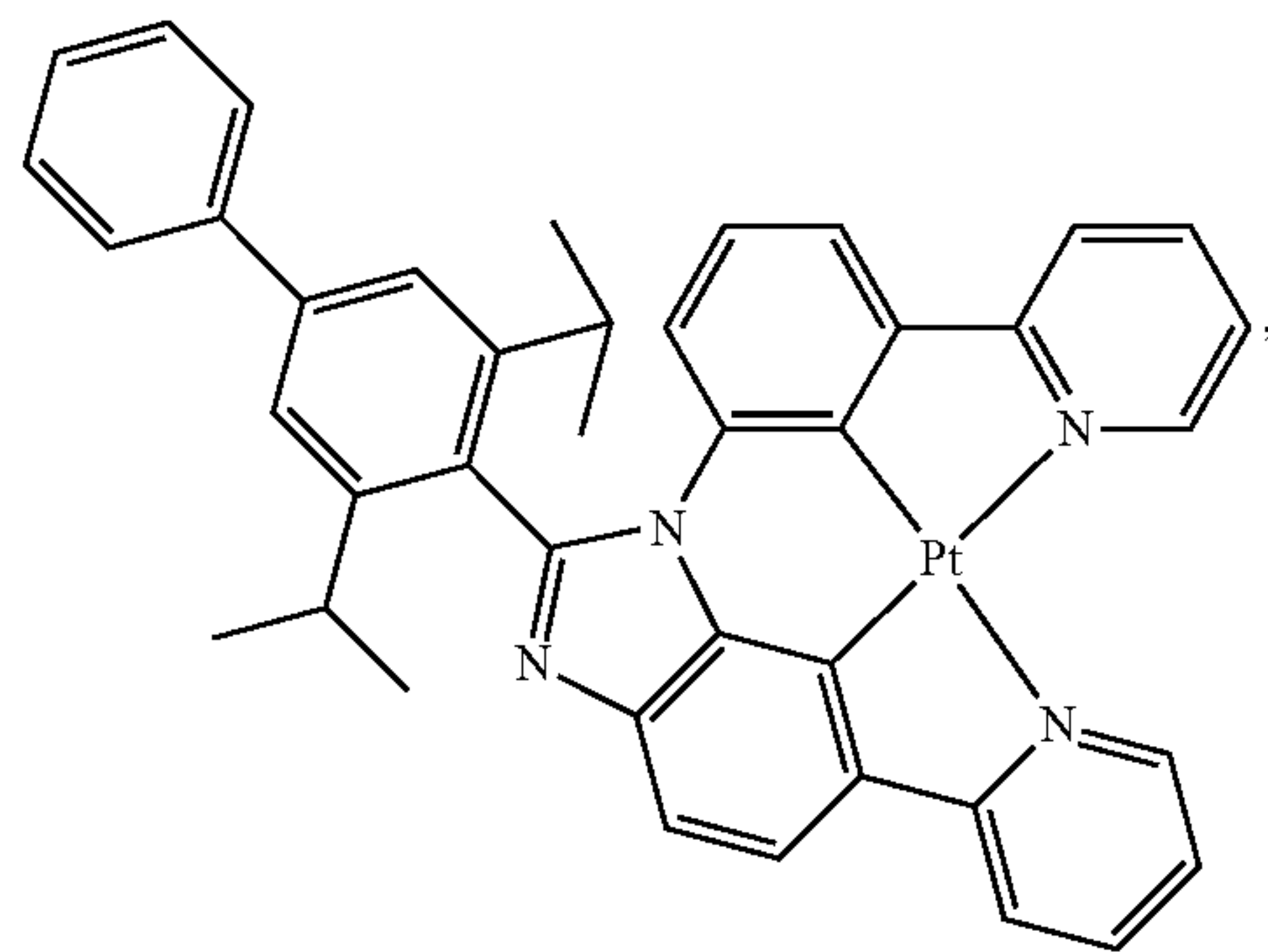
Compound 7
