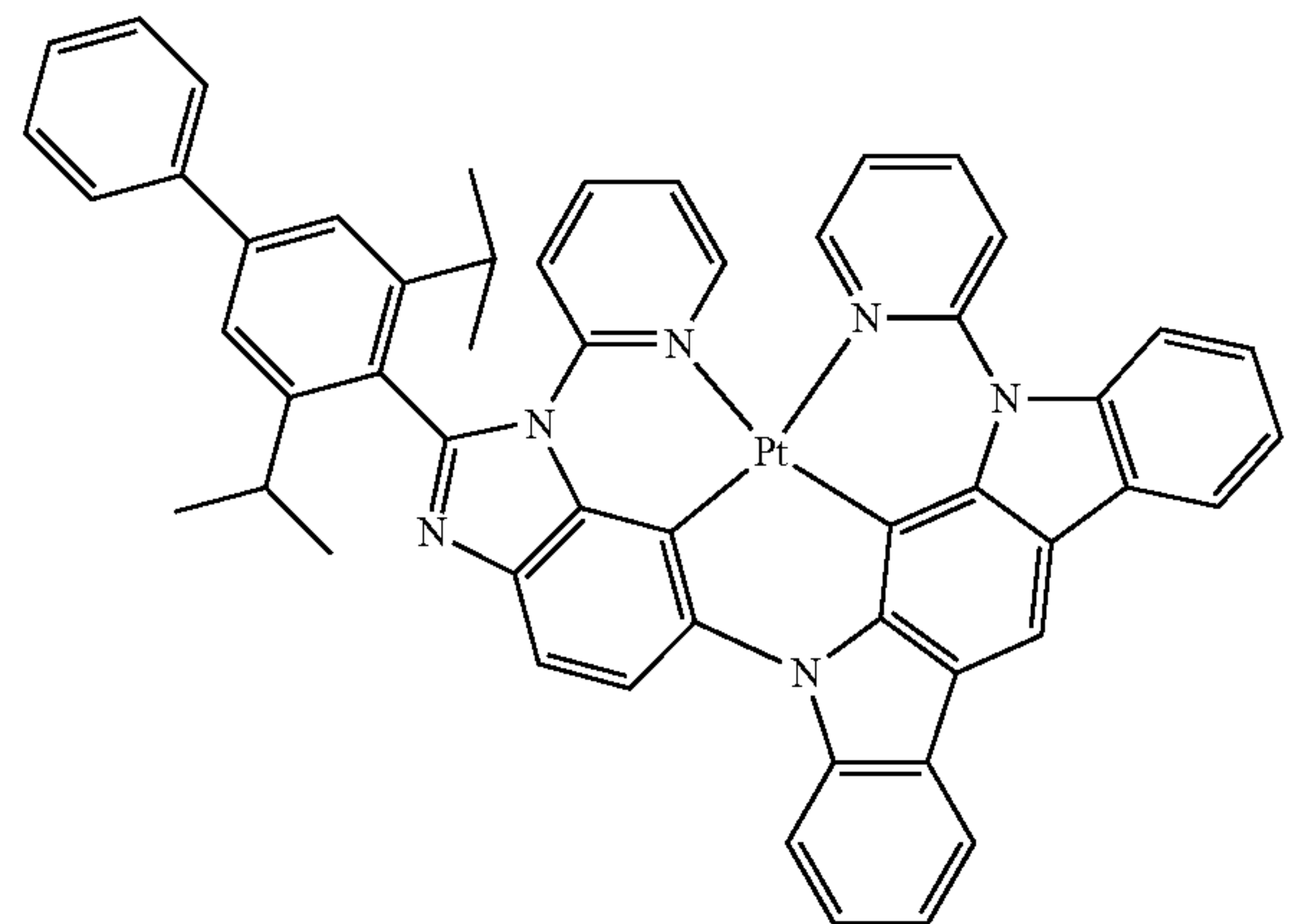
Compound 89
