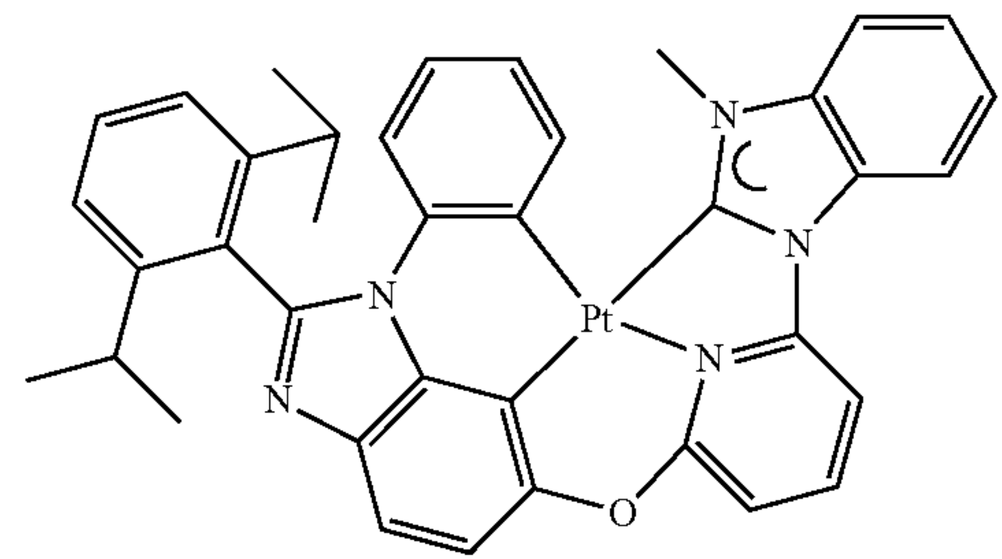
Compound 30
