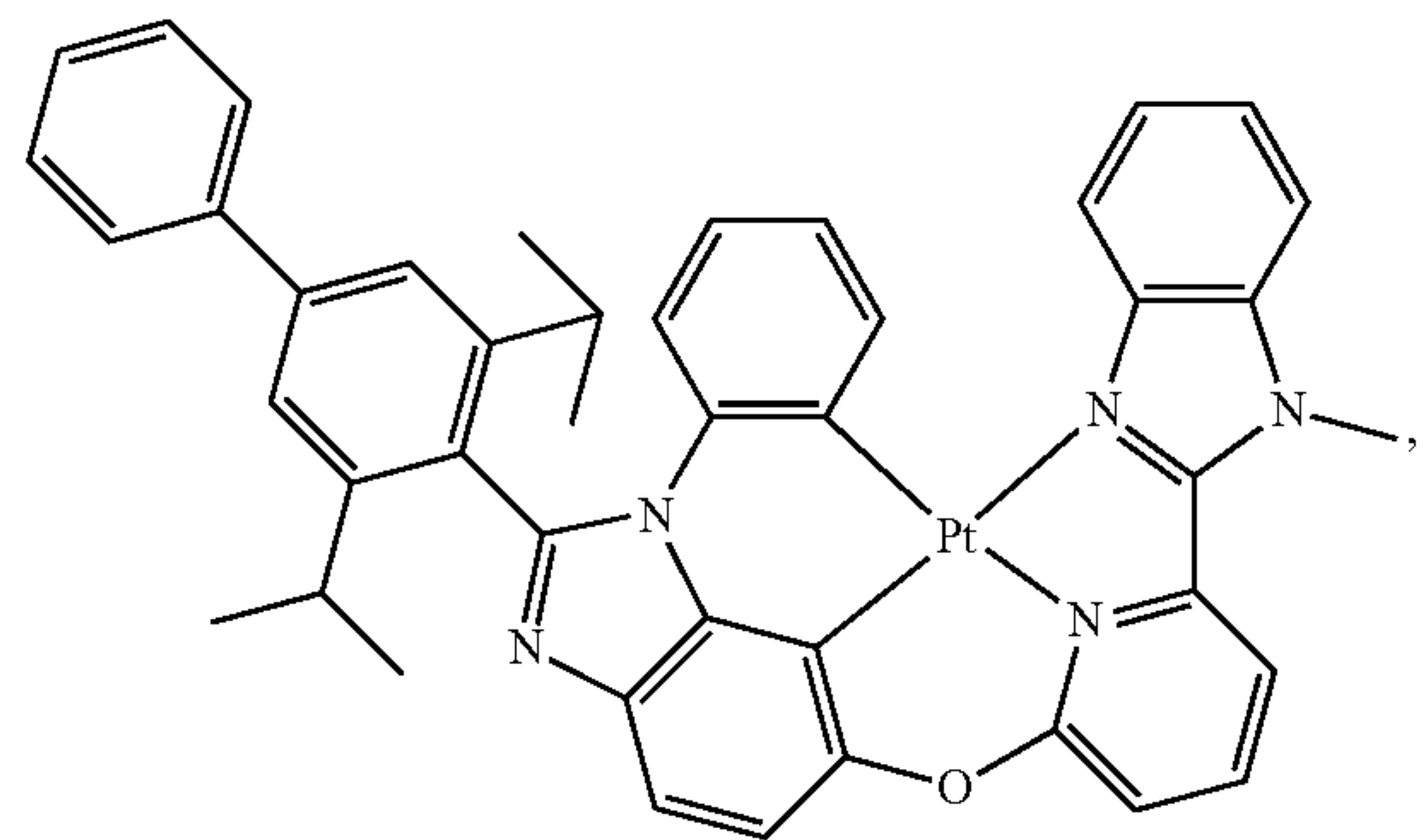
Compound 49
