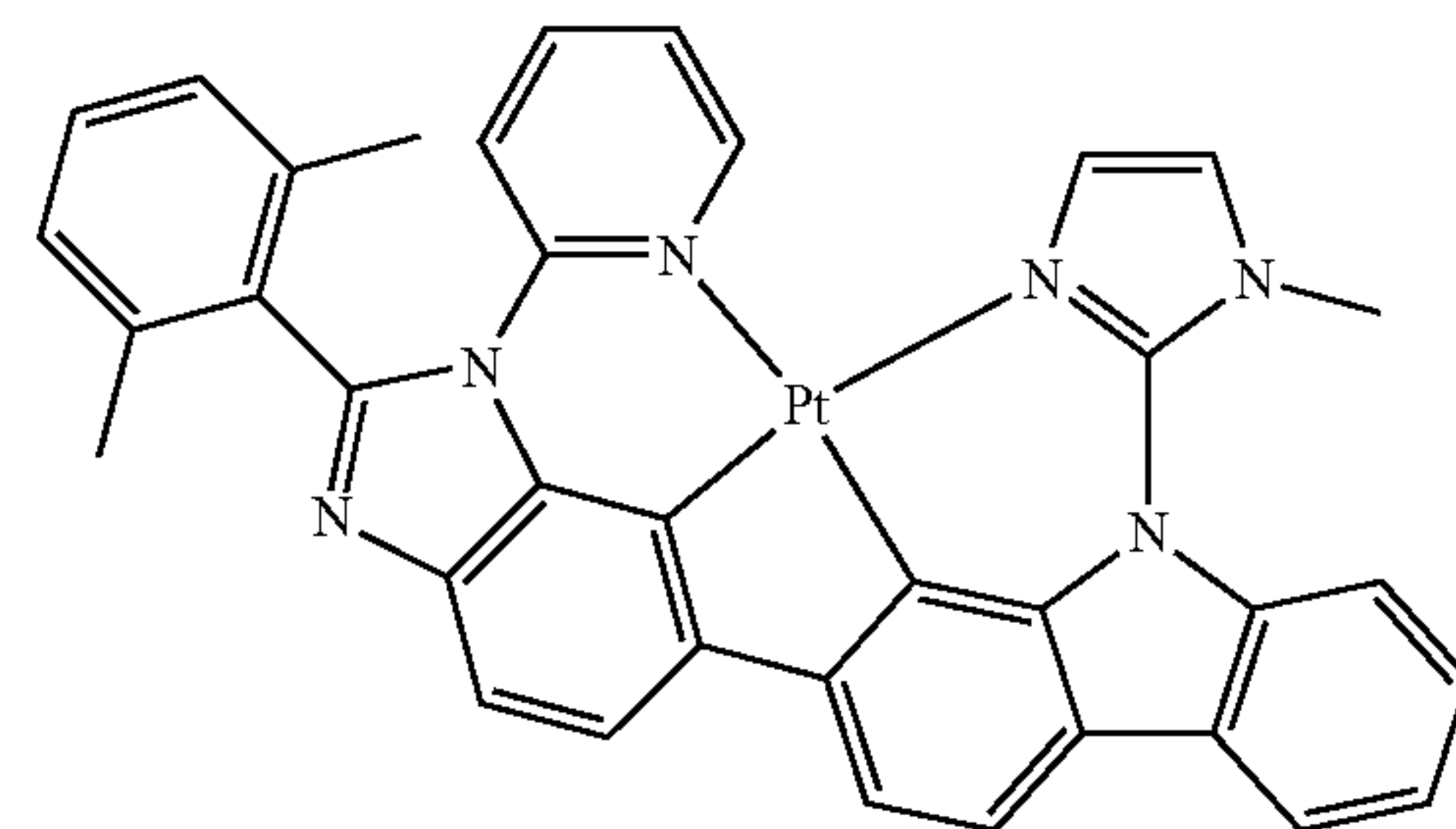
Compound 80
