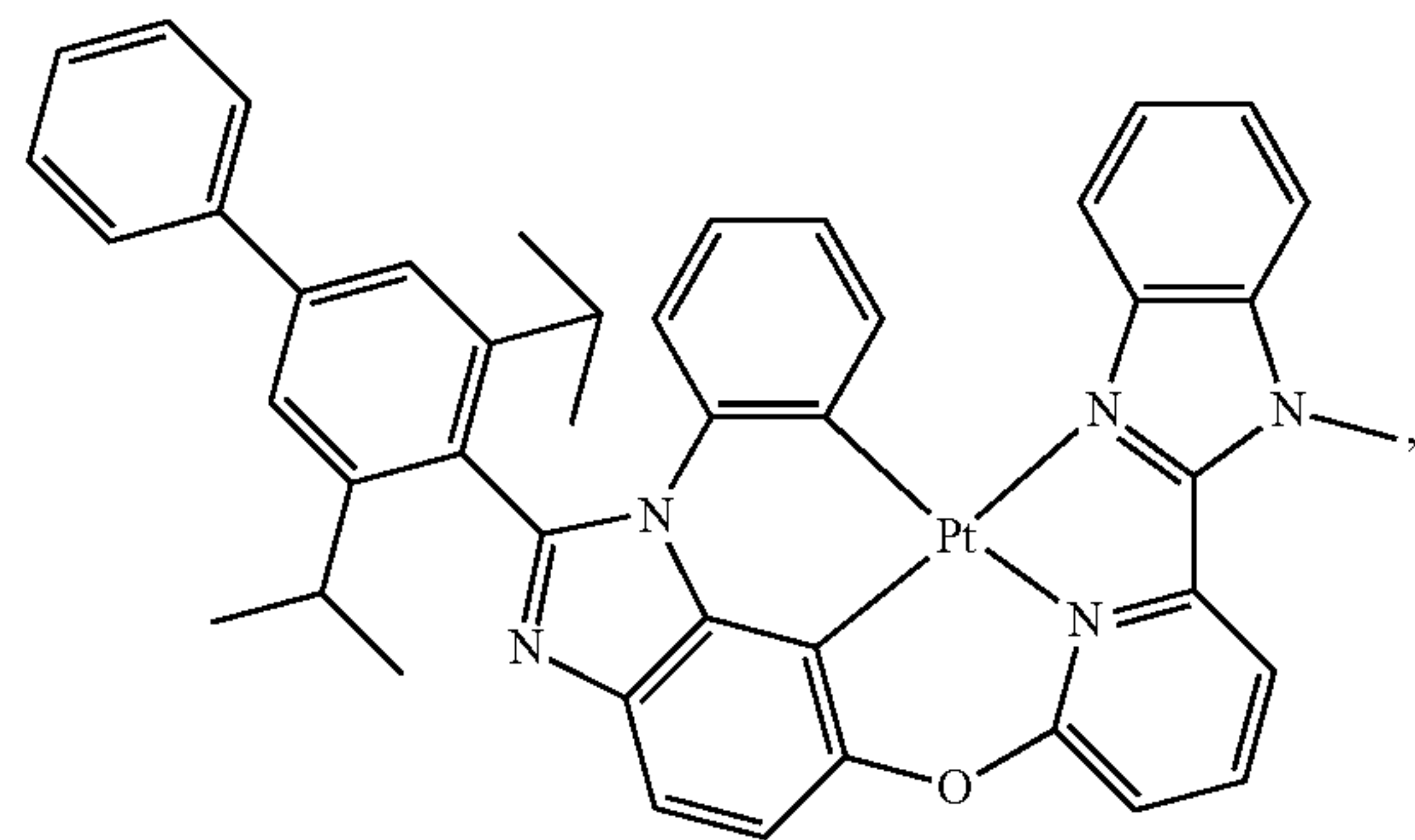
Compound 49
