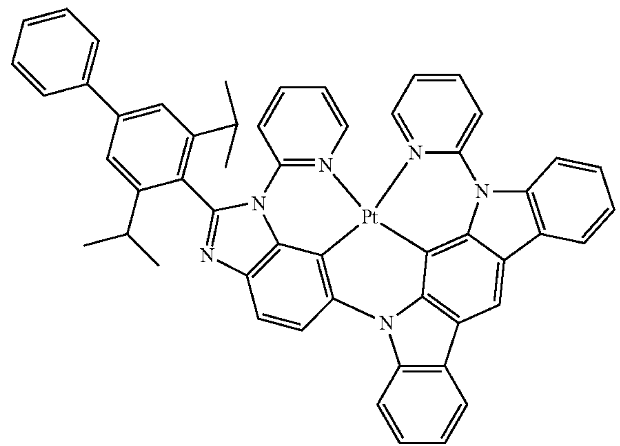
Compound 89
