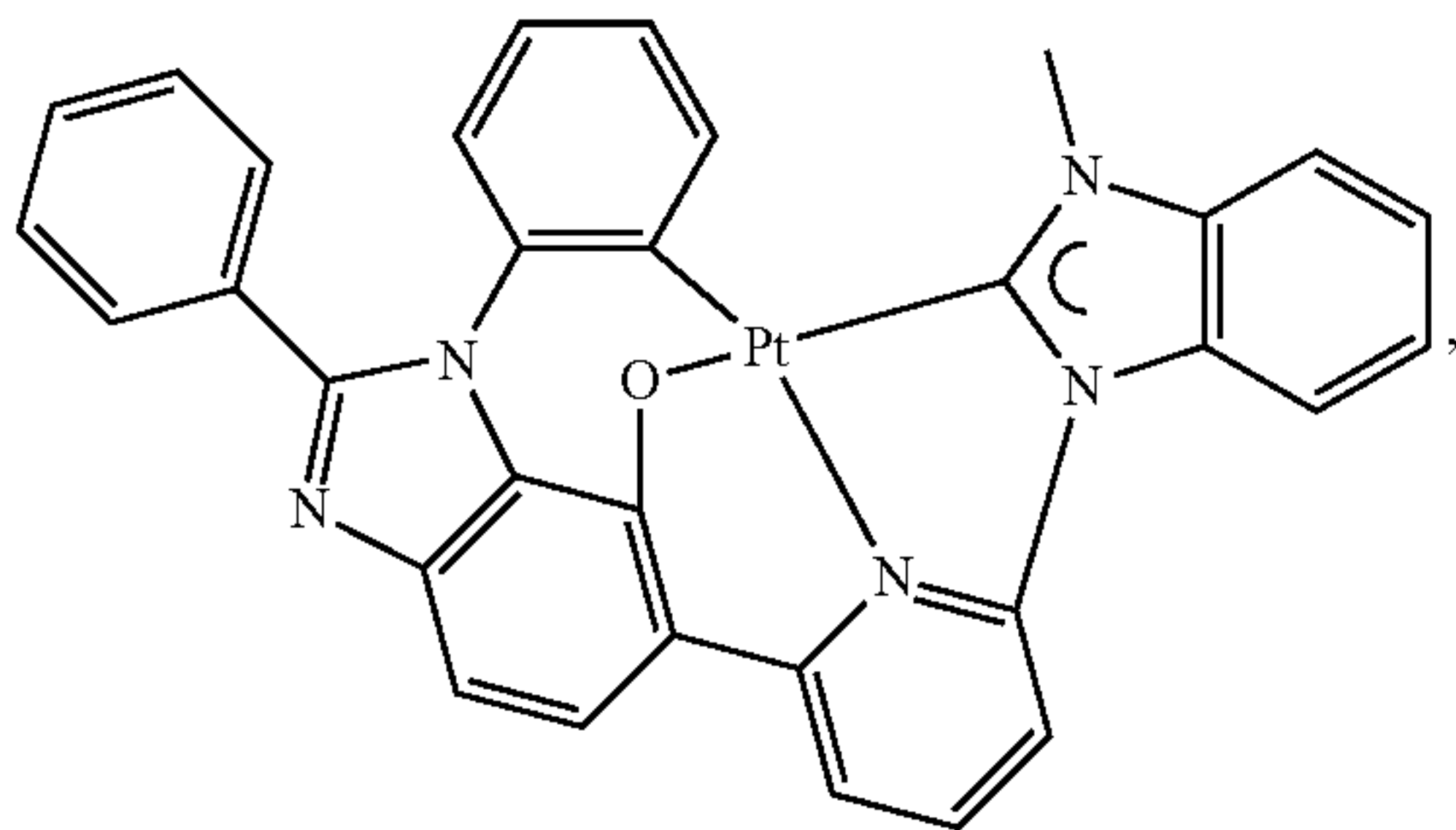
Compound 35
