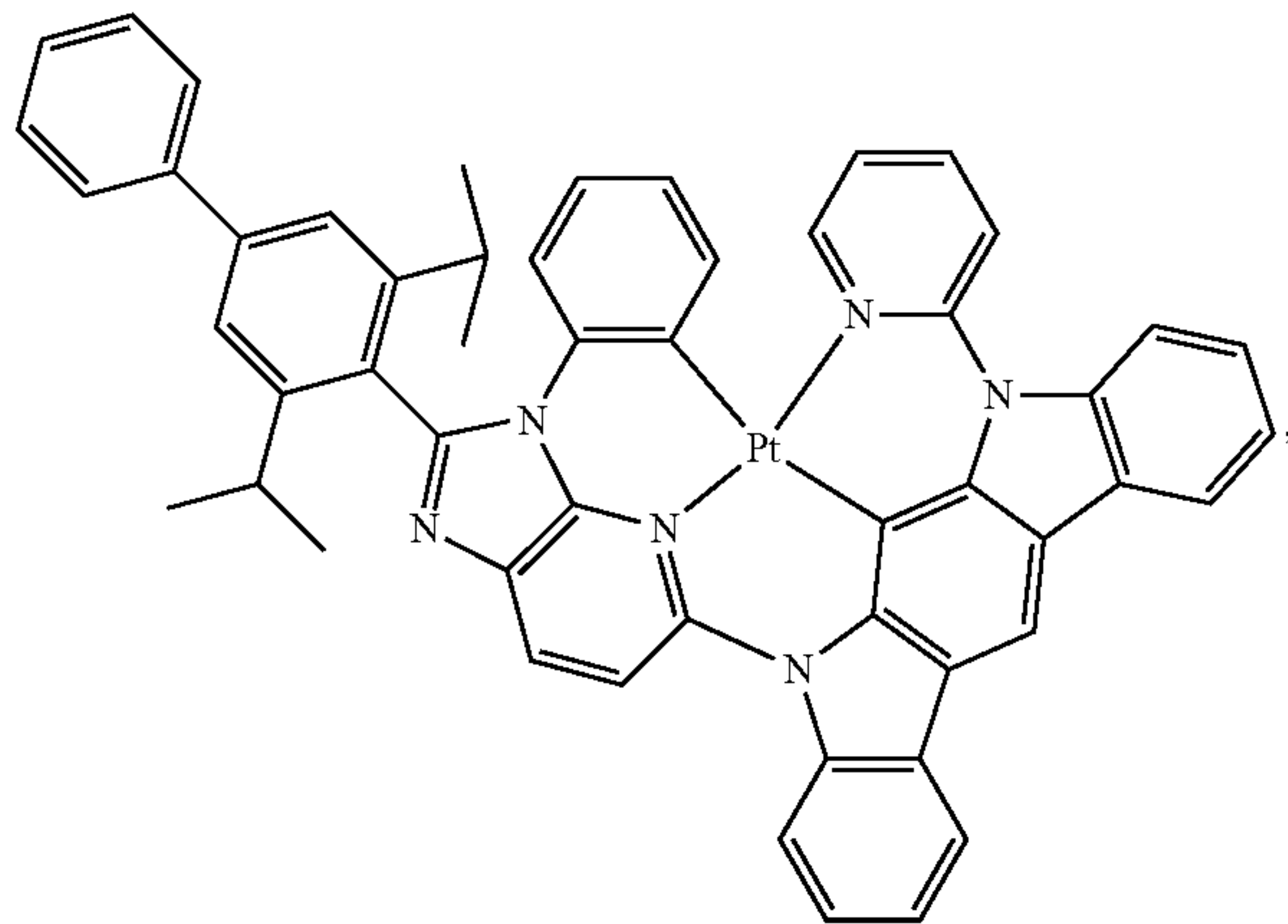
Compound 93
