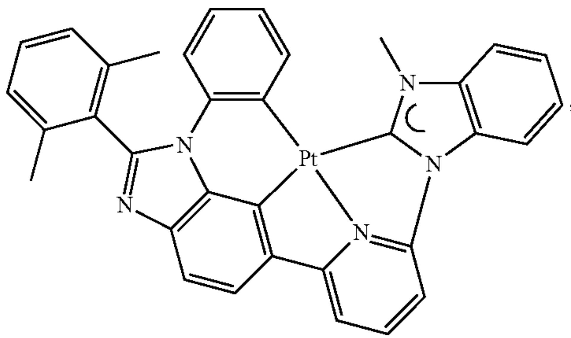
Compound 24
