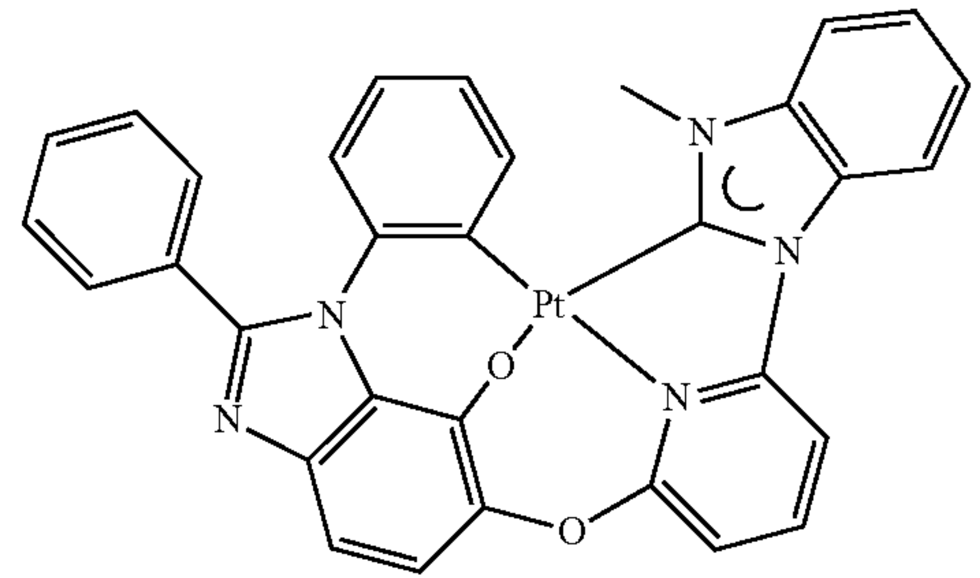
Compound 39
