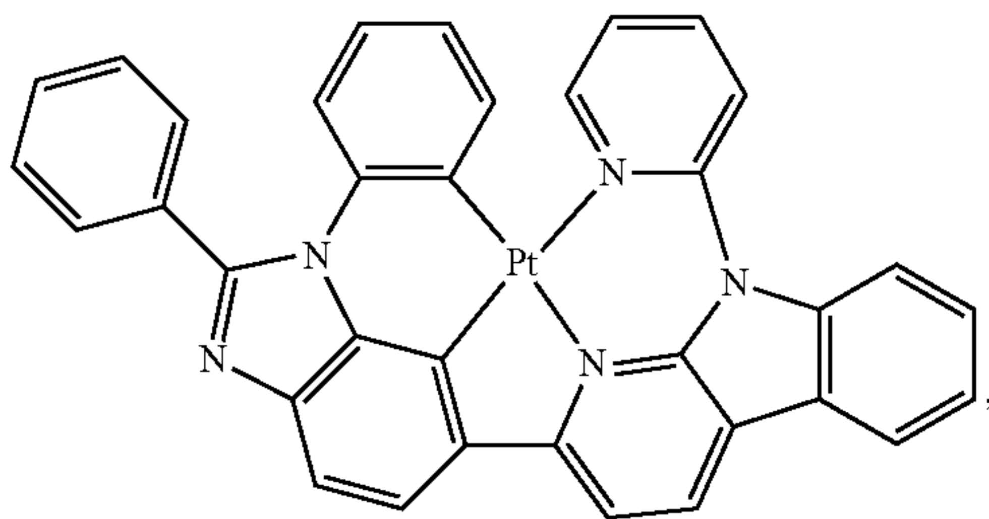
Compound 84
