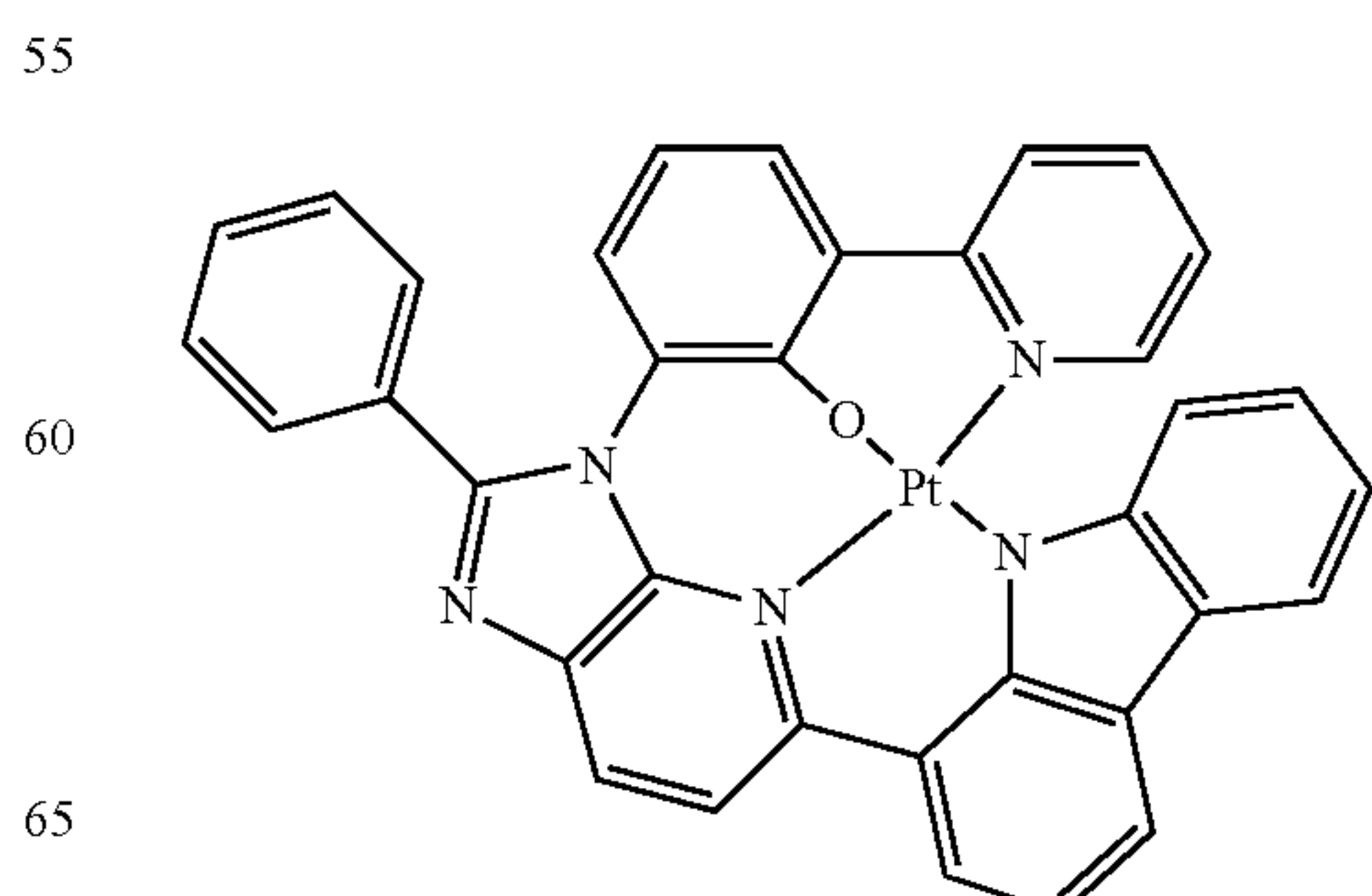
Compound 72
