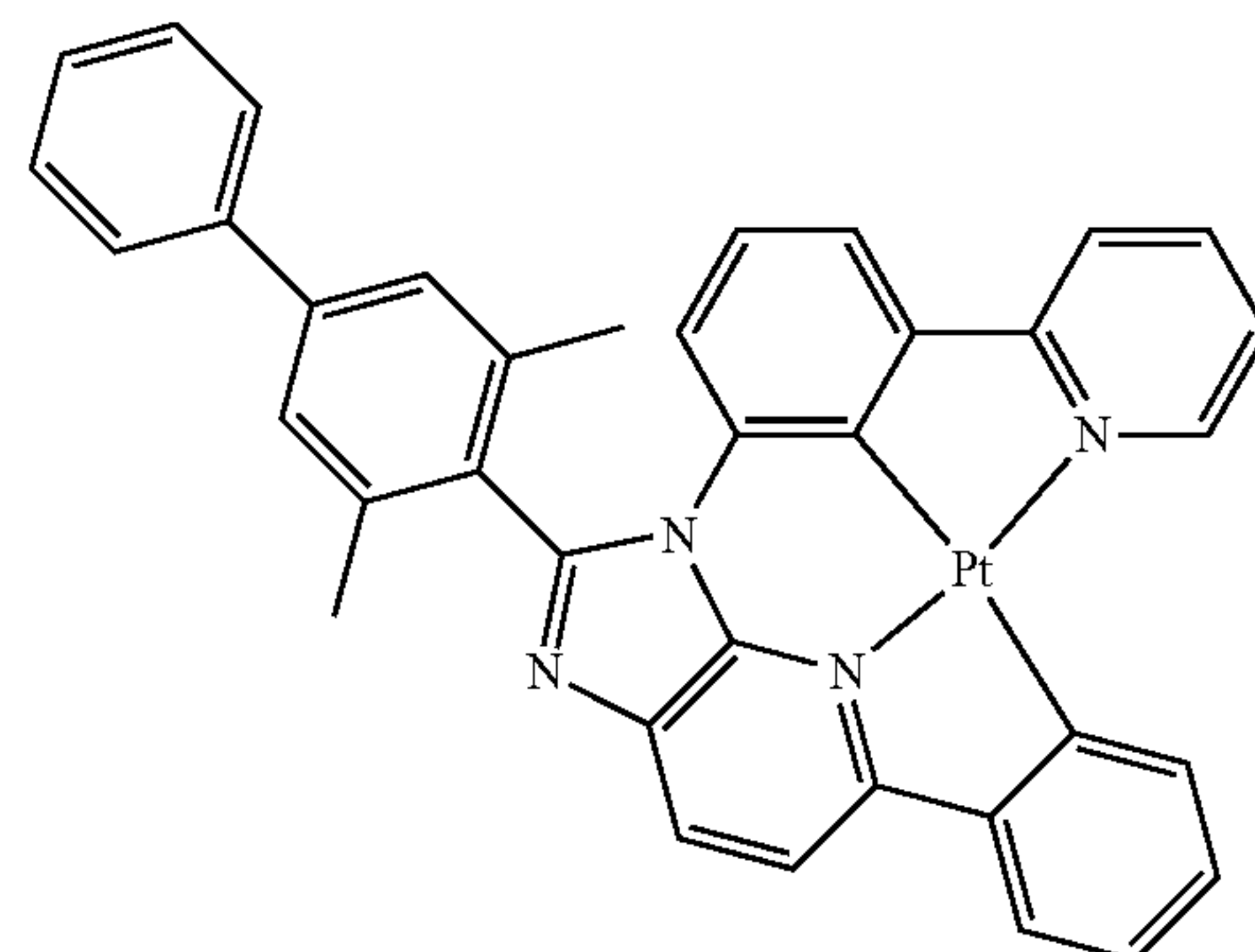
Compound 103
