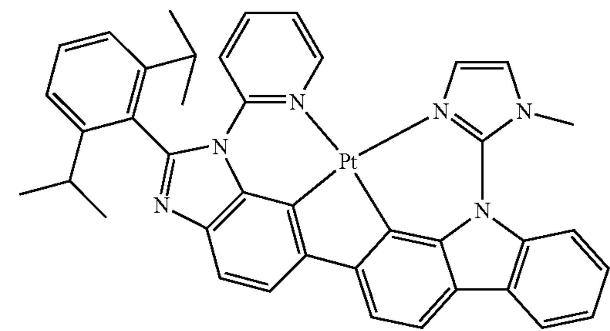
Compound 80
