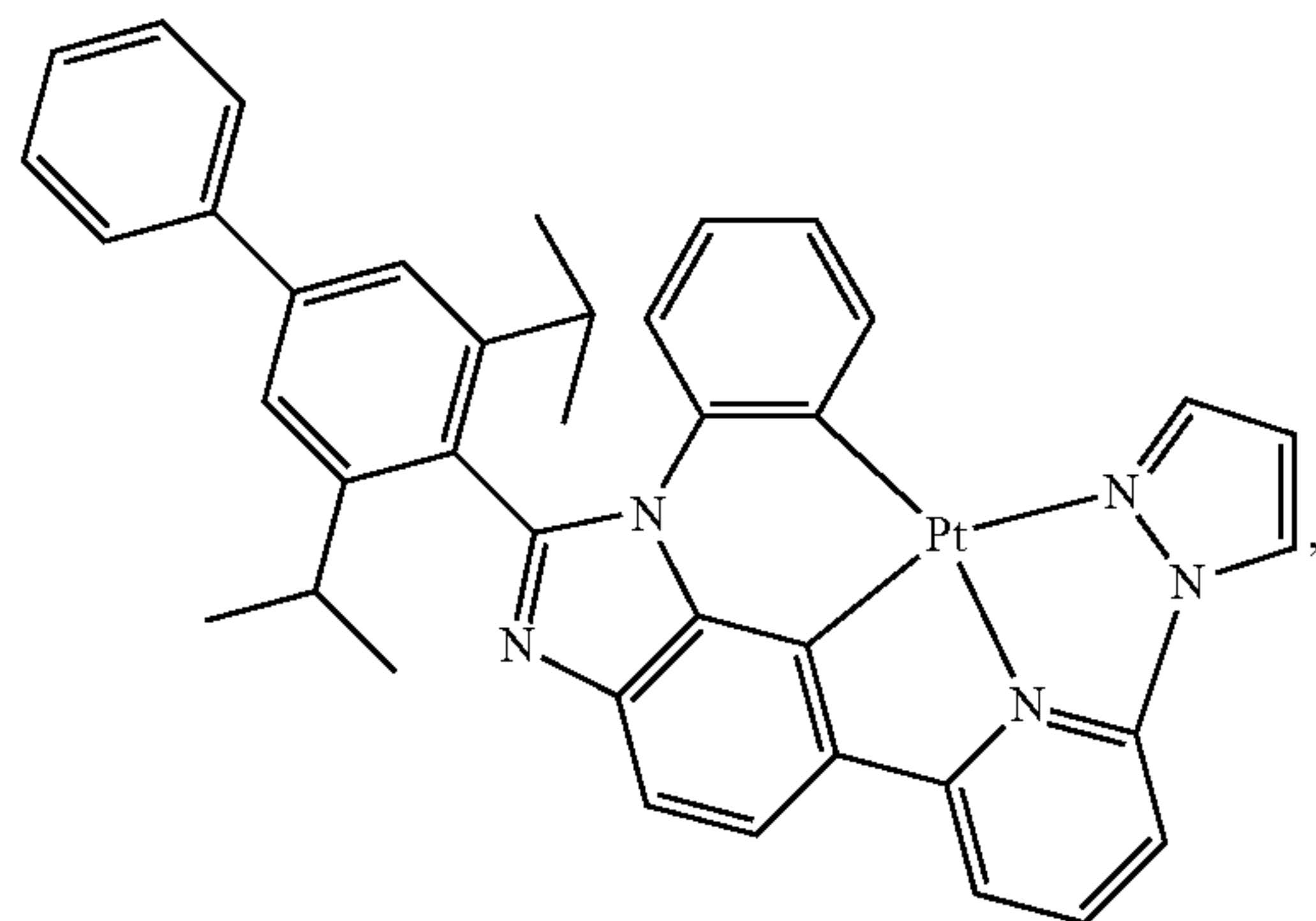
Compound 56
