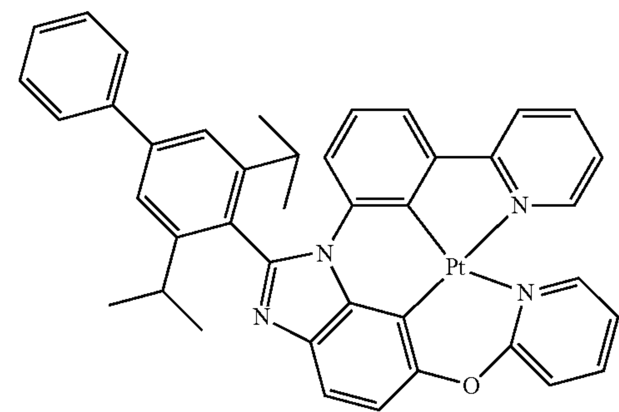
Compound 10
