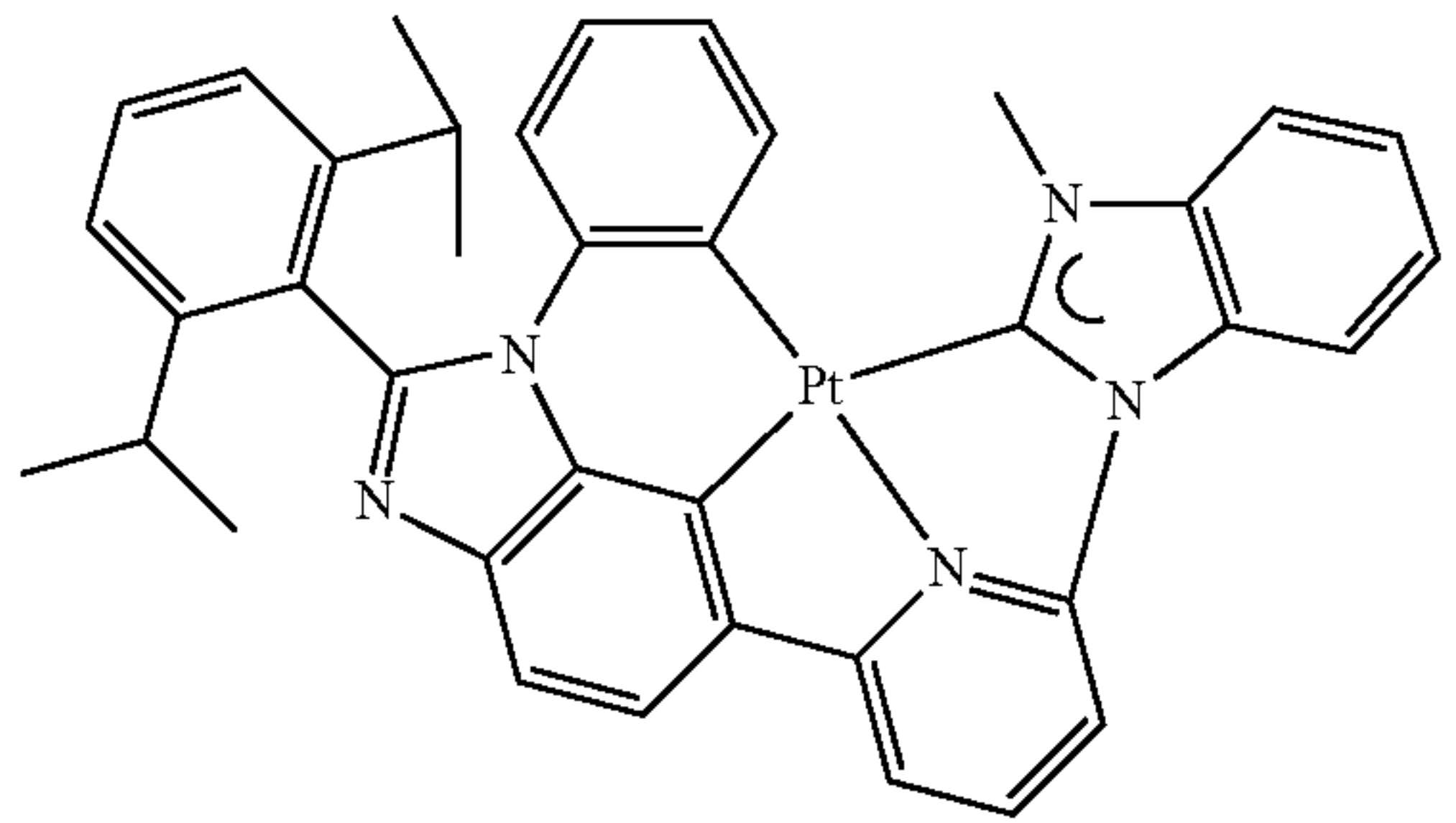
Compound 25
