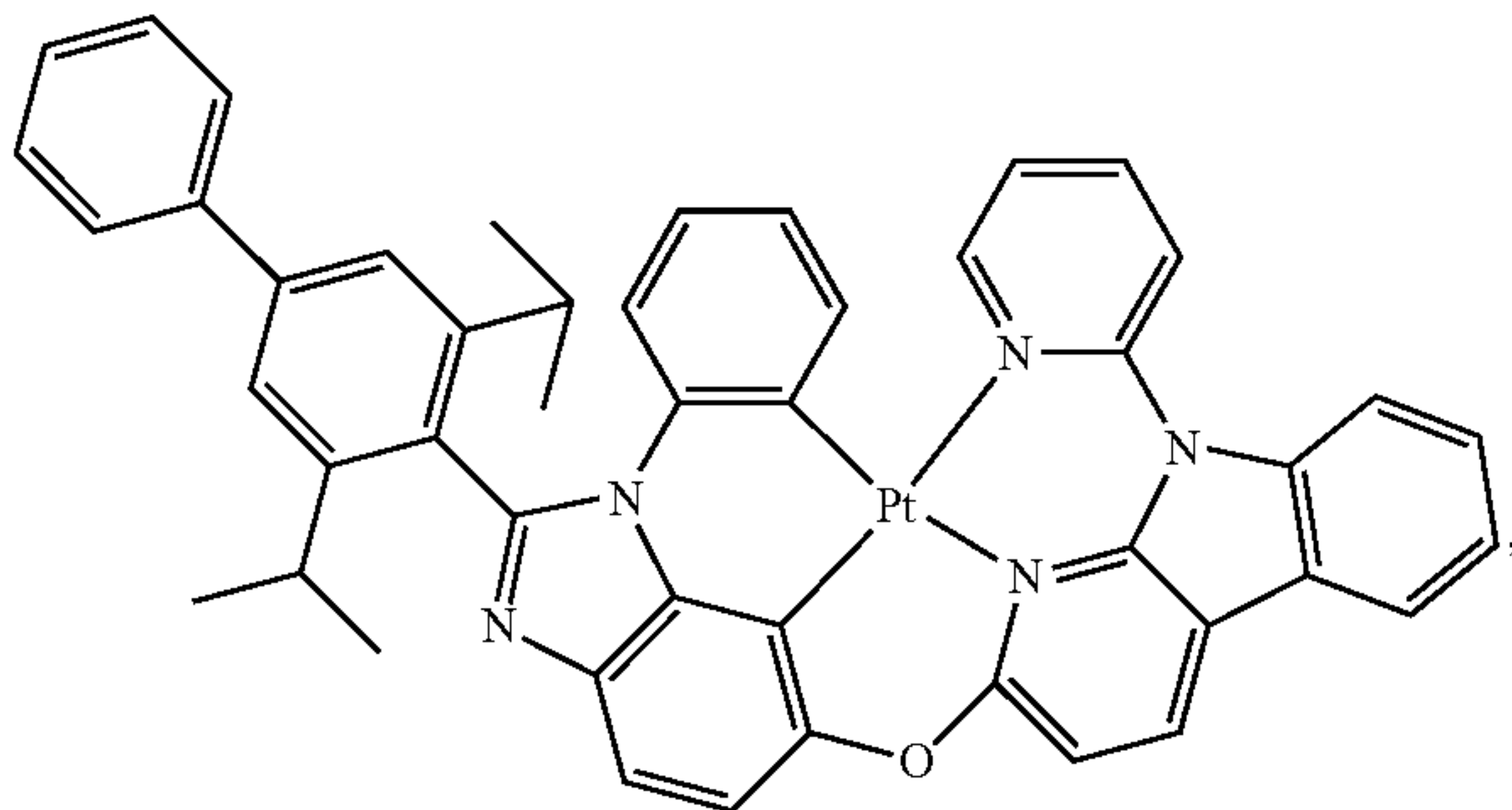
Compound 85
