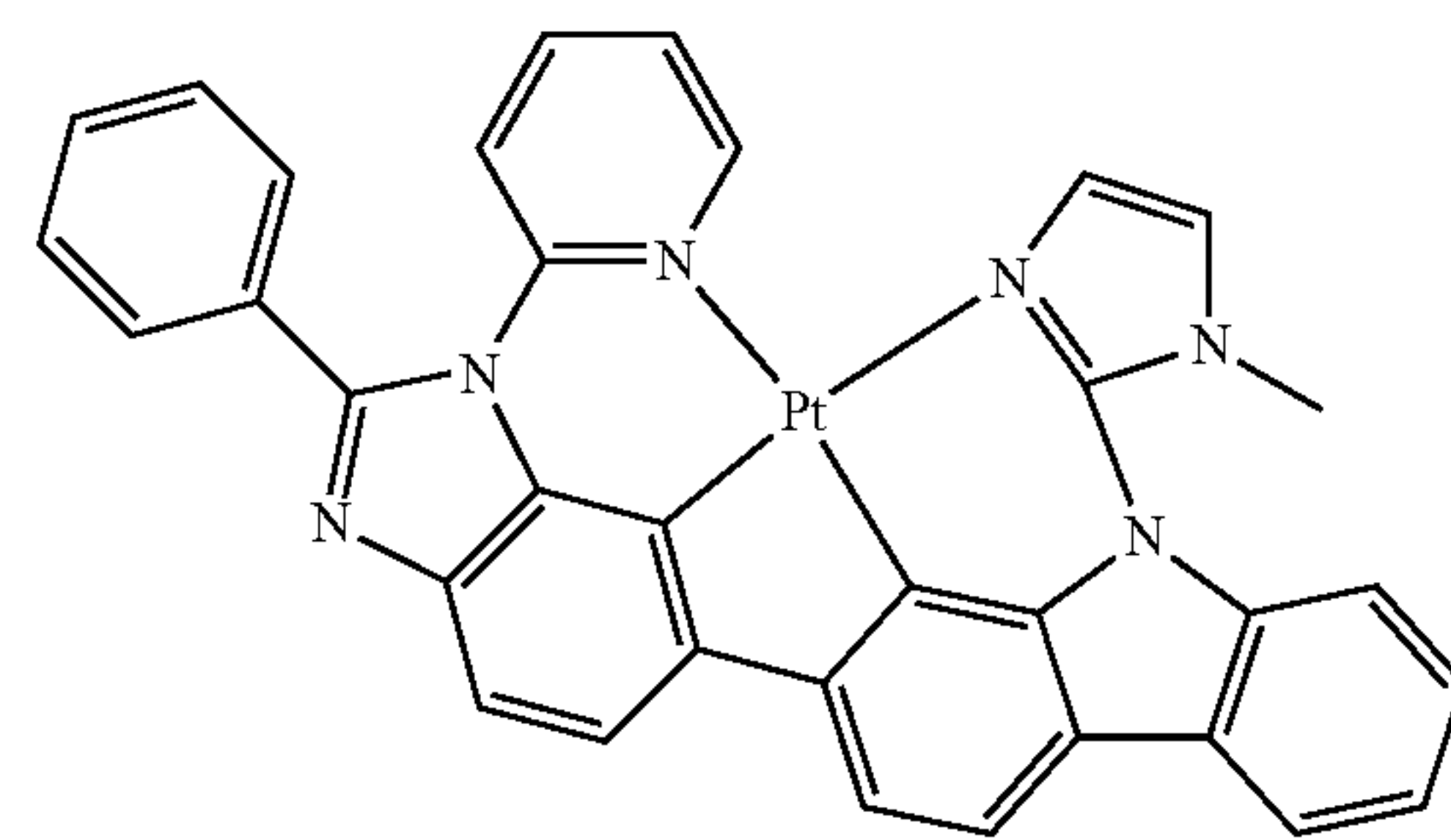
Compound 79
