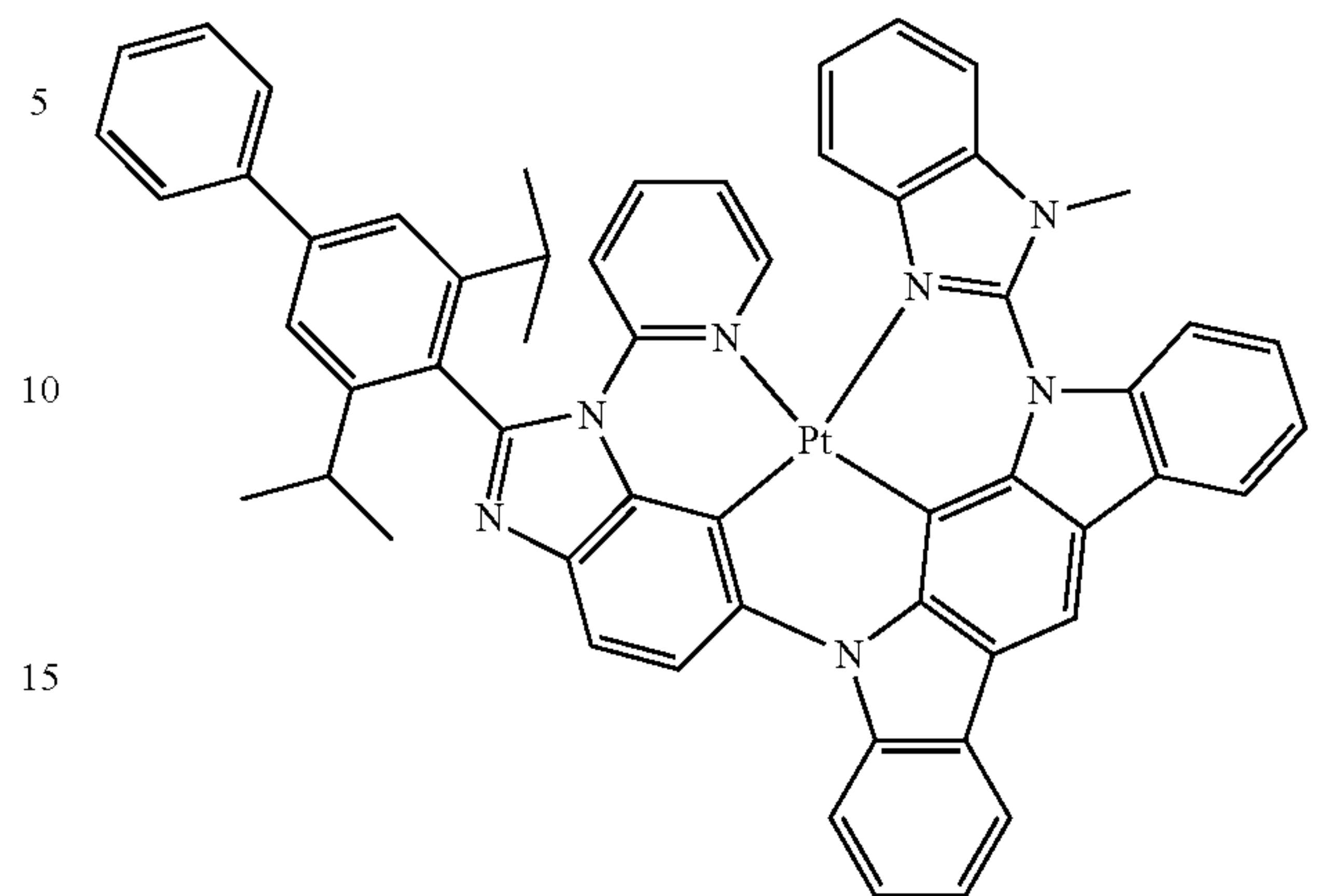
Compound 95
