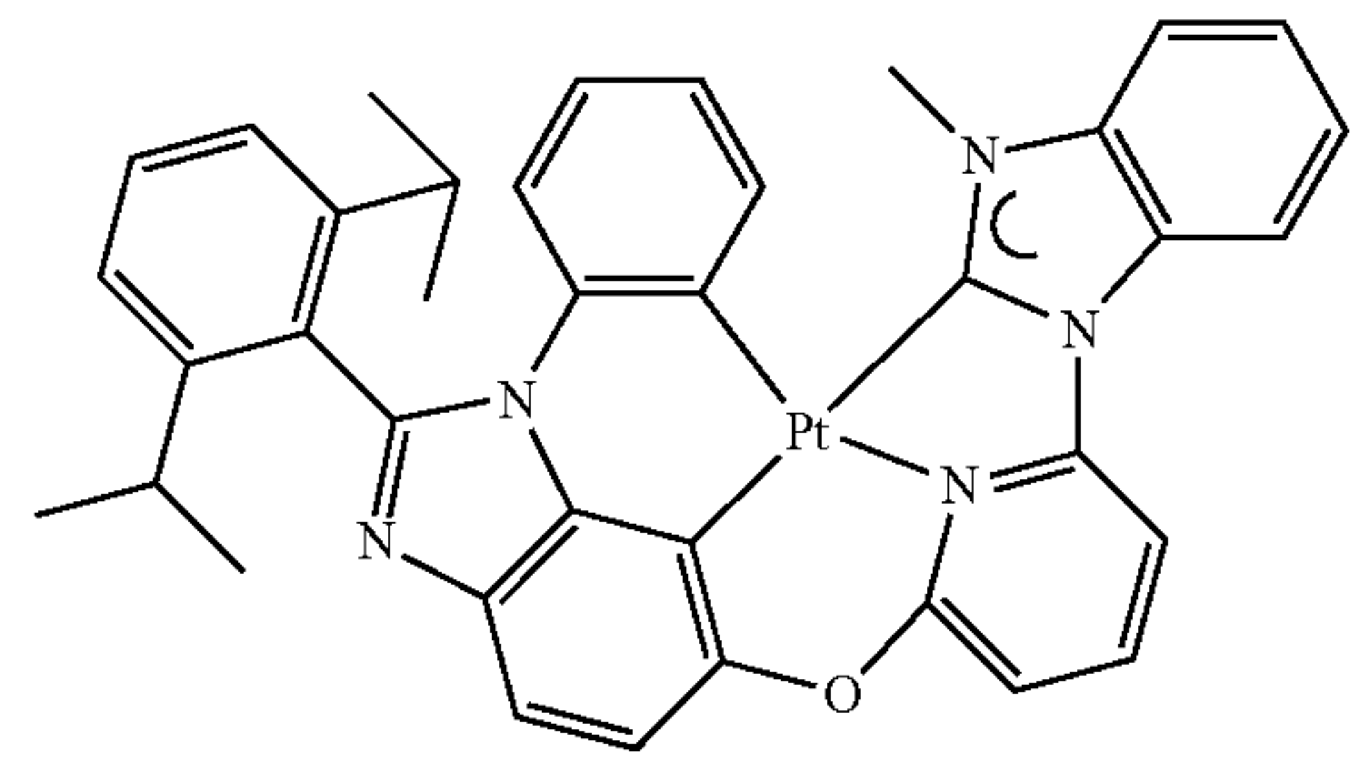
Compound 30
