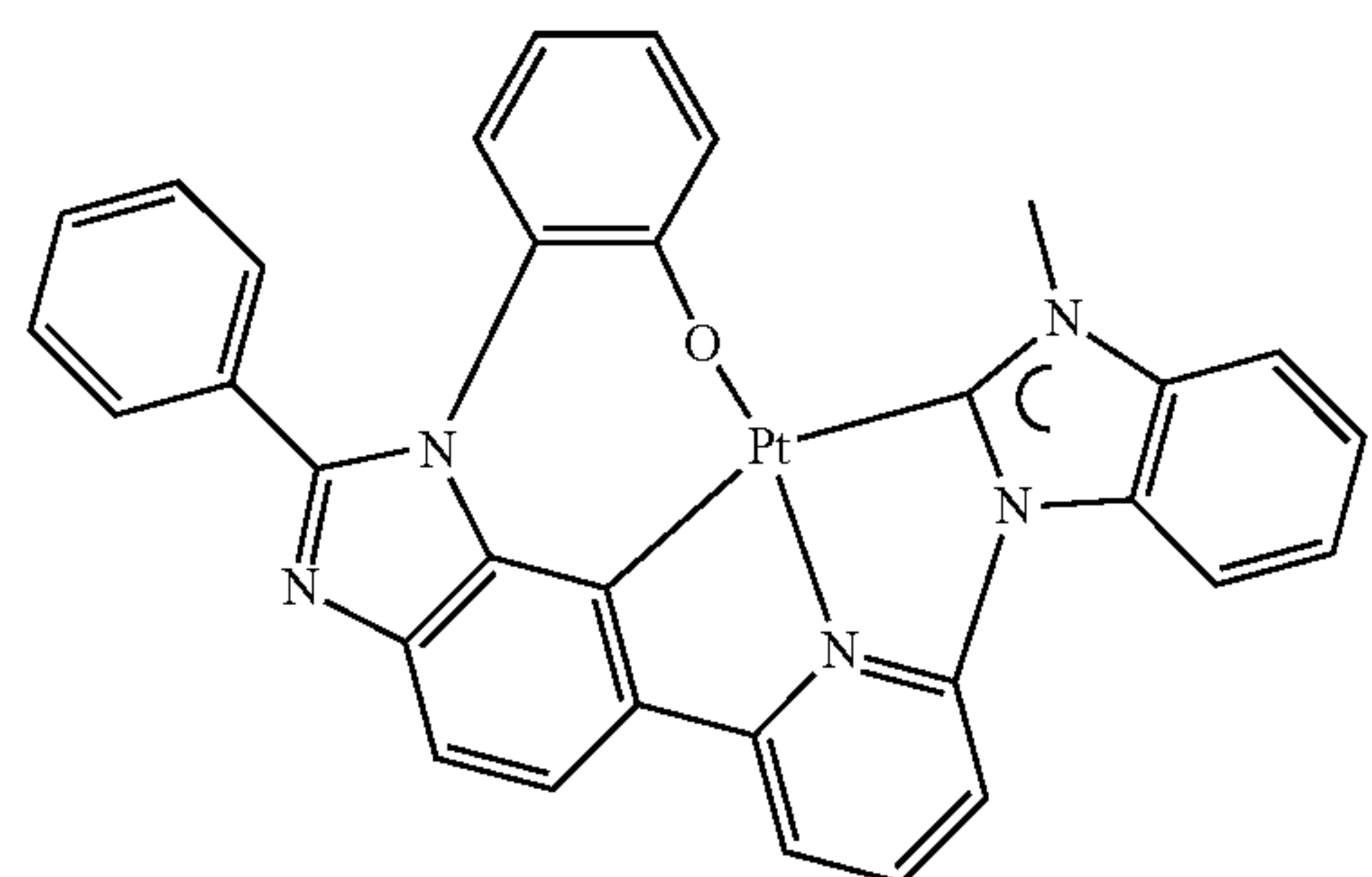
Compound 32
