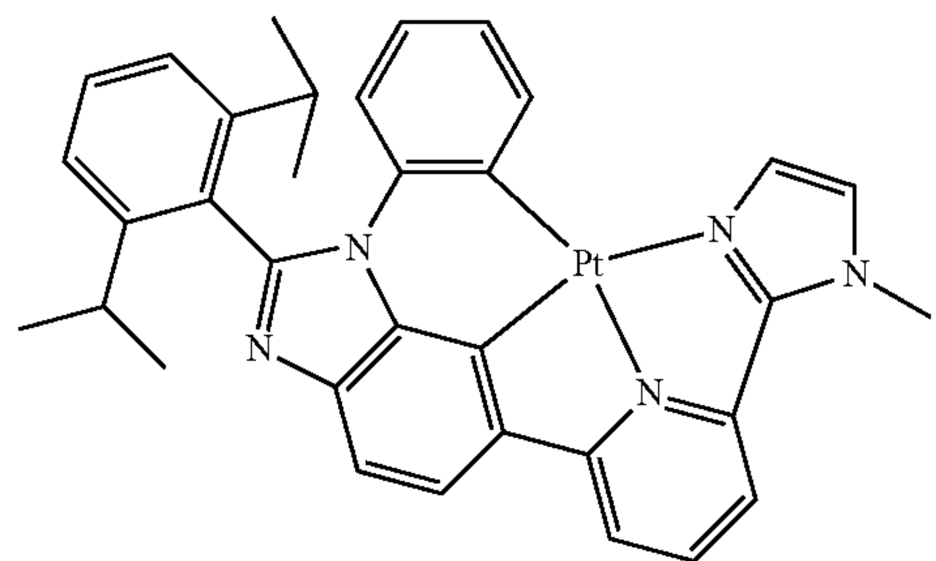
Compound 42
