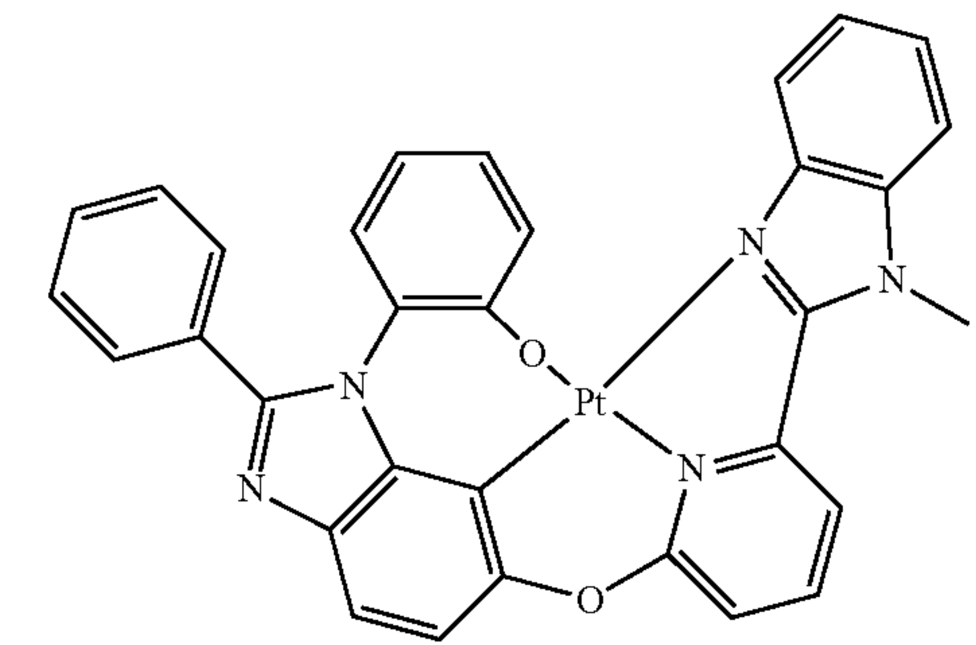
Compound 50
