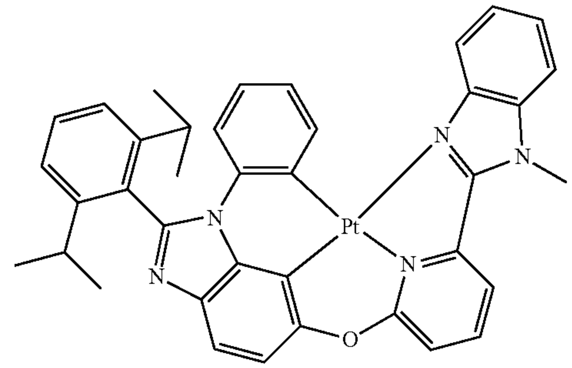
Compound 48
