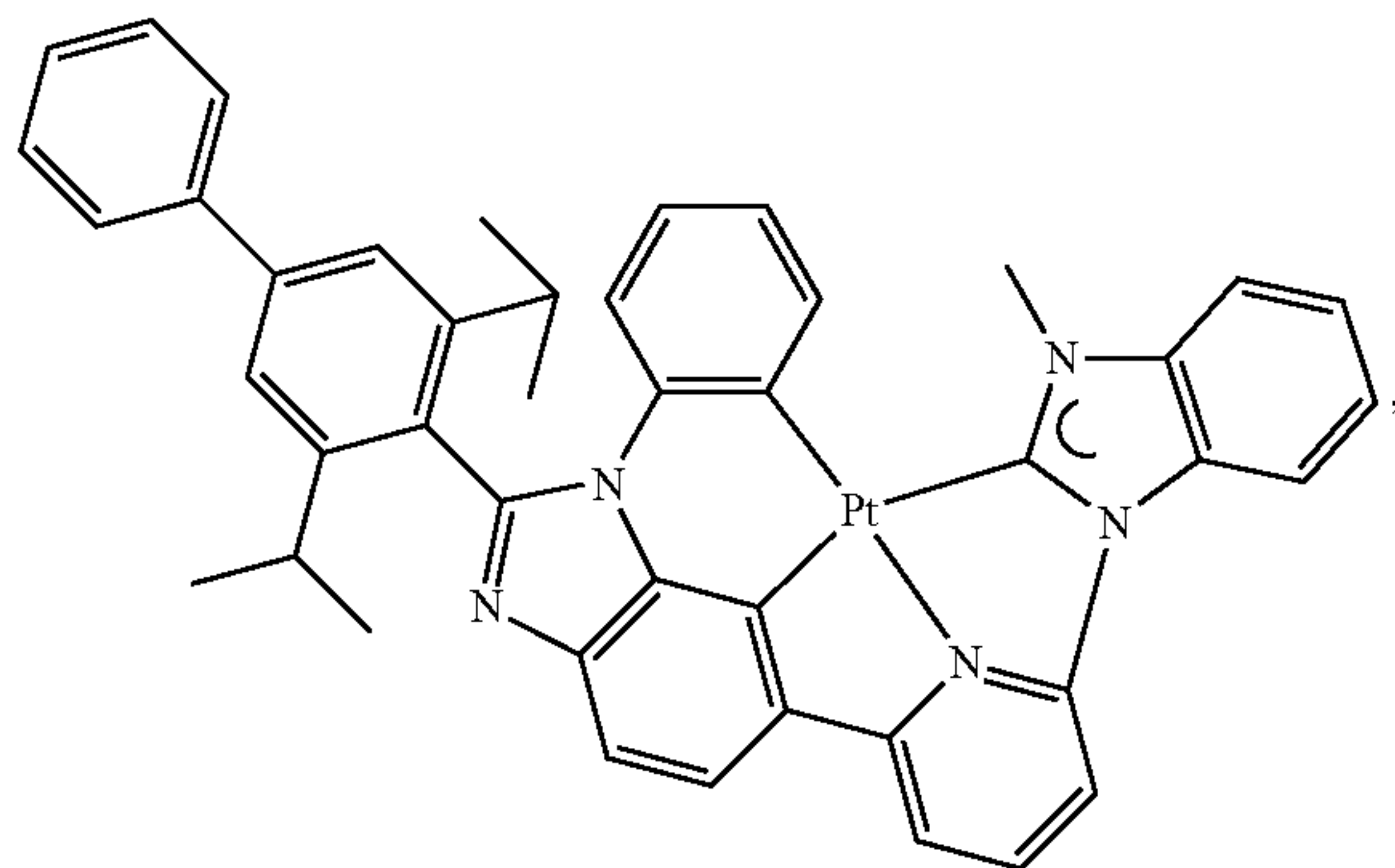
Compound 27
