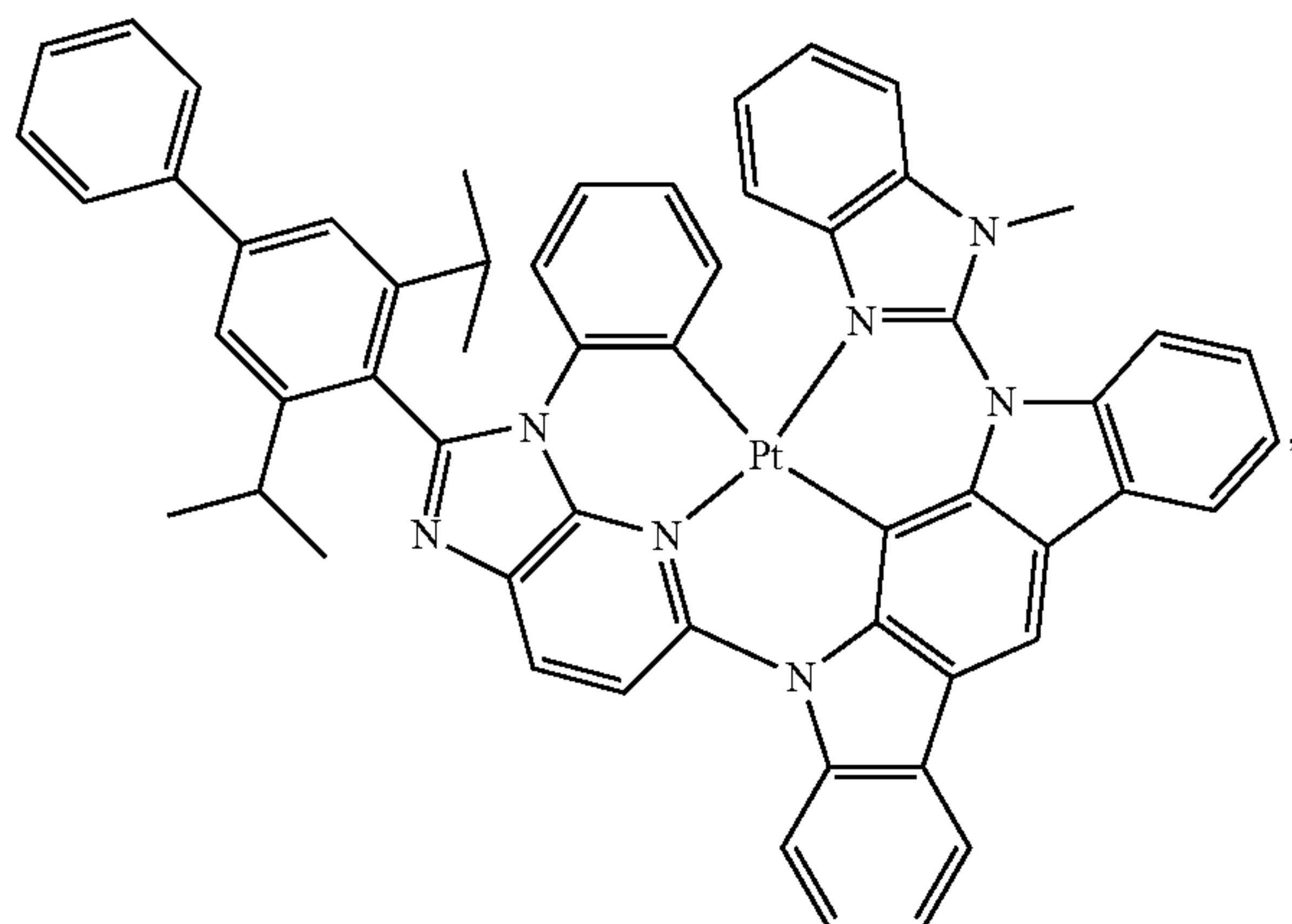
Compound 99
