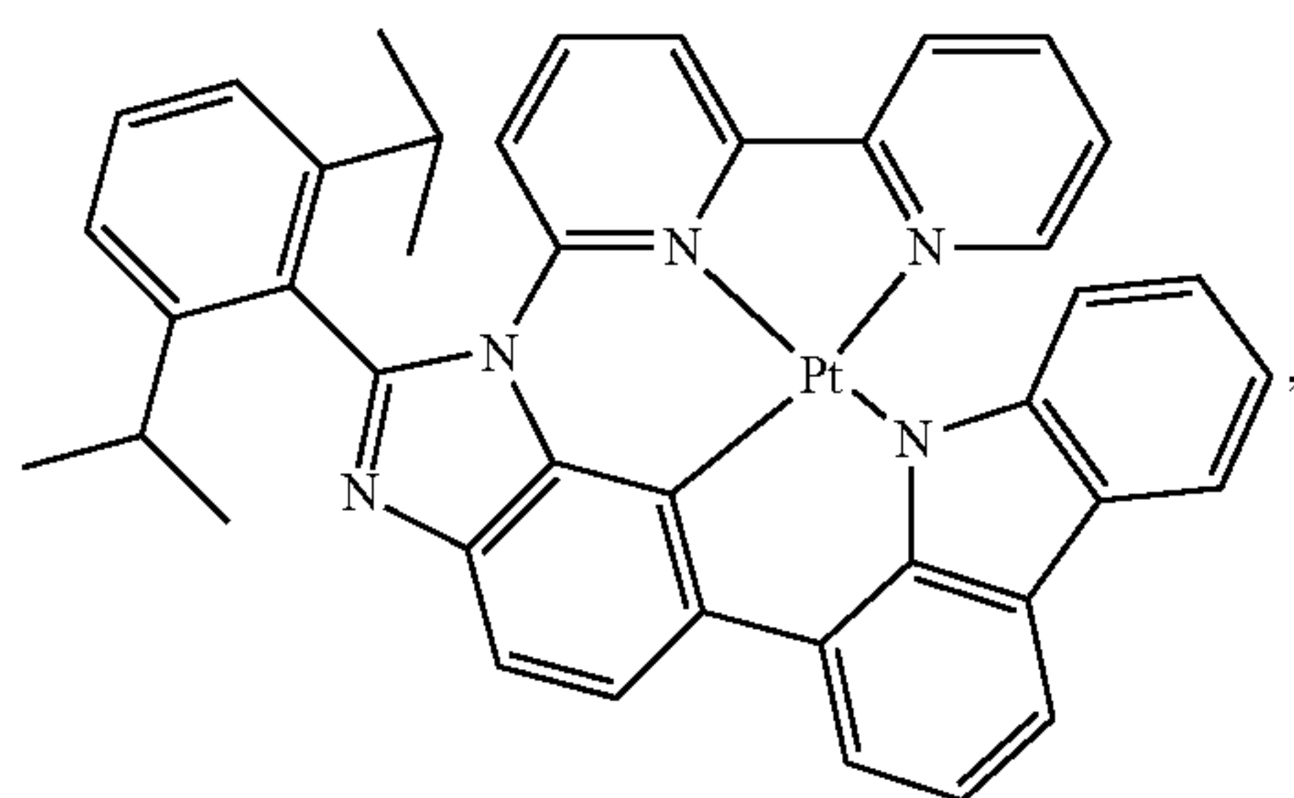
Compound 66
