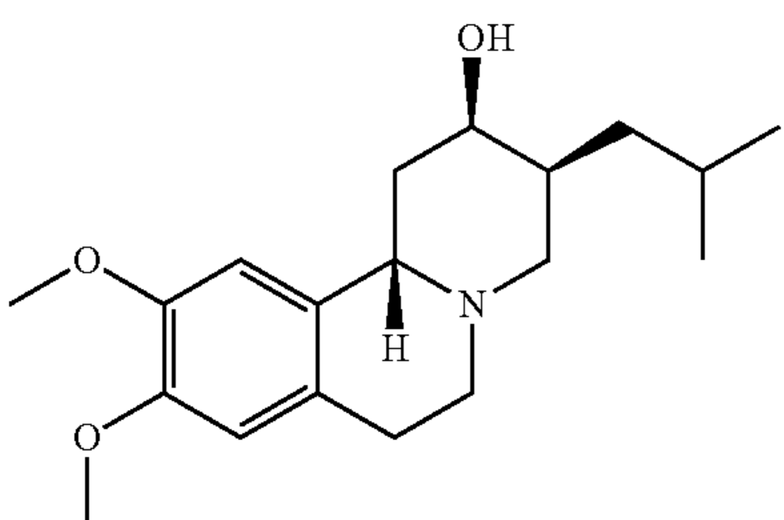
(-) -beta-dihydrotrabenzazine
