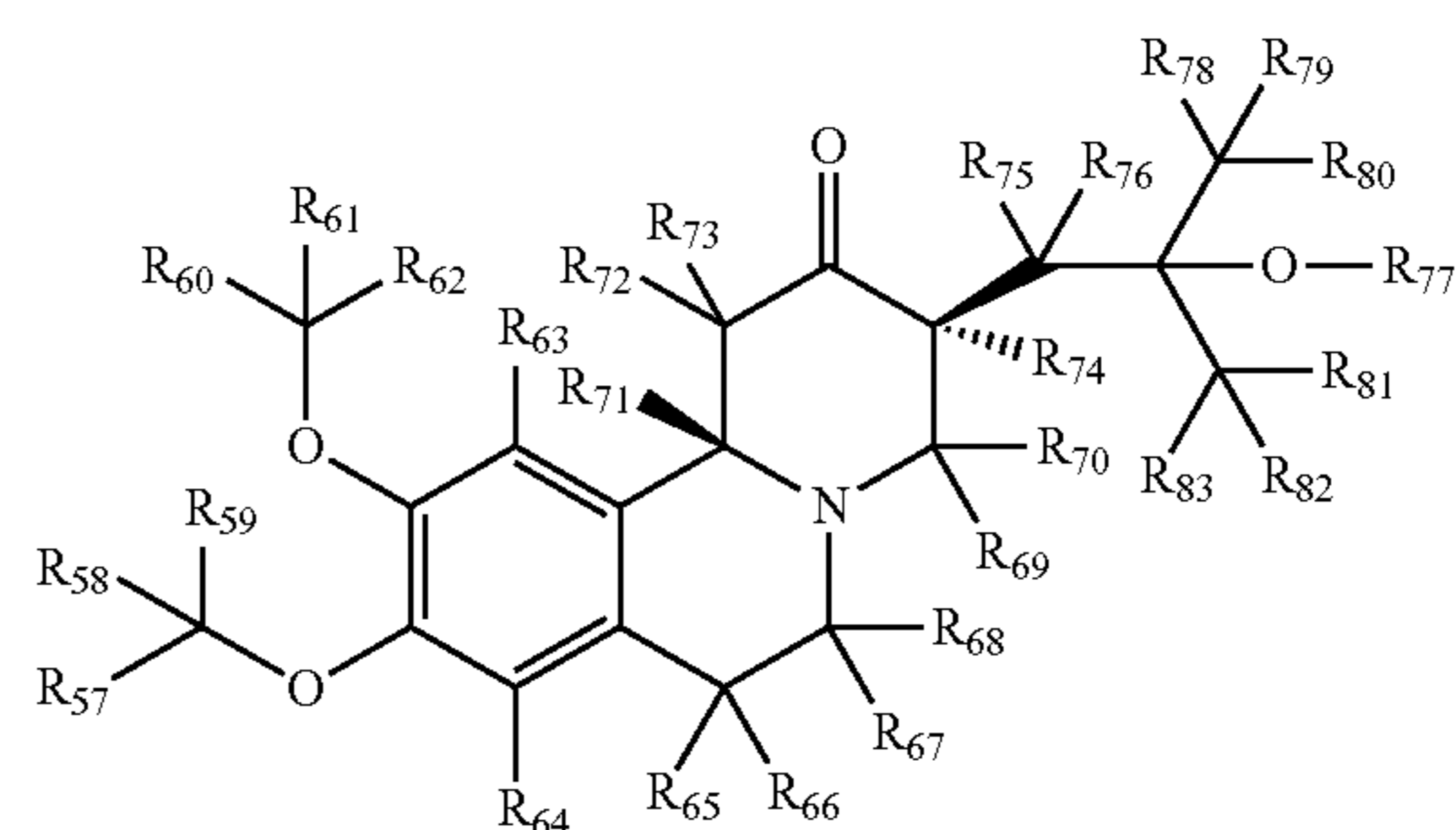
(3S, 11bS)-enantiomer
