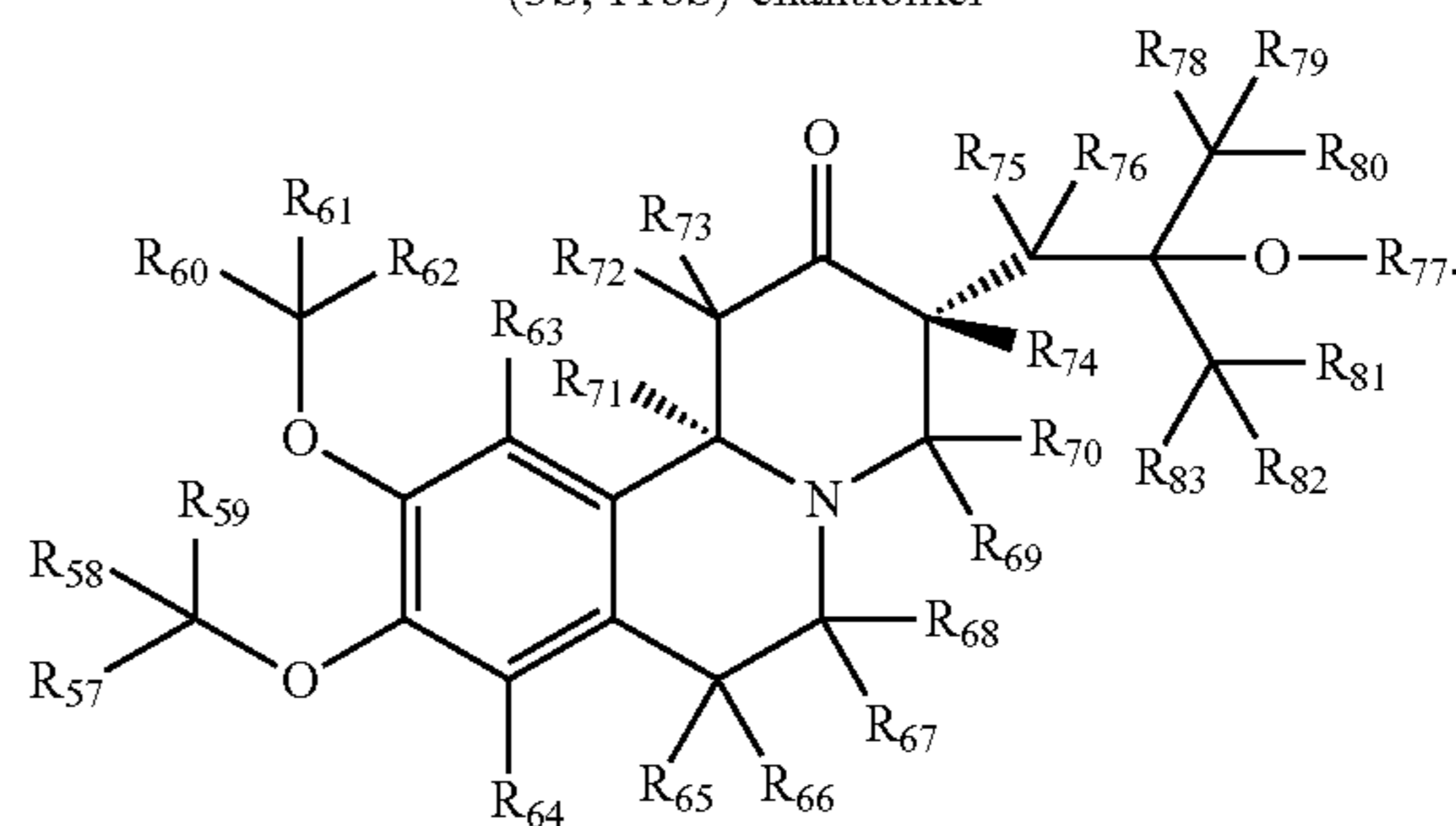
(3R, 11bR)-enantiomer
