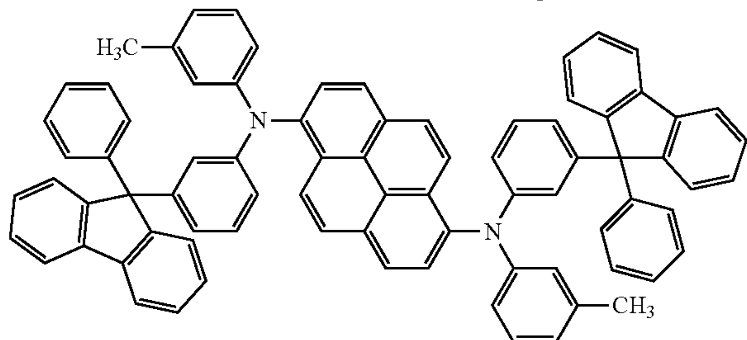
1,6mMemFLPAPrn
