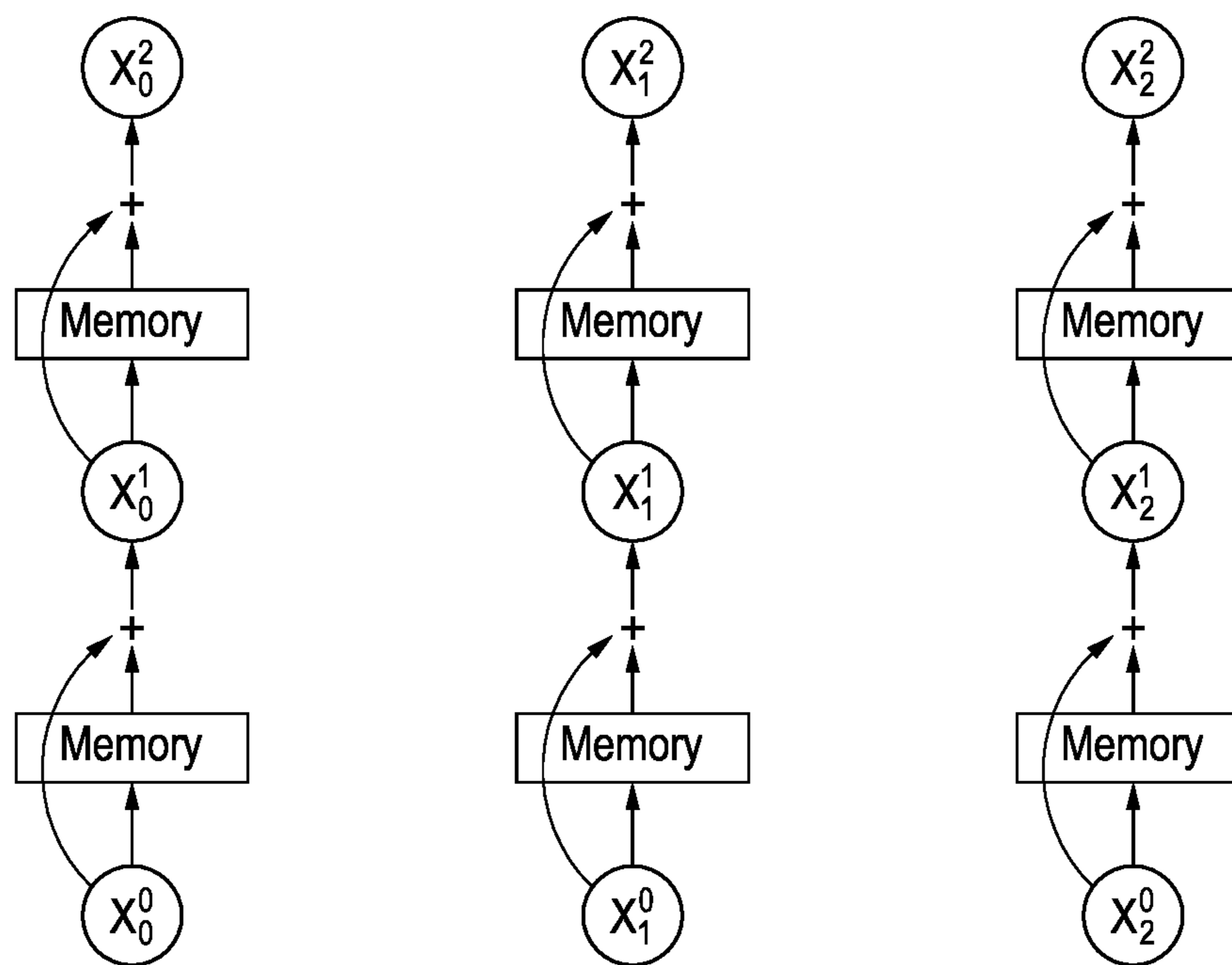
Neural Network
