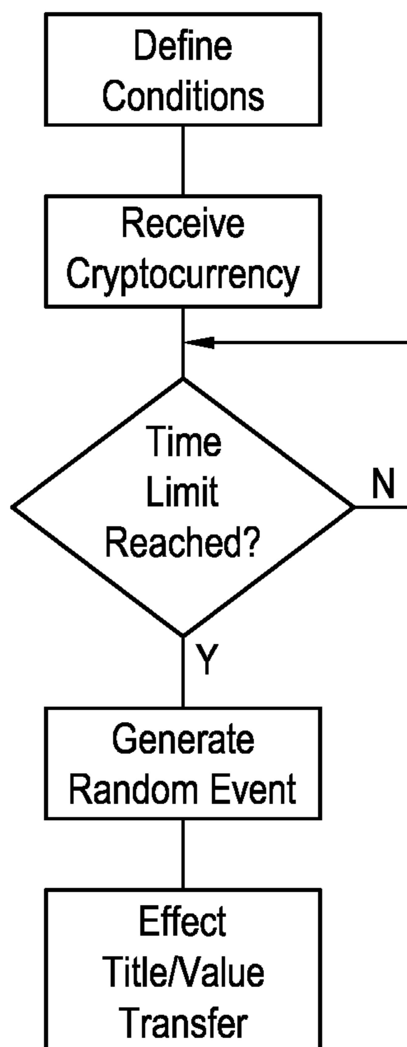
Flowchart for Crypto Currency Lottery
