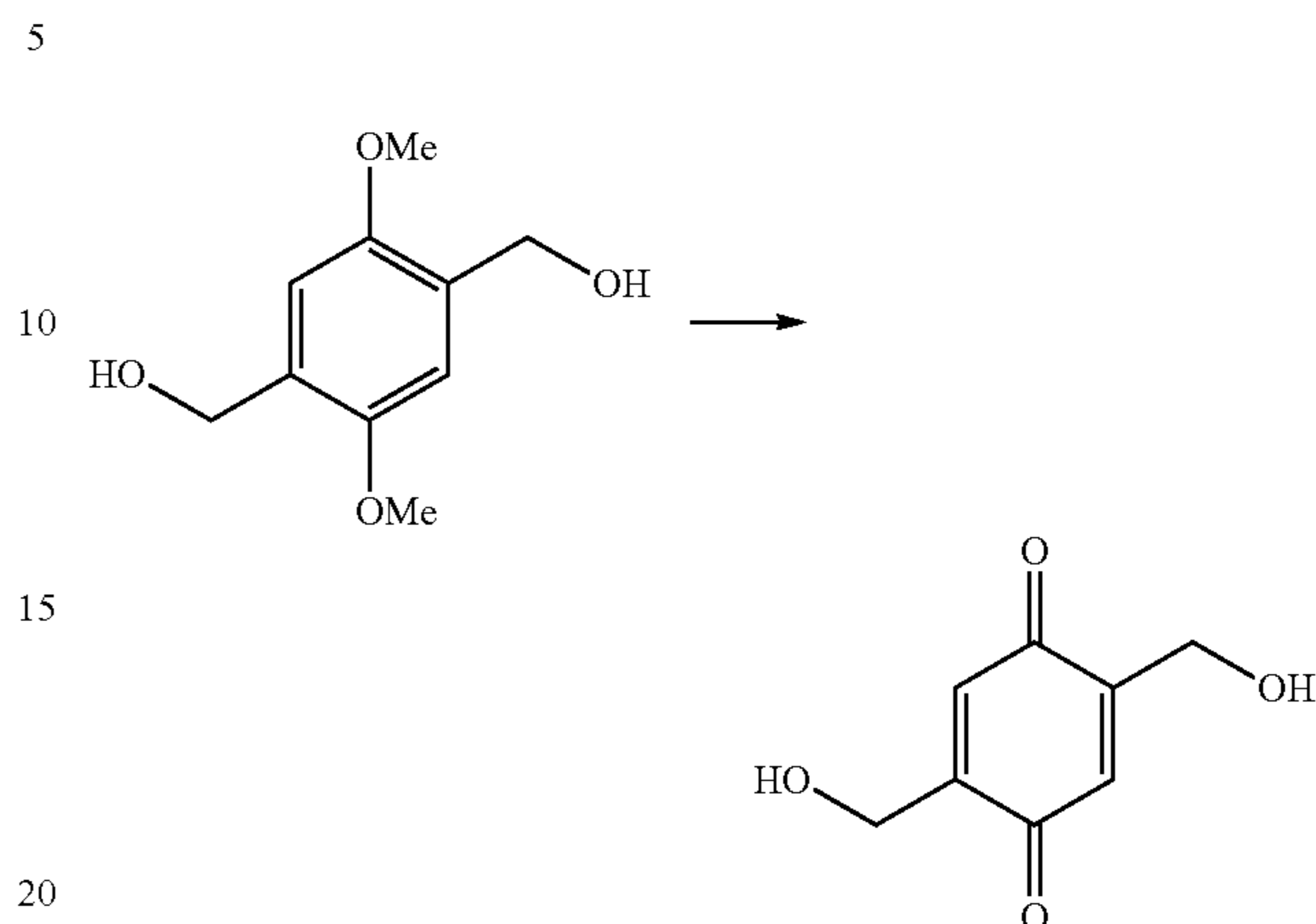
2,5-dimethoxymethyl-1,4-benzoquinone
