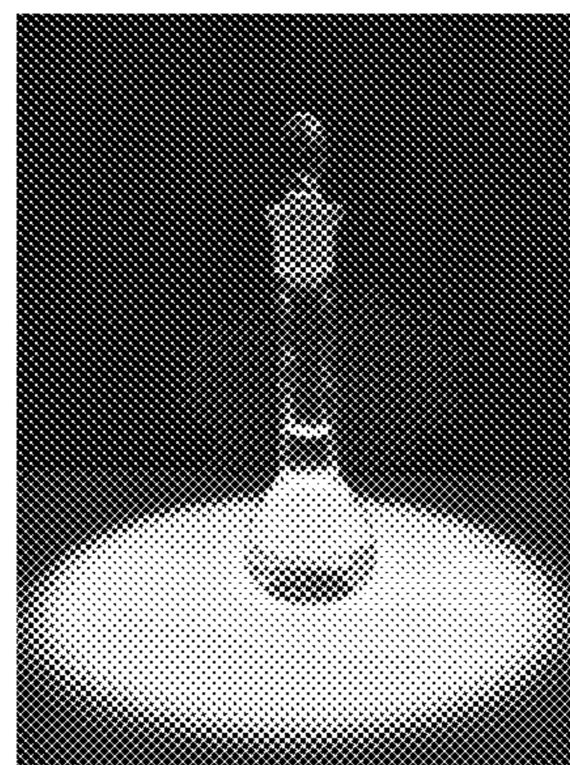
ARGININE IN WATER
