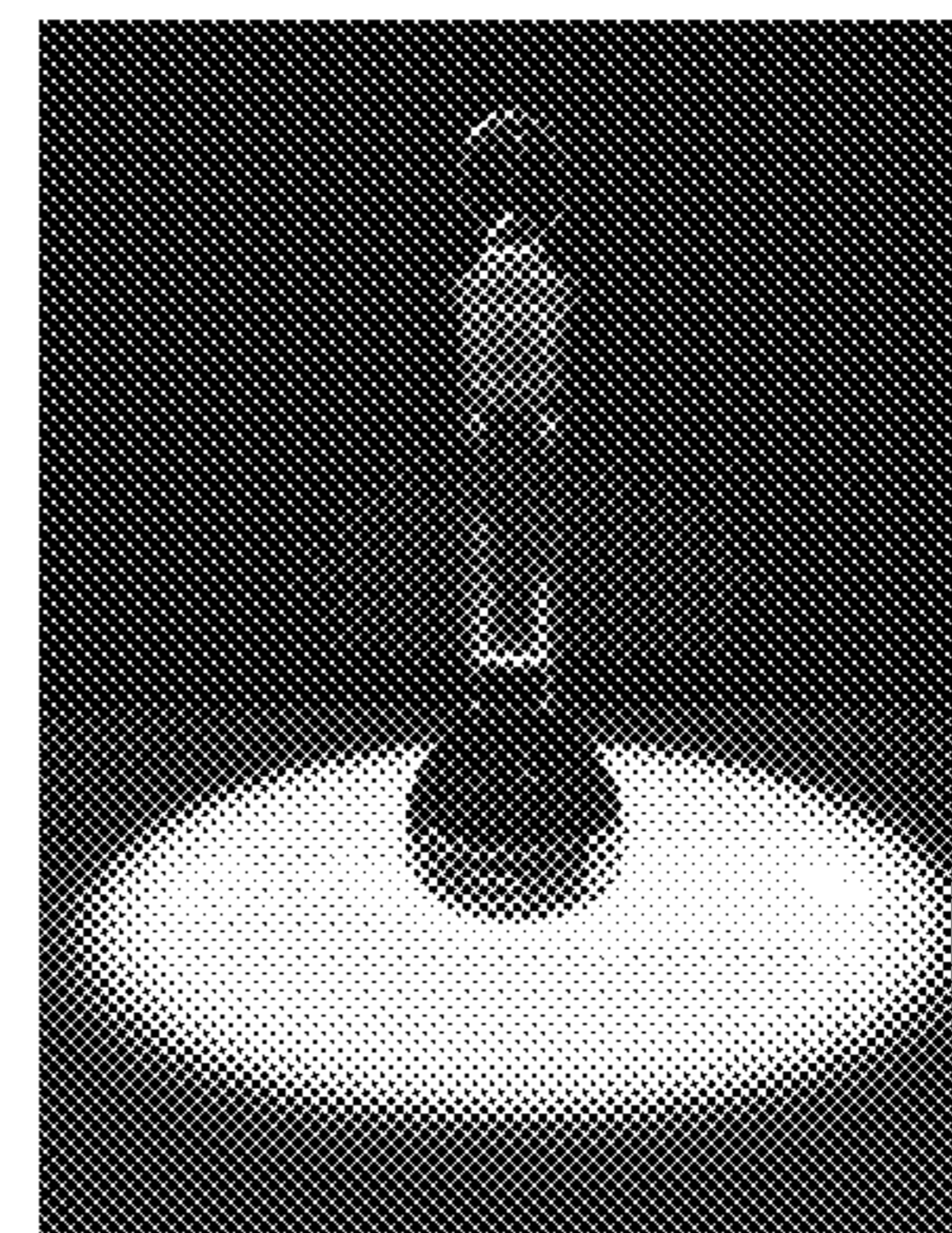
ARGININE + NINHYDRIN + HEAT
