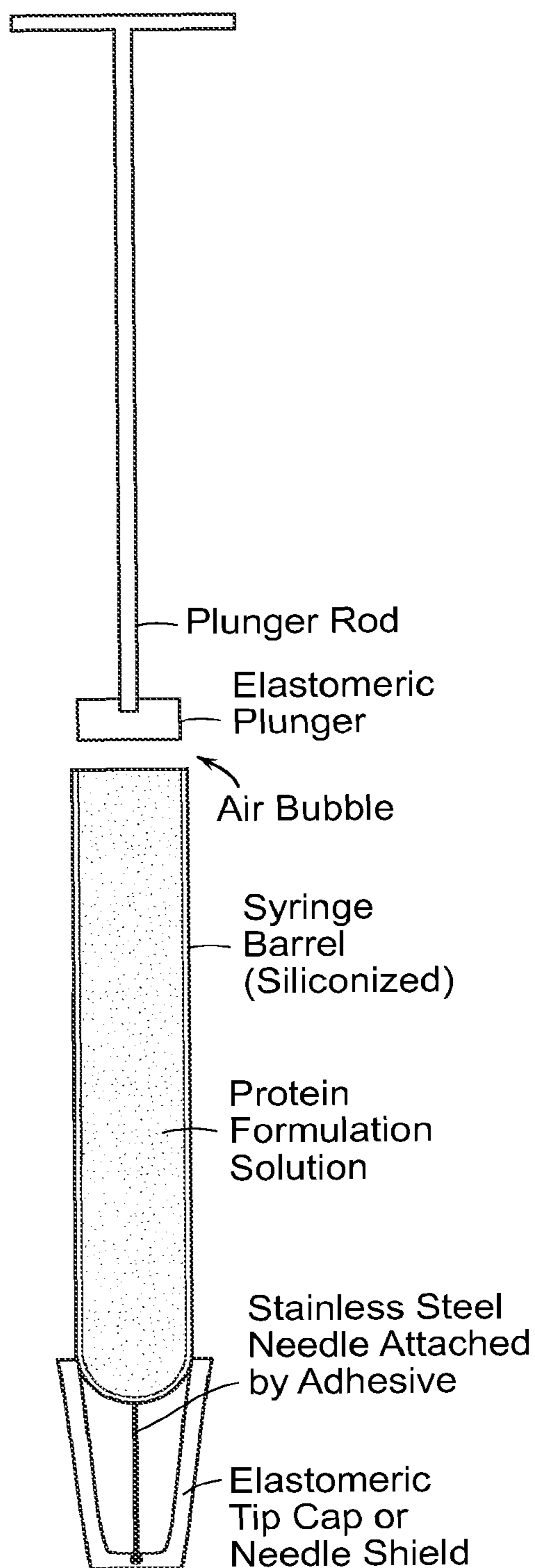
Components of a Protein Product in a Pre-filled Syringe
