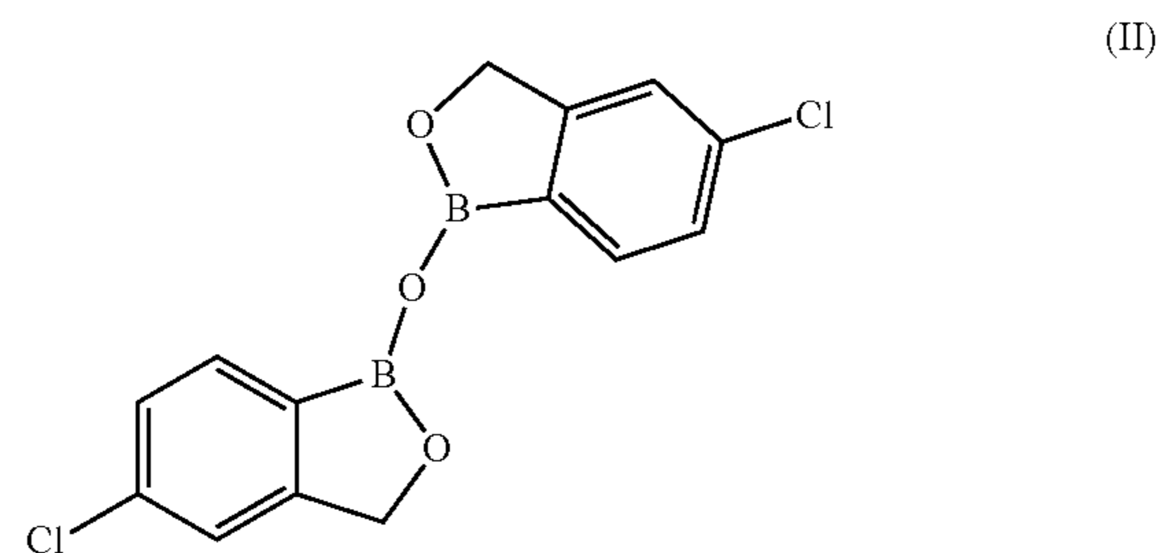
1,1'-oxybis(5-chloro-1,3-dihydrobenzo[c][1,2]oxaborole).
