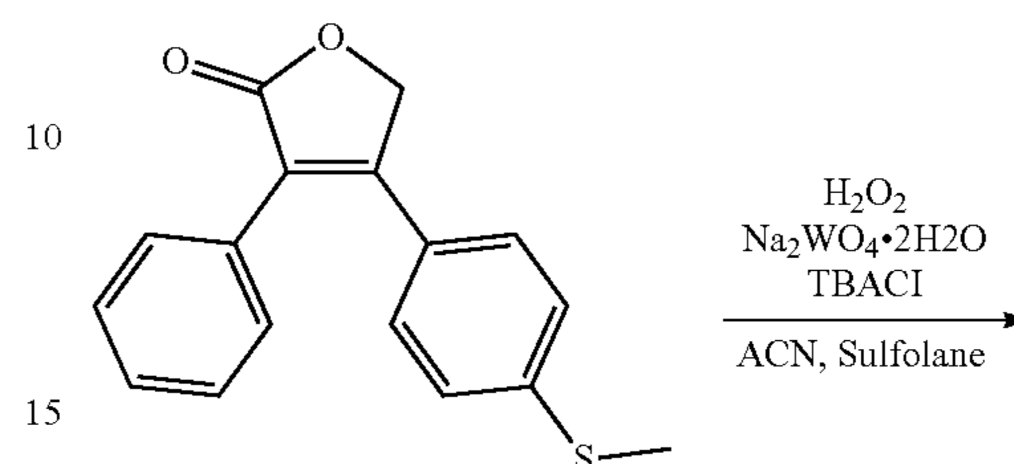
Stage 3 RXB-Furanone C 17 H 14 O 2 S MW = 282.36
