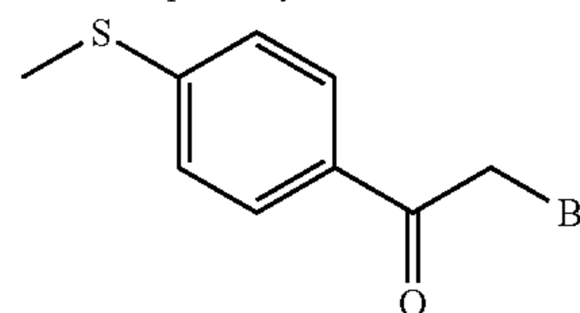
2-bromoacetophenone
