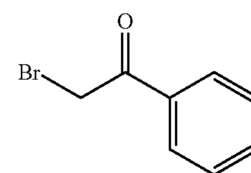
phenacyl bromide
