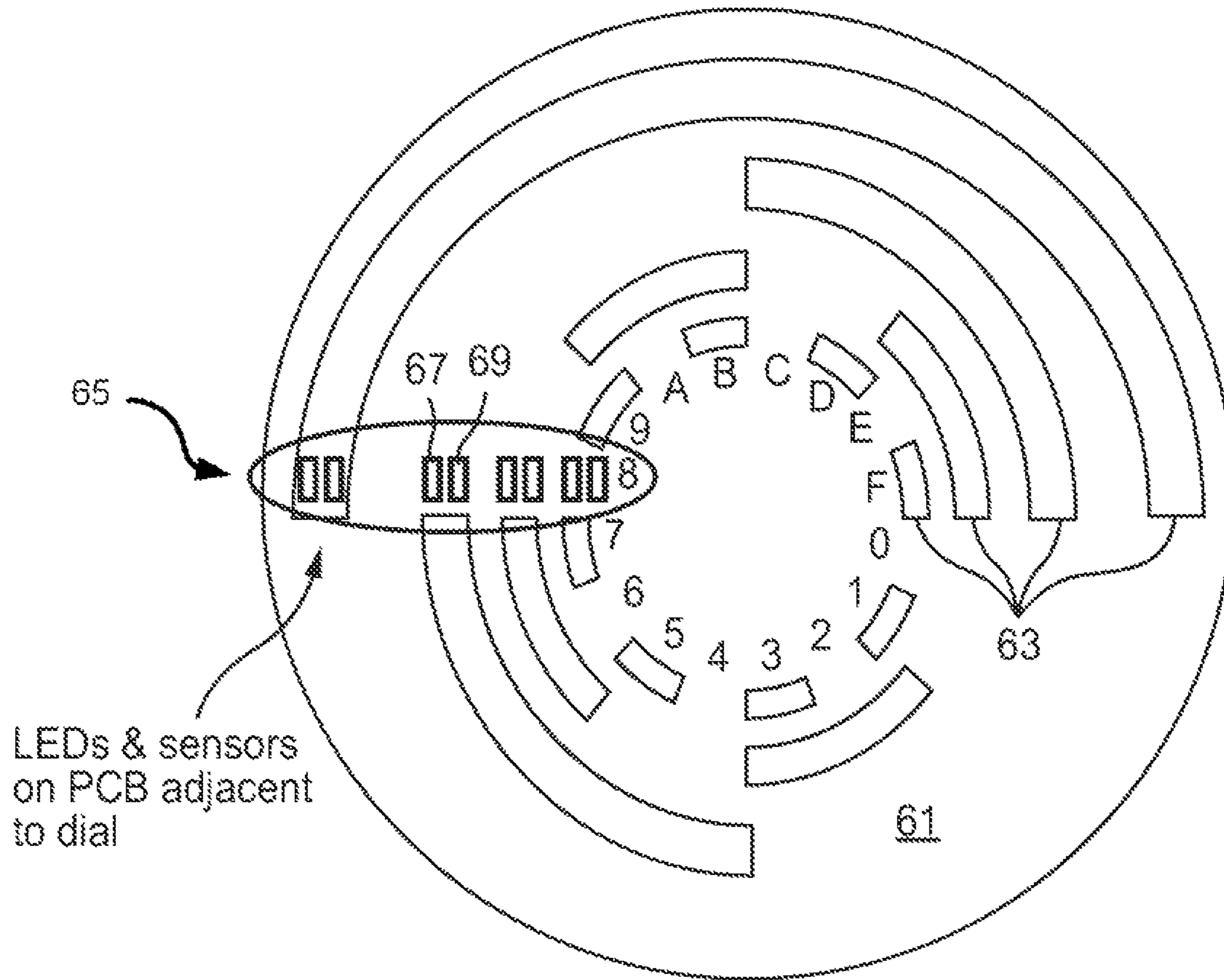
Layout of Dial Grooves
