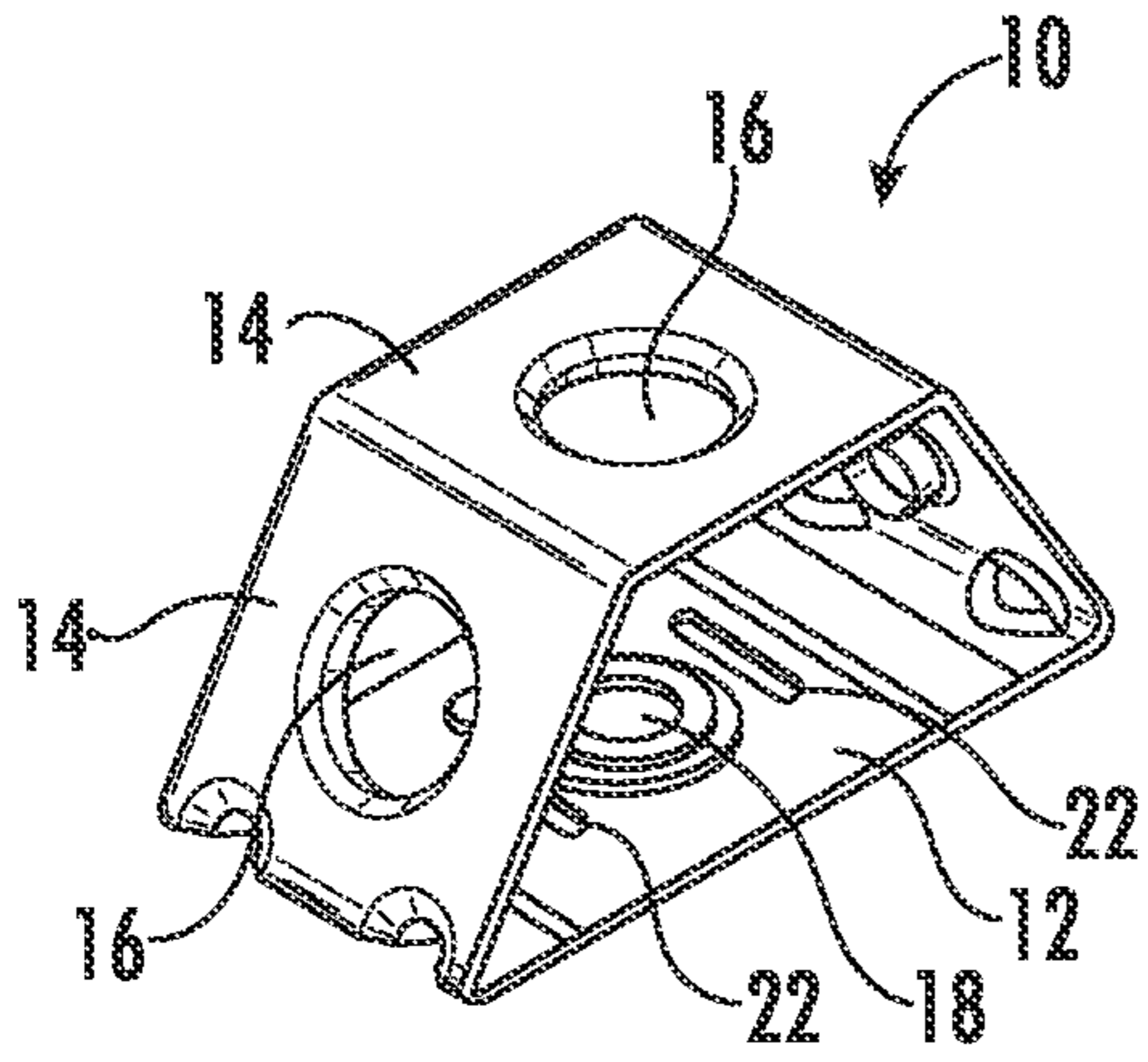
FIG. 1 {PRIOR ART}
