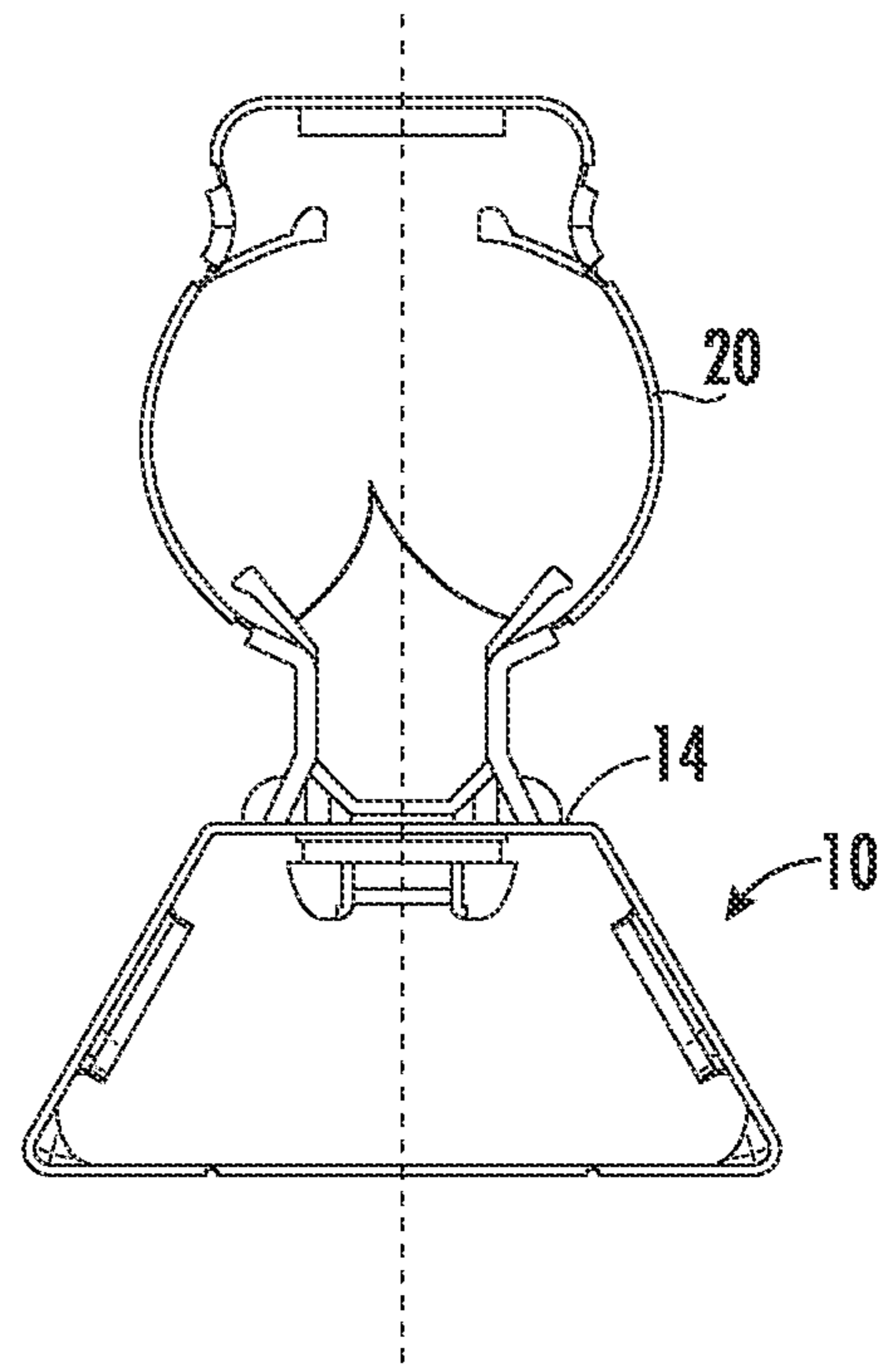
FIG. 2 {PRIOR ART}
