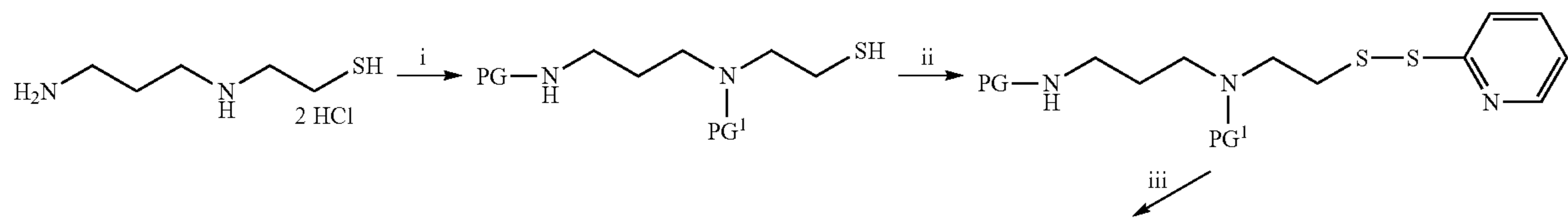
Scheme 3.
