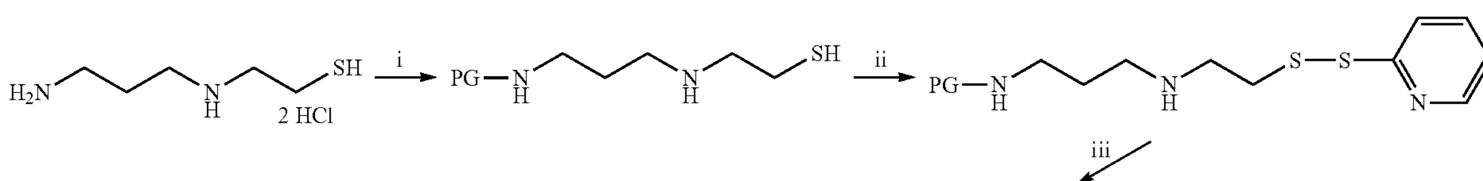
Scheme 2.
