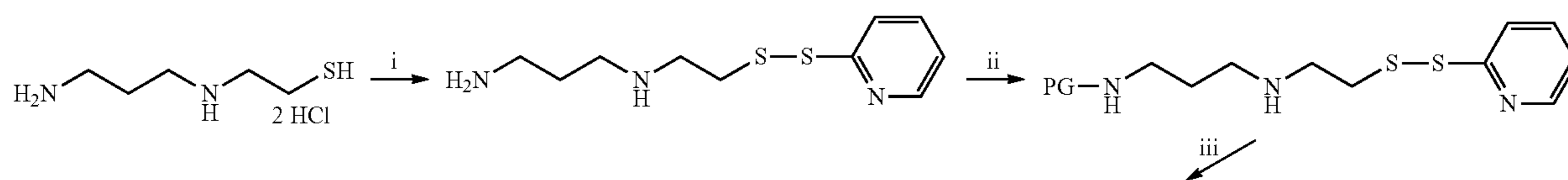
Scheme 4.
