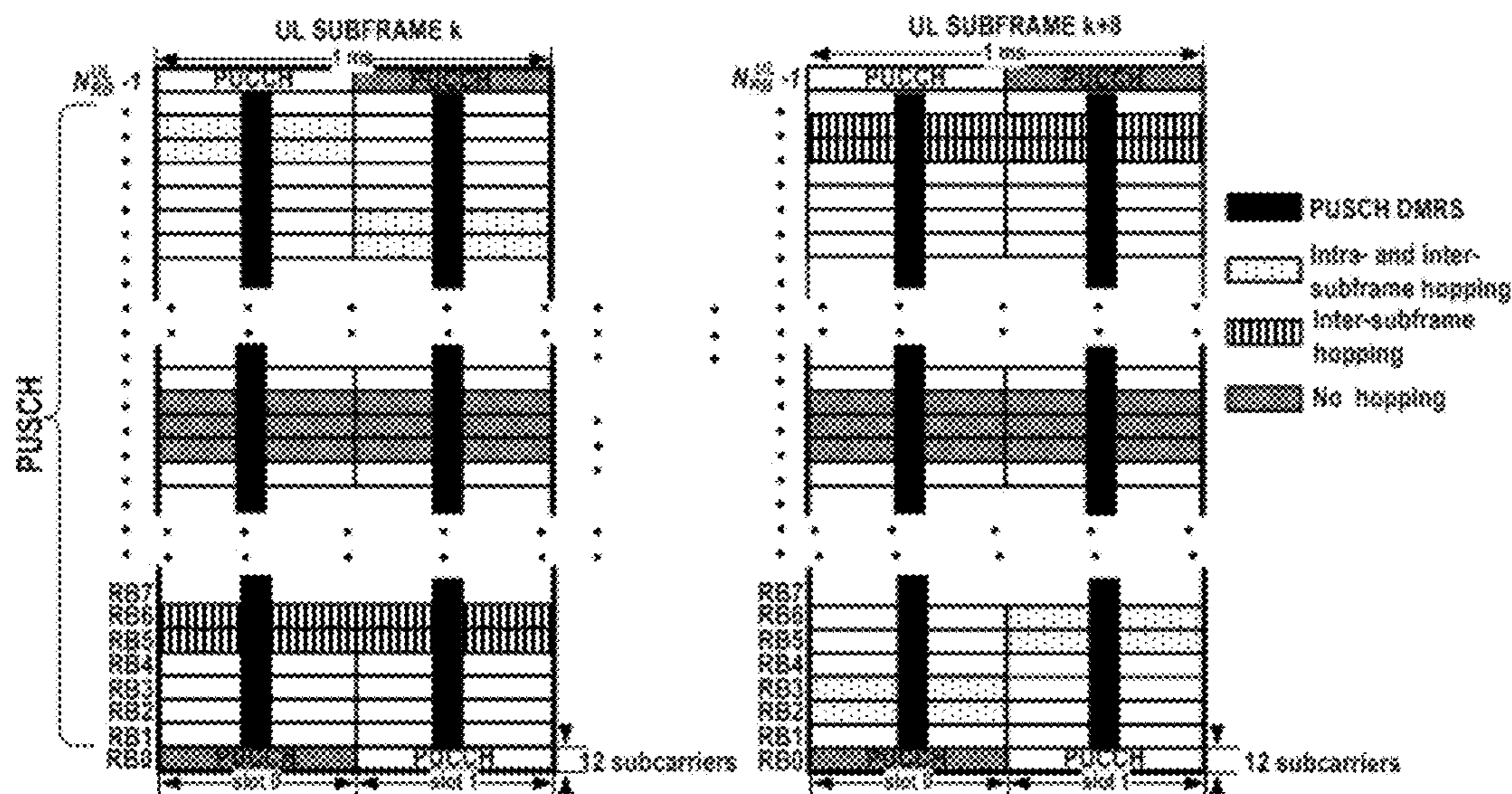
Fig. 3 (Related Art)
