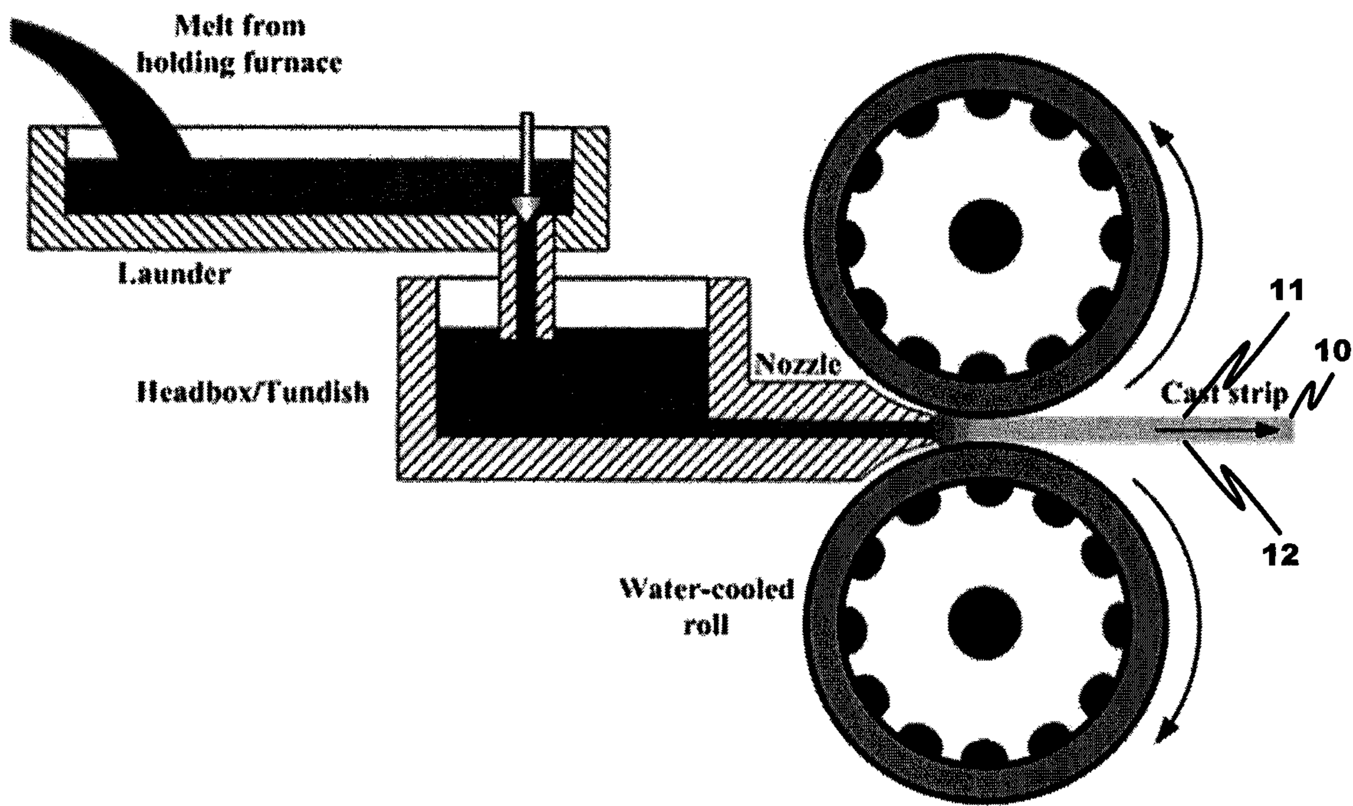
Fig. 8 (Prior Art)
