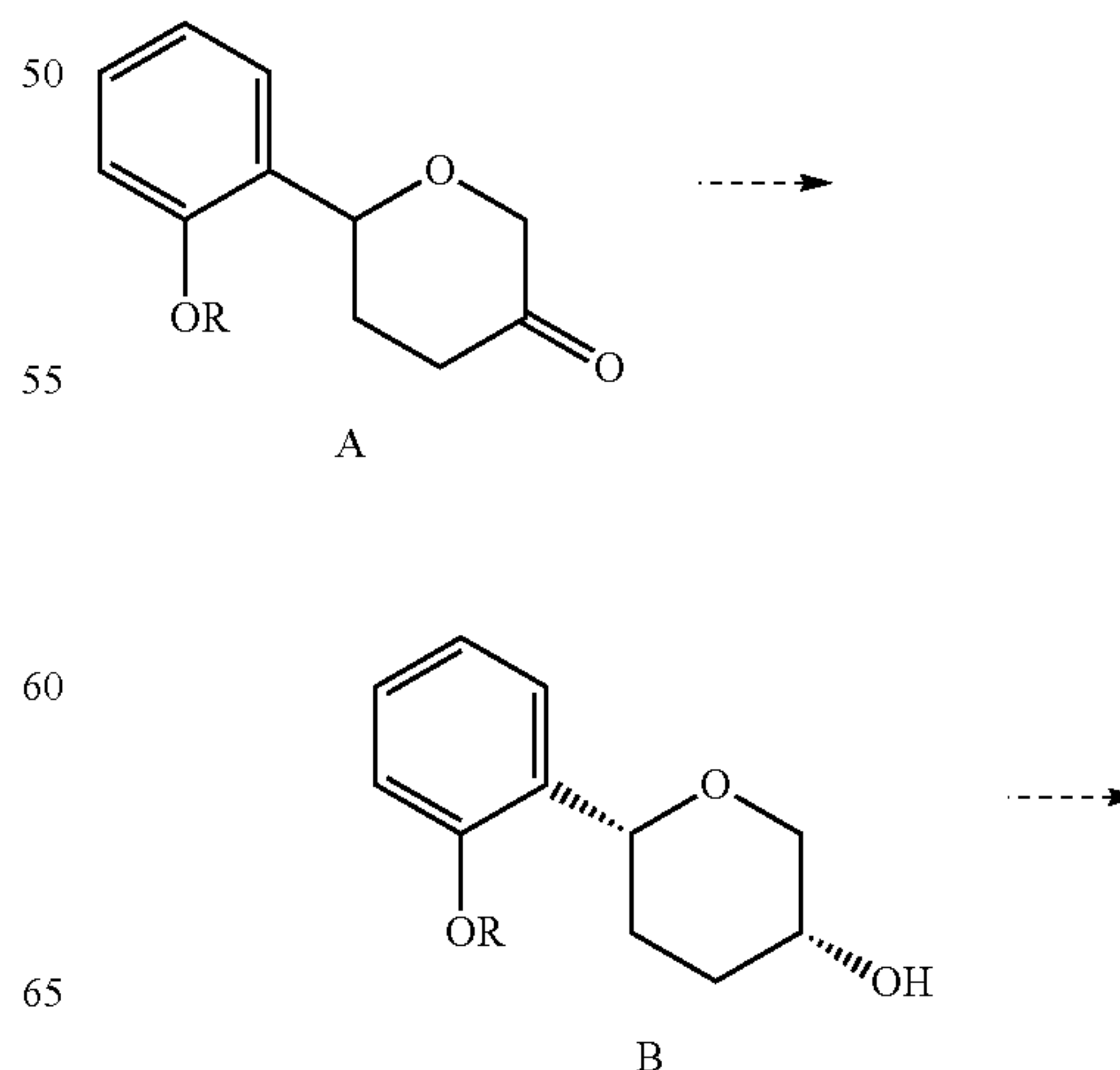
Scheme 2
