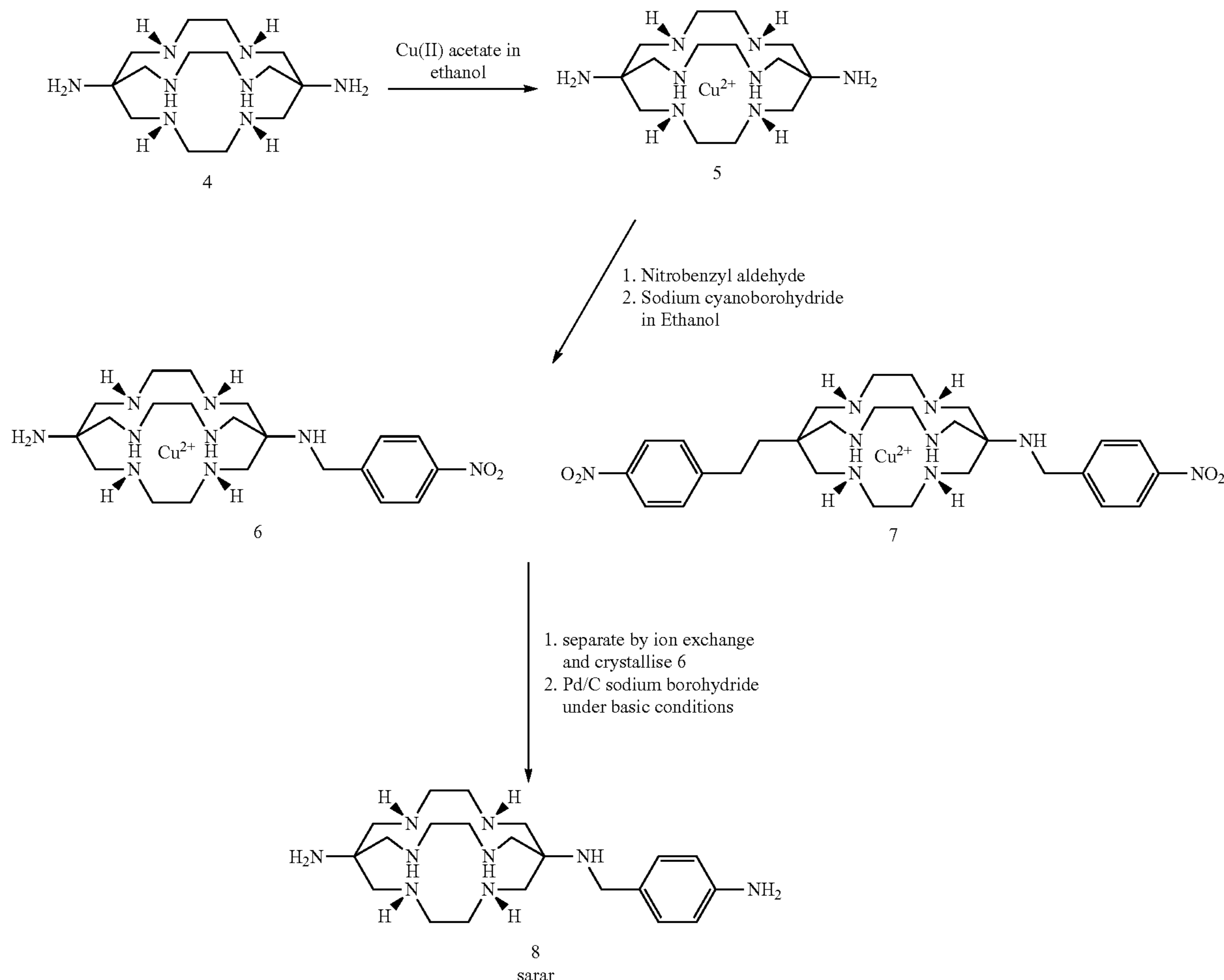
Scheme 2 - Synthesis of sarar (compound 8)
