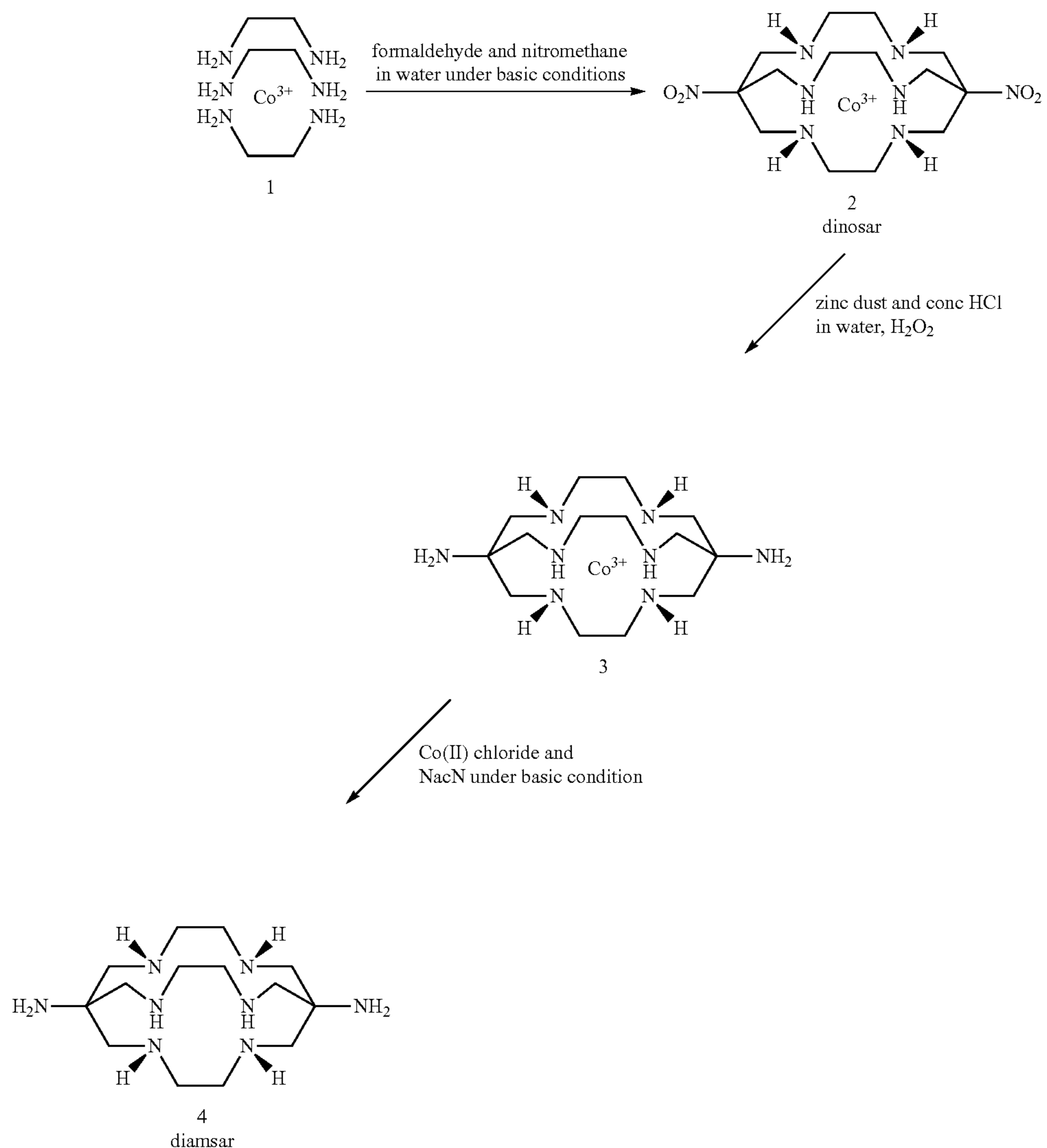
Scheme 1 - Synthesis of diamsar (compound 4)
