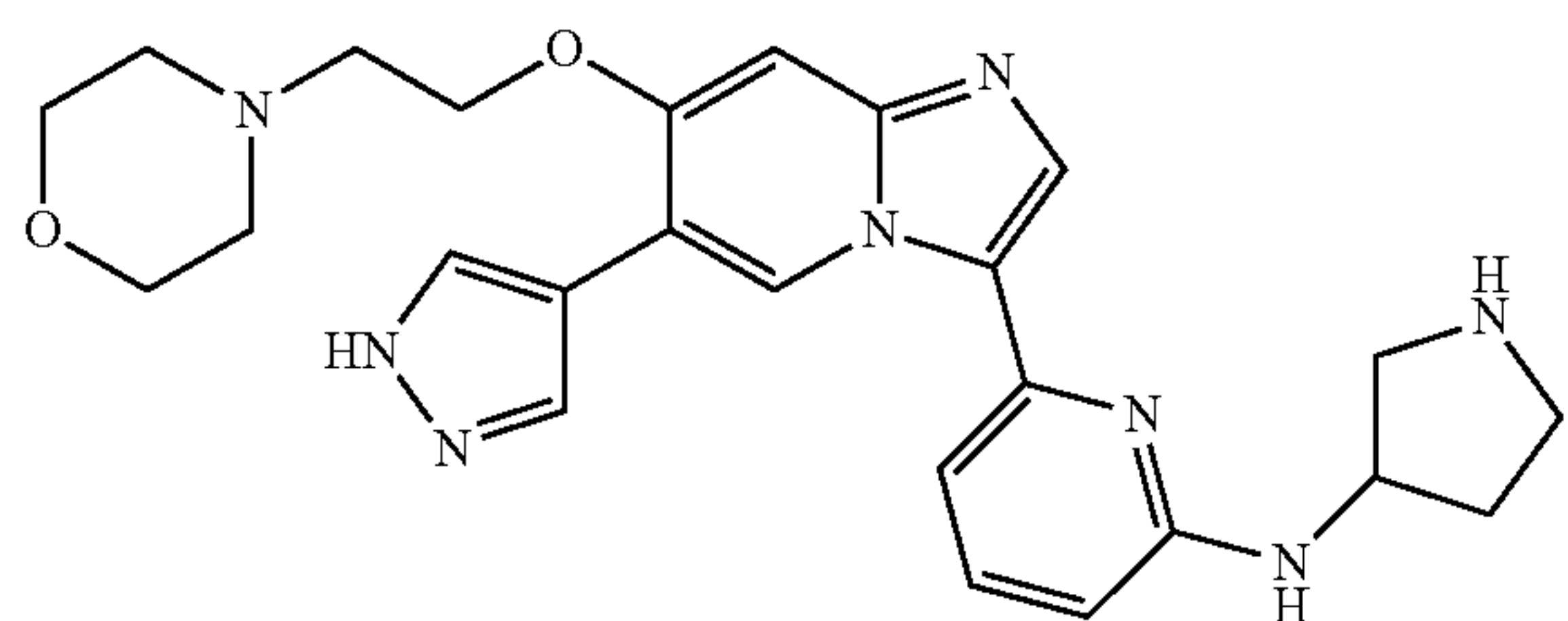
6-(7-(2-morpholinoethoxy)-6-(1H-pyrazol-4-yl)imidazo[1,2-a]pyridin-3-yl)-N-(pyrrolidin-3-yl)pyridin-2-amine (I-41)
