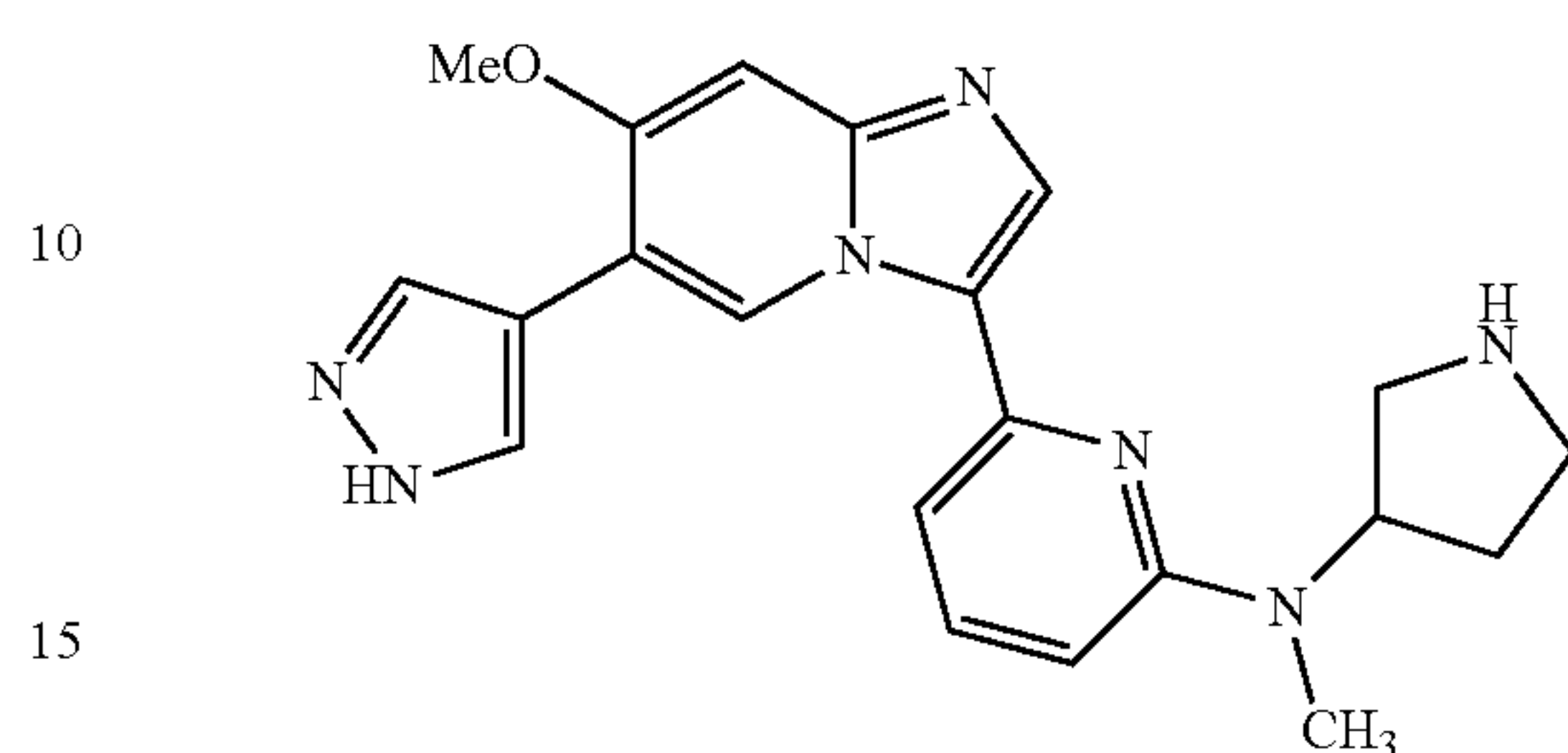
6-(7-methoxy-6-(1H-pyrazol-4-yl)imidazo[1,2-a]pyridin-3-yl)-N-methyl-N-(pyrrolidin-3-yl)pyridin-2-amine (I-31)
