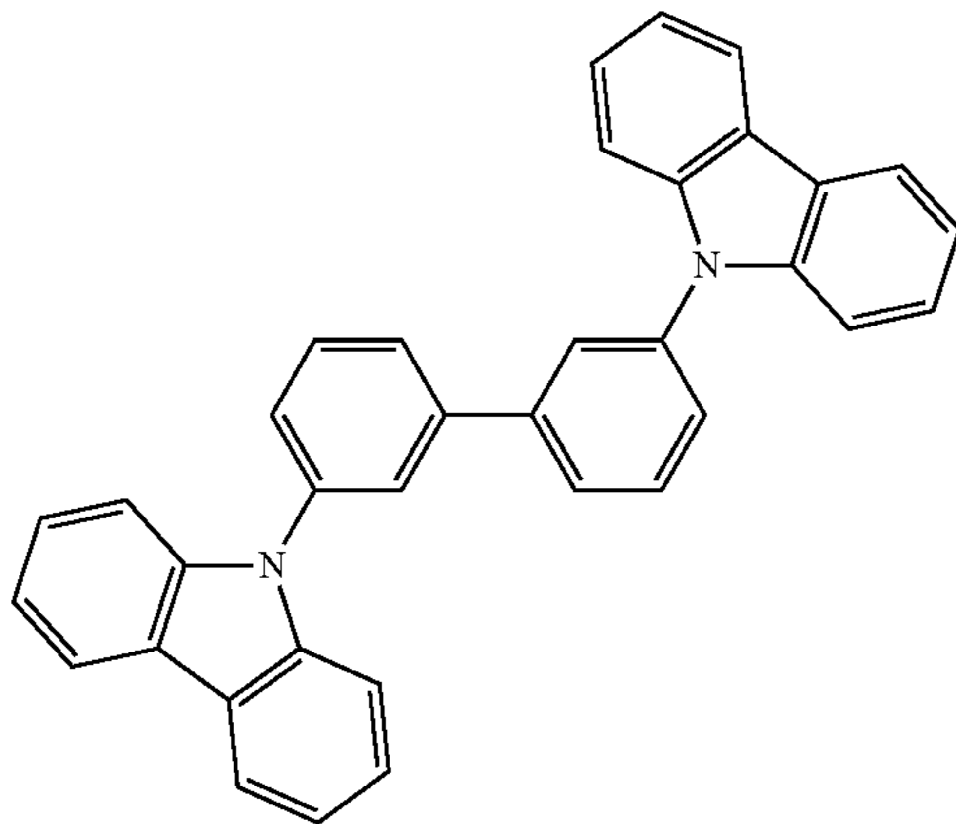
mCBP
