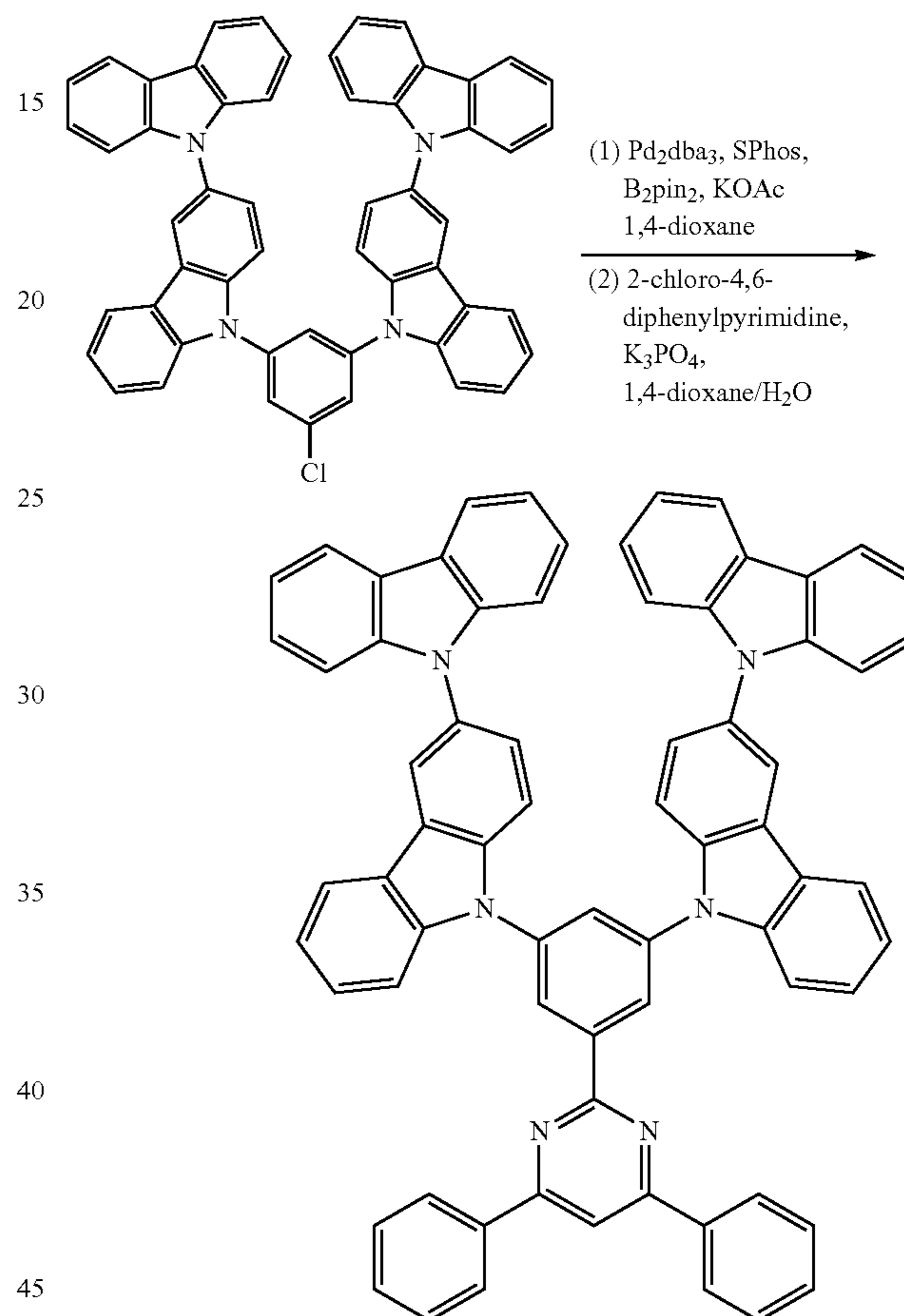
Synthesis of 9,9''-(5-(4,6-diphenylpyrimidin-2-yl)-1,3-phenylene)bis(9H-3,9'-bicarbazole)) (Compound 1)
