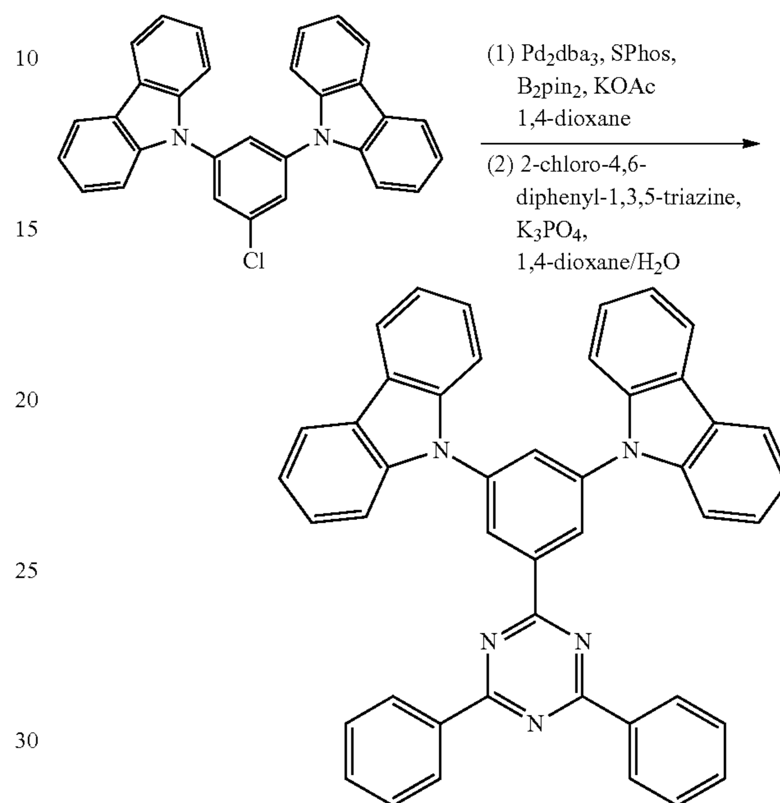
Synthesis of 9,9'-(5-(4,6-diphenyl-1,3,5-triazin-2-yl)-1,3-phenylene)bis(9H-carbazole) (Compound 3)
