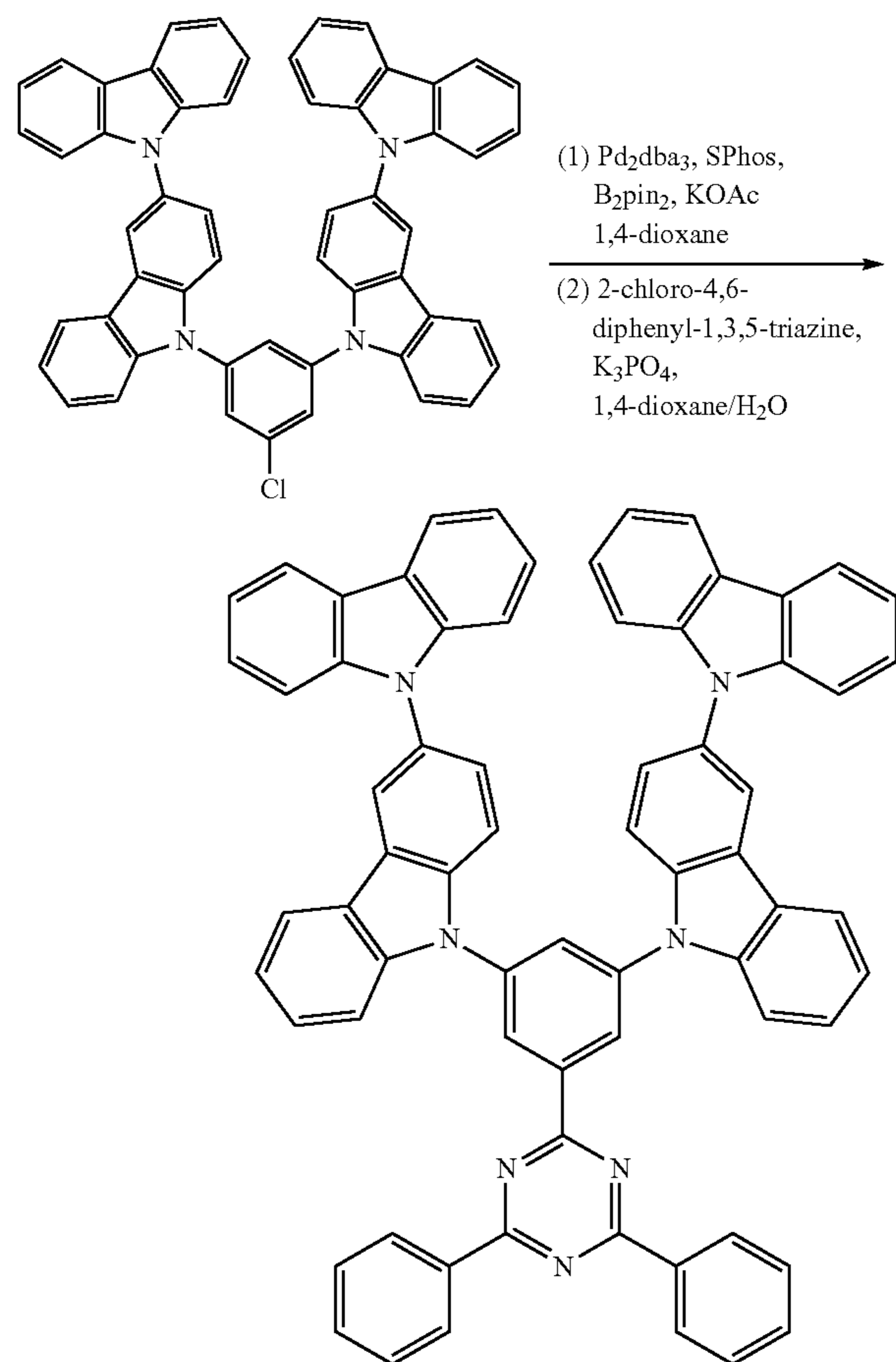
Synthesis of 9,9'-(5-(4,6-diphenyl-1,3,5-triazin-2-yl)-1,3-phenylene)bis(9H-3,9'-bicarbazole) (Compound 2)
