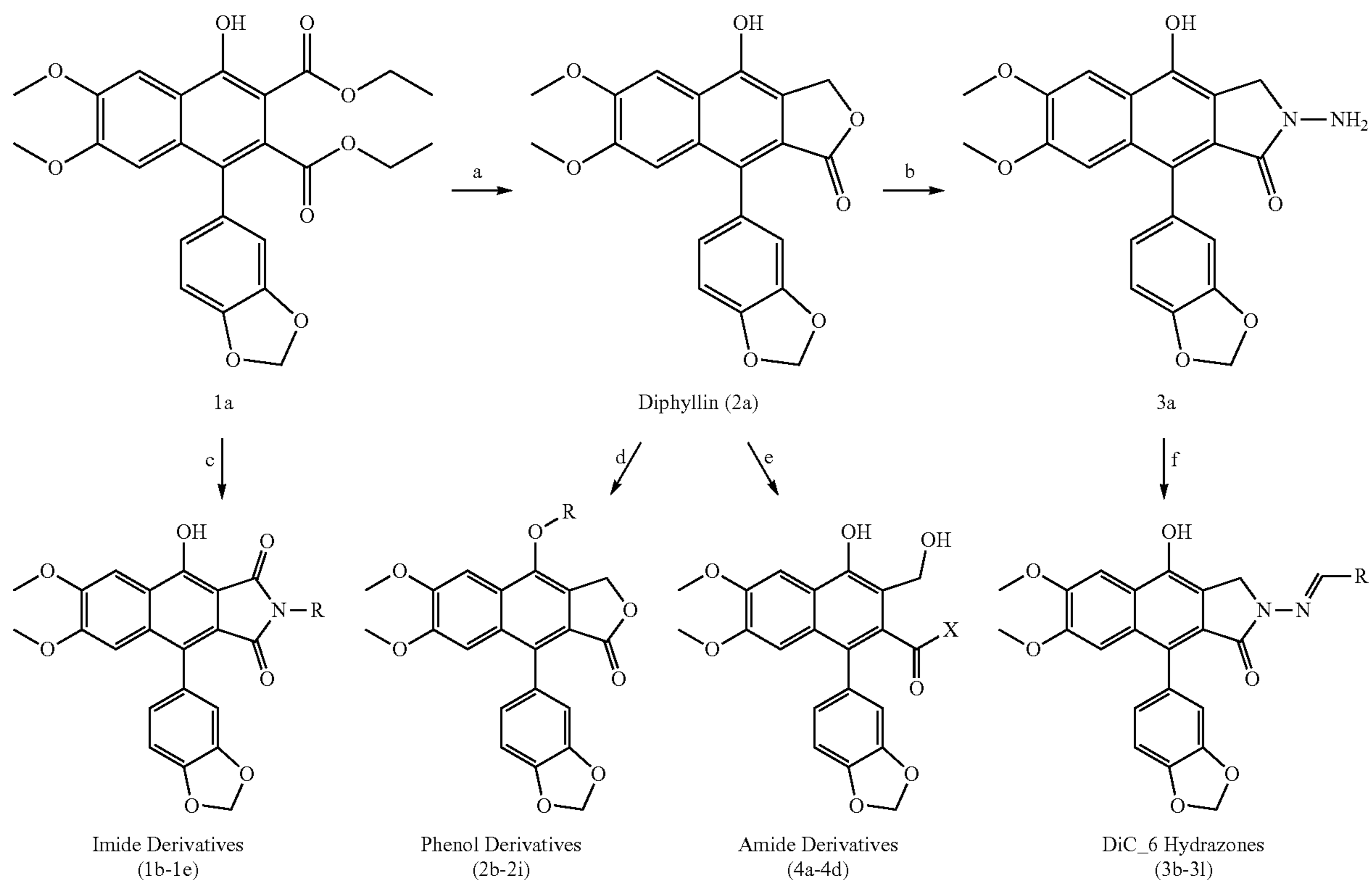
Scheme 1 Synthesis of Diphyllin Derivatives *
