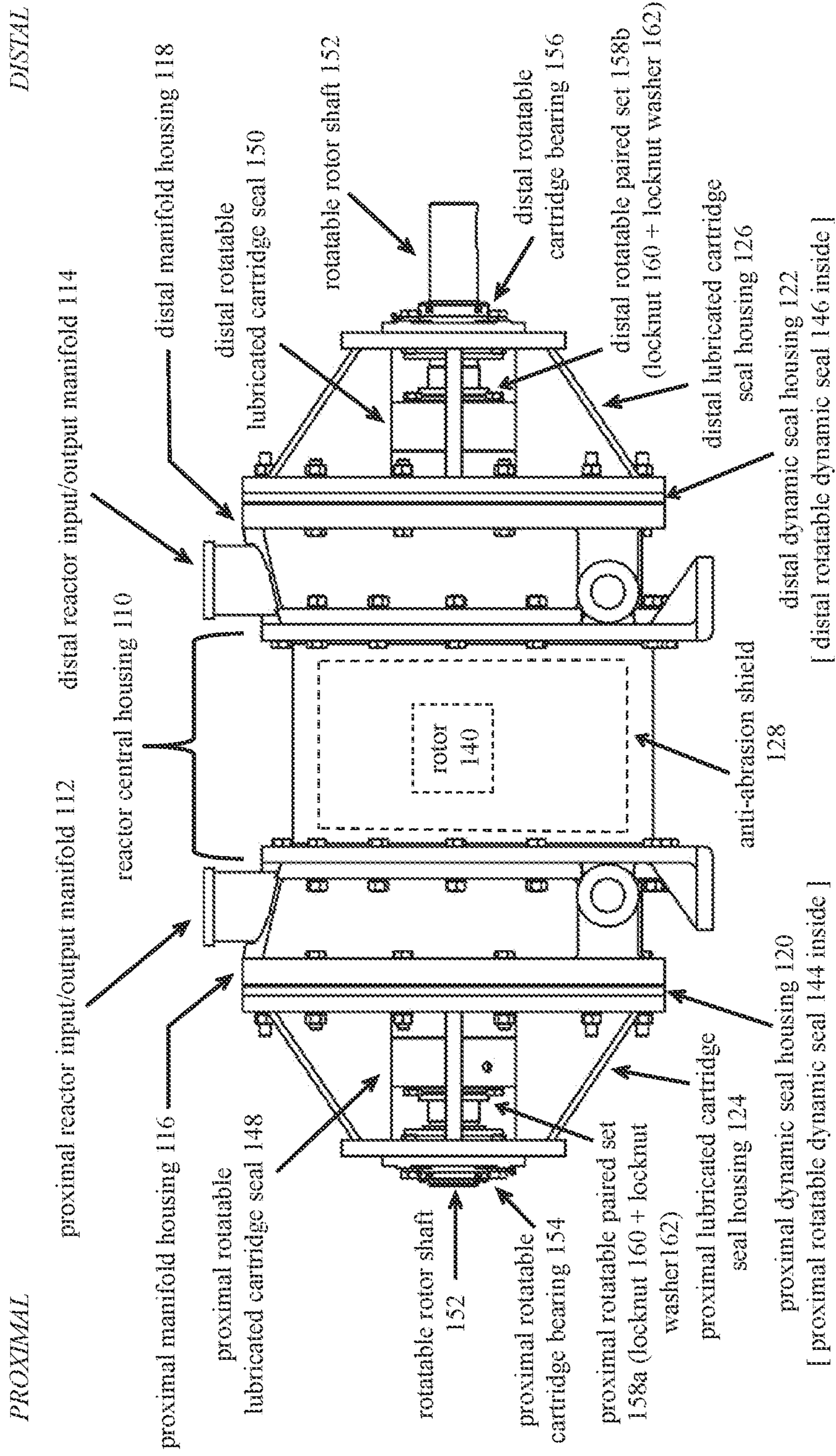
FIG. 1 (side view) chemical reactor 100
