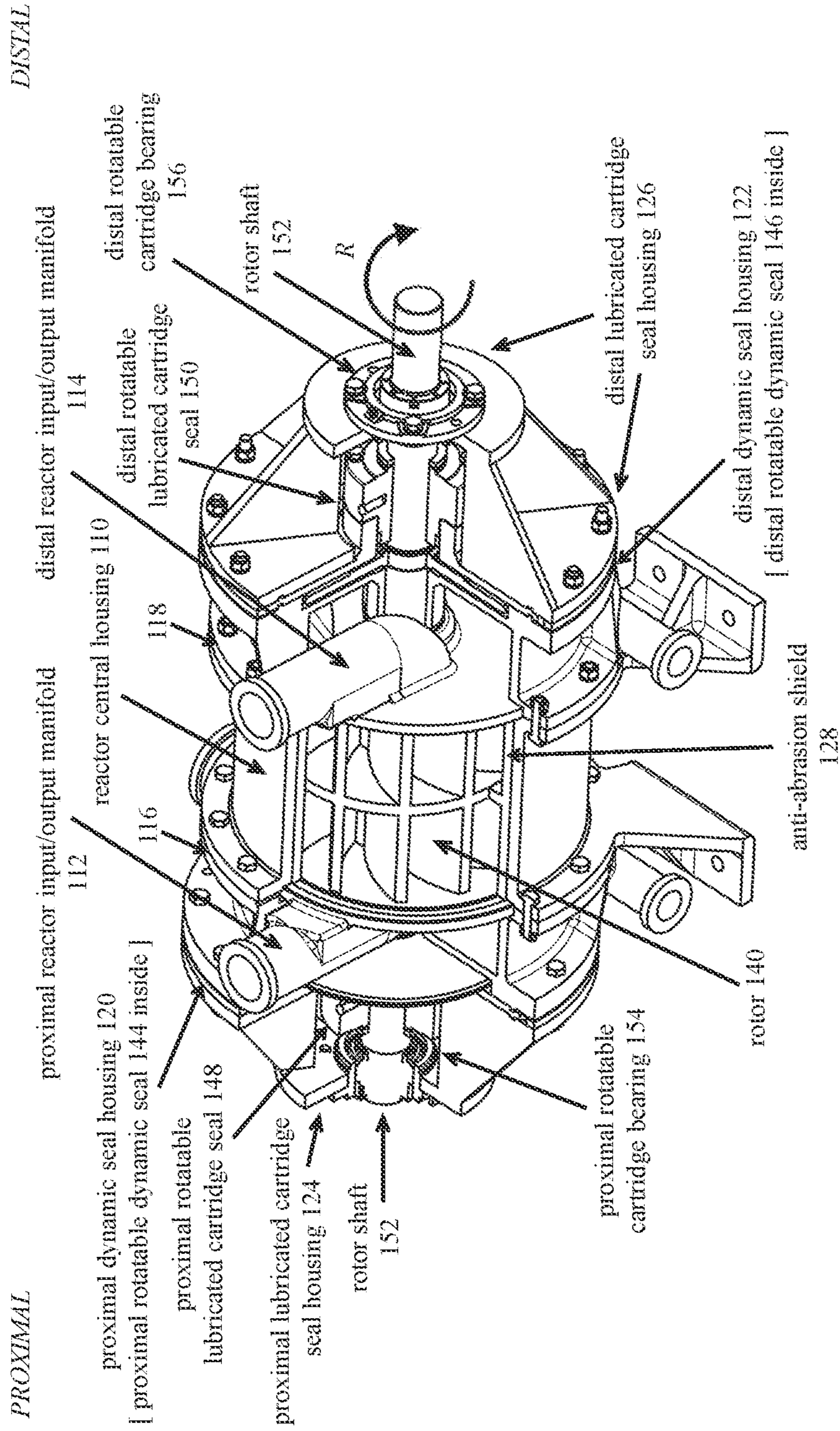
chemical reactor 100 FIG. 2A (perspective view)
