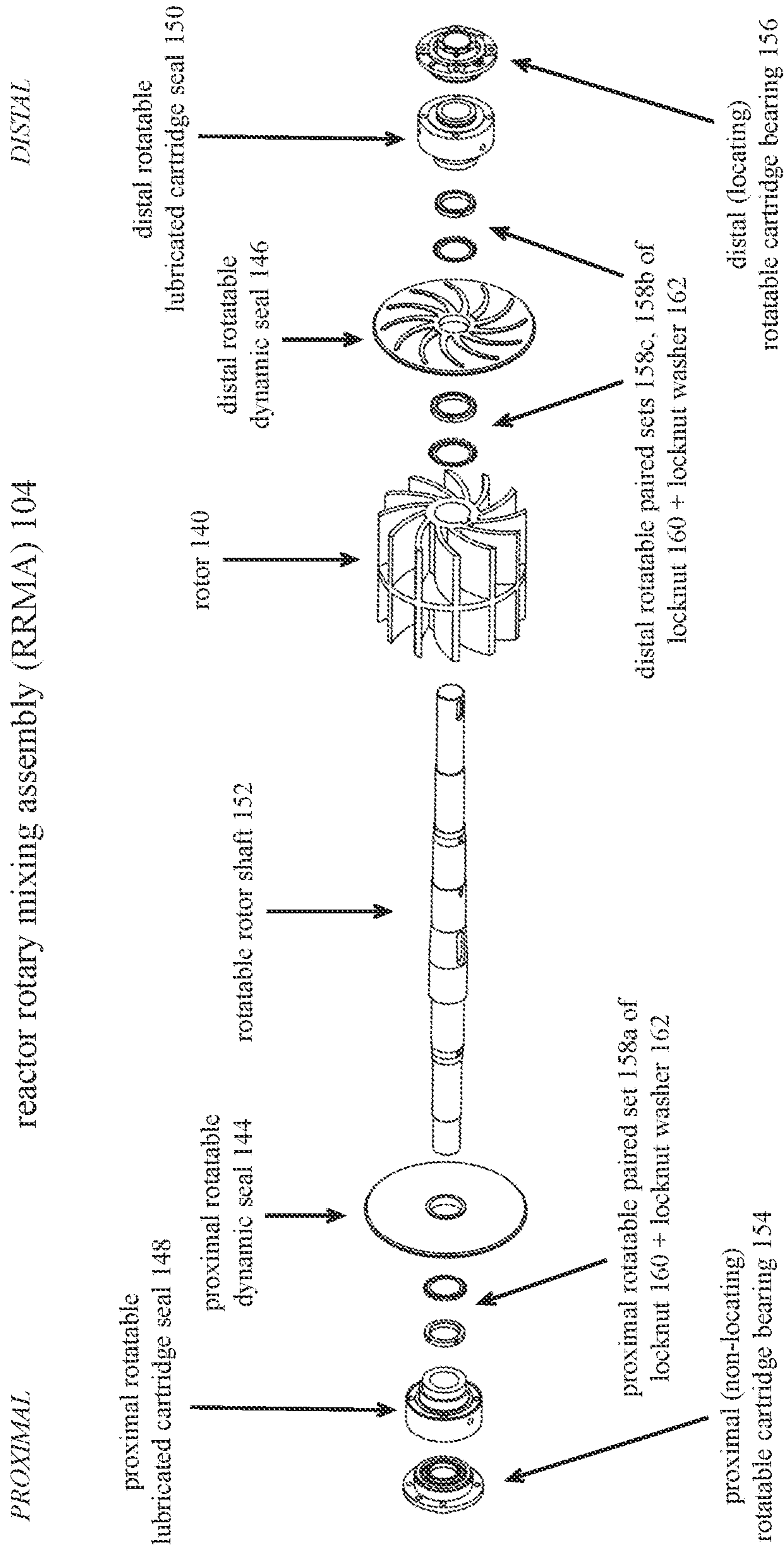
FIG. 5 (exploded perspective view)
