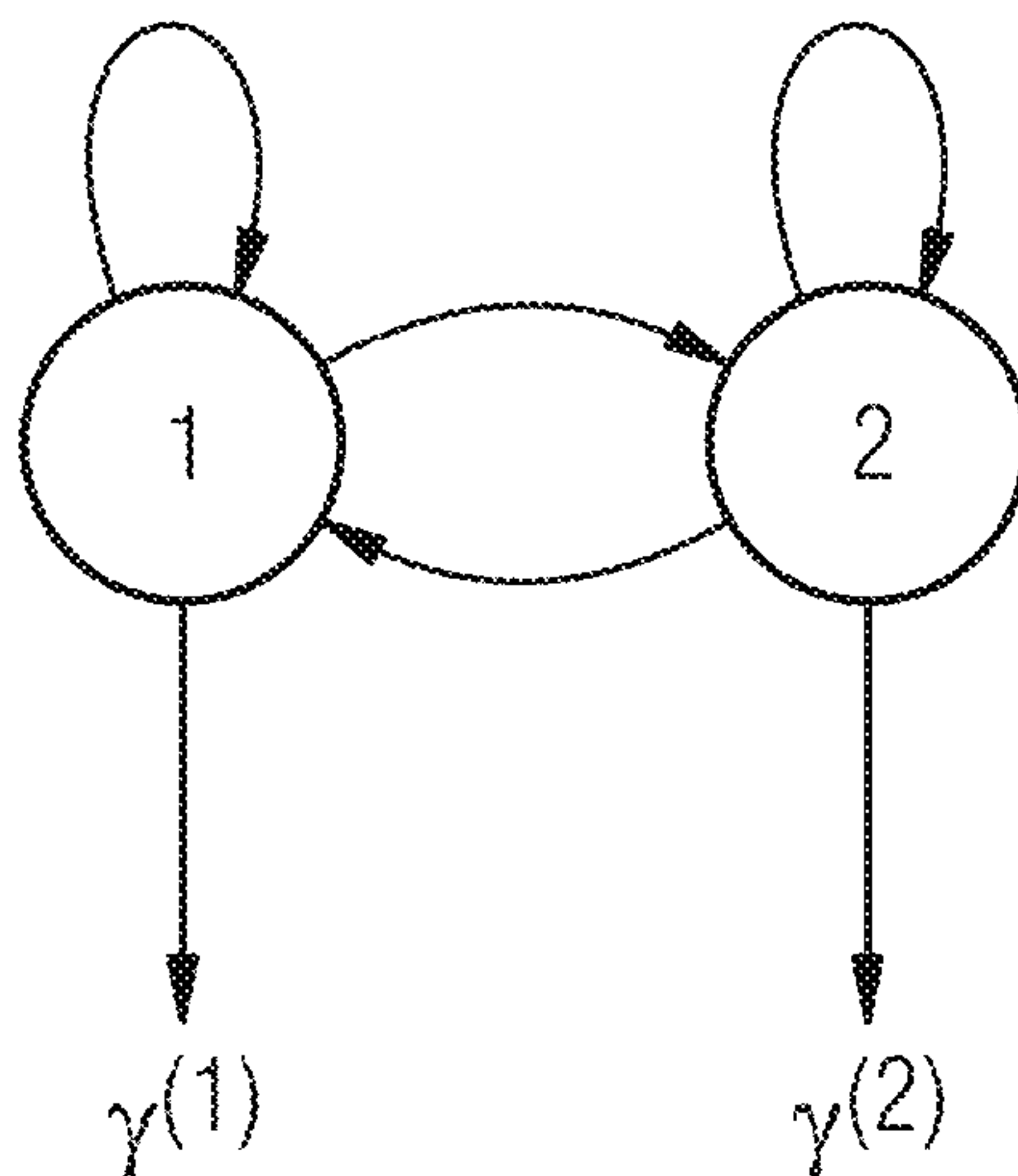
HMM of the NULL class with the states z_N \in \{1, 2\} and outputs \gamma .
