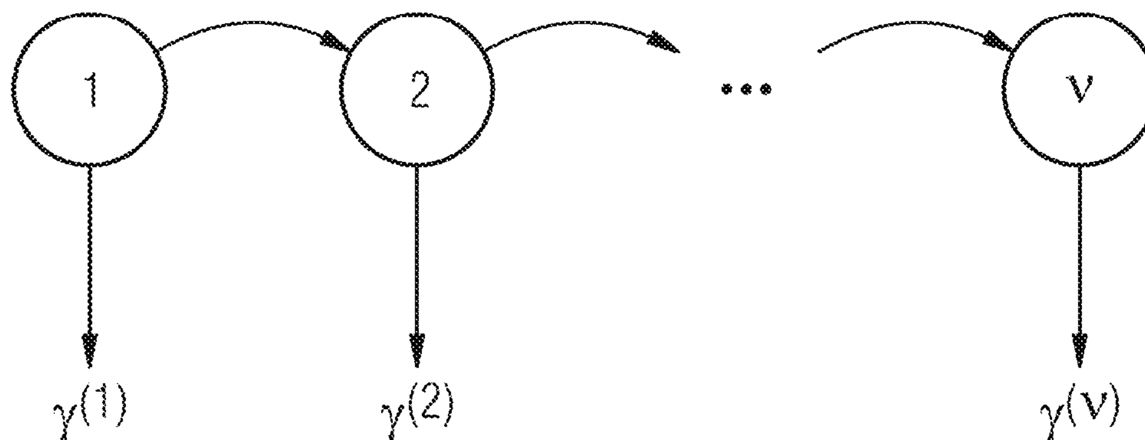
HMM of the event to be determined with the states z_k \in \{1, \dots, v\} and outputs \gamma .
