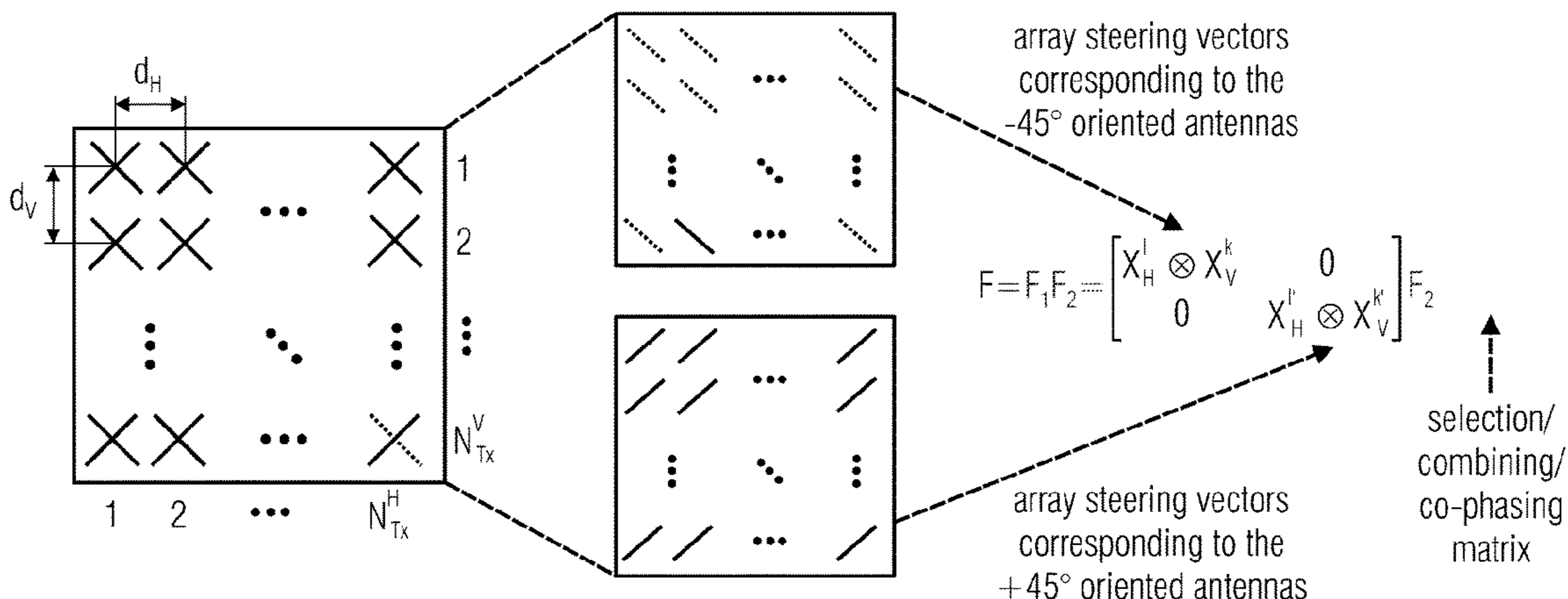
uniform planar array with dual polarized antennas in FD-MIMO
