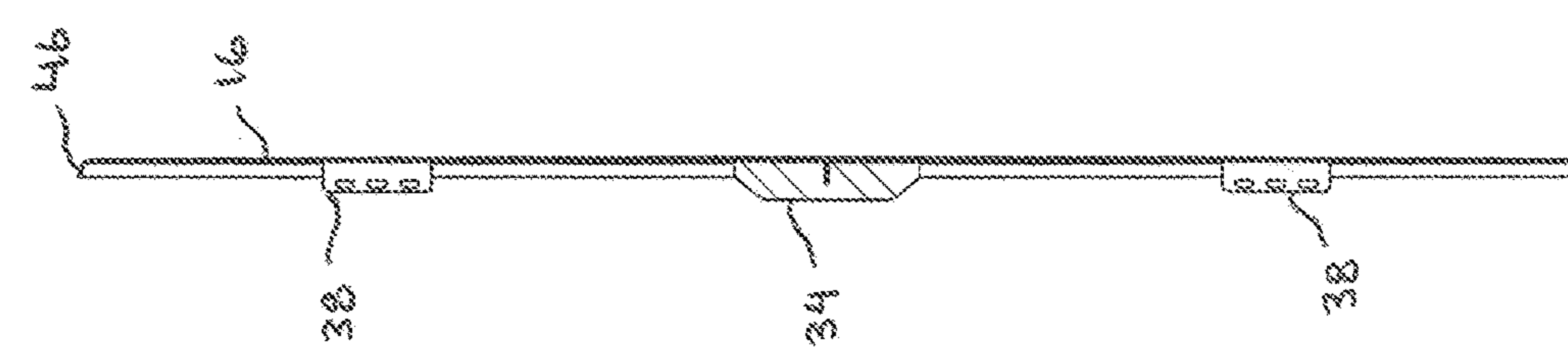
SECTION B-B
