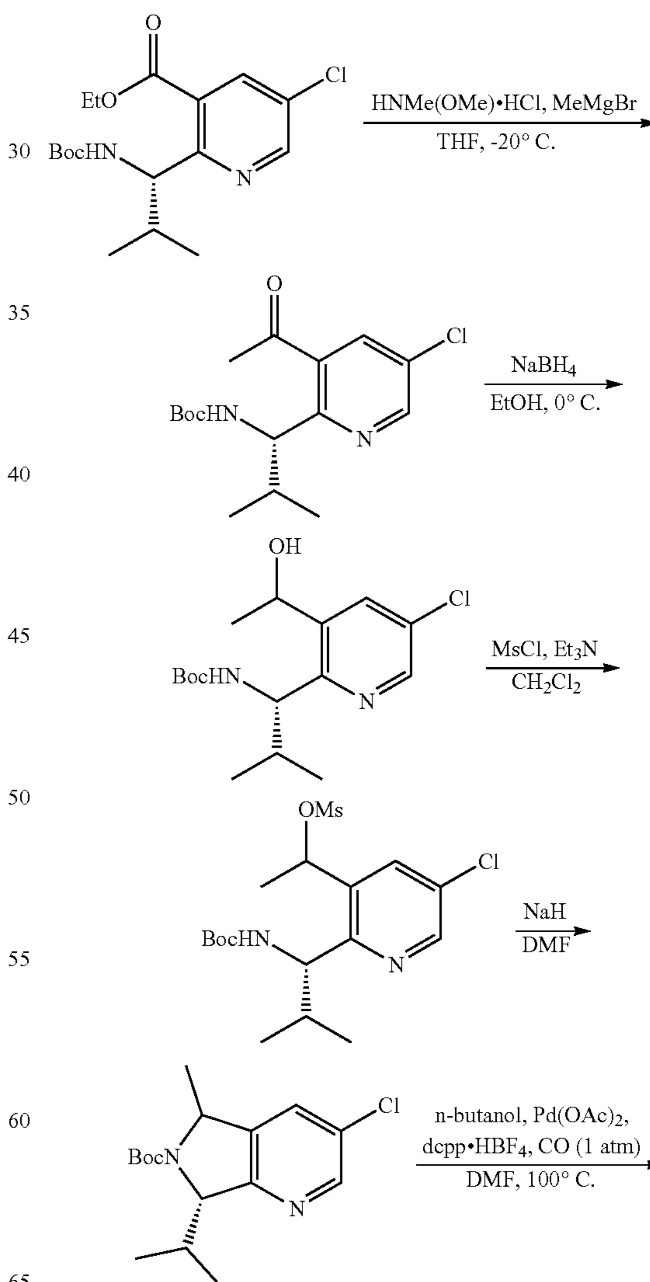
Scheme 11.
