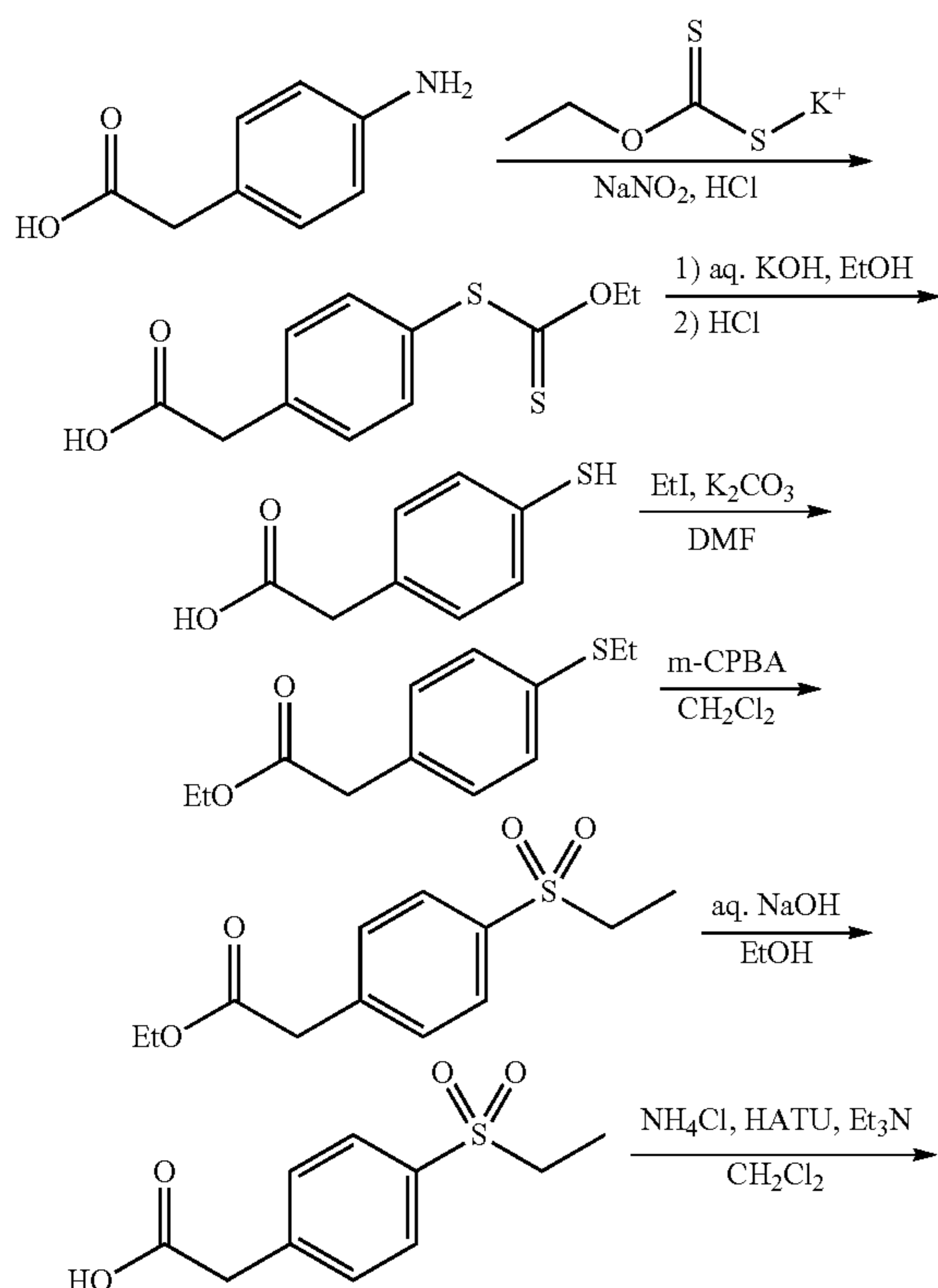
Scheme 9.
