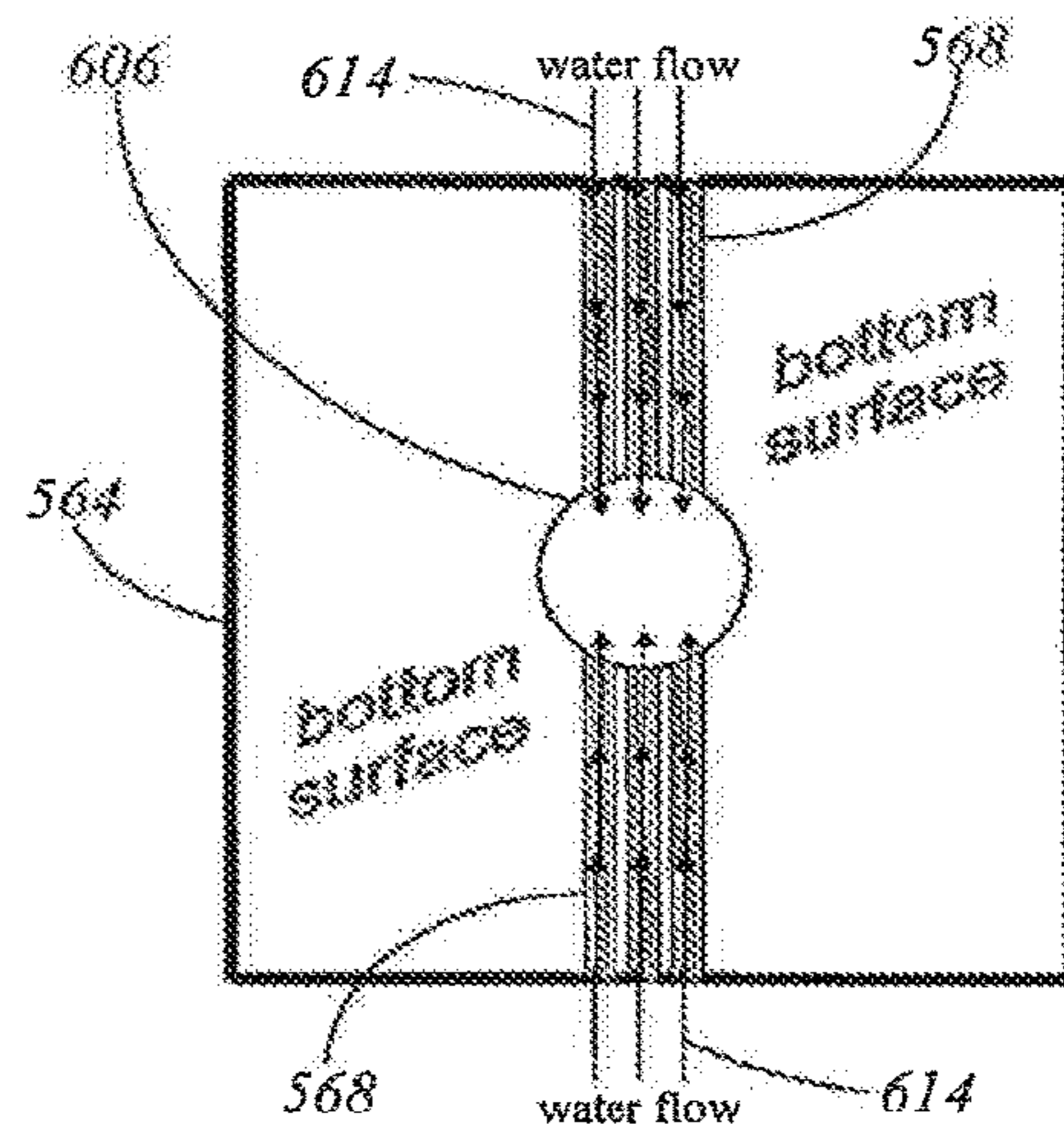
FIG. 17B bottom view
