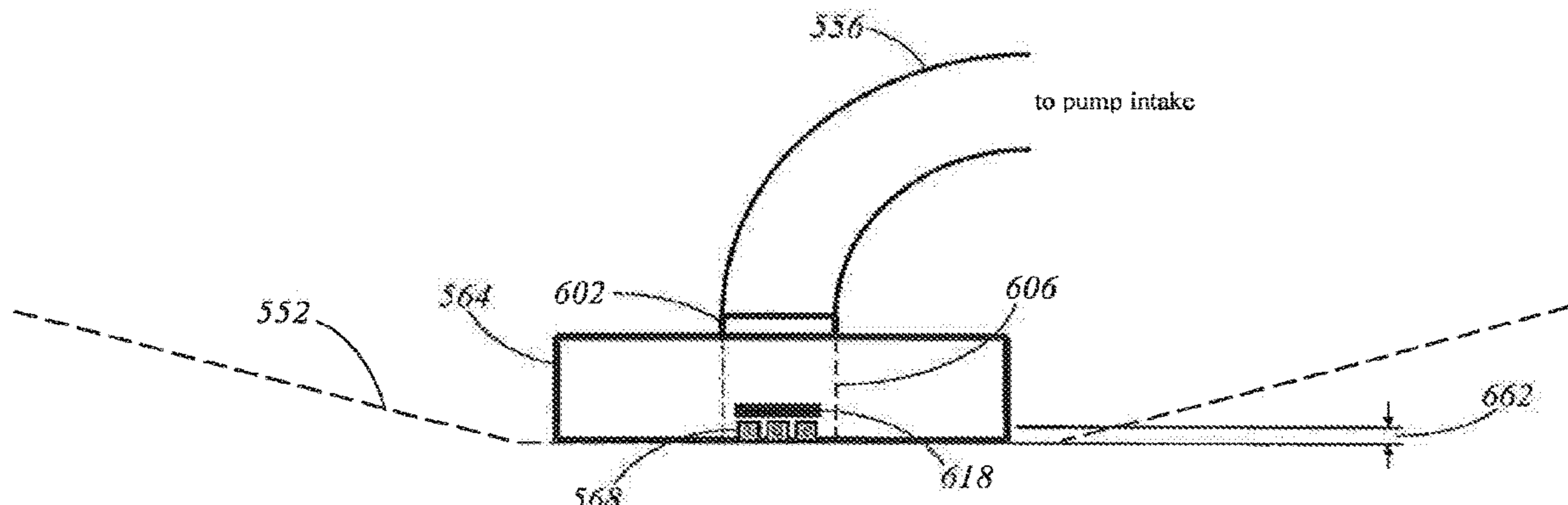
FIG. 17A side view
