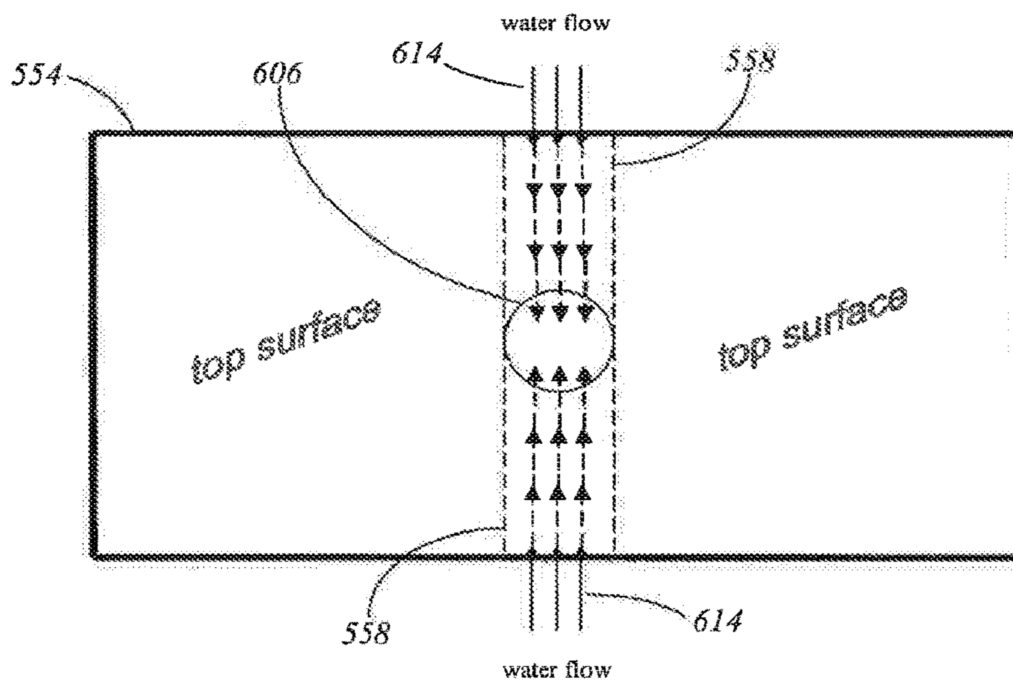
FIG. 16B top view
