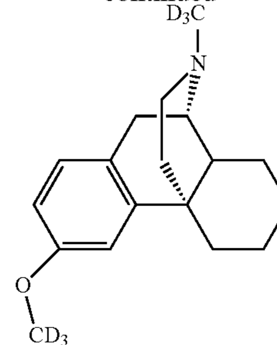
d6-dextromethorphan
