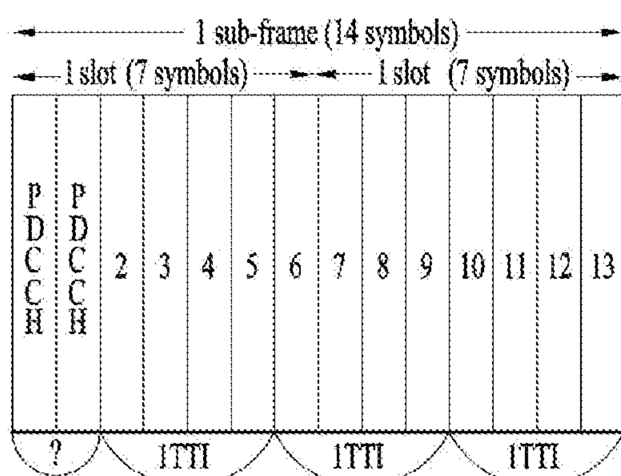
(c) 4 symbol TTI DL structure
