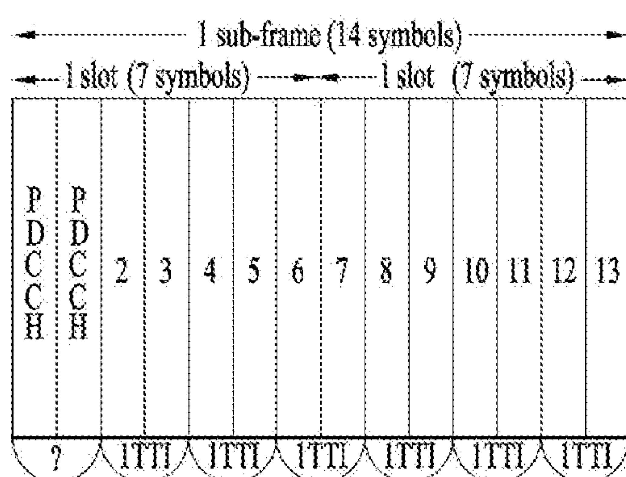
(a) 2 symbol TTI DL structure
