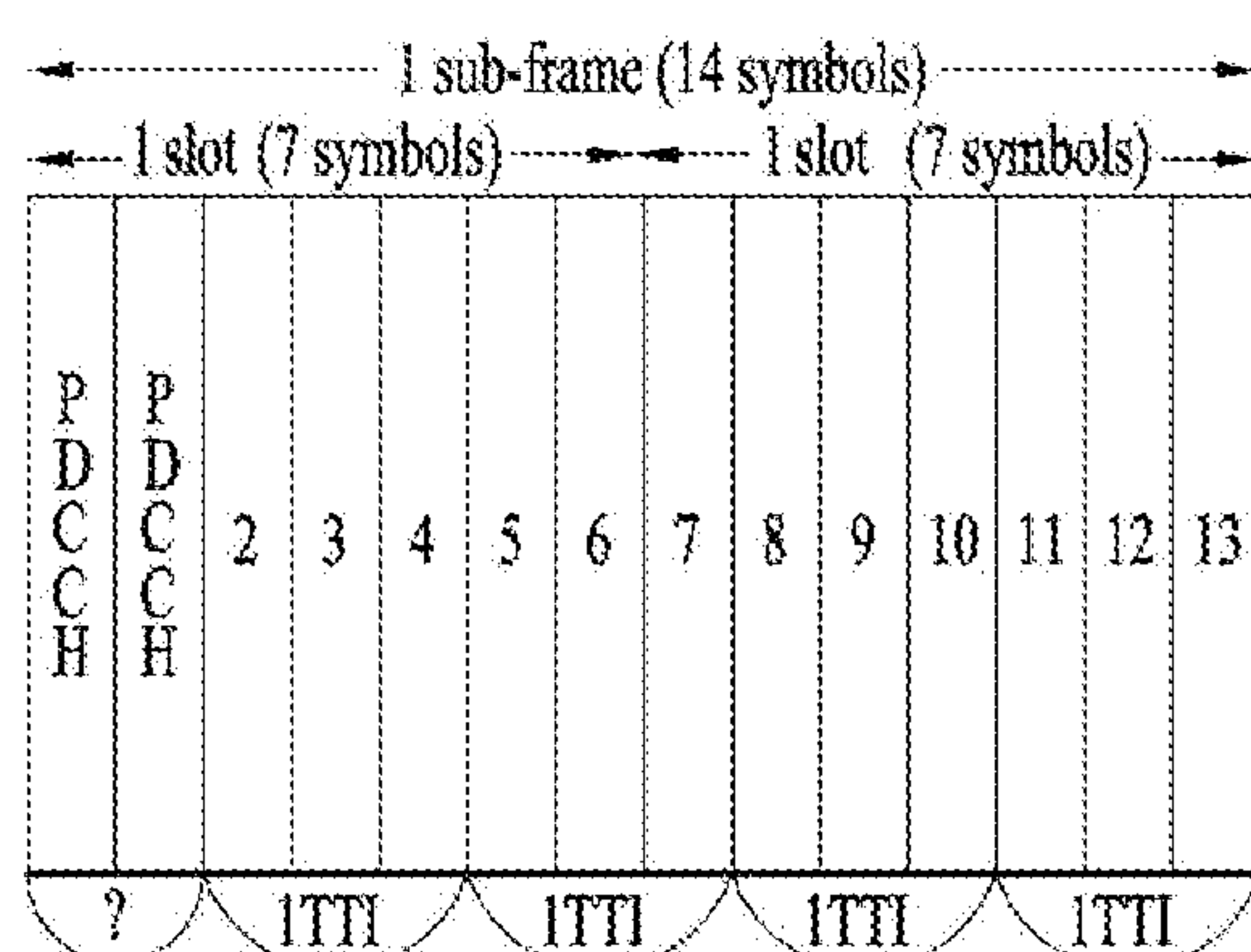
(b) 3 symbol TTI DL structure
