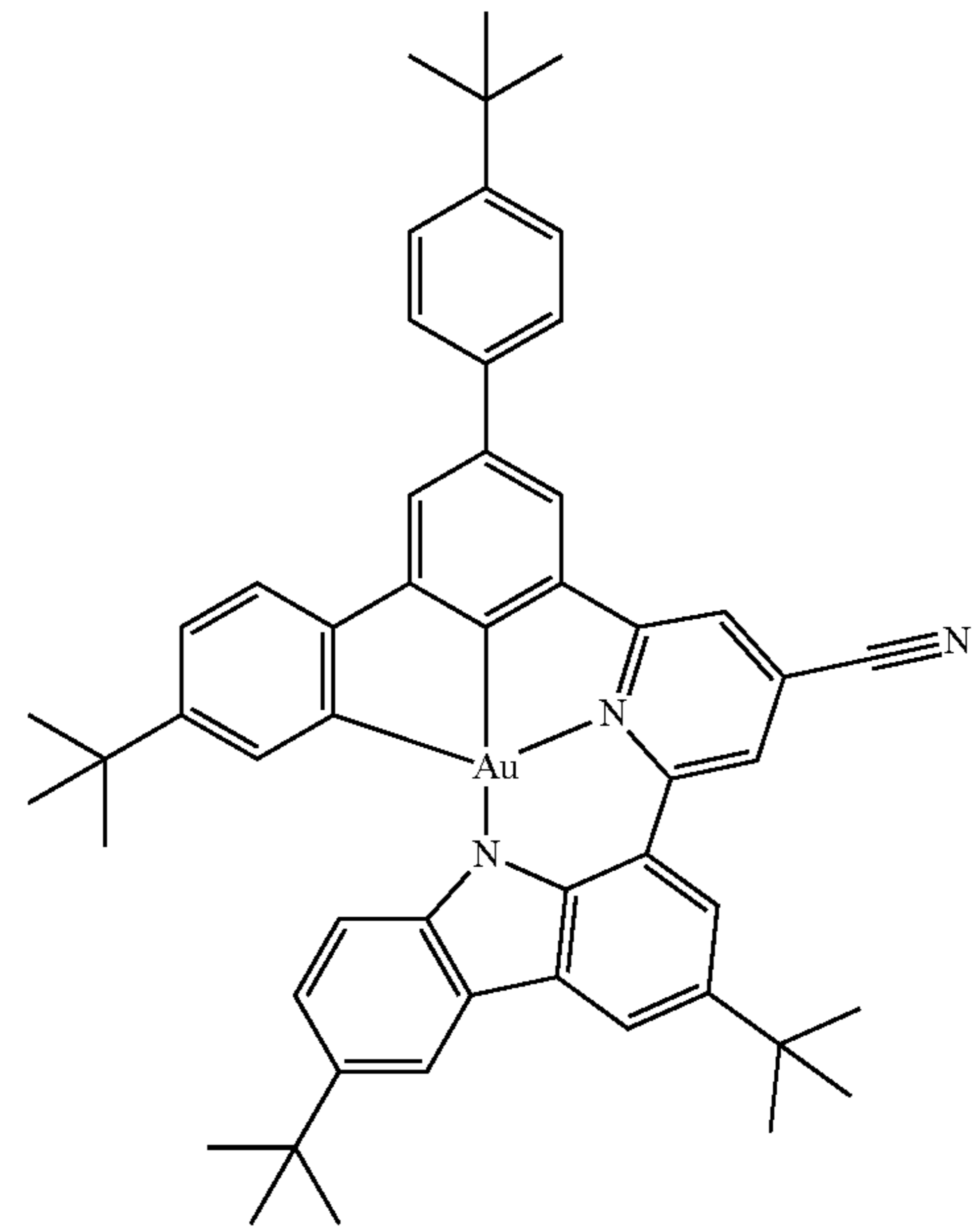
Compound 131
