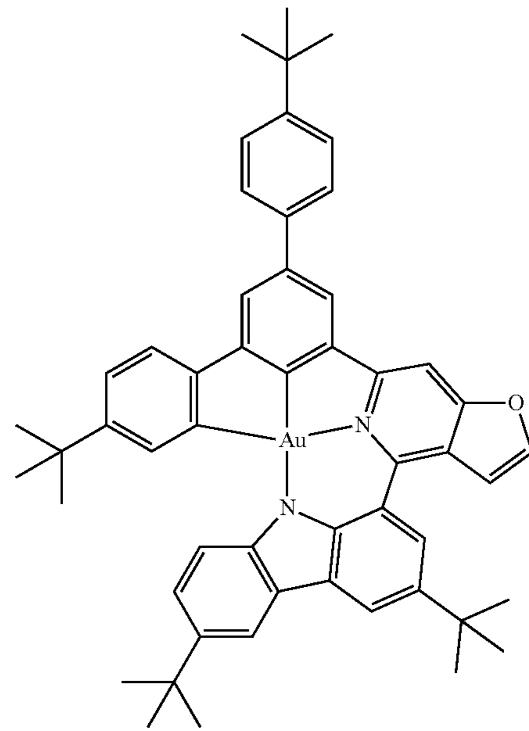
Compound 148
