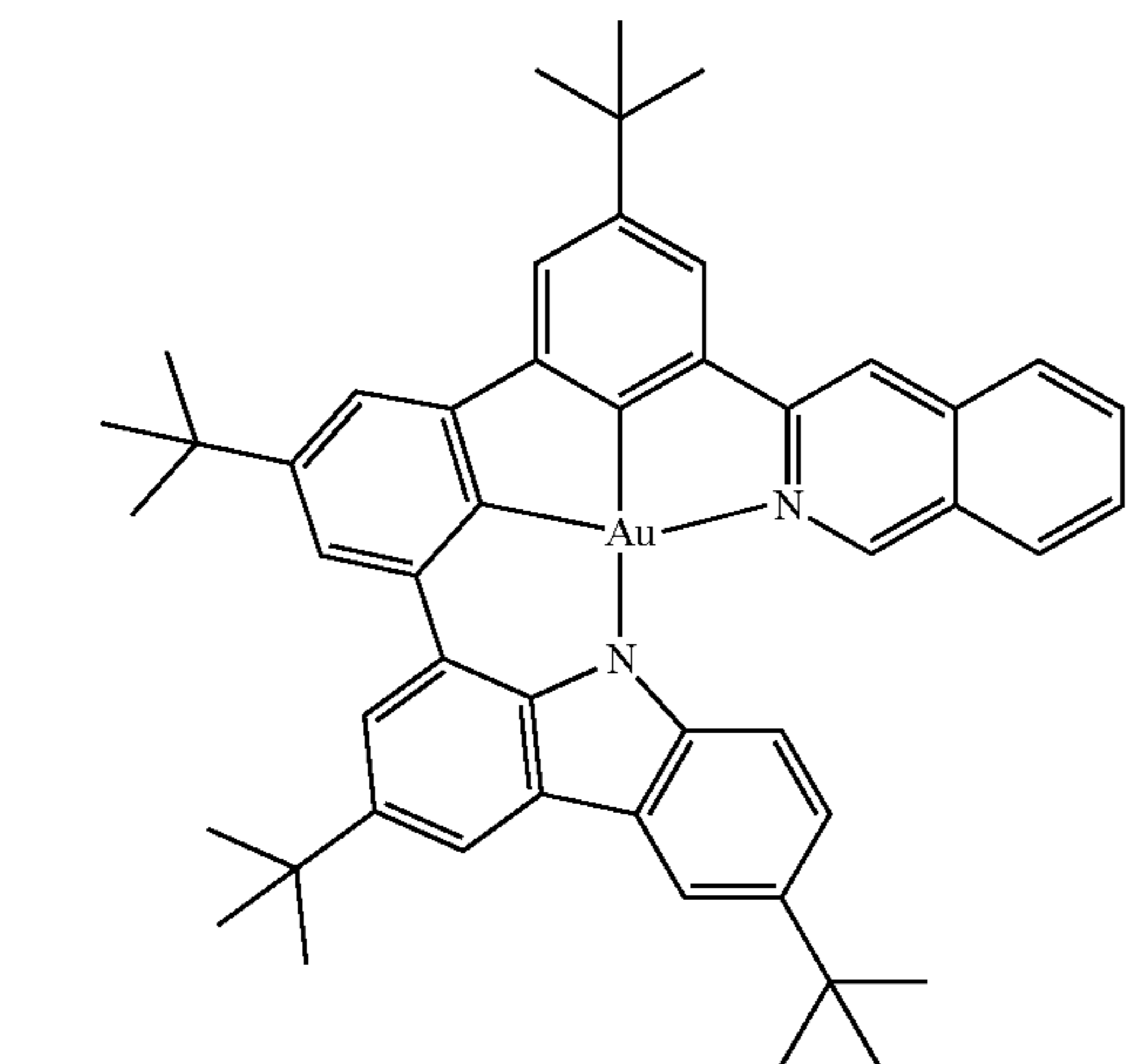
Compound 156
