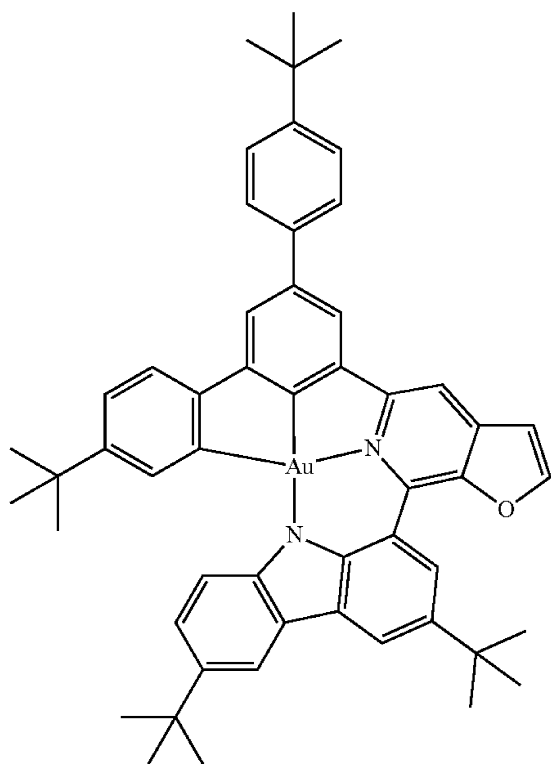
Compound 147
