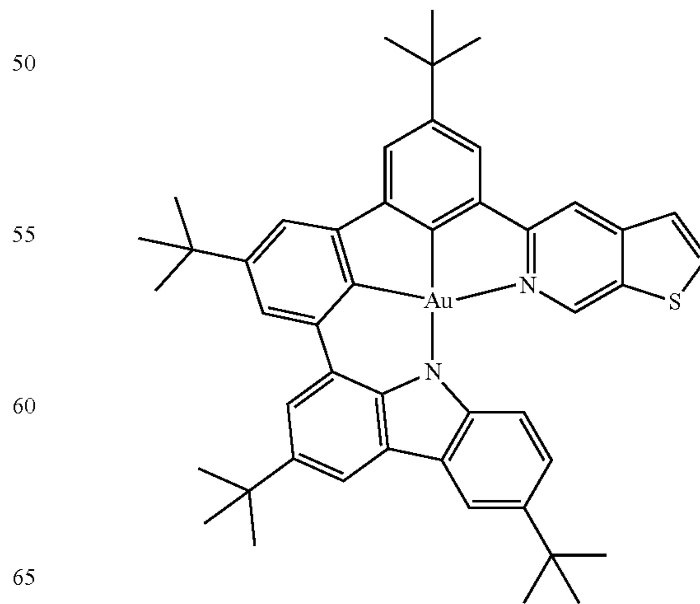
Compound 159
