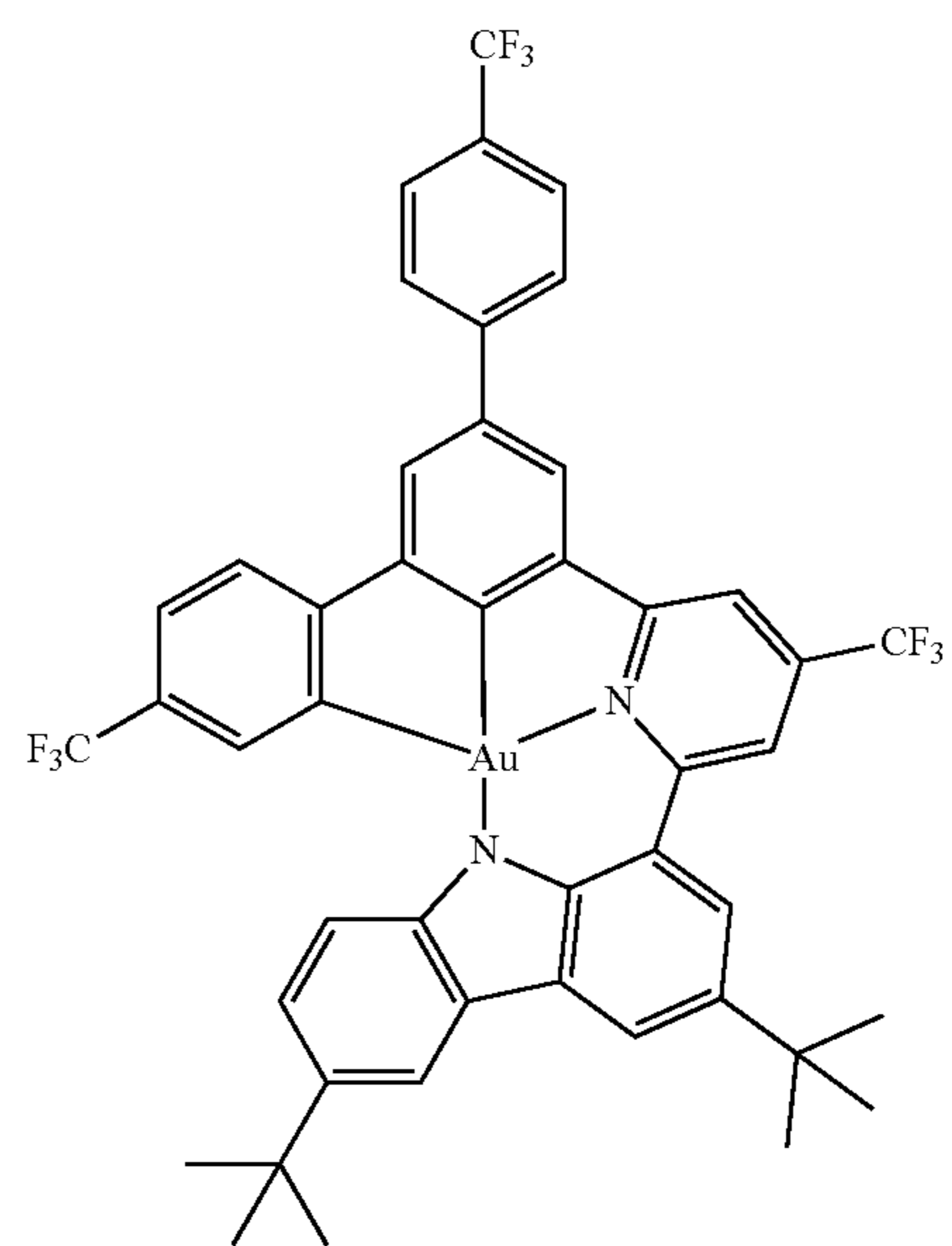
Compound 132
