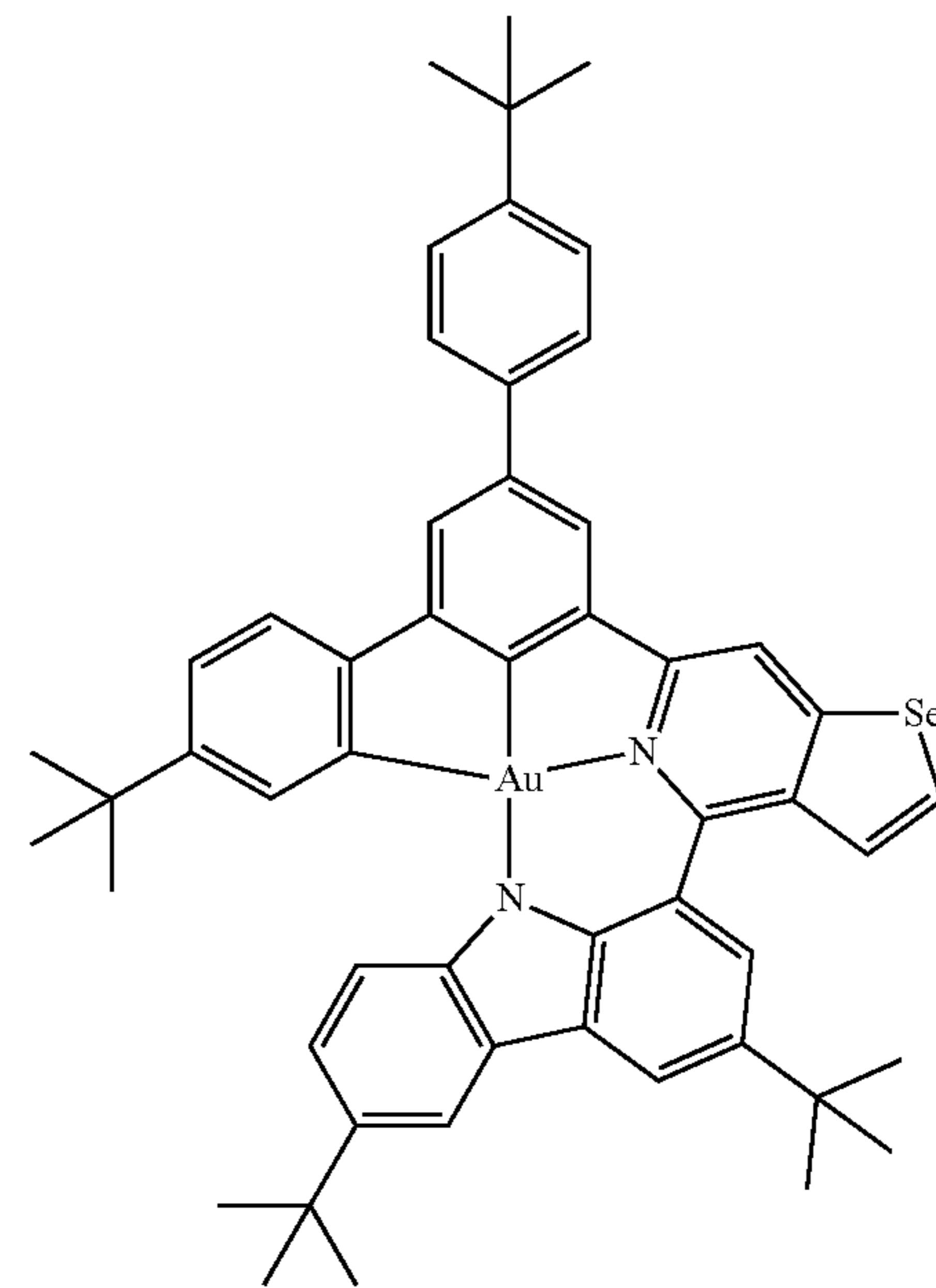
Compound 152
