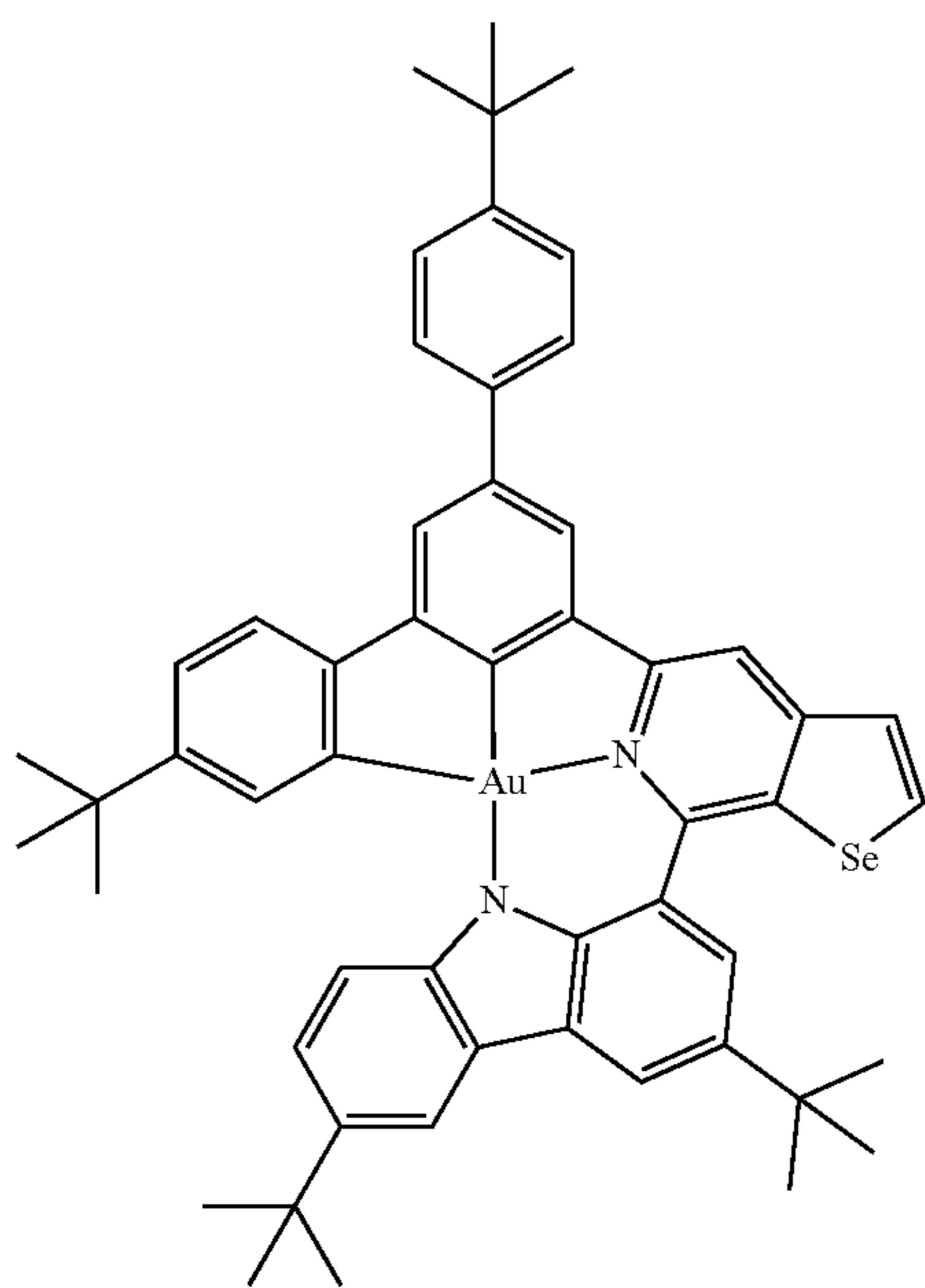
Compound 151
