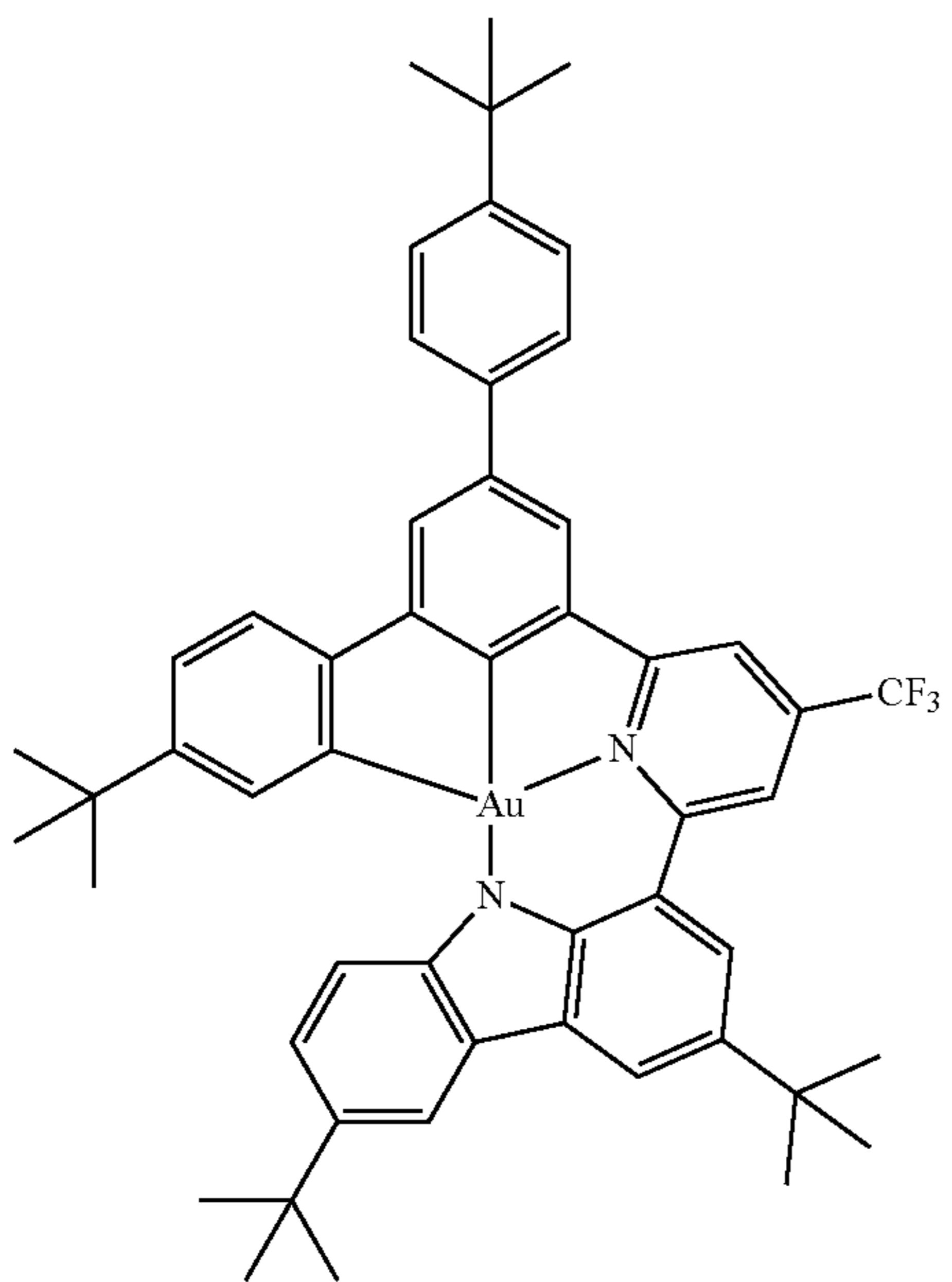
Compound 130
