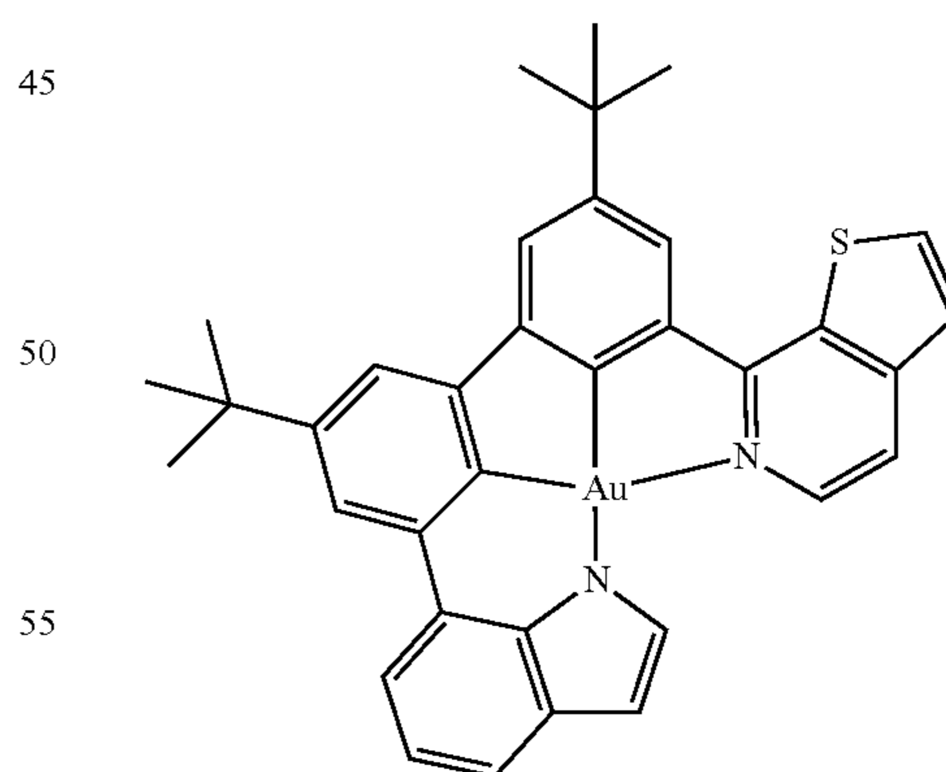
Compound 220
