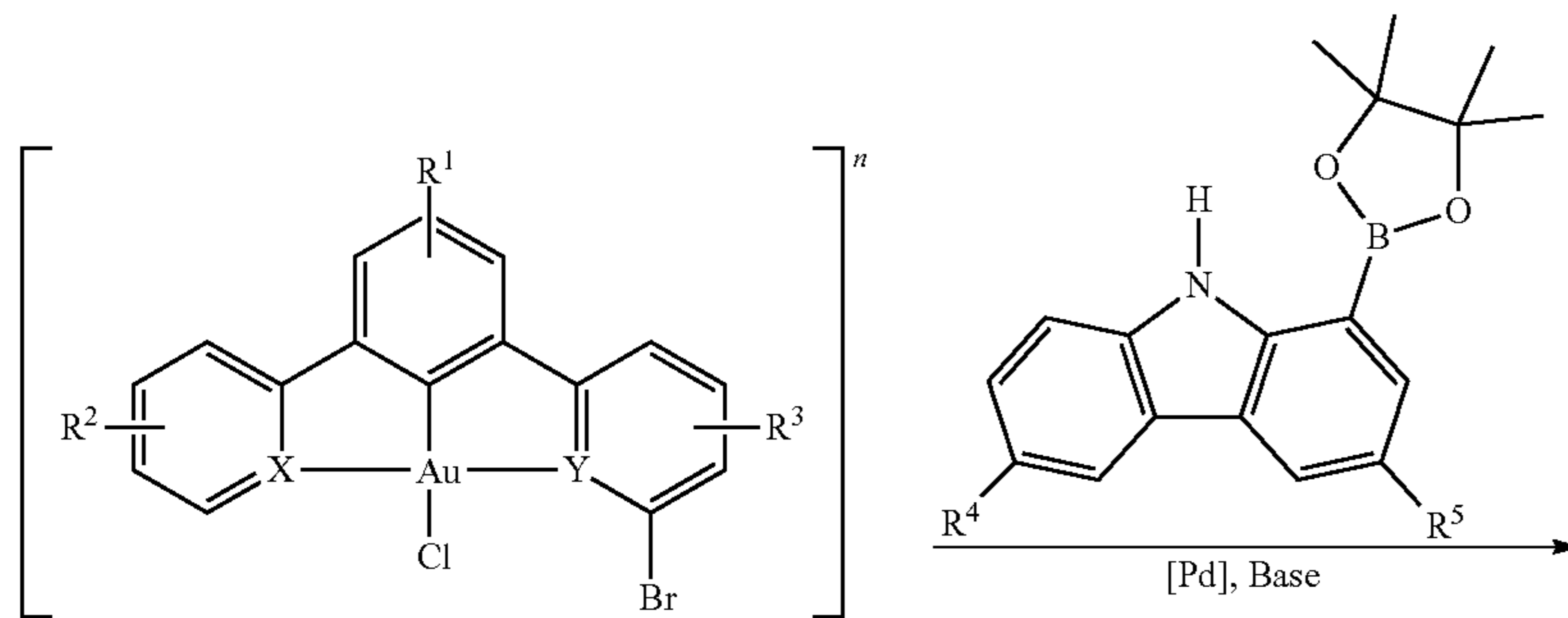
Scheme 1
