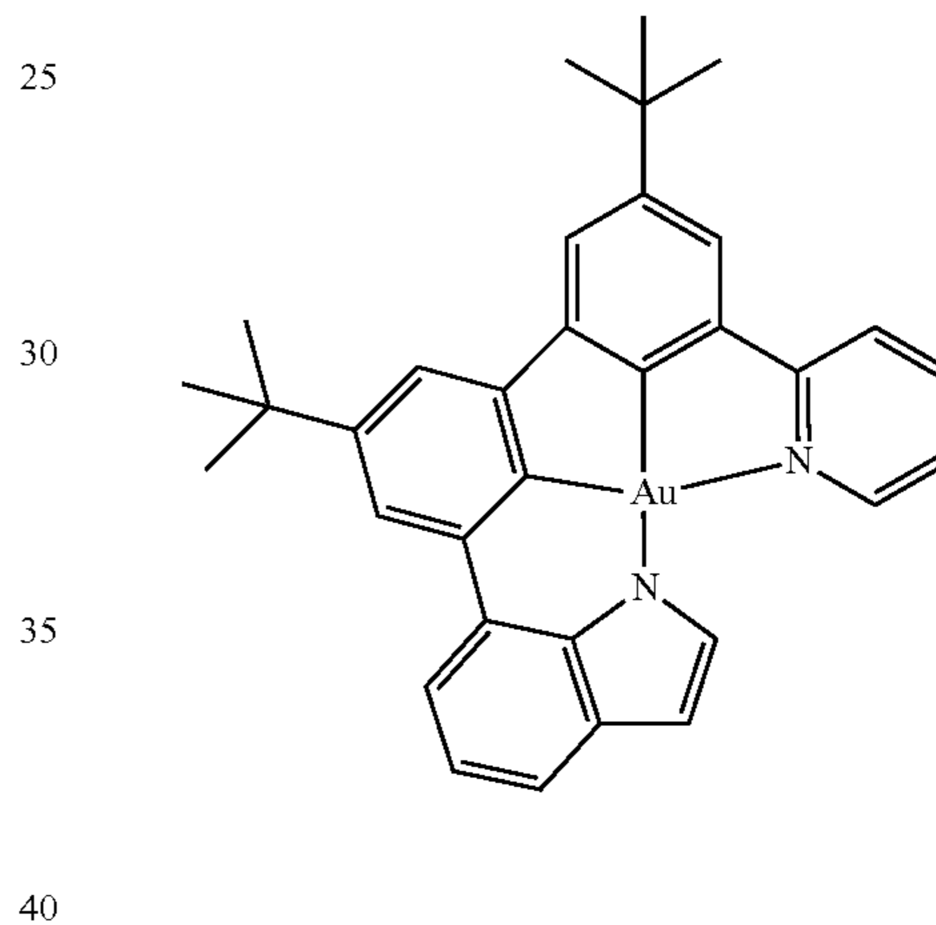
Compound 216
