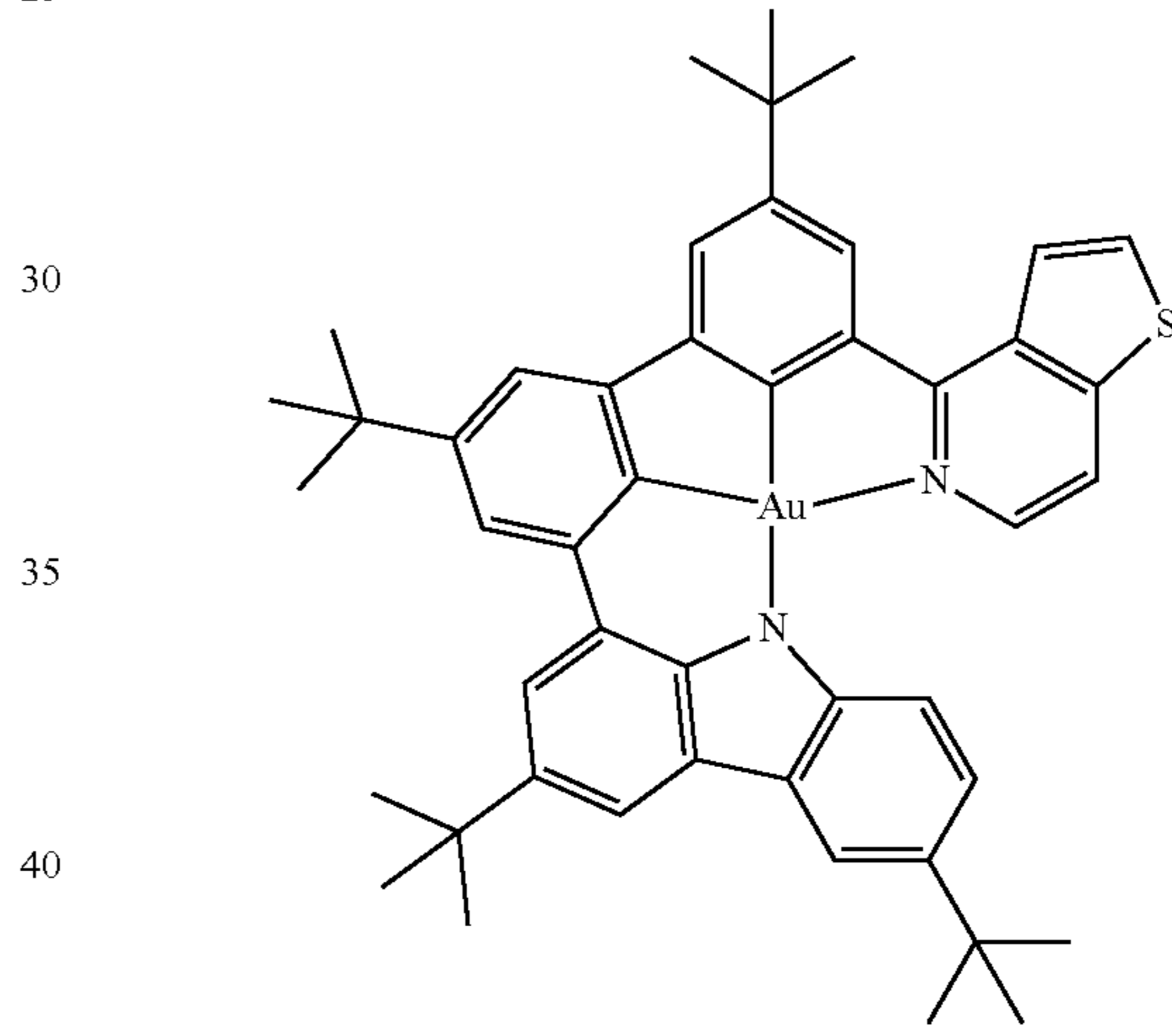
Compound 158
