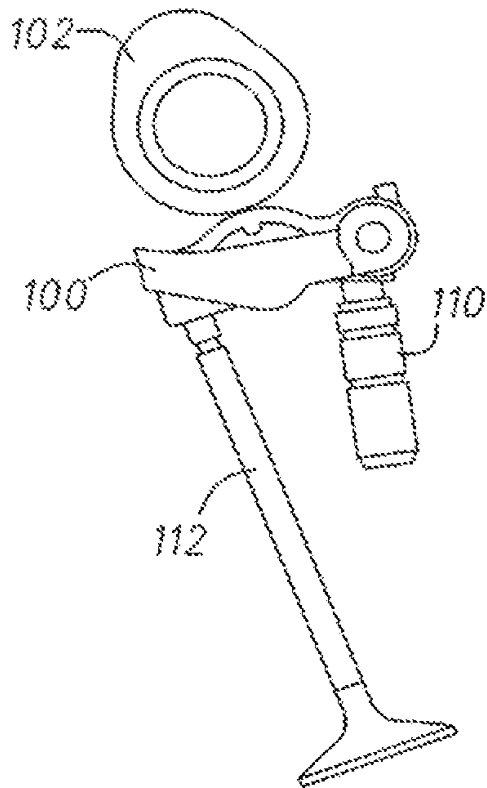
DVVL INTAKE VALVE LINE
