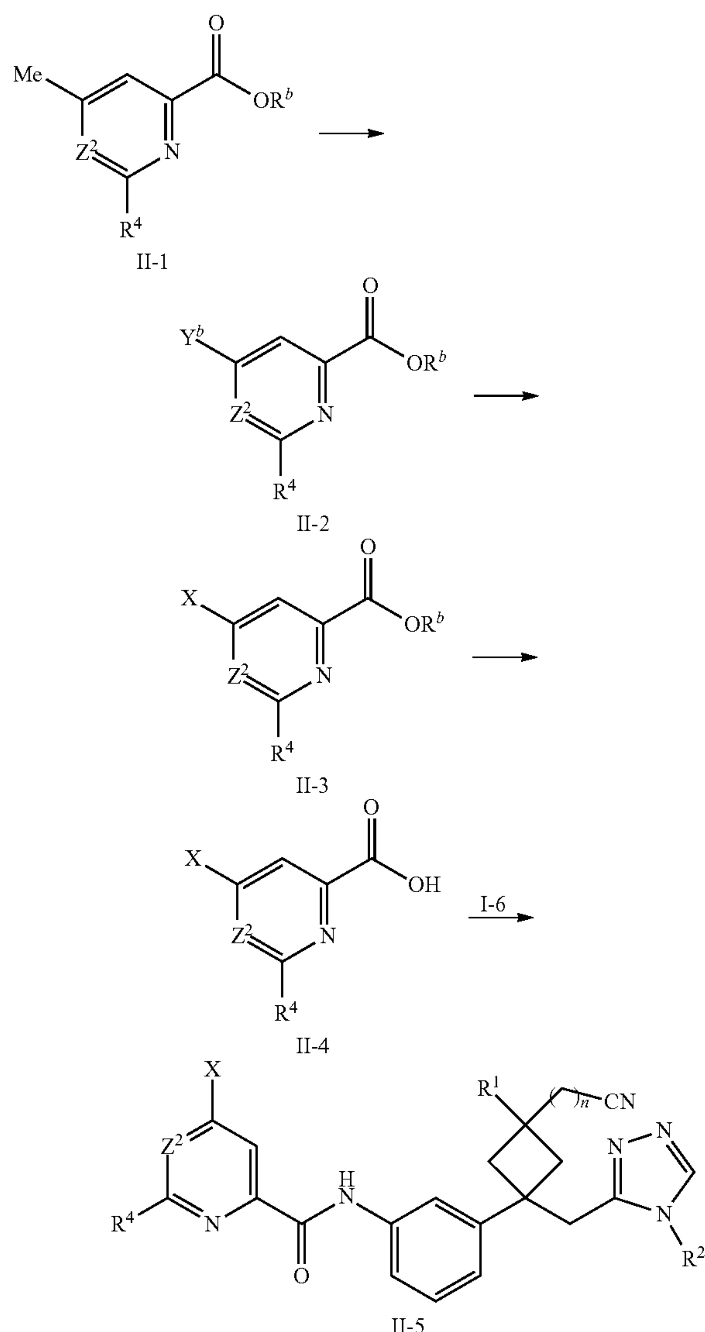
Scheme II.
