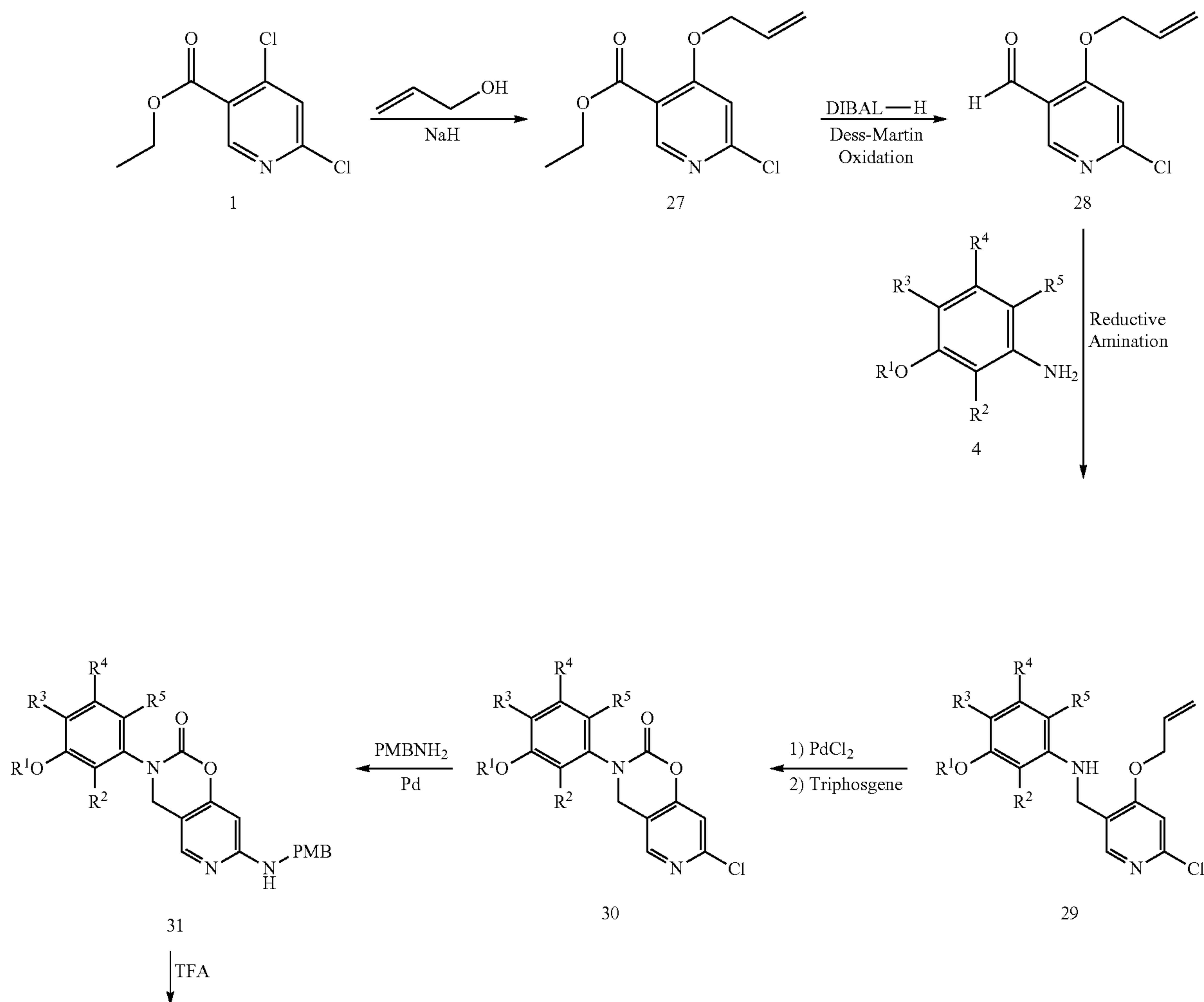
Scheme 6
