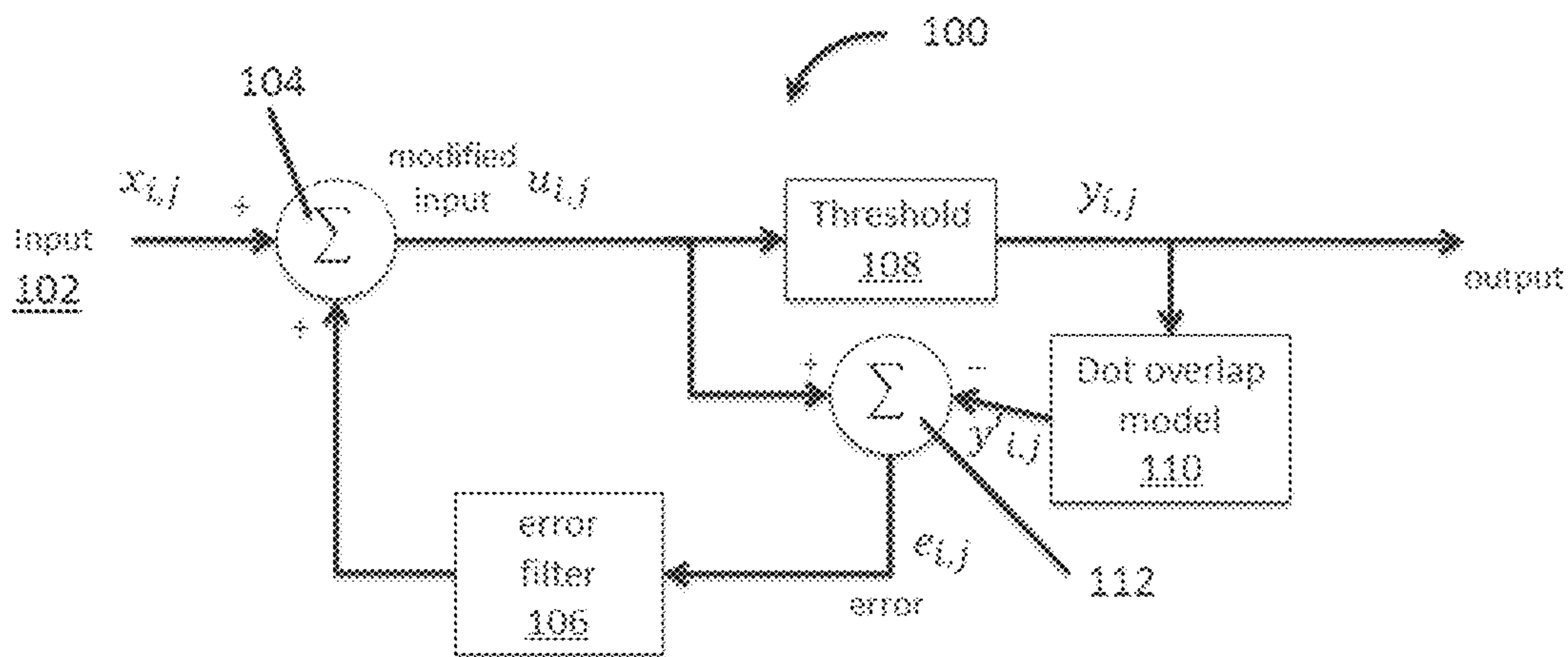
Fig. 1 (Prior Art)
