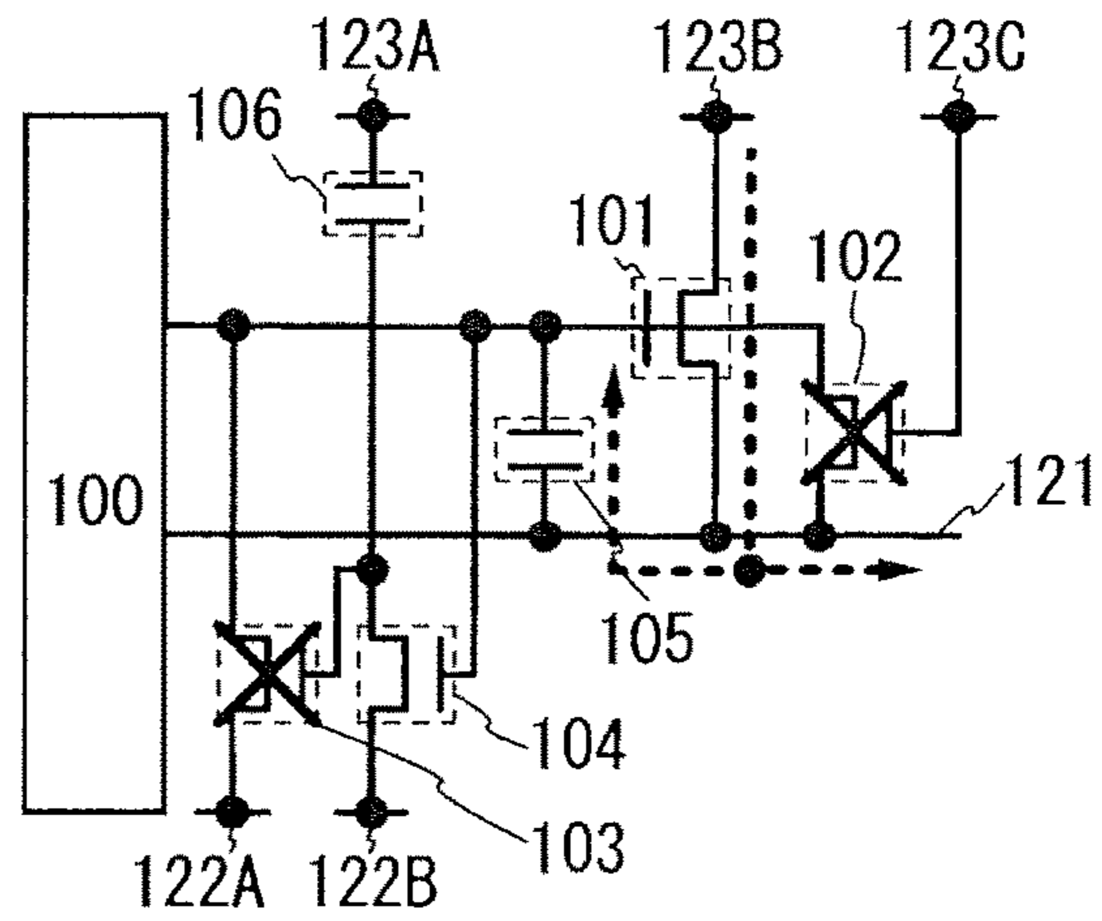
FIG. 2D PERIOD T4
