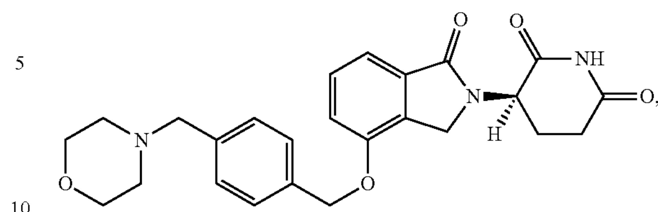
Compound IB
