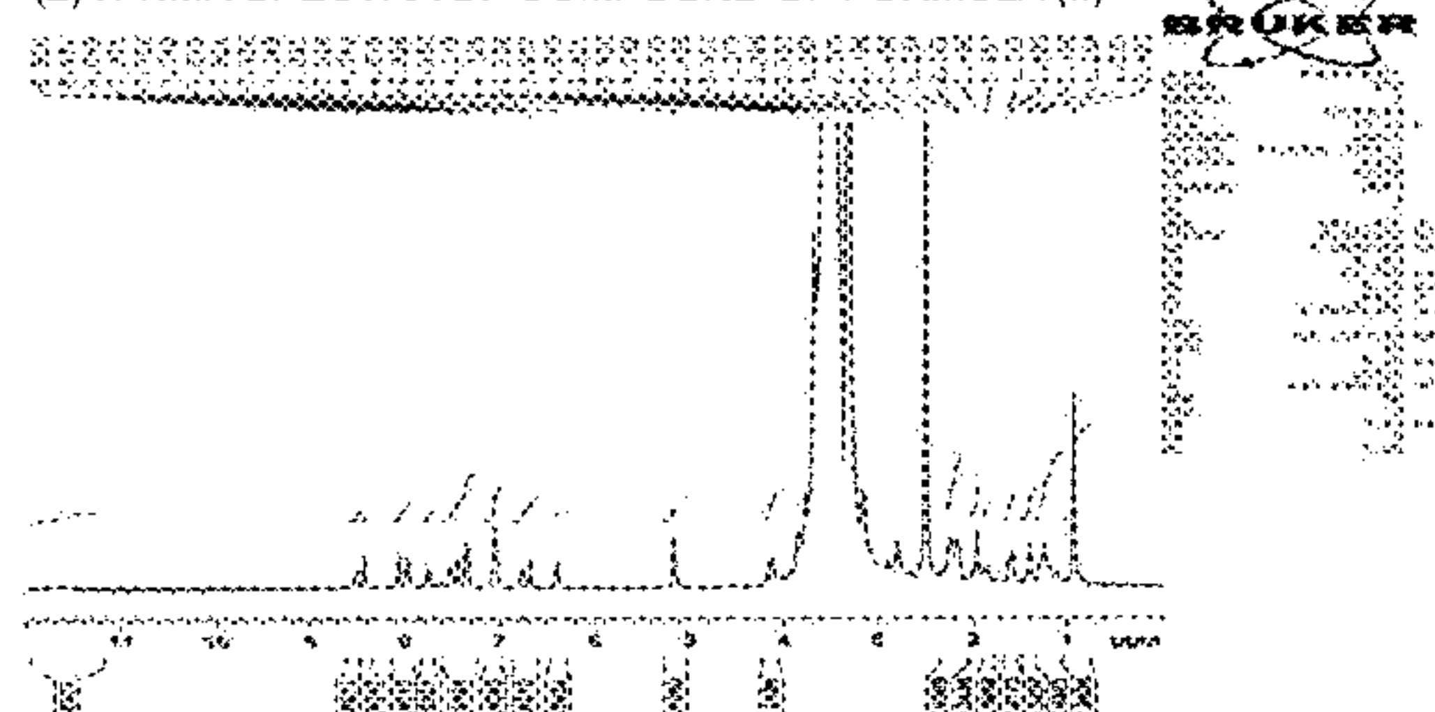
(2) H-NMR SPECTRA OF COMPOUND OF FORMULA (II)
