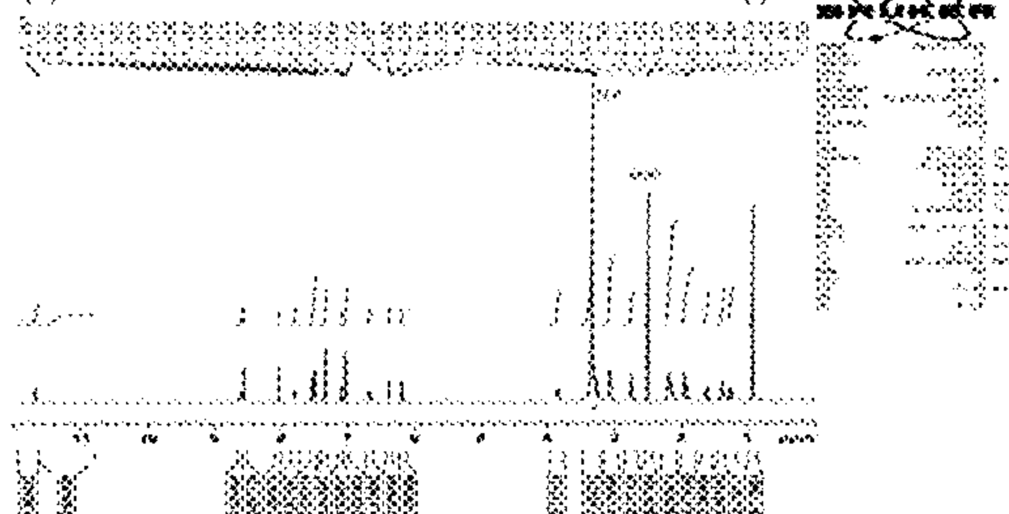
(1) H-NMR SPECTRA OF COMPOUND OF FORMULA (I)
