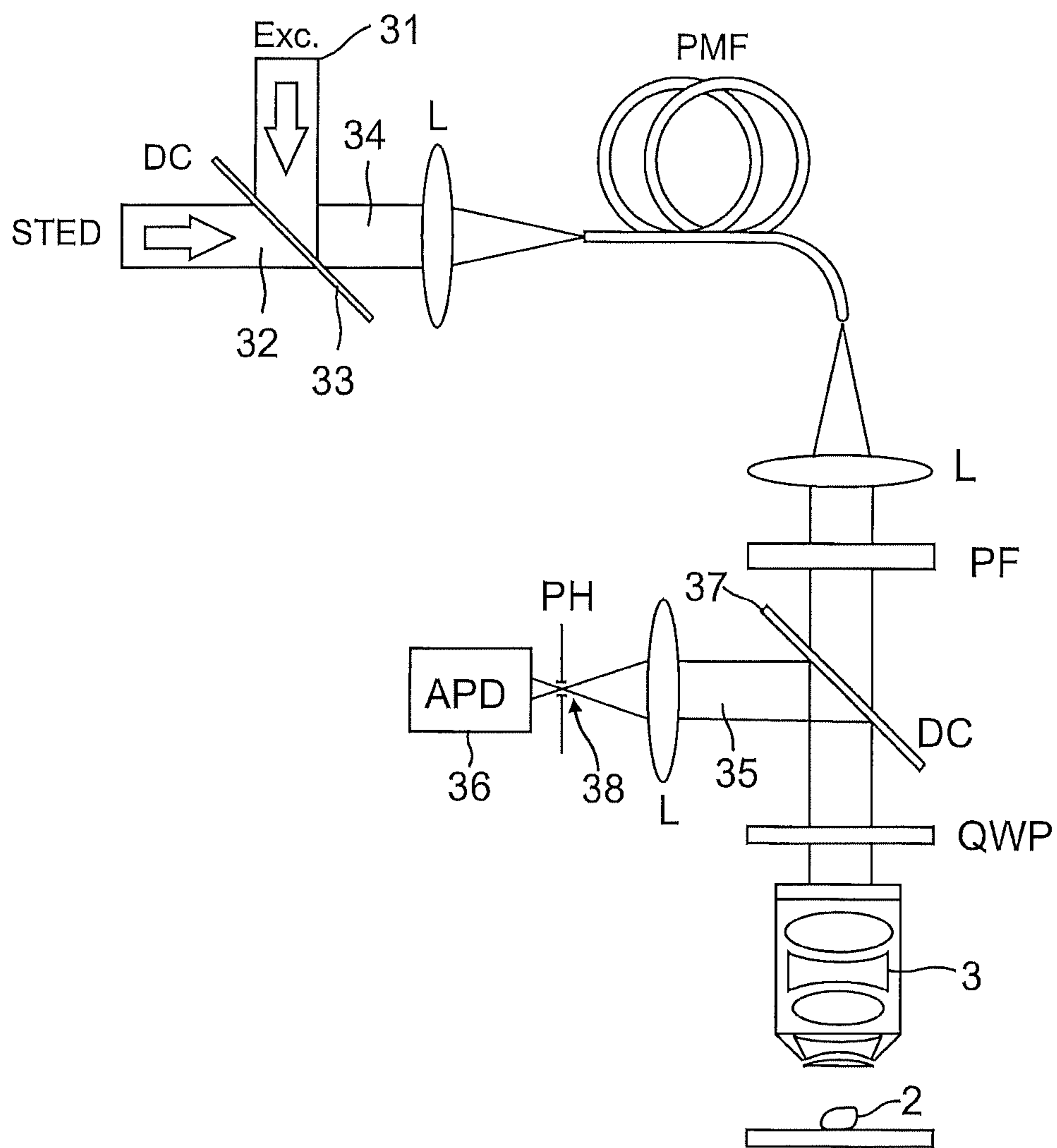
FIG. 6 (Prior Art)
