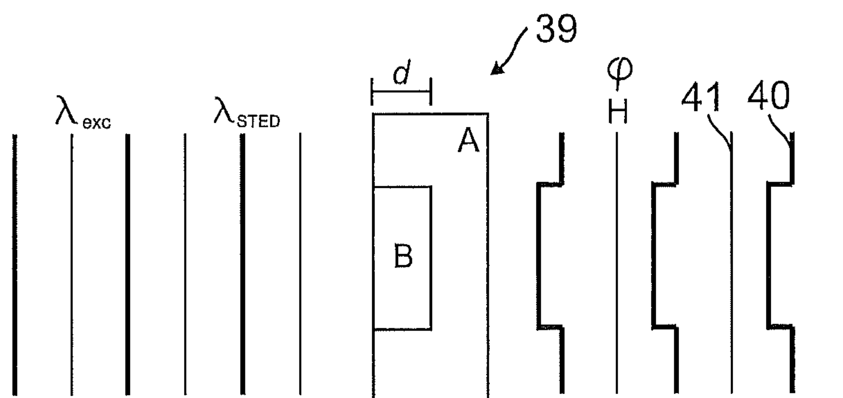
FIG. 7 (Prior Art)
