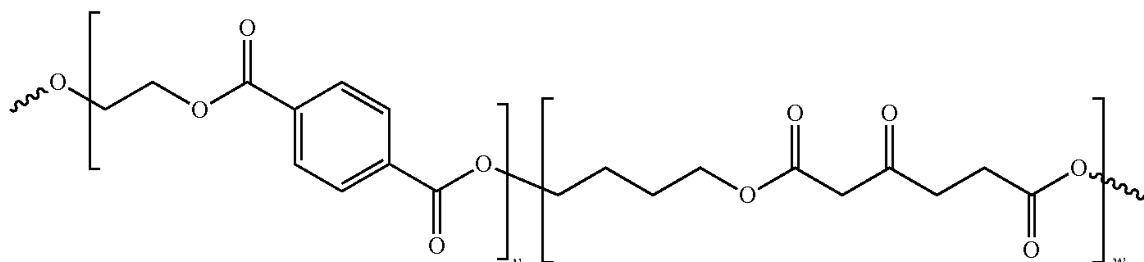
Scheme 1
