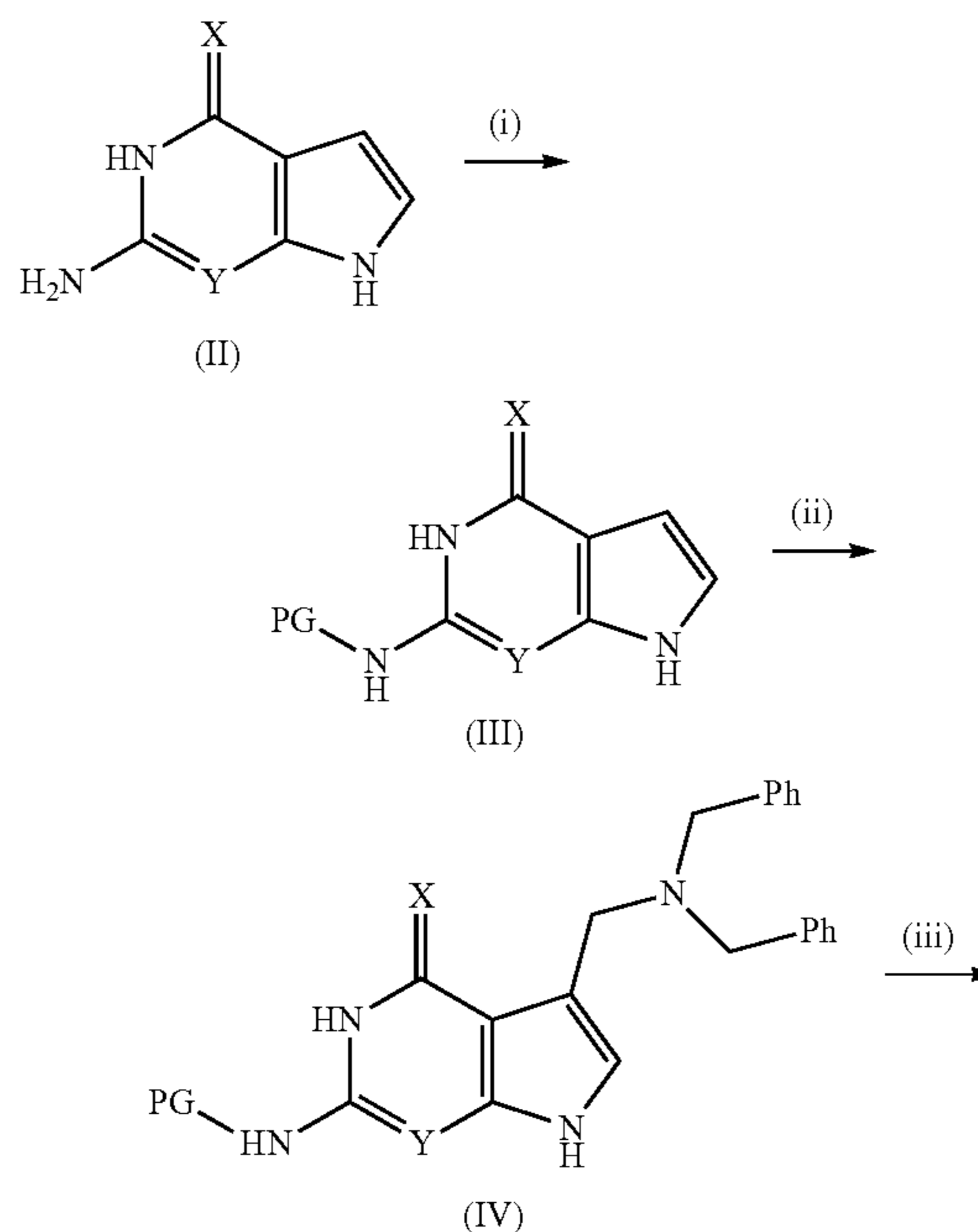
Scheme 1
